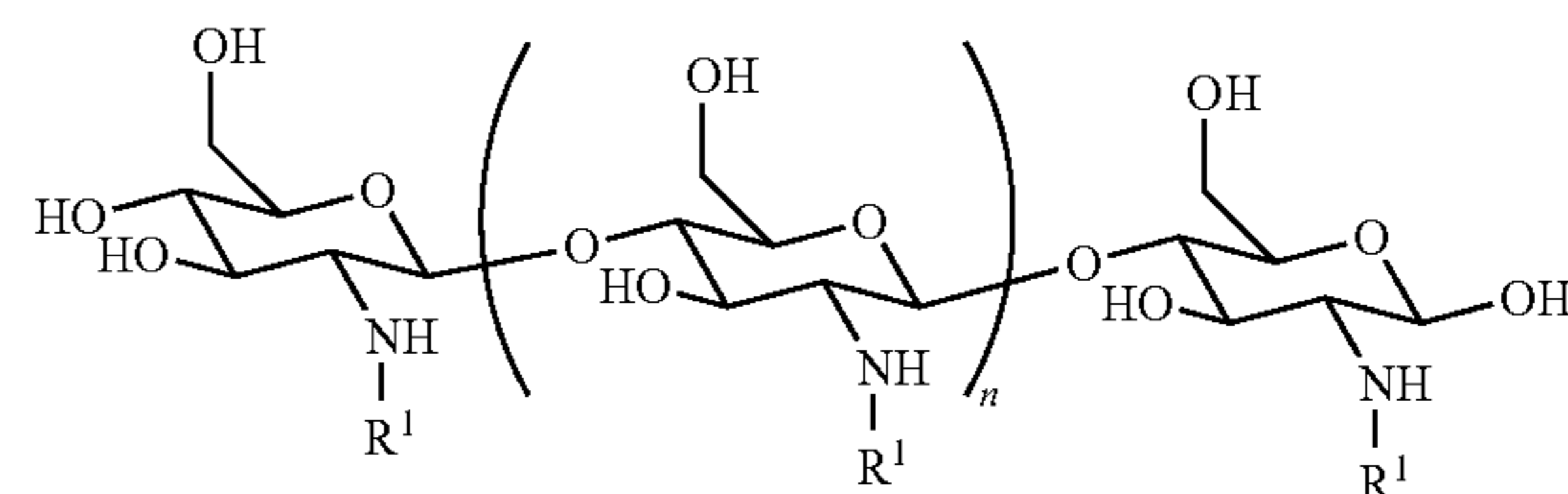
formula (I)
