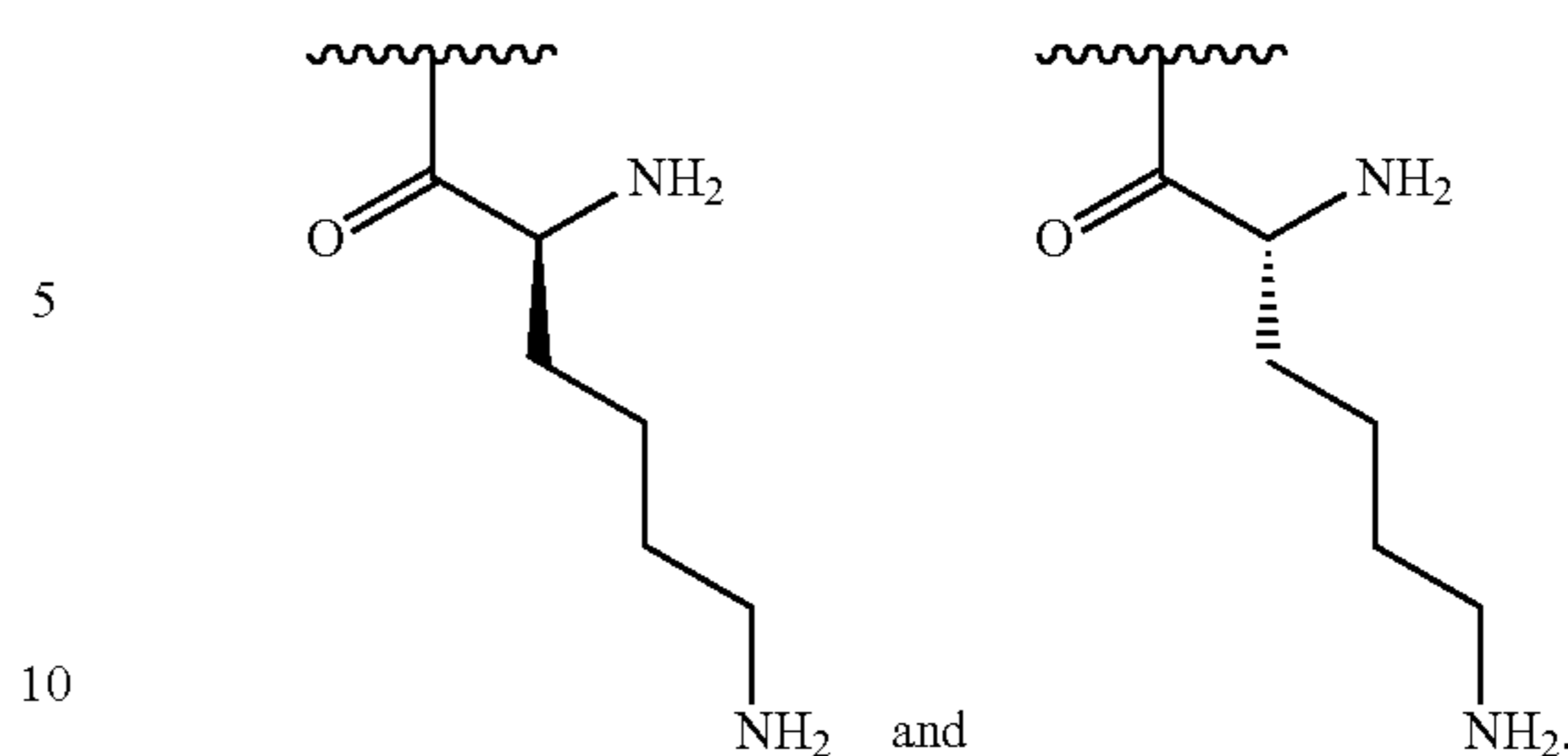
formula (II)
