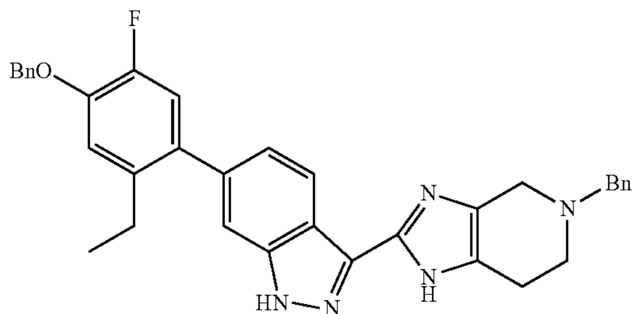
(a) 5-Benzyl-2-(6-(4-(benzyloxy)-2-ethyl-5-fluorophenyl)-1H-indazol-3-yl)-4,5,6,7-tetrahydro-1H-imidazo[4,5-c]pyridine
