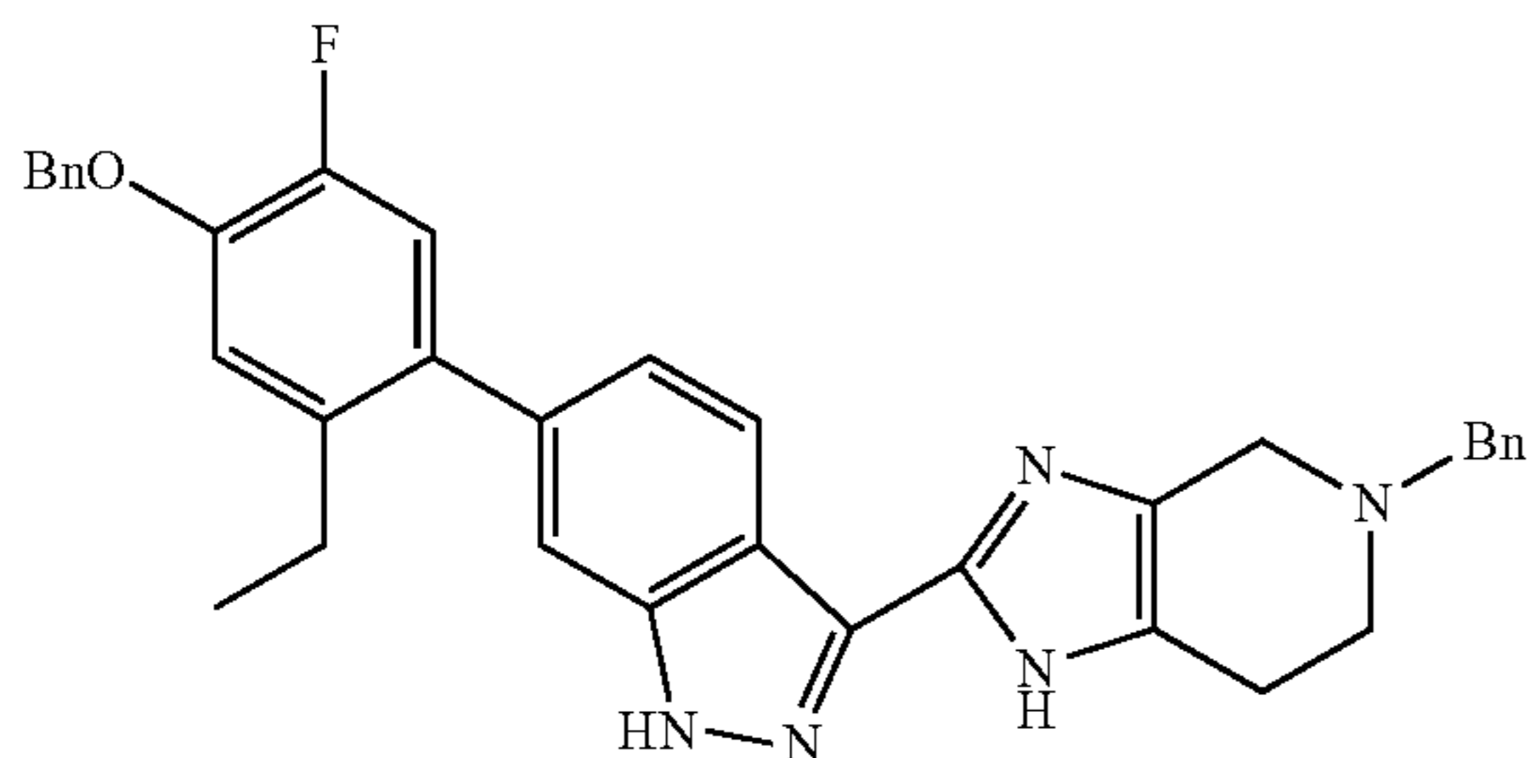
(a) 5-Benzyl-2-(6-(4-(benzyloxy)-2-ethyl-5-fluorophenyl)-1H-indazol-3-yl)-4,5,6,7-tetrahydro-1H-imidazo[4,5-c]pyridine
