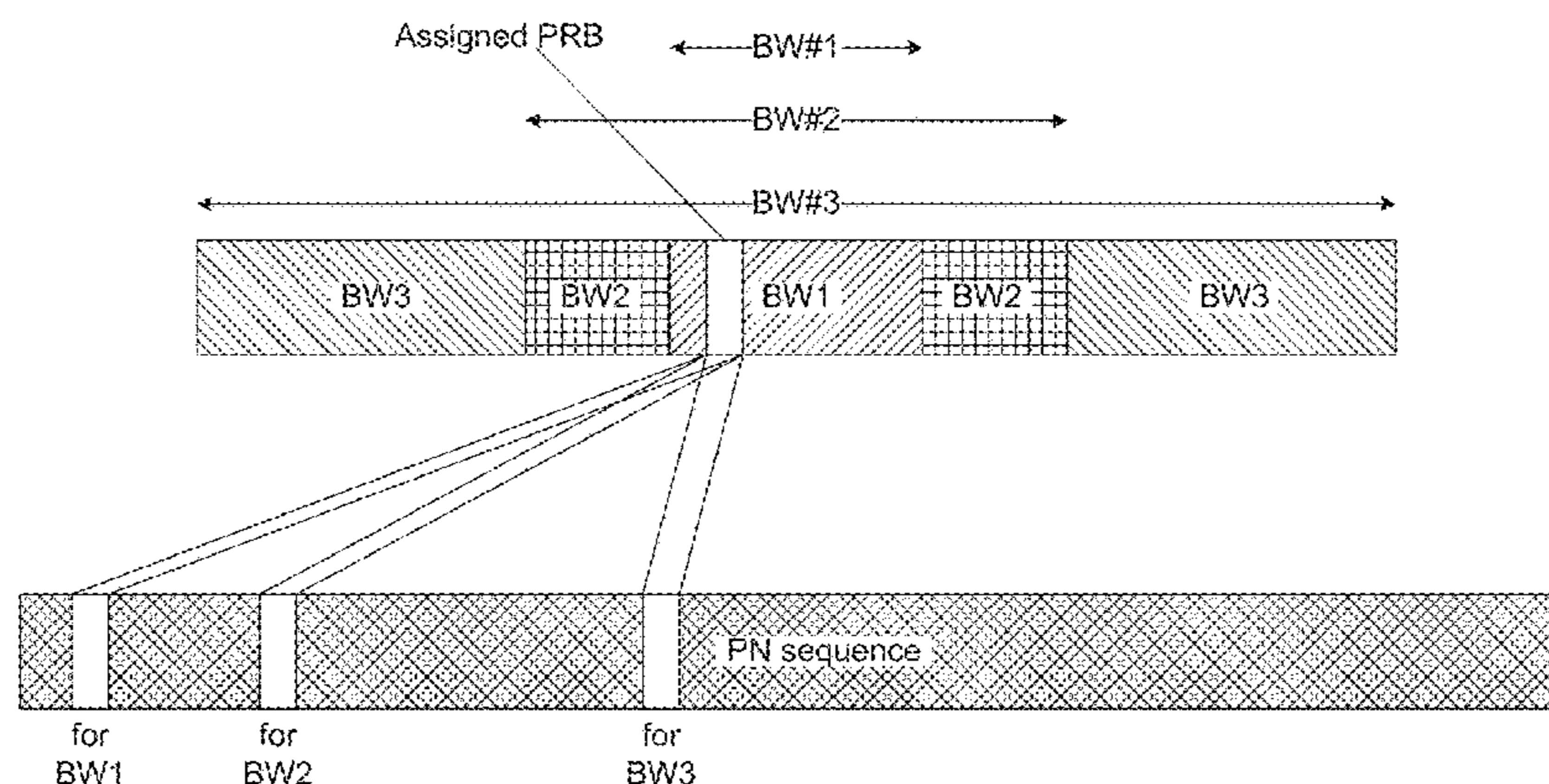
PN sequence generated for the maximum system BW supported by current release
