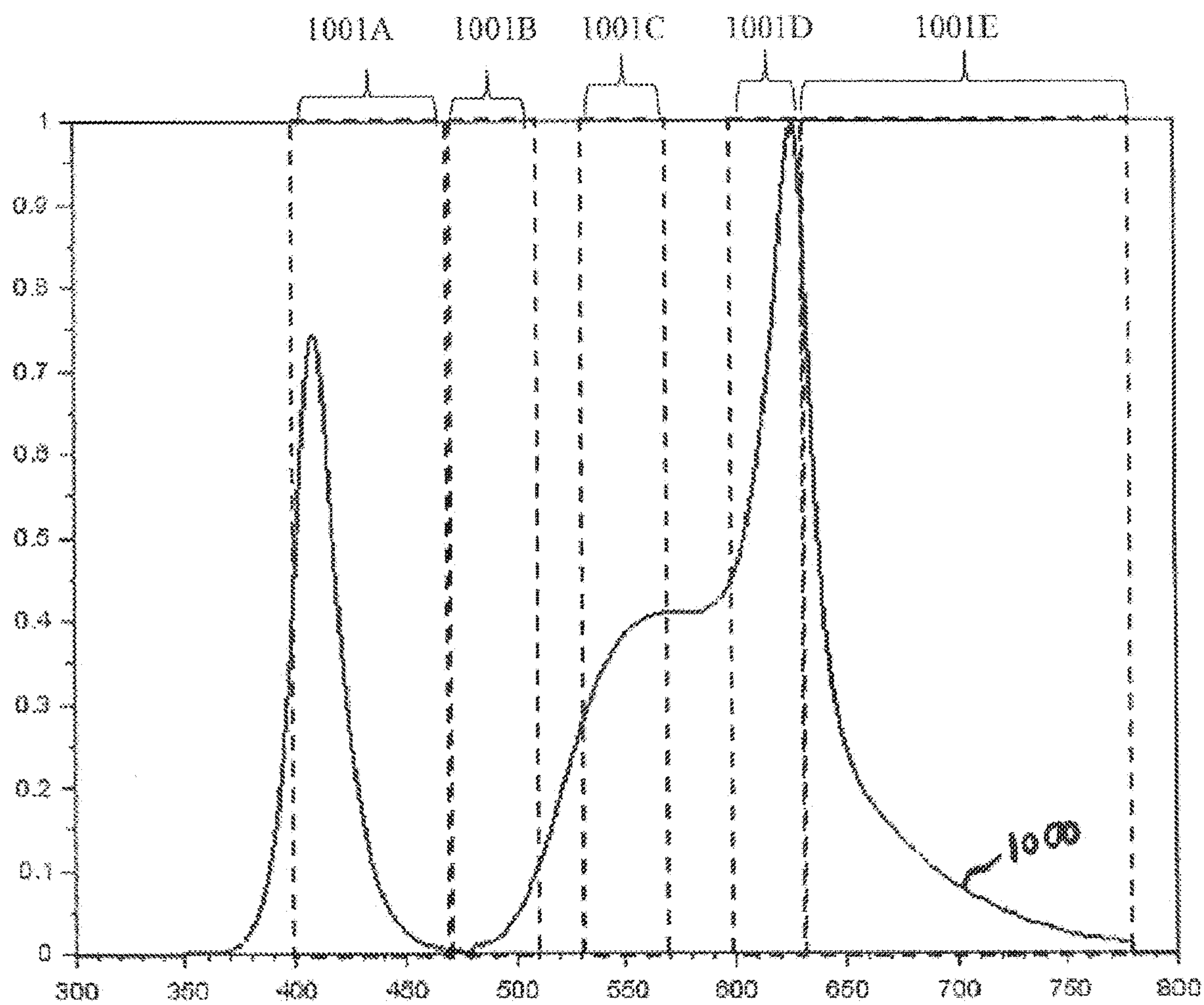
2400K Ch3: Normalized Output vs. Wavelength (nm)
