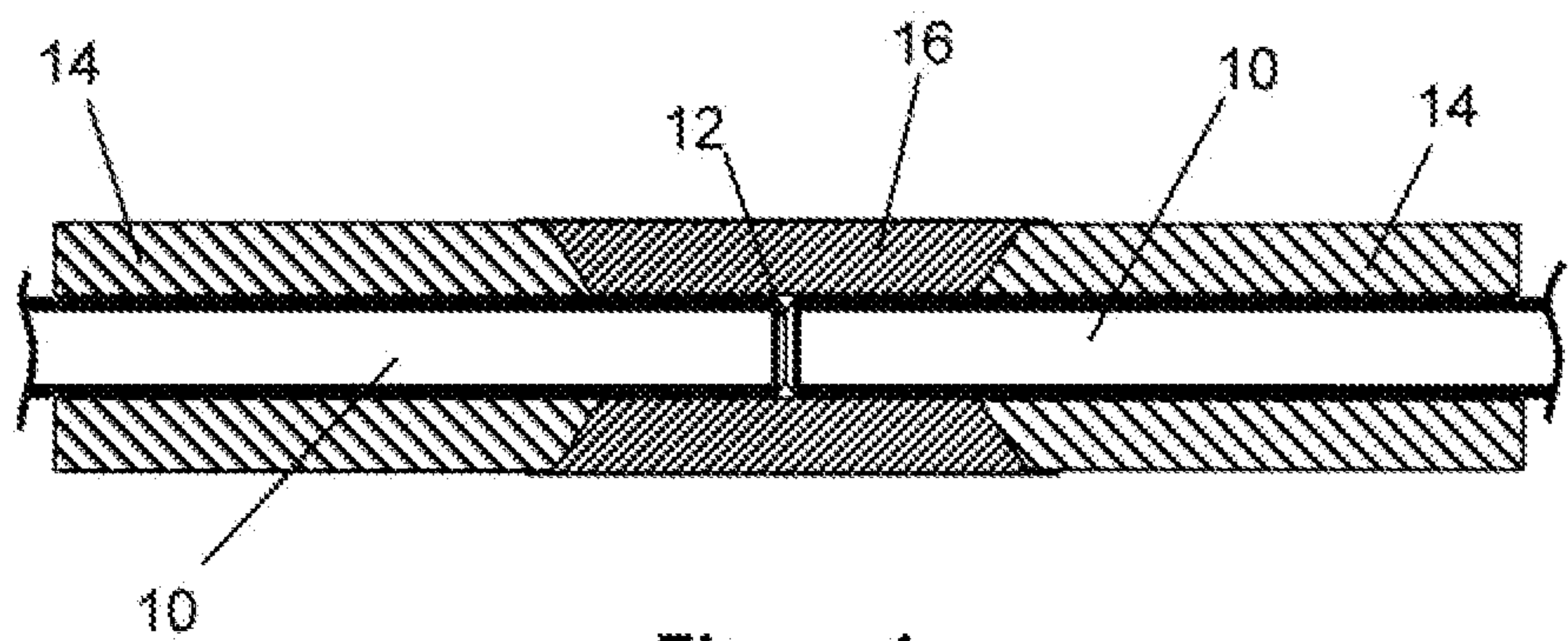
Figure 1 PRIOR ART
