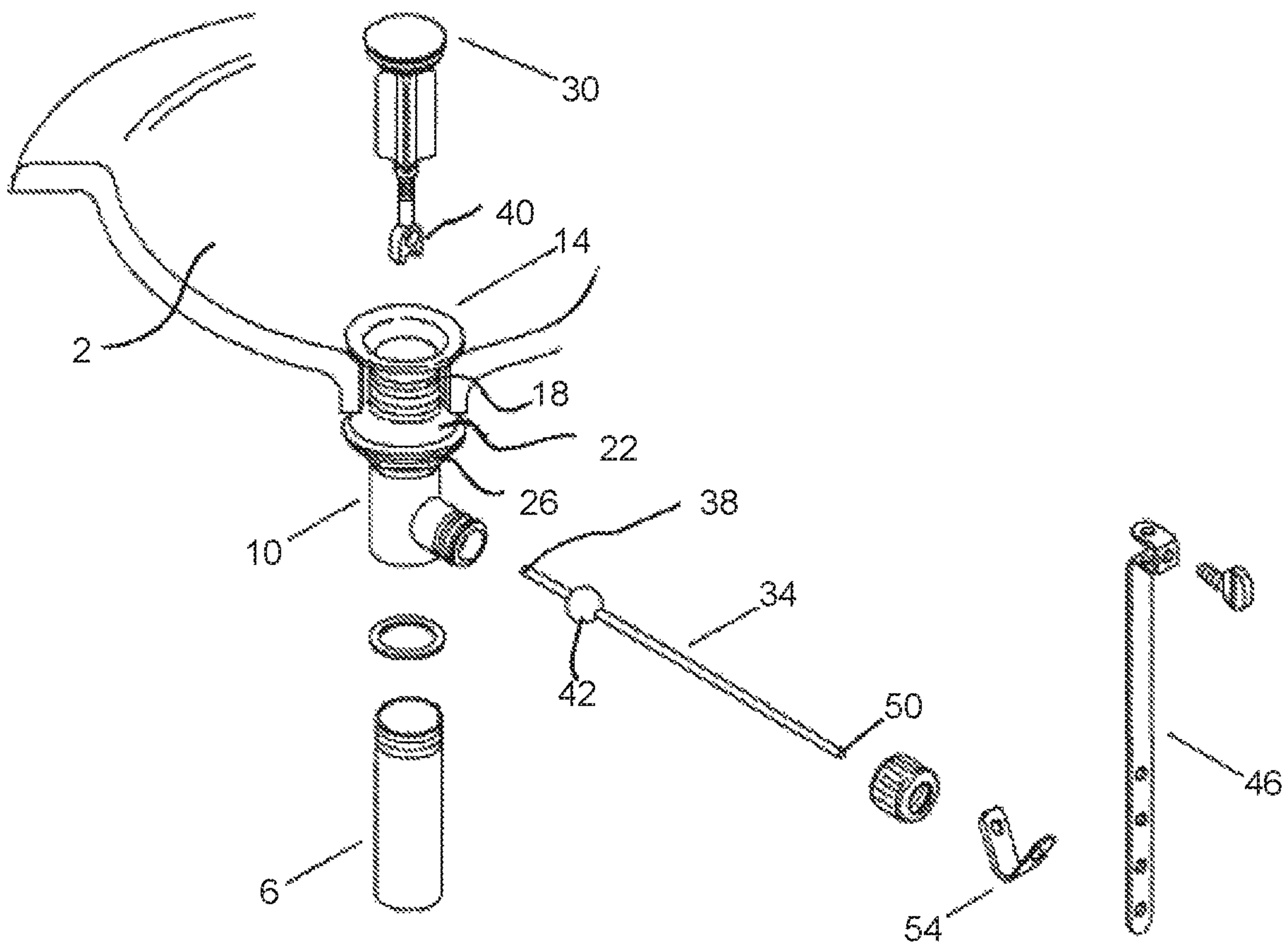
FIG. 1 (Prior Art)
