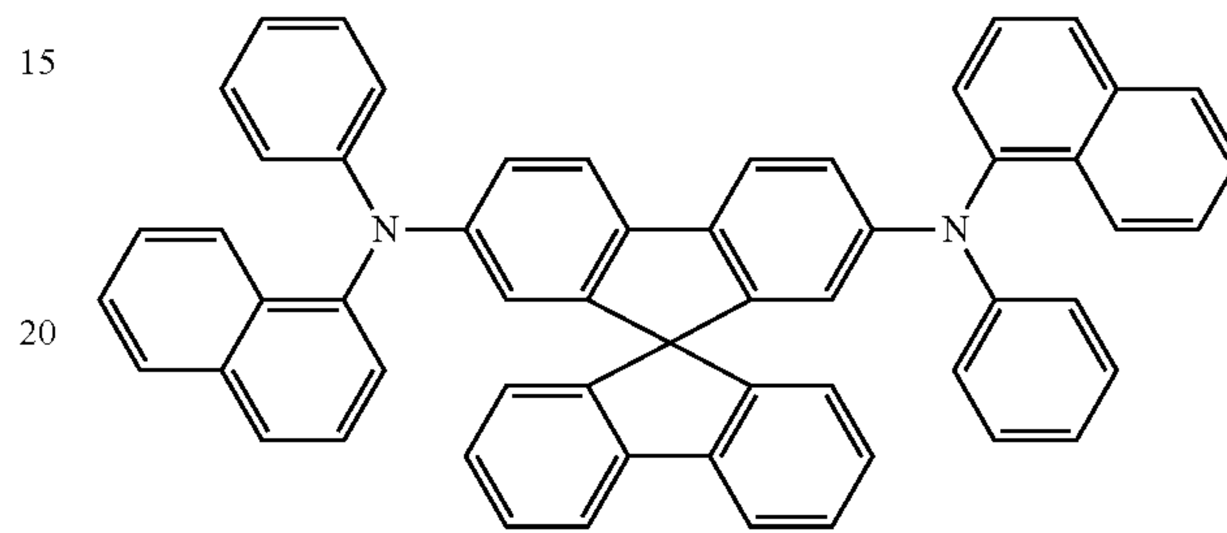
Spiro-NPB
