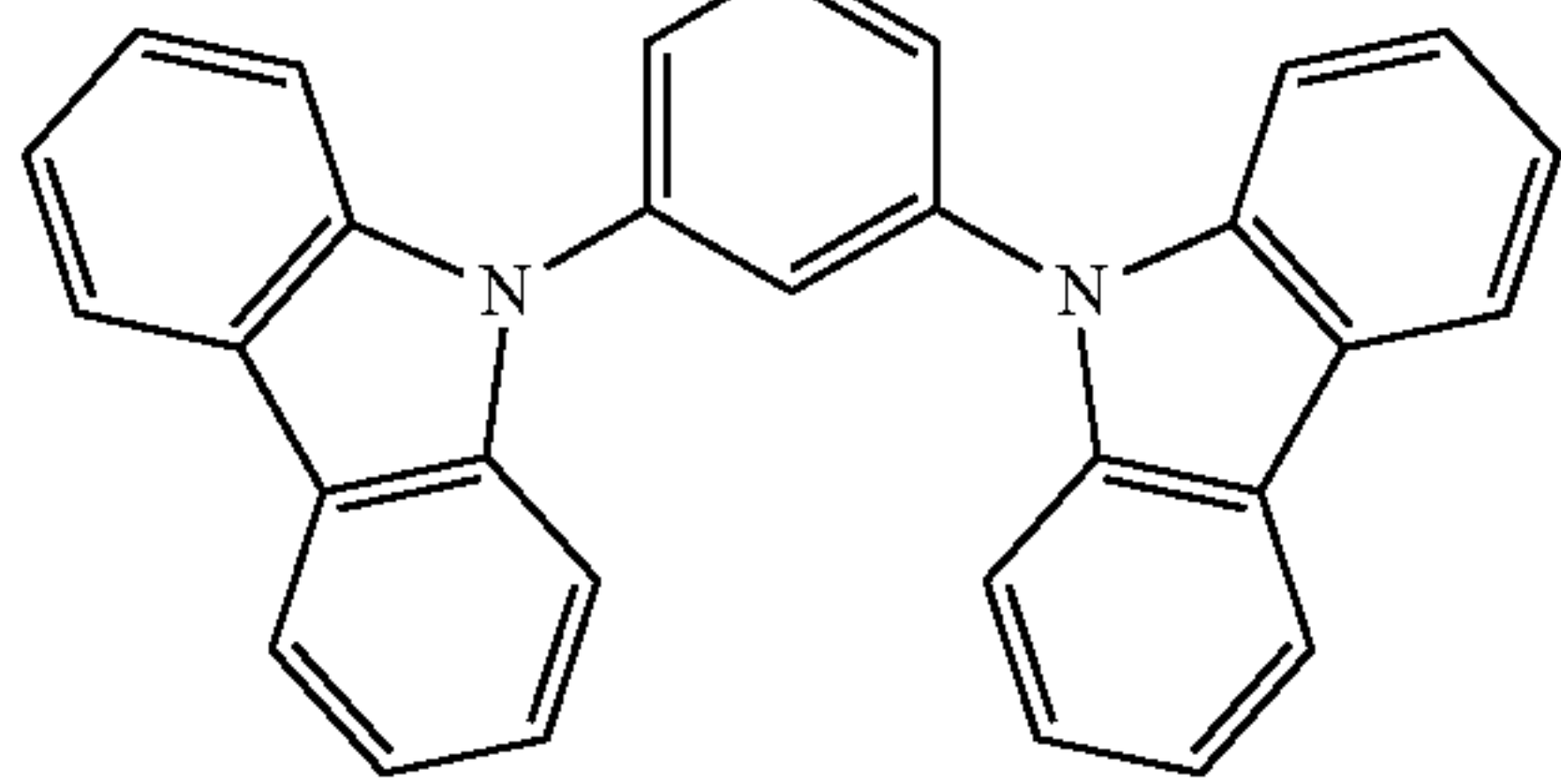
mCP
