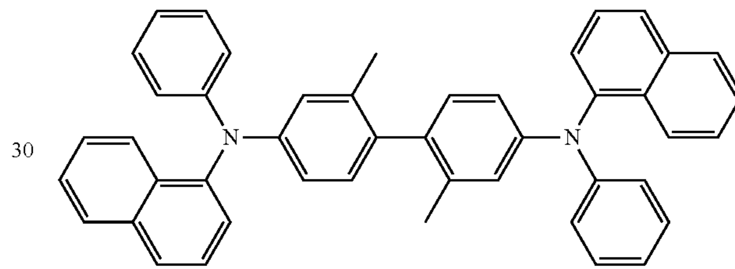
methylated NPB
