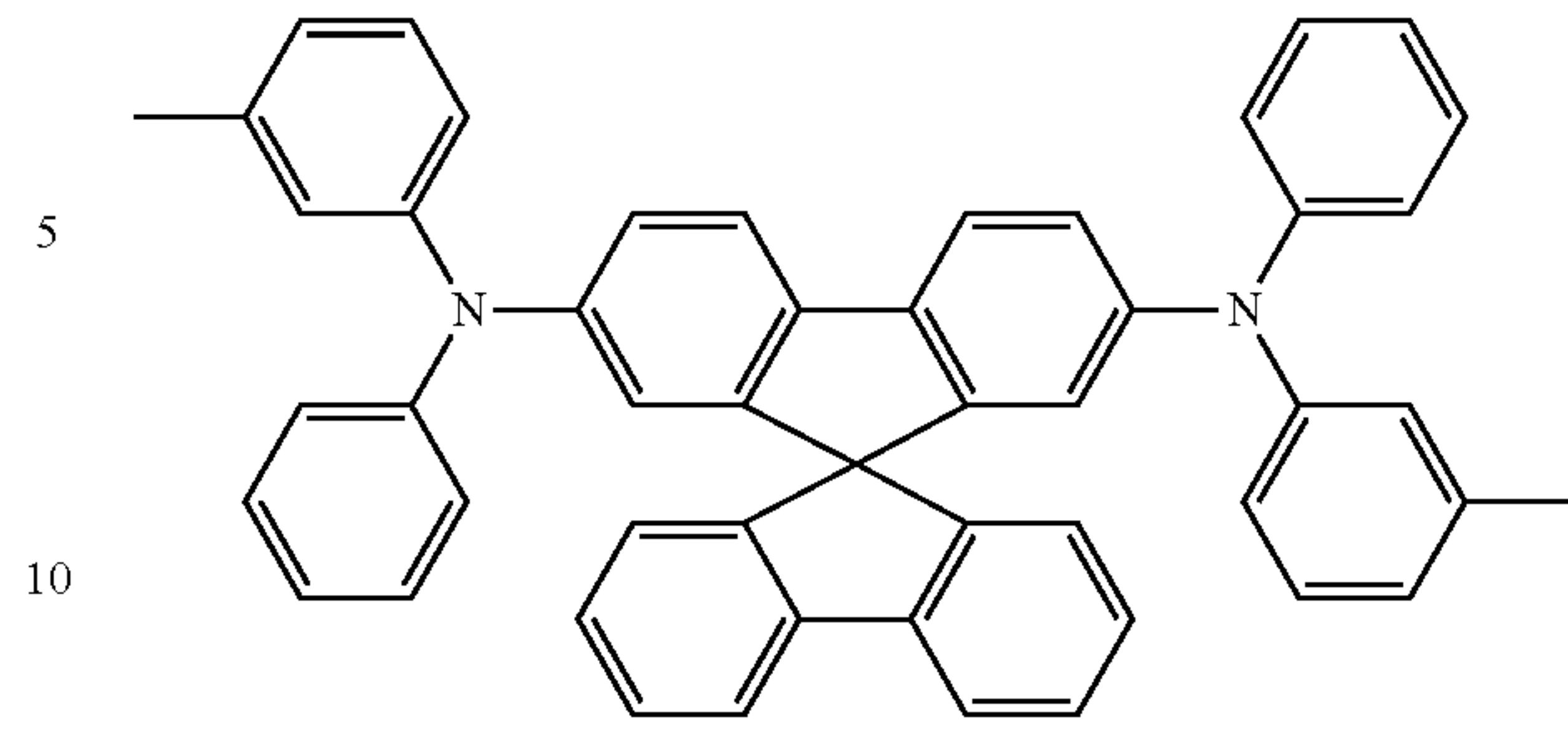
Spiro-TPD
