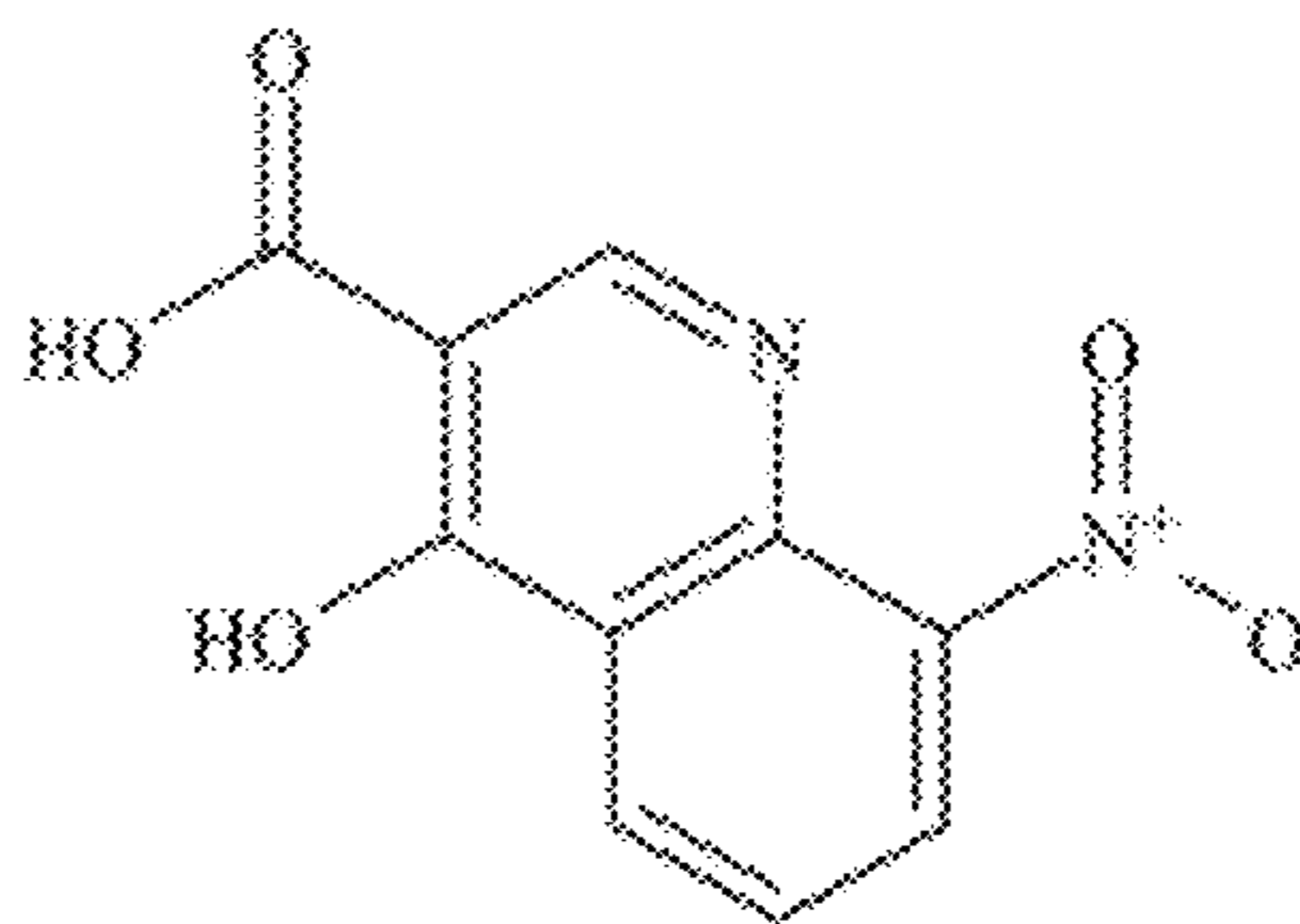
4-hydroxy-8-nitroquinoline-3-carboxylic acid
