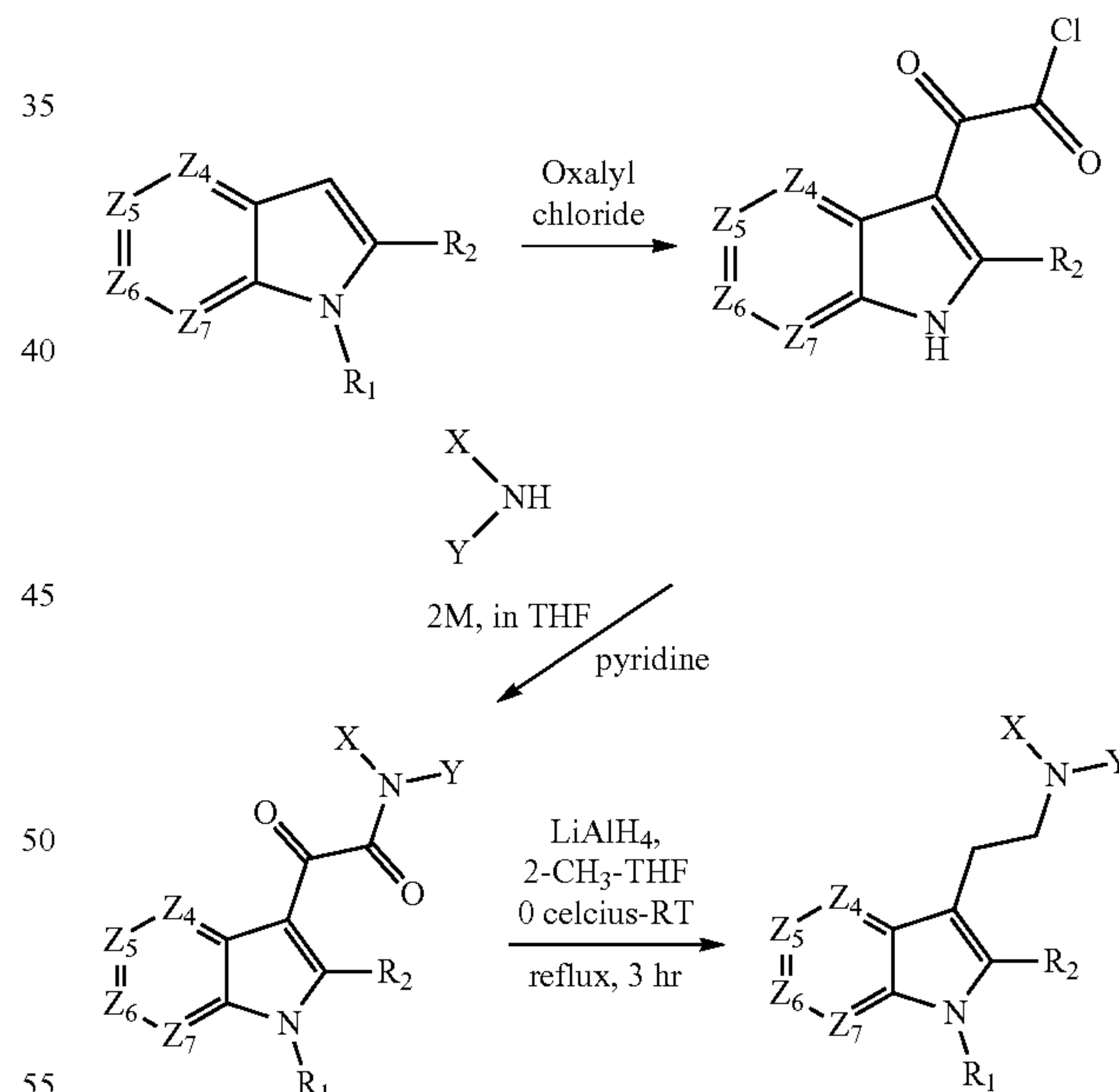
Scheme 1D
