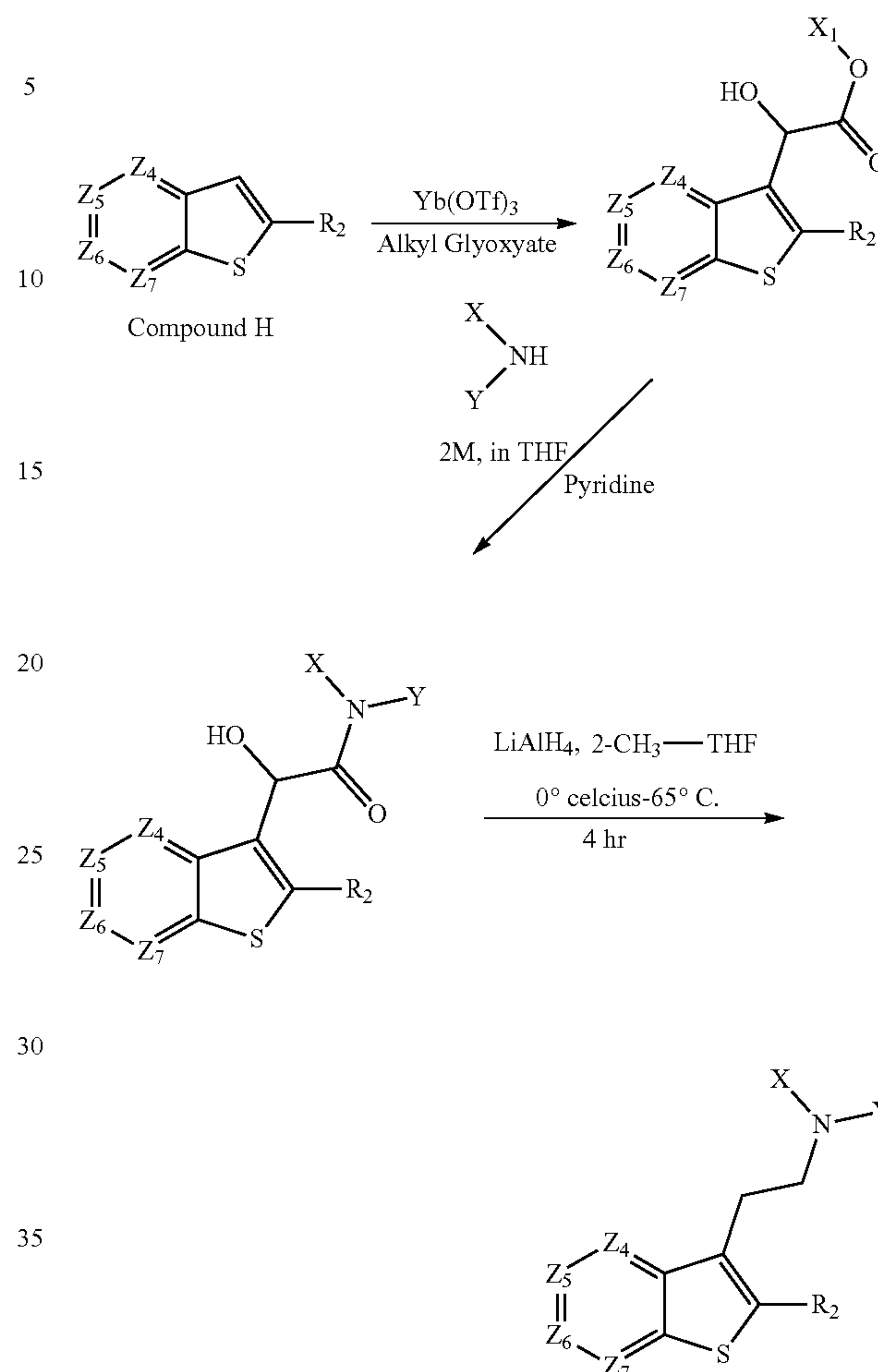
Scheme 4B
