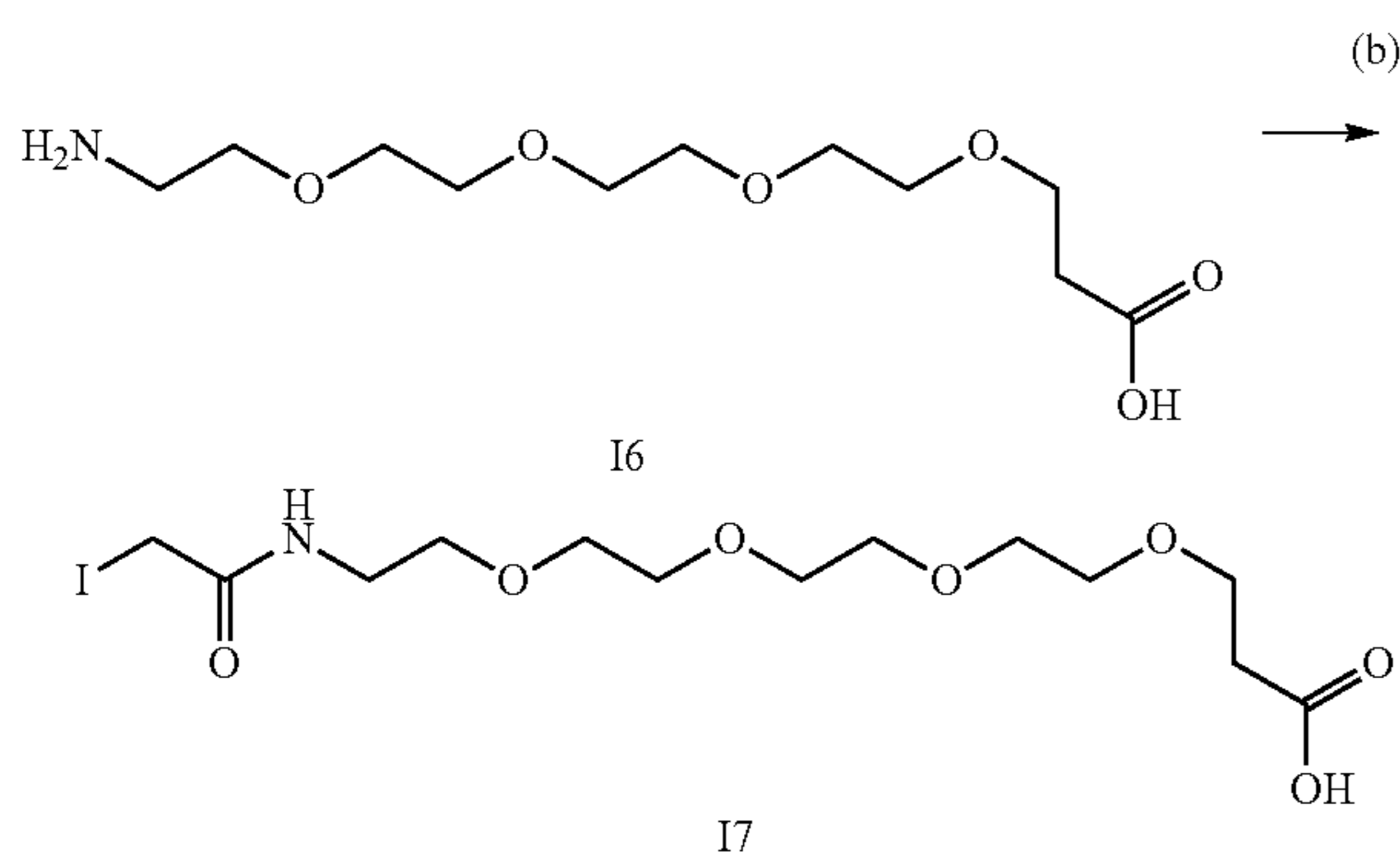
1-iodo-2-oxo-6,9,12,15-tetraoxa-3-azaocadecan-18-oic acid (17)
