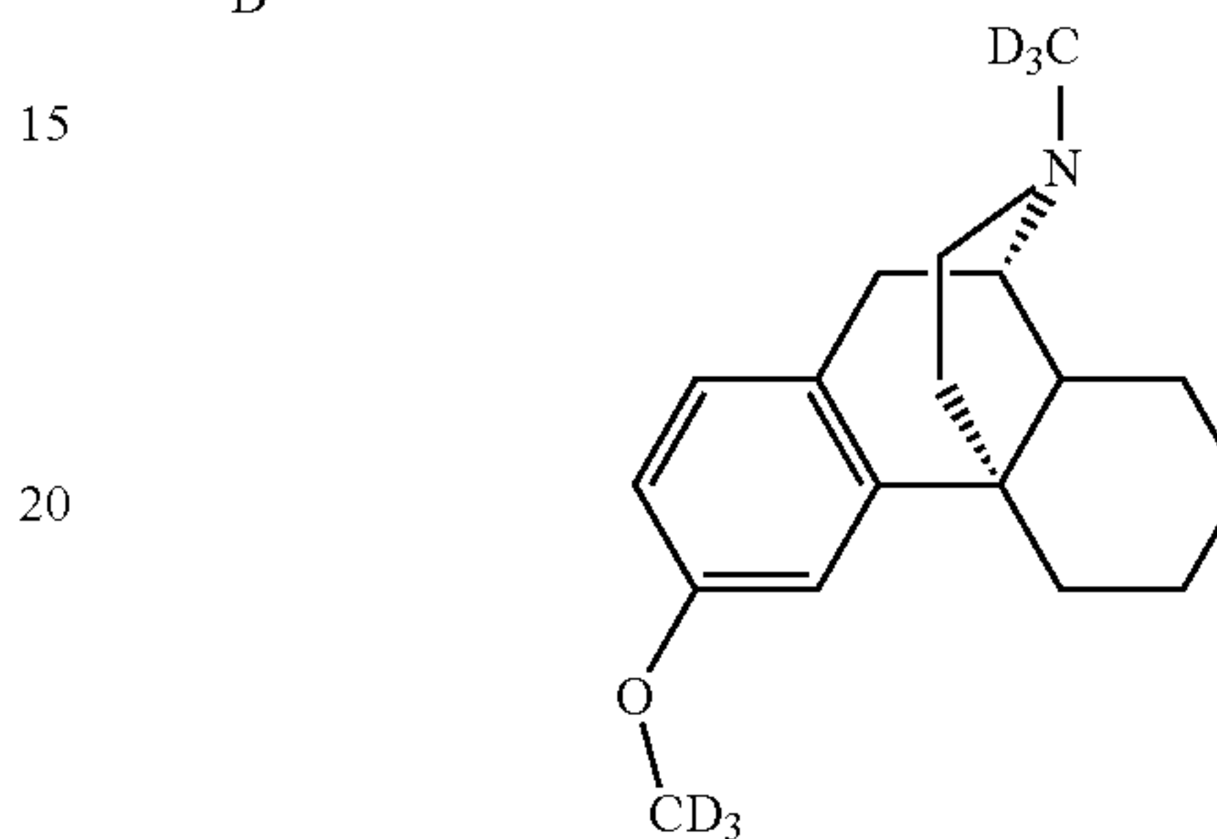
d6-dextromethorphan
