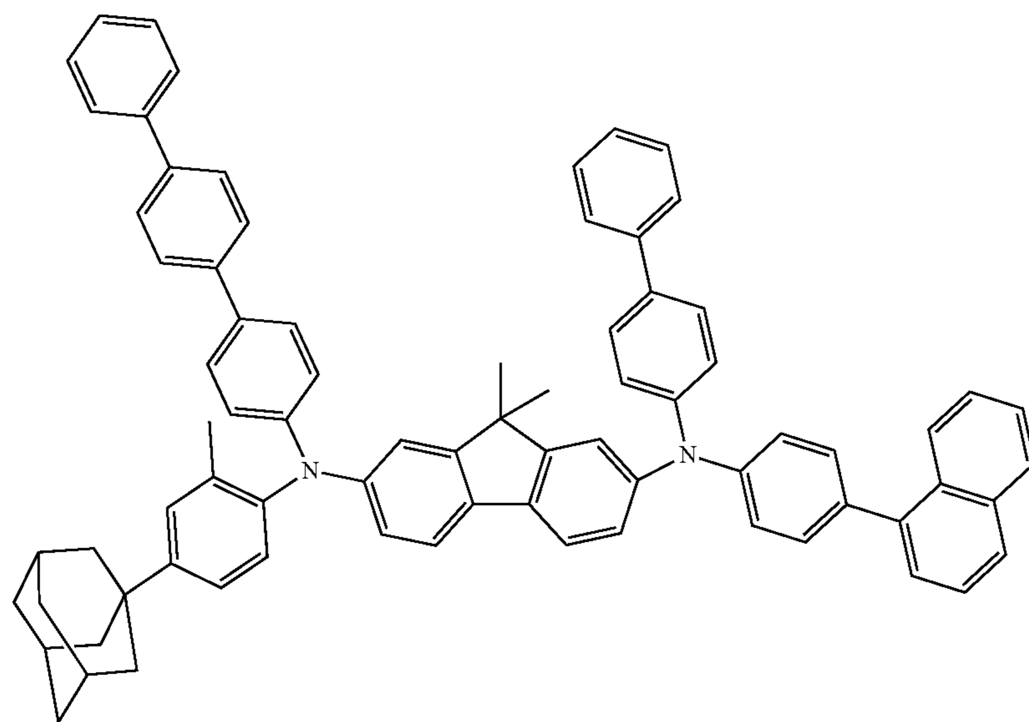
Compound 8
