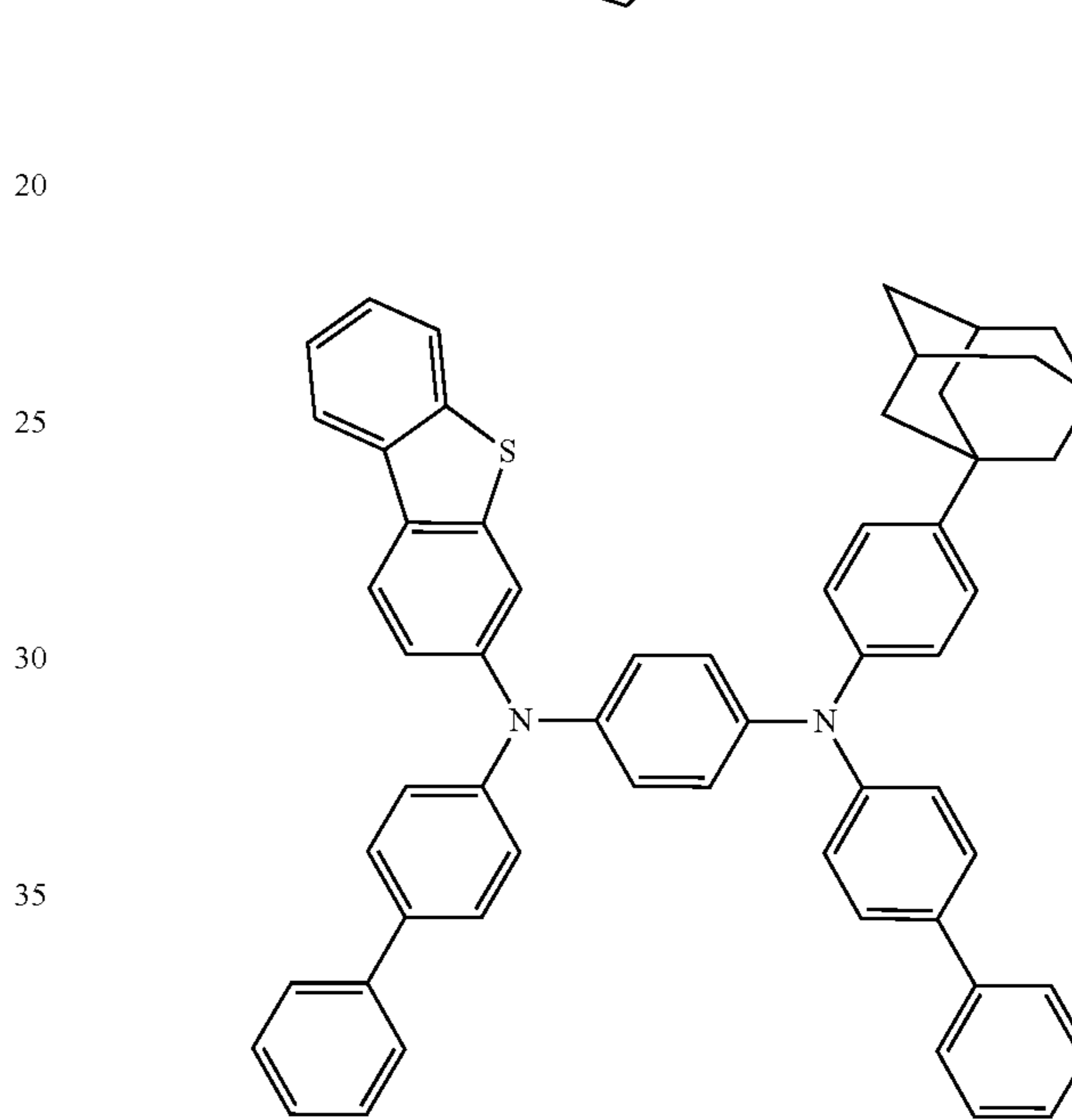
Compound31
