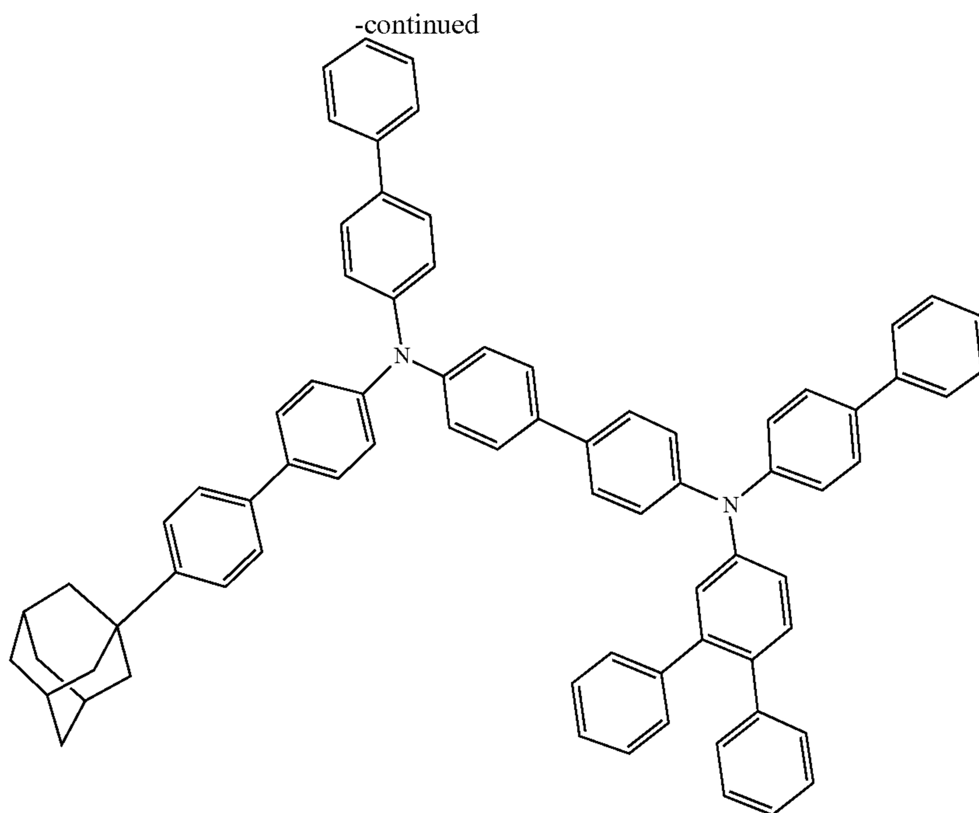
Compound 5
