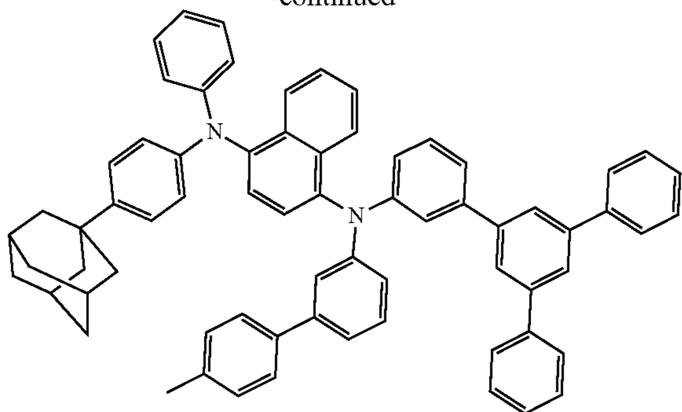
Compound 9
