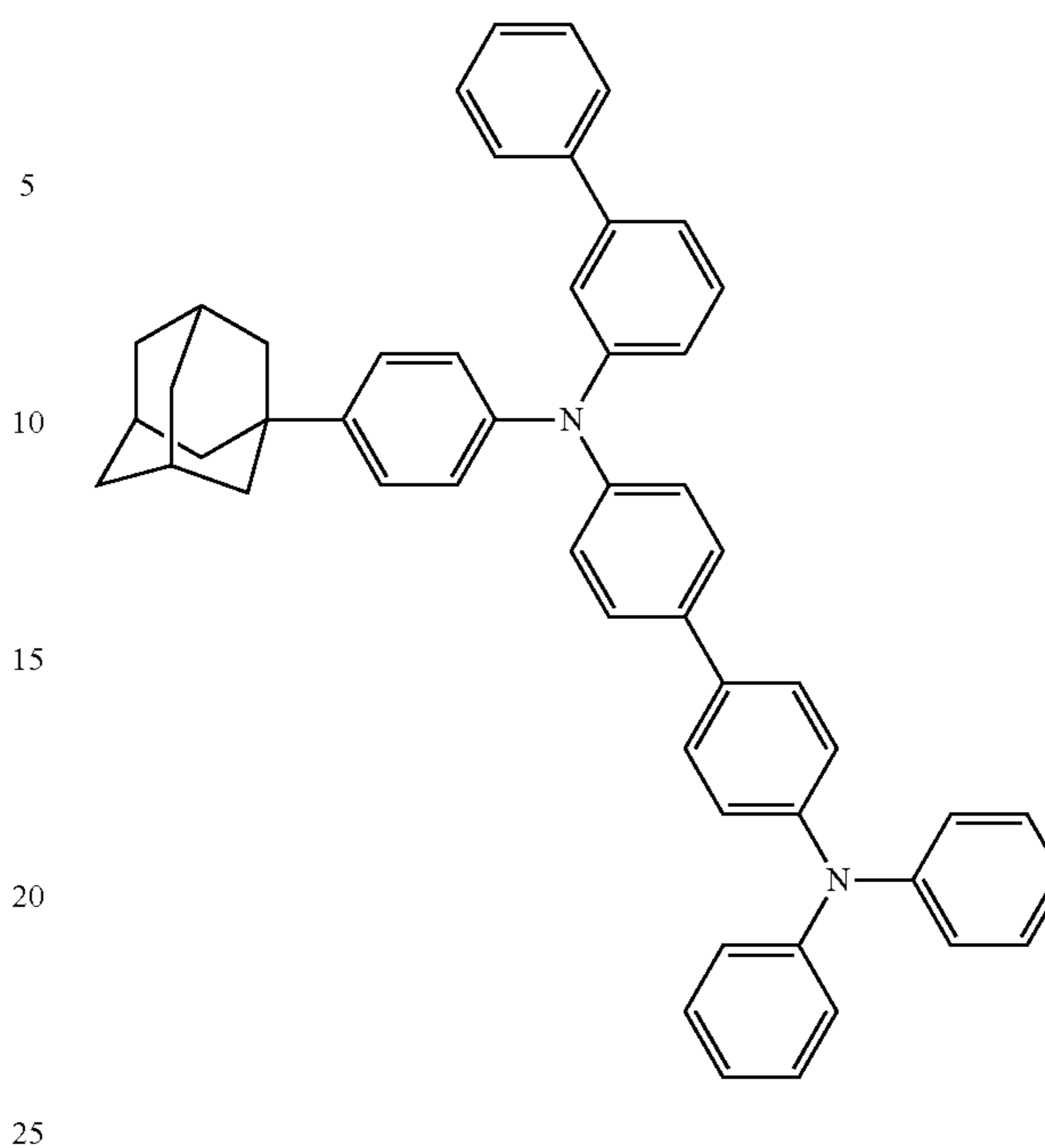
Synthesis Example 16
