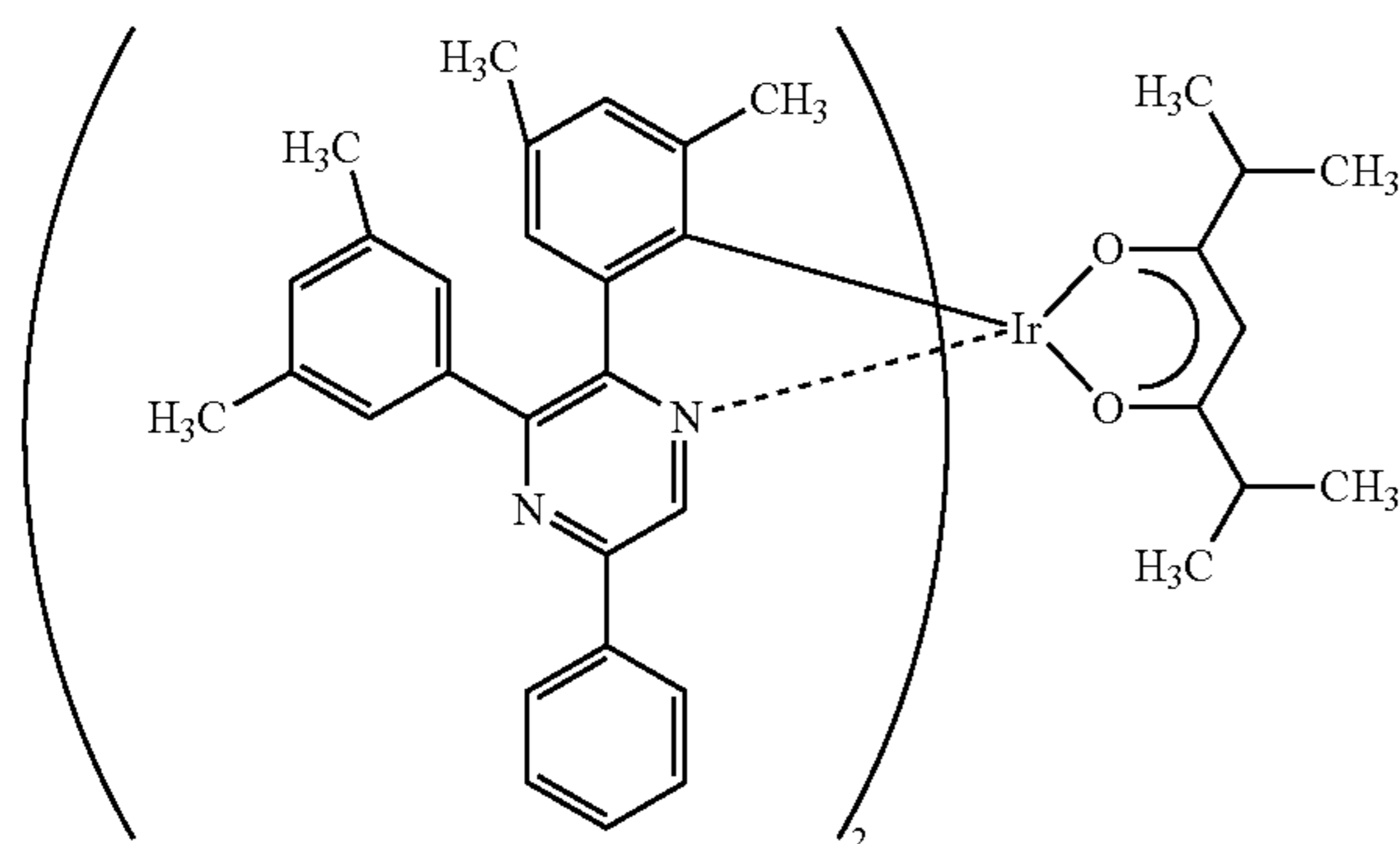
Ir(dmppr-P) 2 (dibm)
