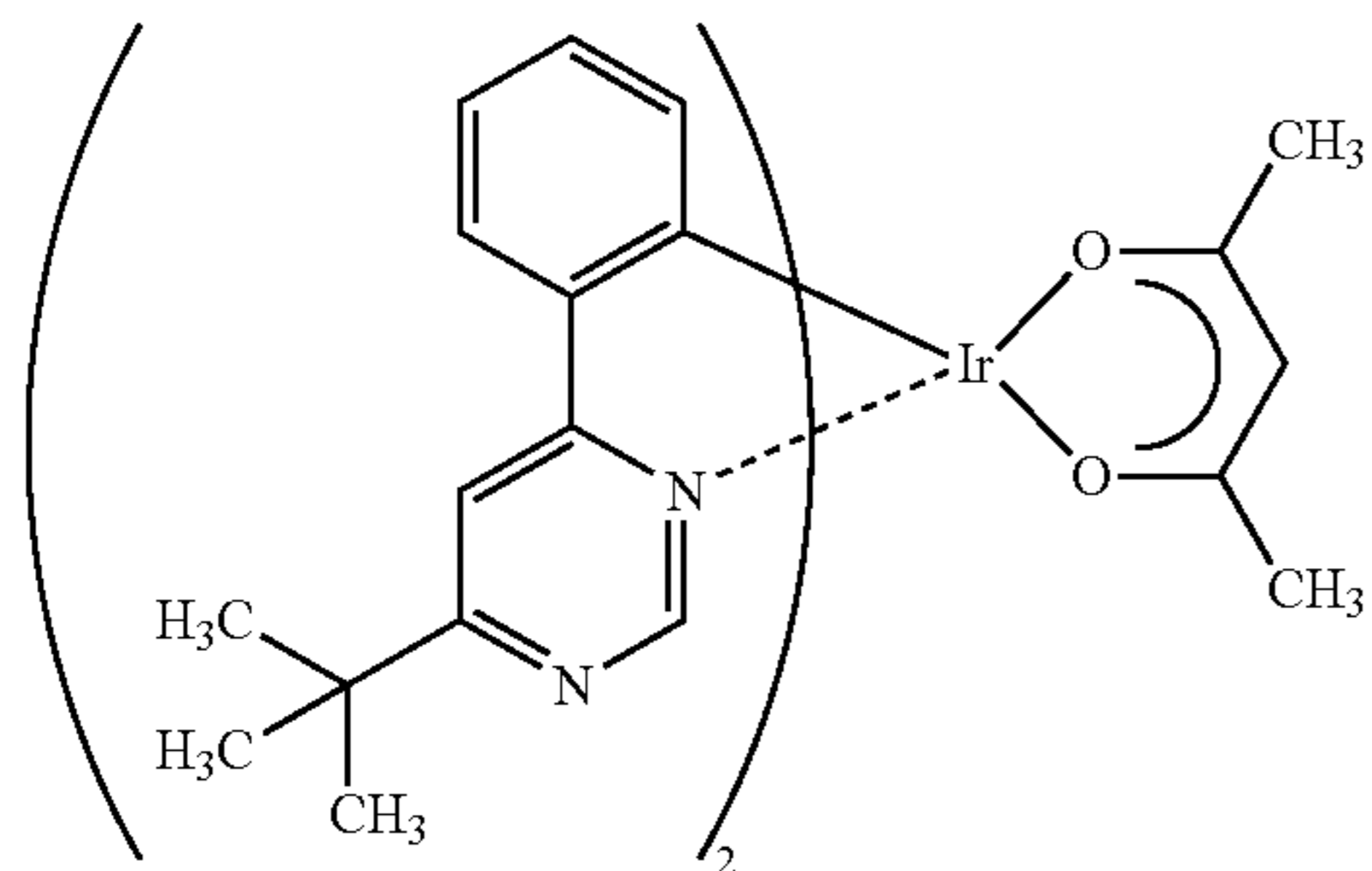
Ir(tBuppm) 2 (acac)
