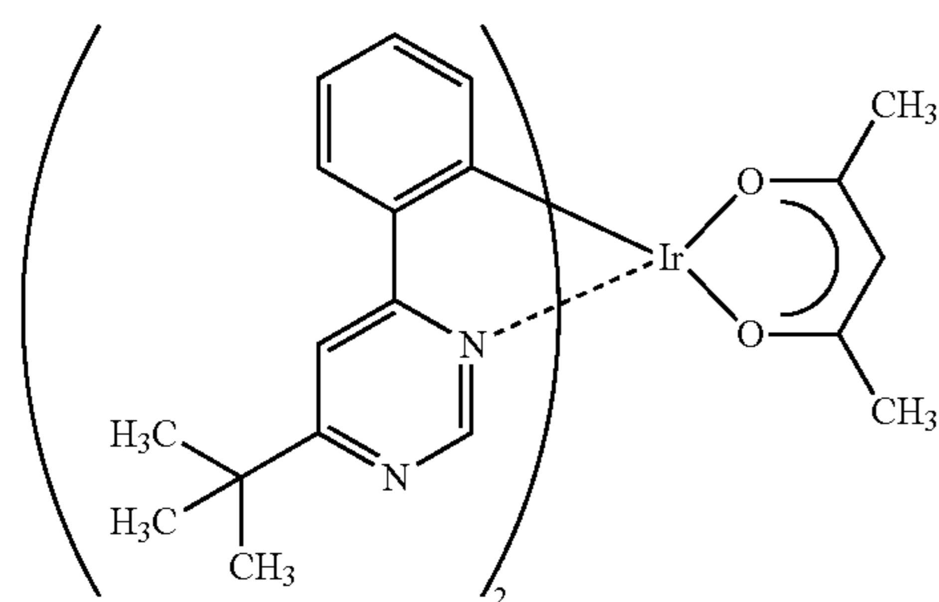
Ir(tBuppm) 2 (acac)
