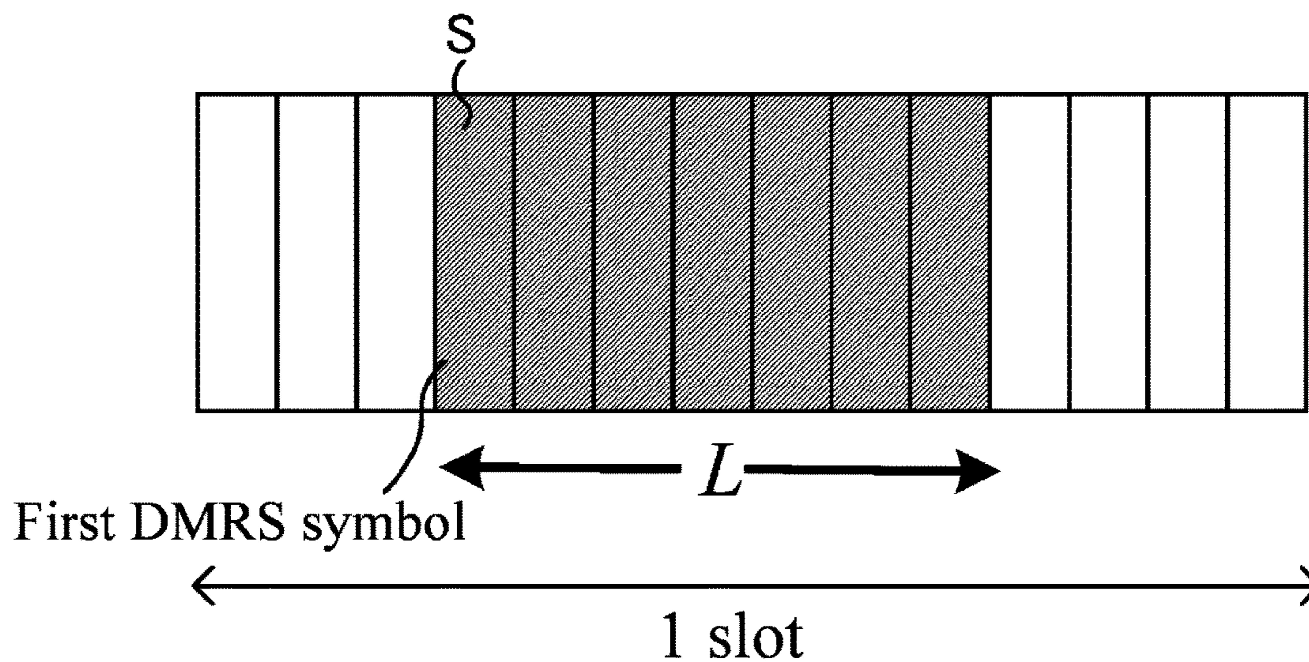
(A) PDSCH mapping type A
