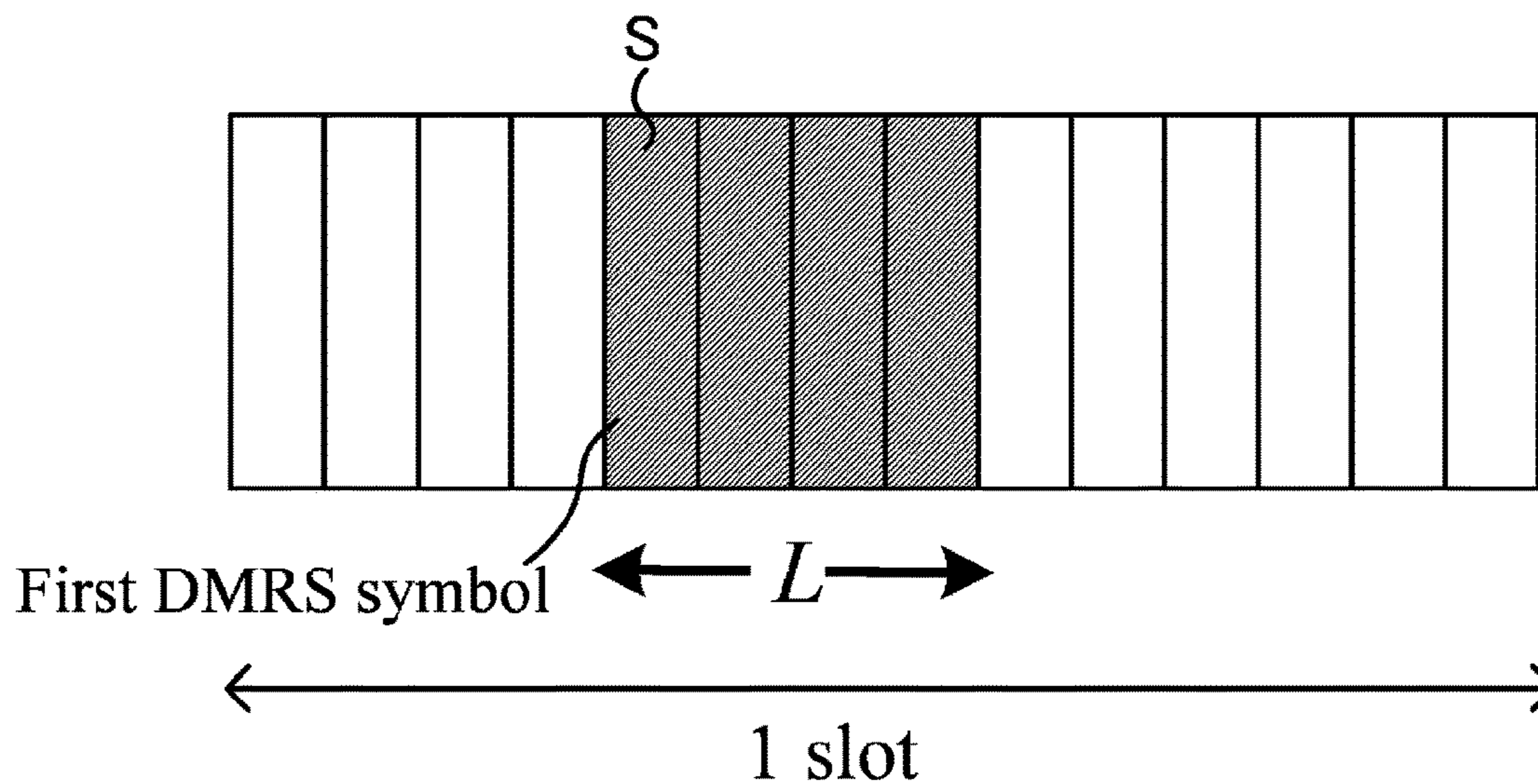
(B) PDSCH mapping type B
