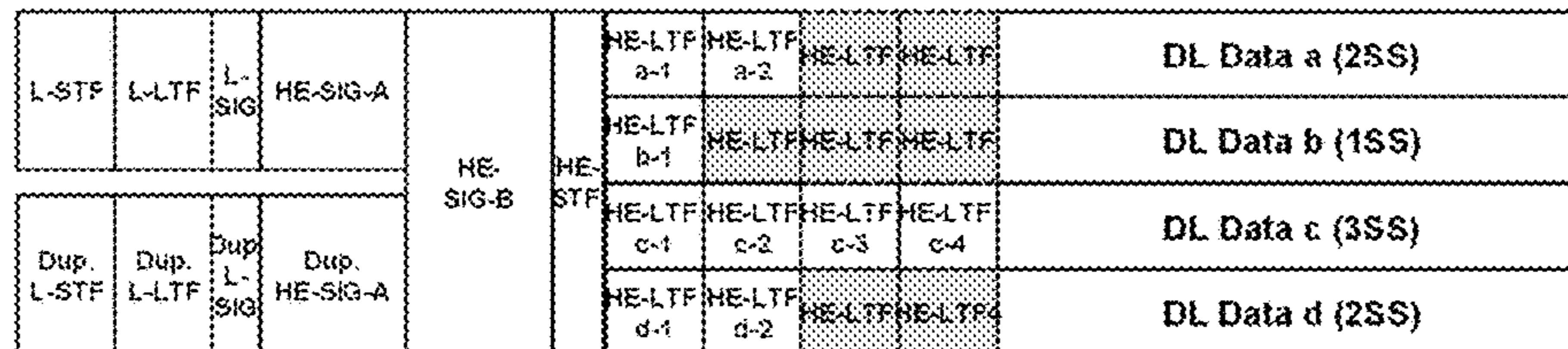
(a) [Type E] DL OFDMA (SU-MIMO)
