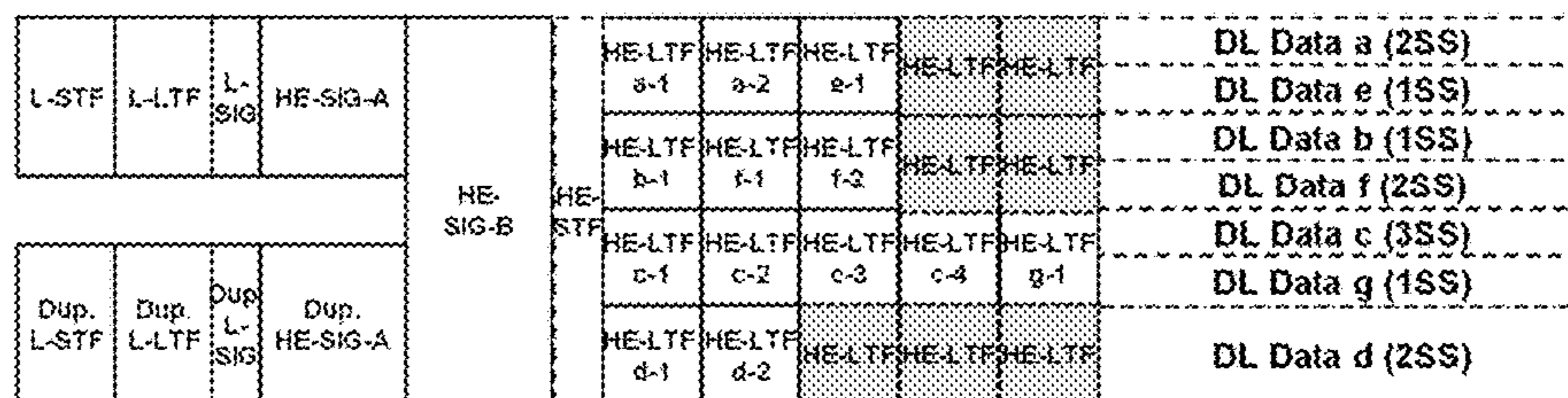
(b) [Type F] DL OFDMA (MU-MIMO)
