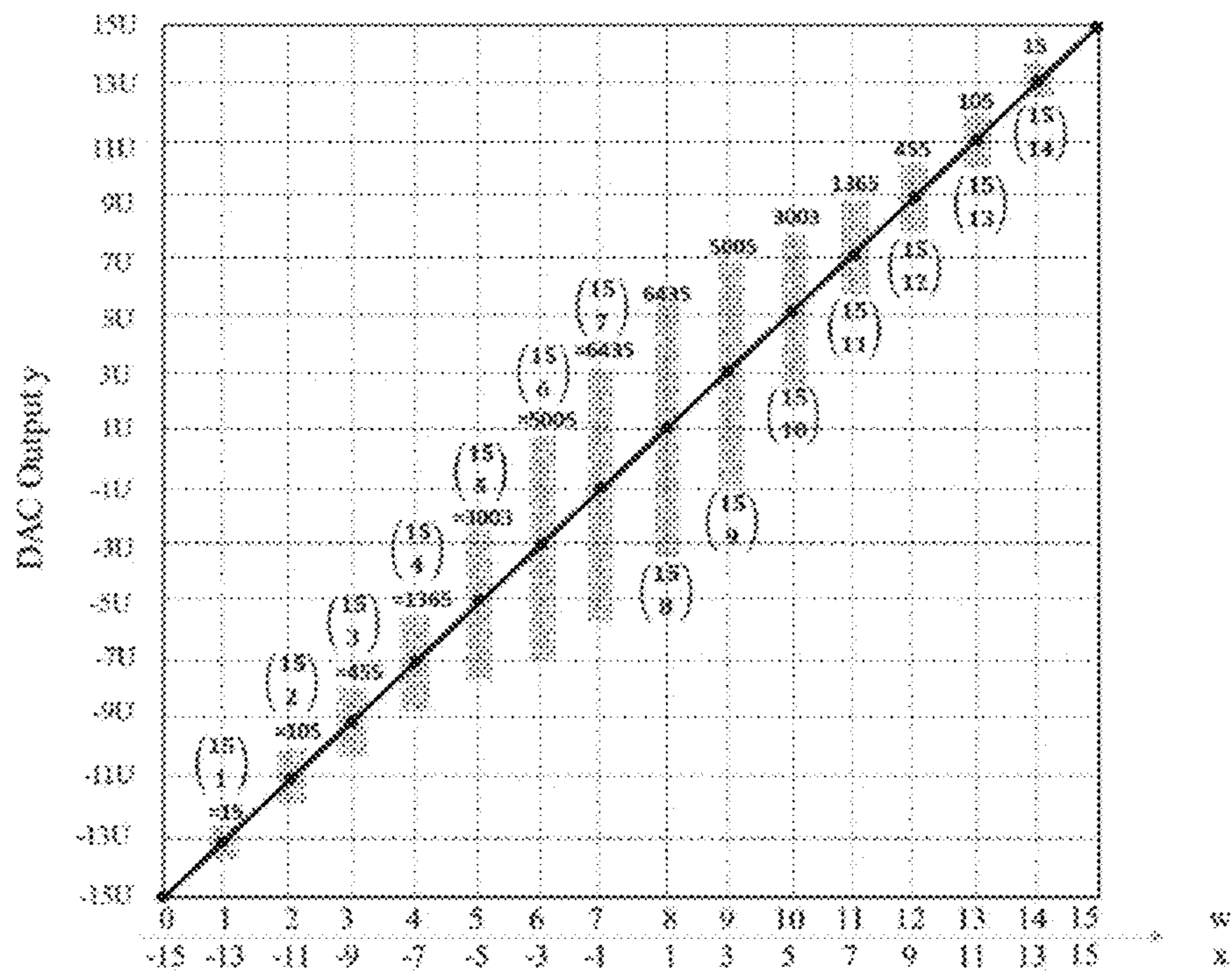
FIG. 9 (Prior art)
