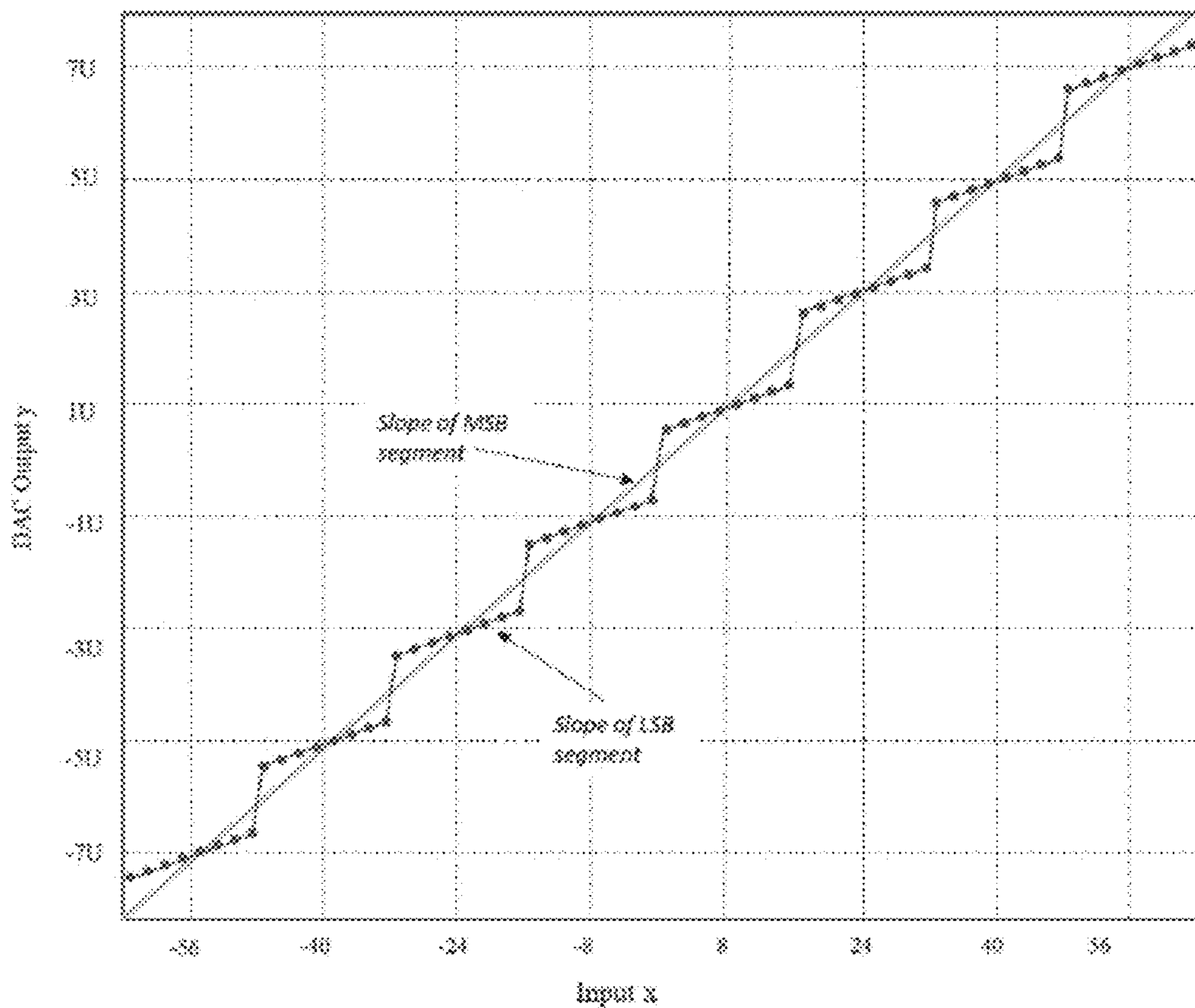
FIG. 12 (Prior art)
