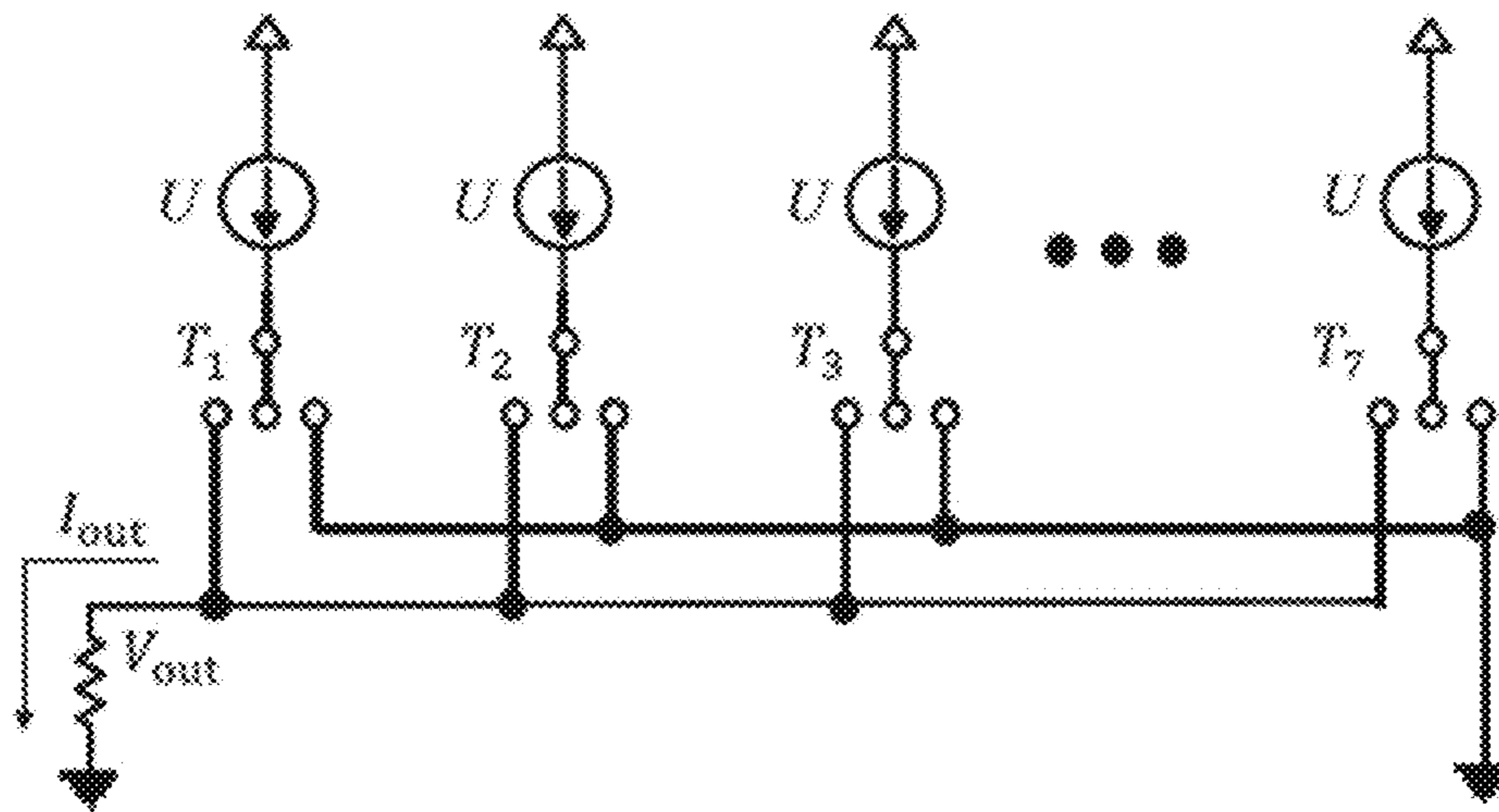
FIG. 4 (Prior art)
