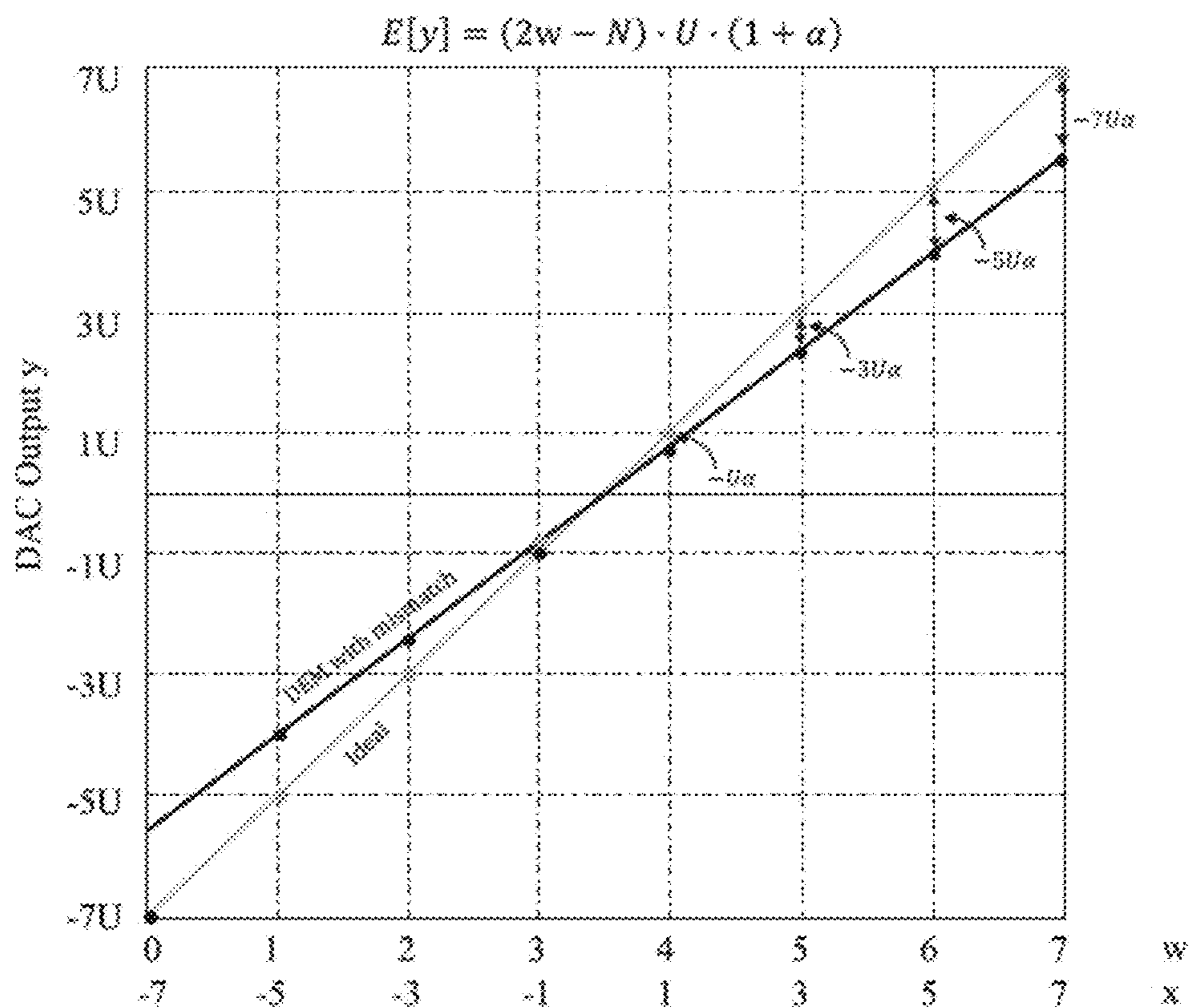
FIG. 11 (Prior art)
