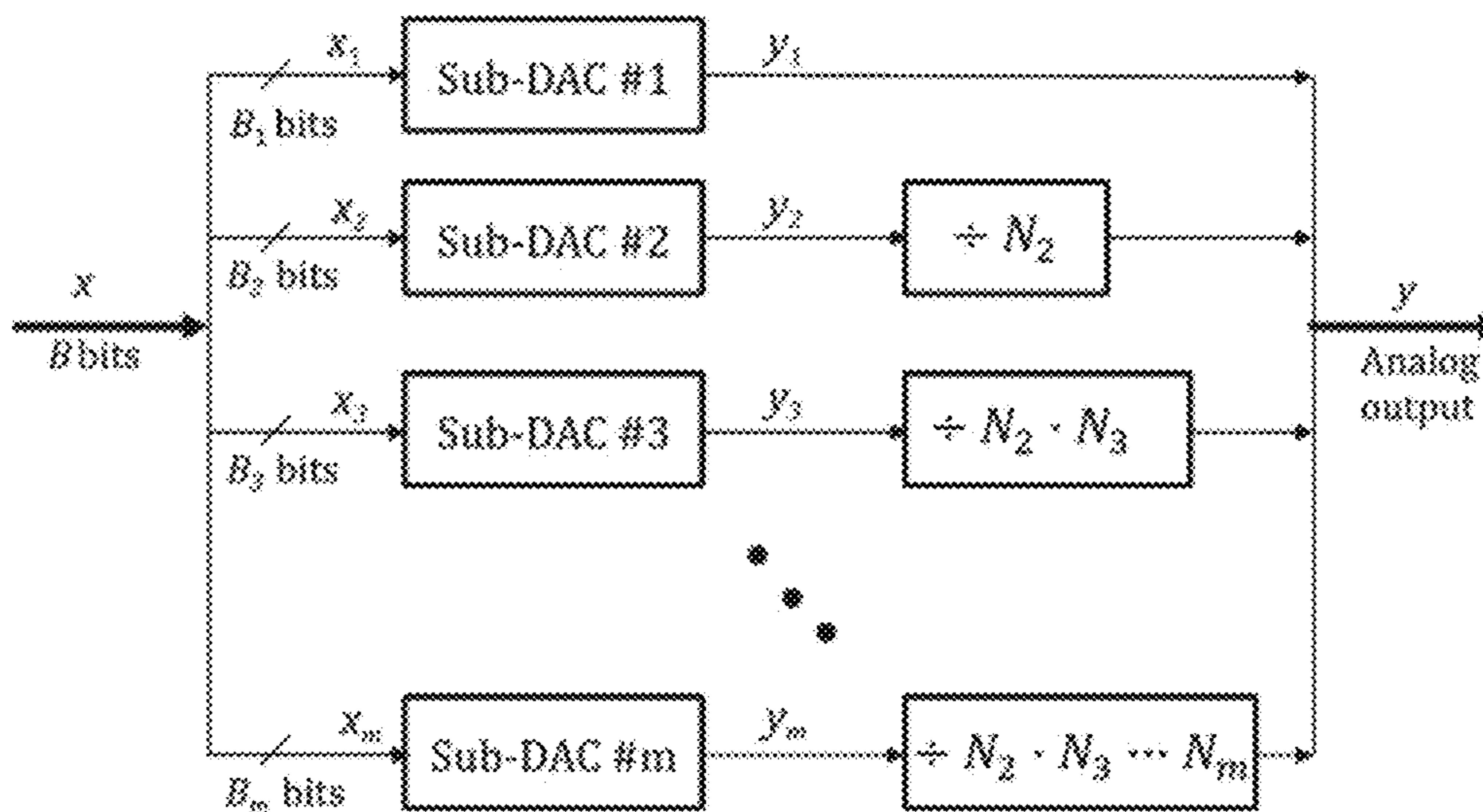
FIG. 13 (Prior art)
