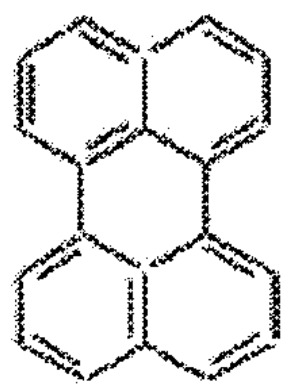
Perylene
