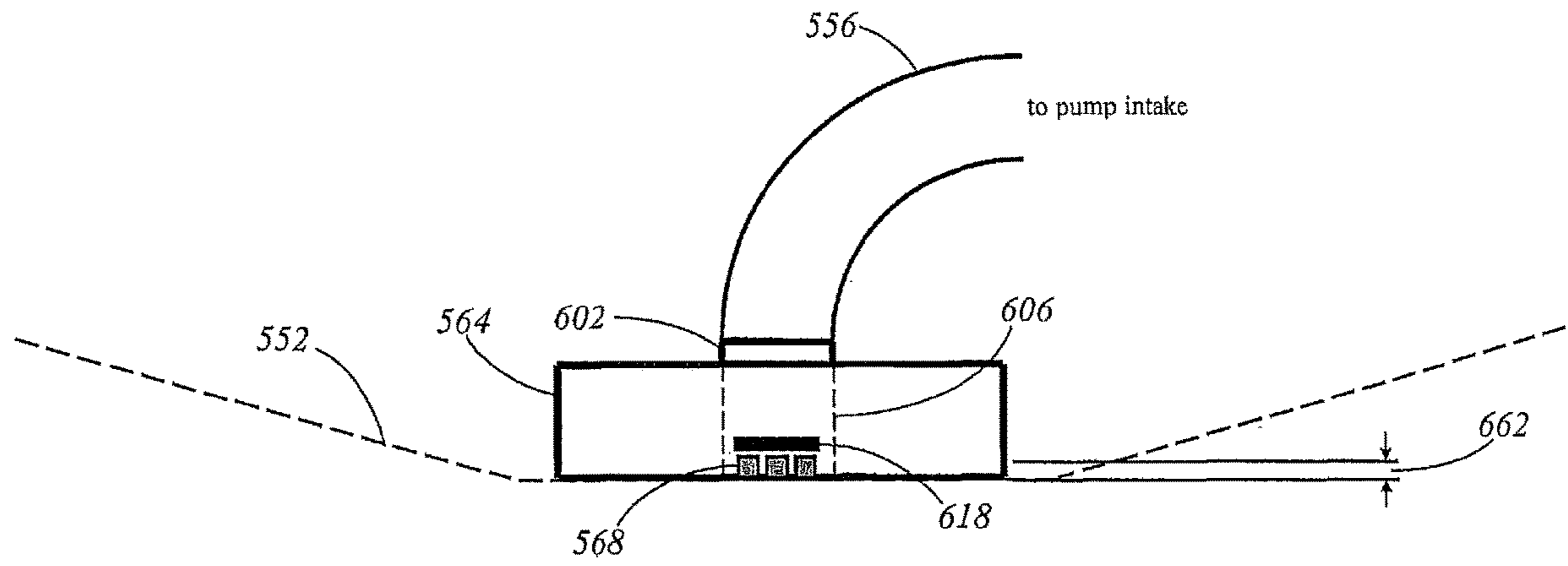
FIG. 17A side view
