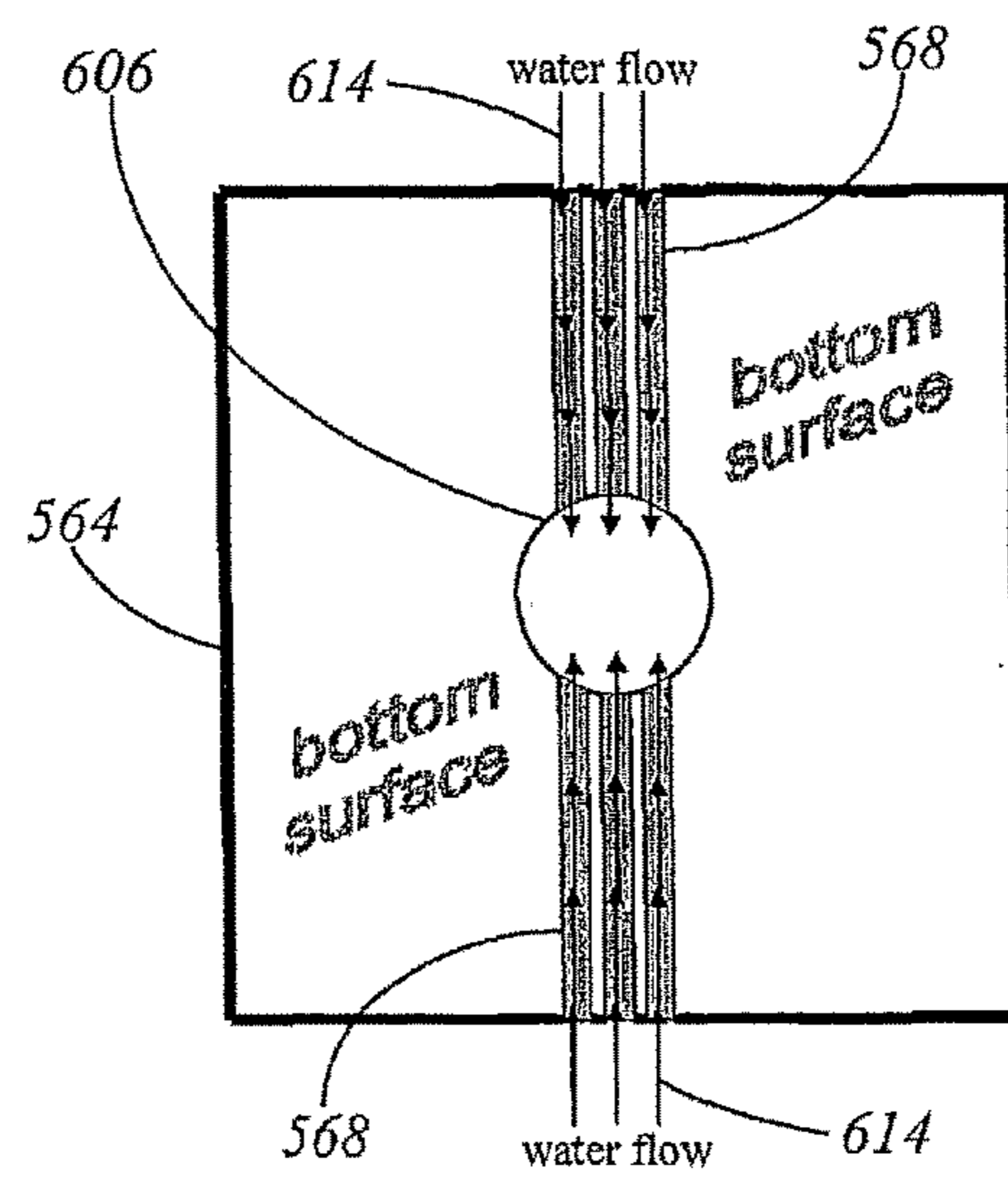
FIG. 17B bottom view
