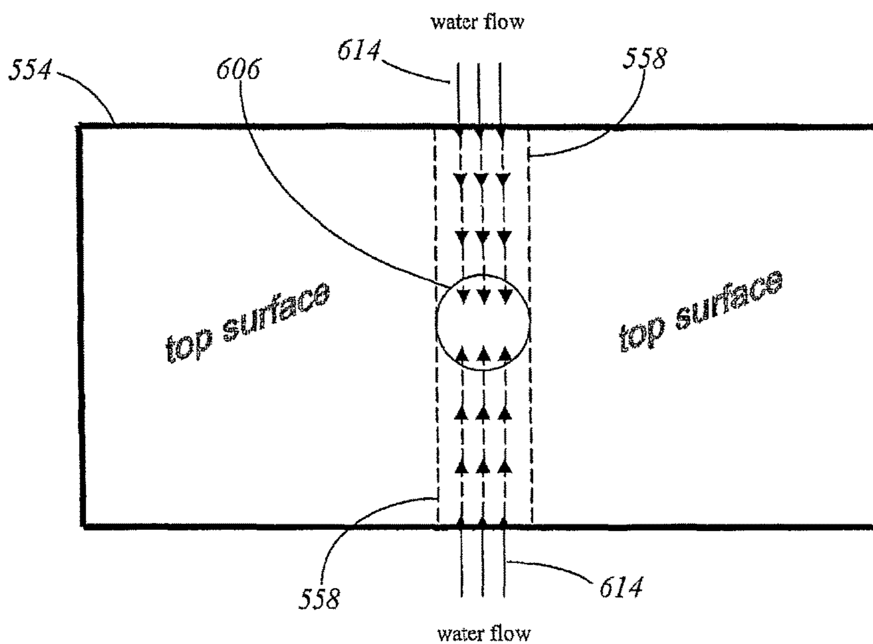
FIG. 16B top view
