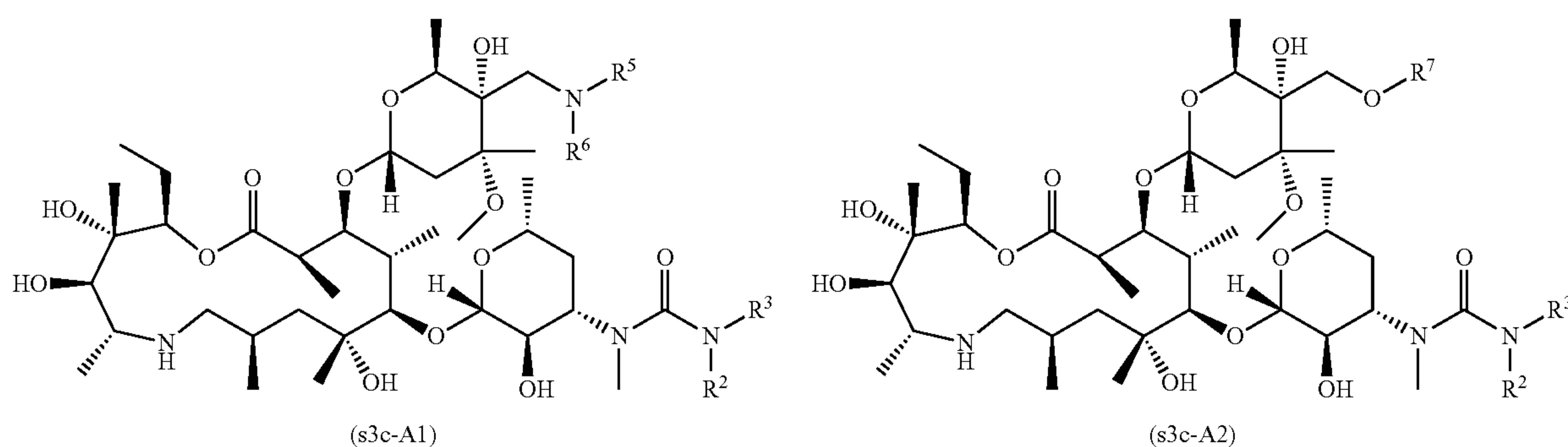
Scheme 3c: Details for Scheme 3a Step 3 (Urea formation)
