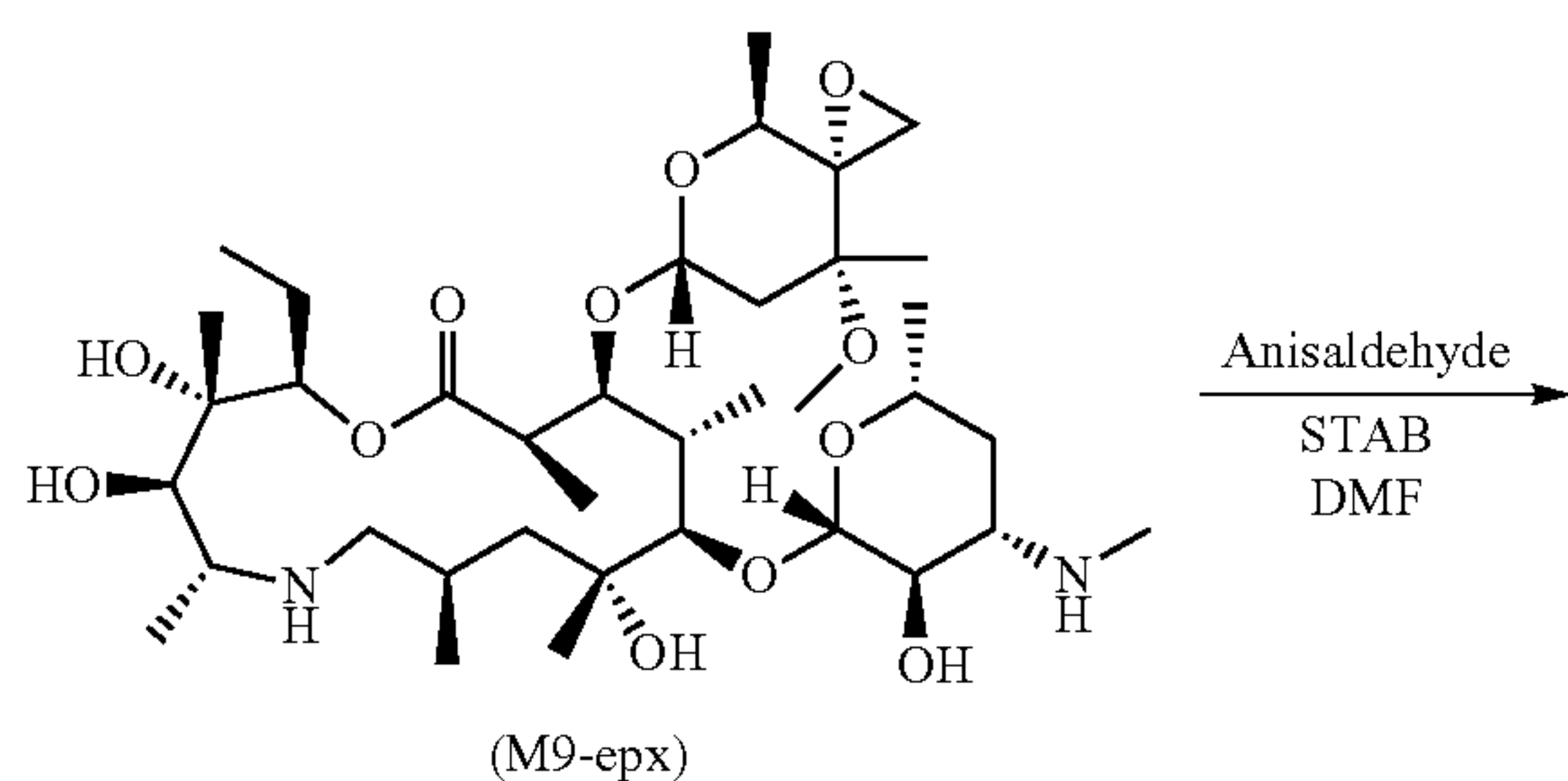
Scheme 6. Preparation of Formula (1) Compounds substituted with various \text{R}^1 and \text{R}^2 groups: Preparation of a common intermediate M8 epoxide (M8-epx)
