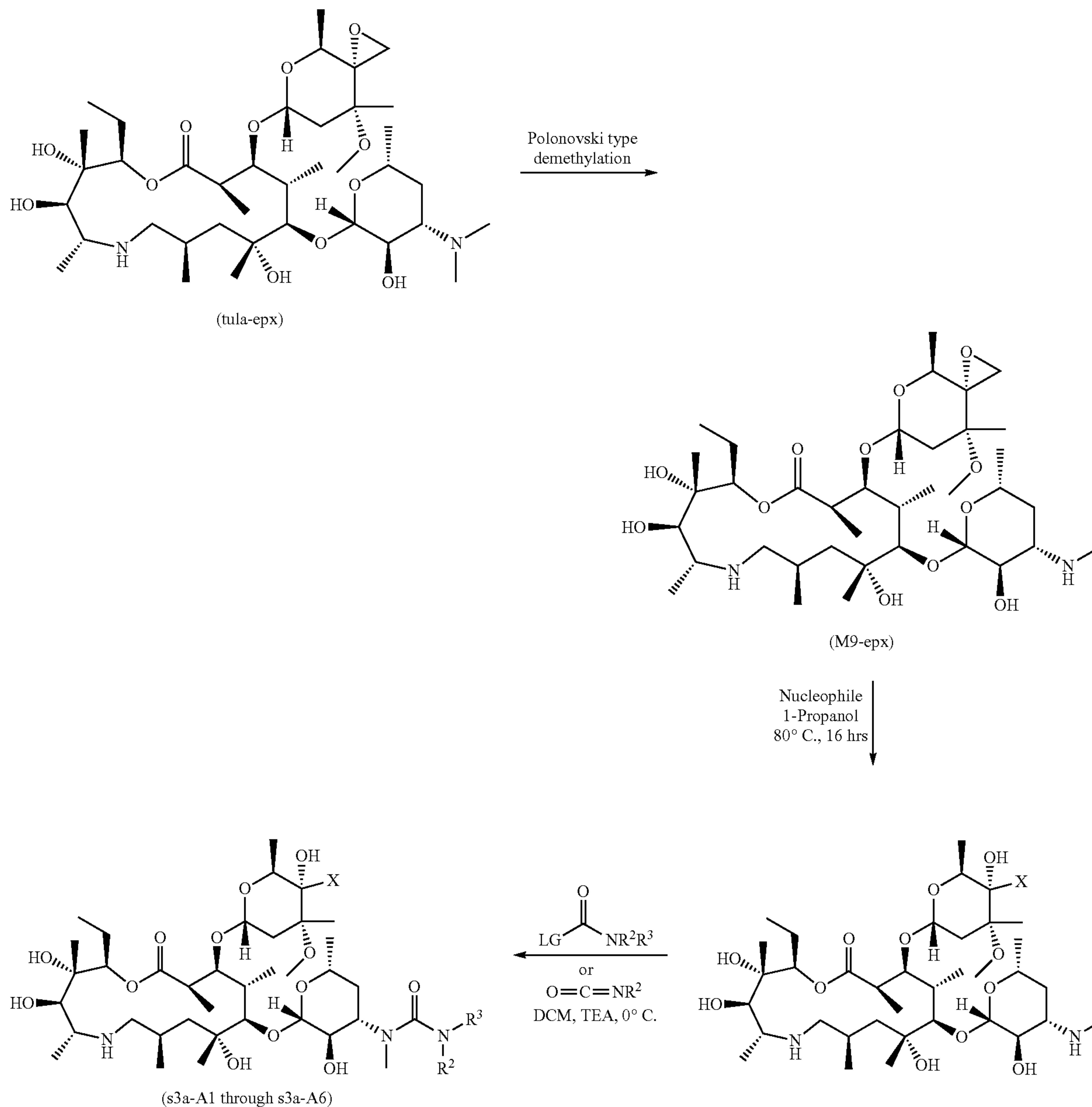
Scheme 3a. Preparation of Formula (1) Compounds (1-A1) through (1-A6)
