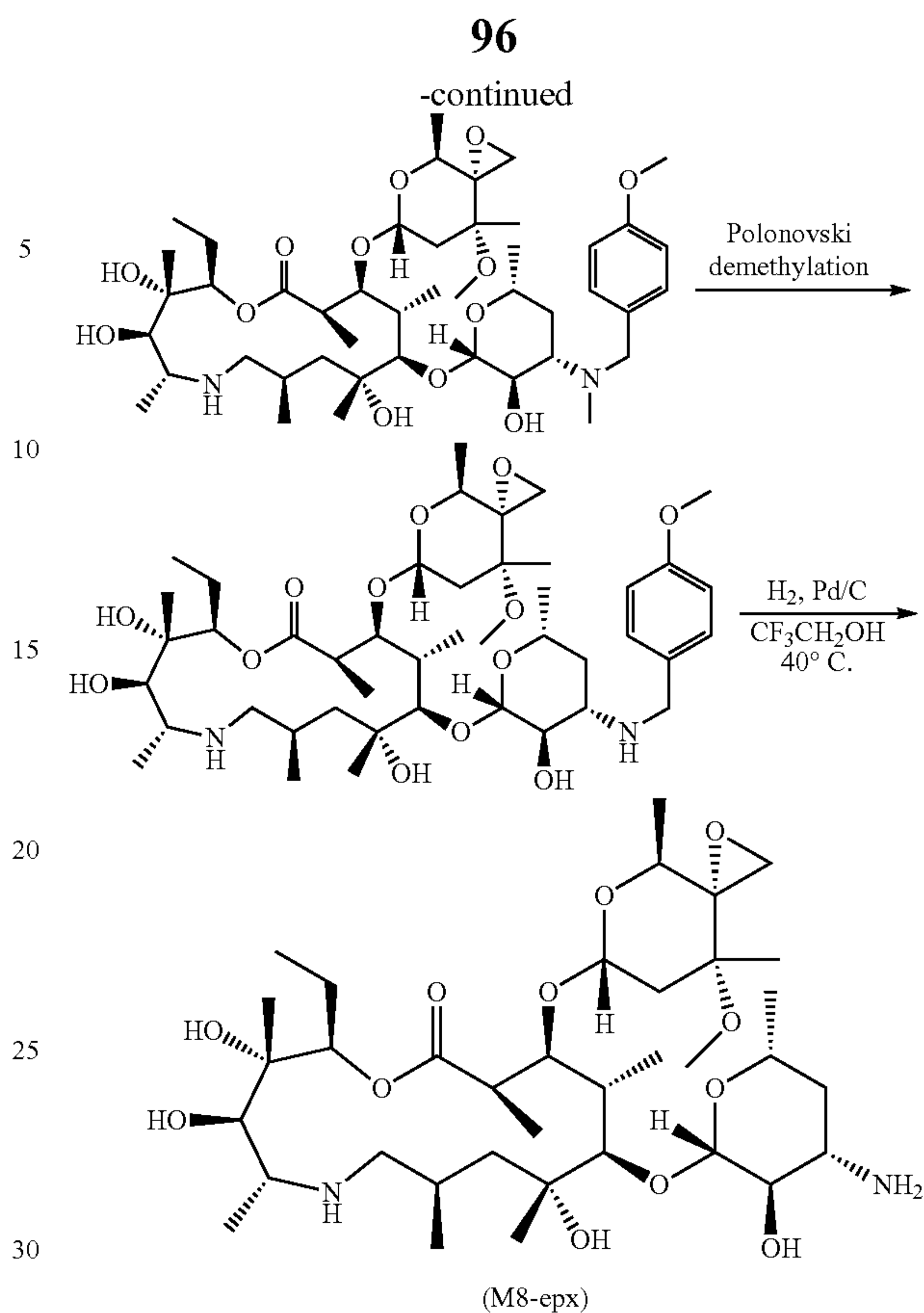
Scheme 6. Preparation of Formula (1) Compounds substituted with various \text{R}^1 and \text{R}^2 groups: Preparation of a common intermediate M8 epoxide (M8-epx)
