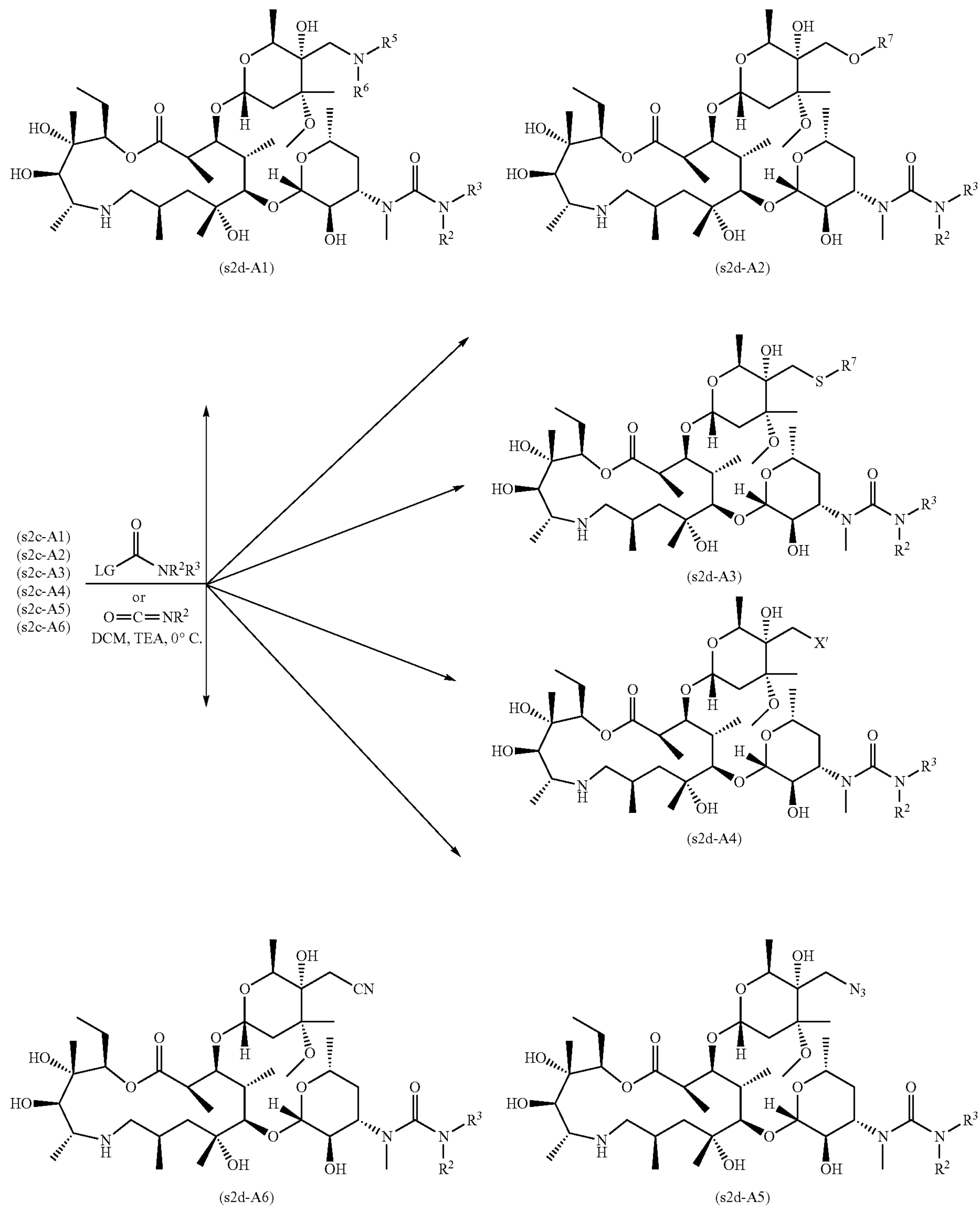
Scheme 2d: Details for Scheme 2a Step 3 (Urea formation)
