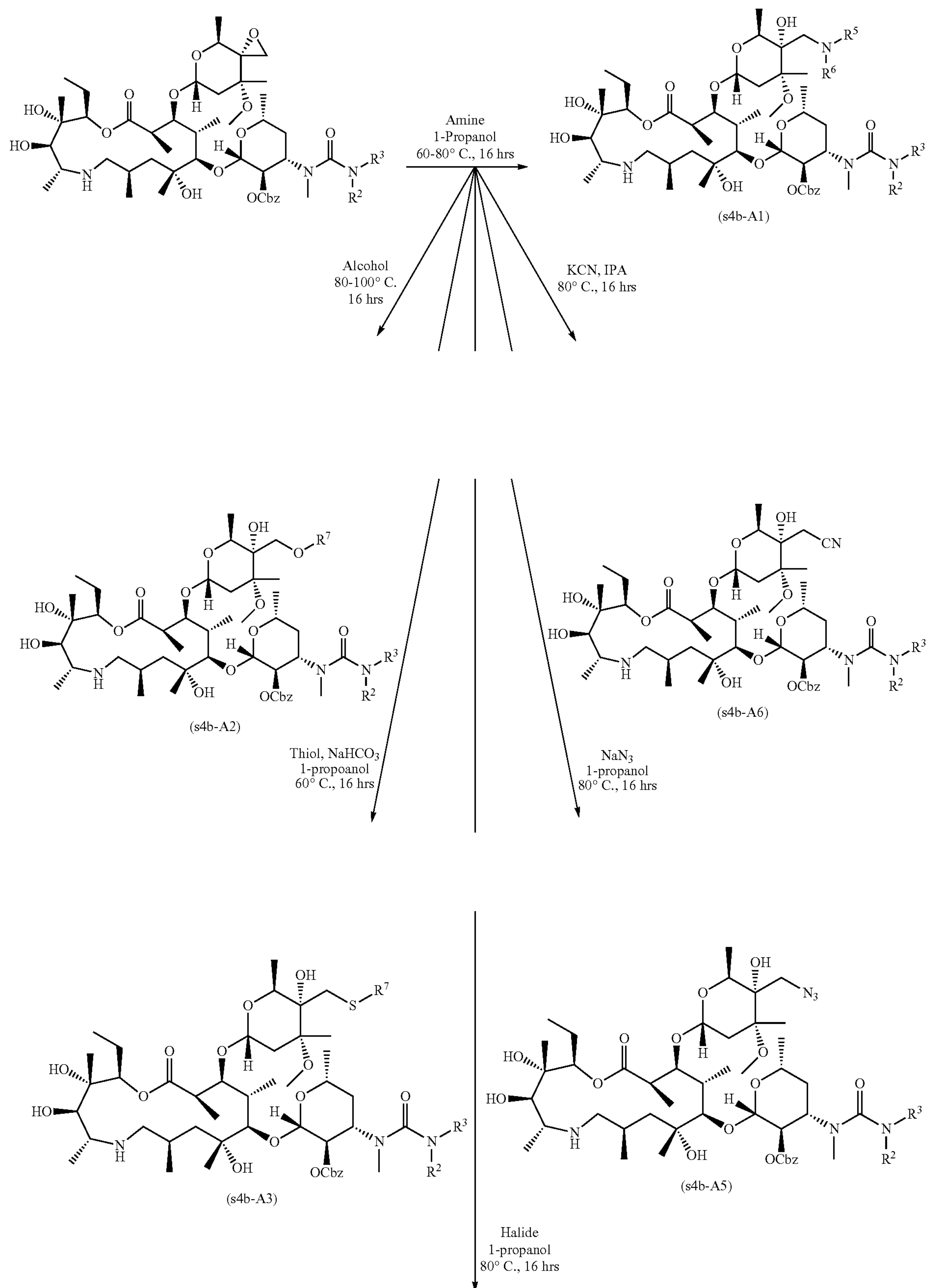
Scheme 4b: Details for Scheme 4a Step 3 (Nucleophilic Epoxide Opening)
