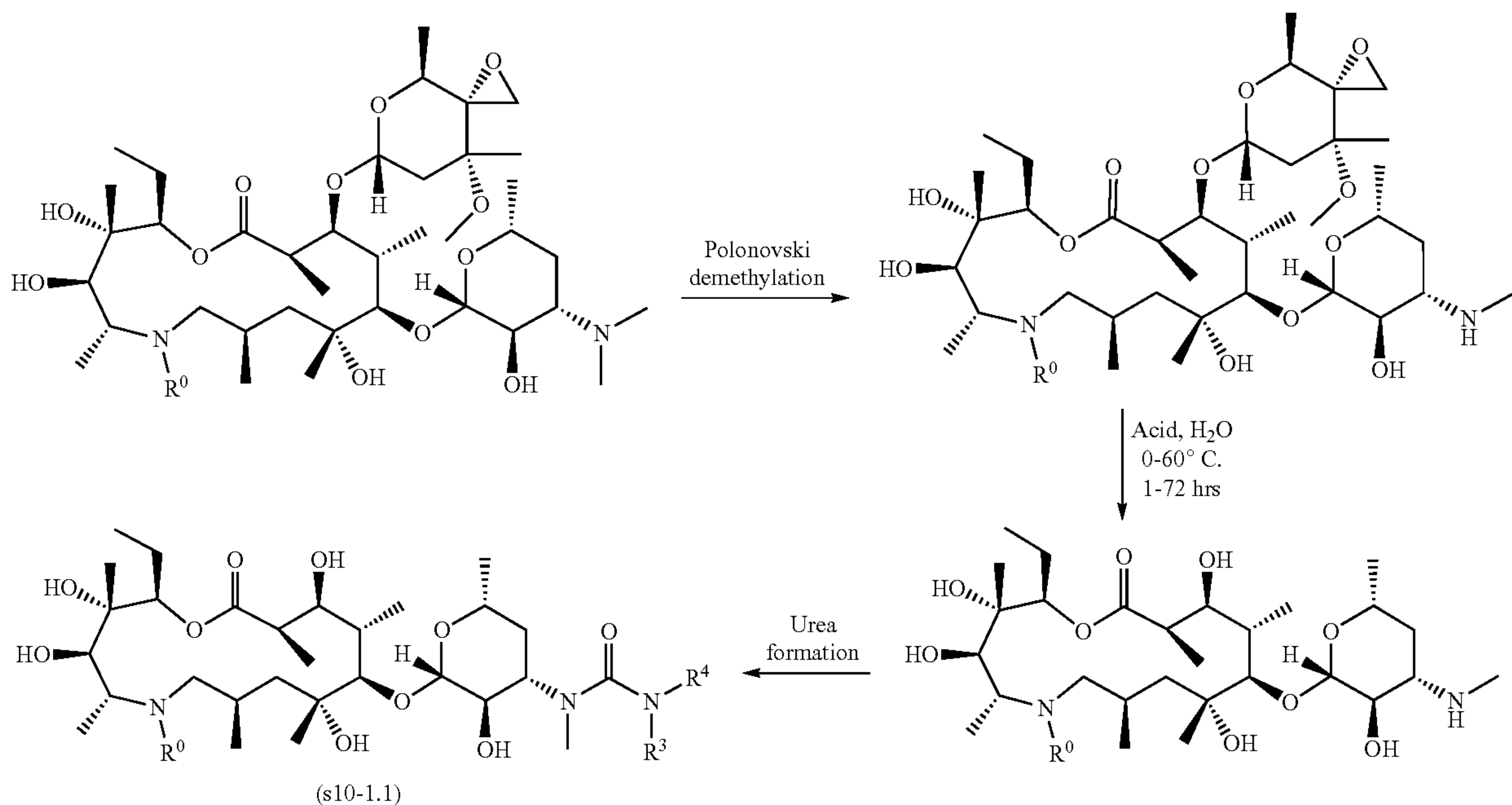
Scheme 10. Preparation of Formula (1.1) Des-cladinose Compounds
