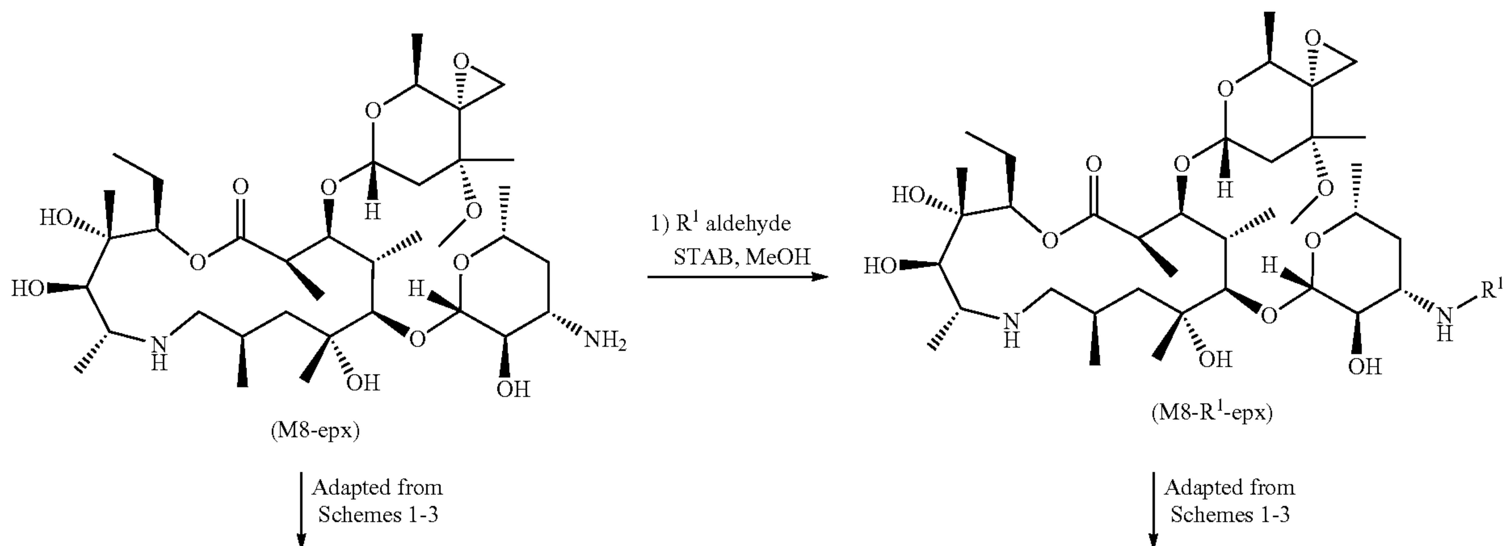
Scheme 7. Preparation of Formula (1) Compounds substituted with various \text{R}^1 groups from M8 epoxide (M8-epx)
