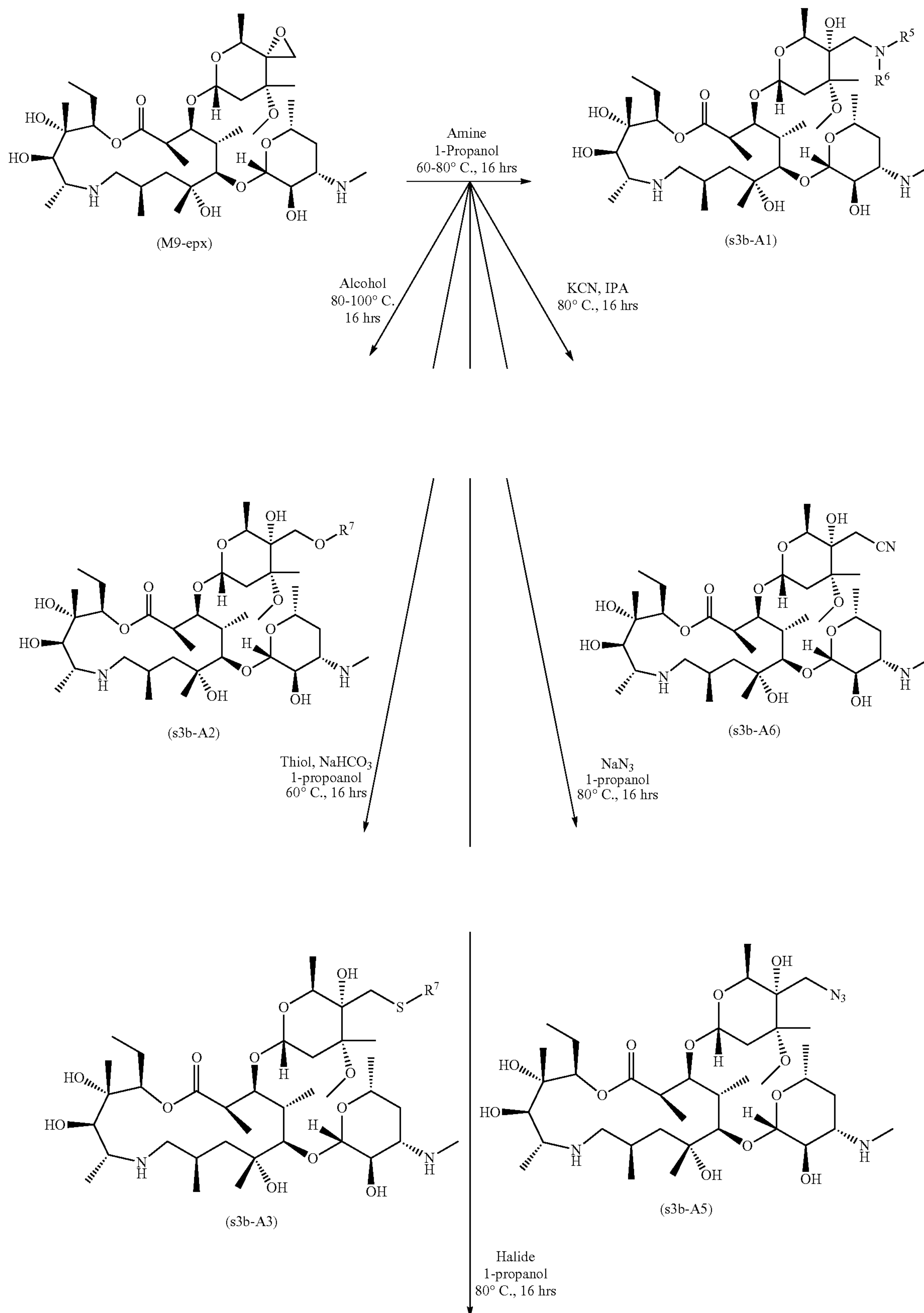
Scheme 3b: Details for Scheme 3a Step 2 (Nucleophilic Epoxide Opening)
