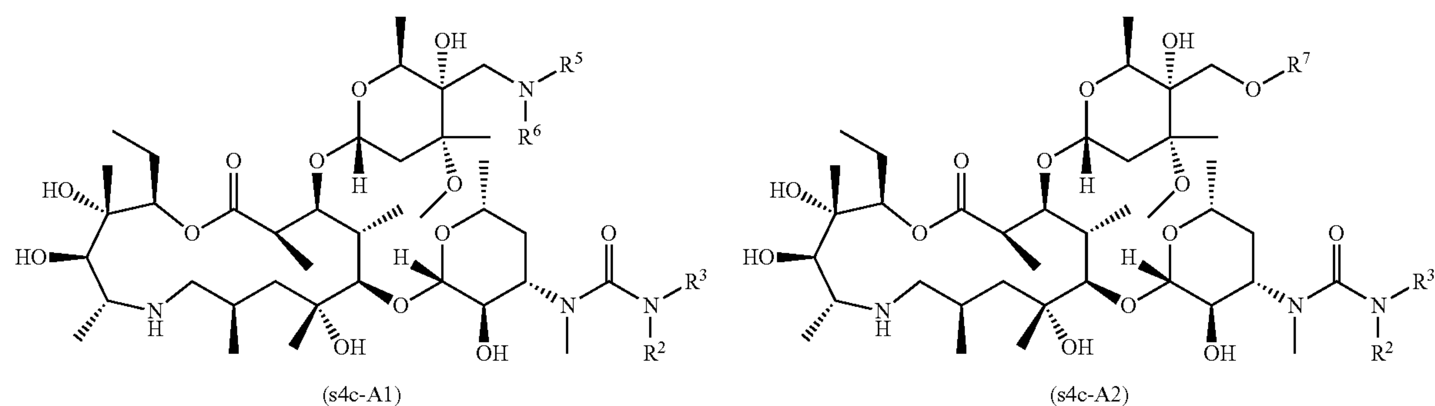
Scheme 4c: Details for Scheme 3a Step 4 (Deprotection)
