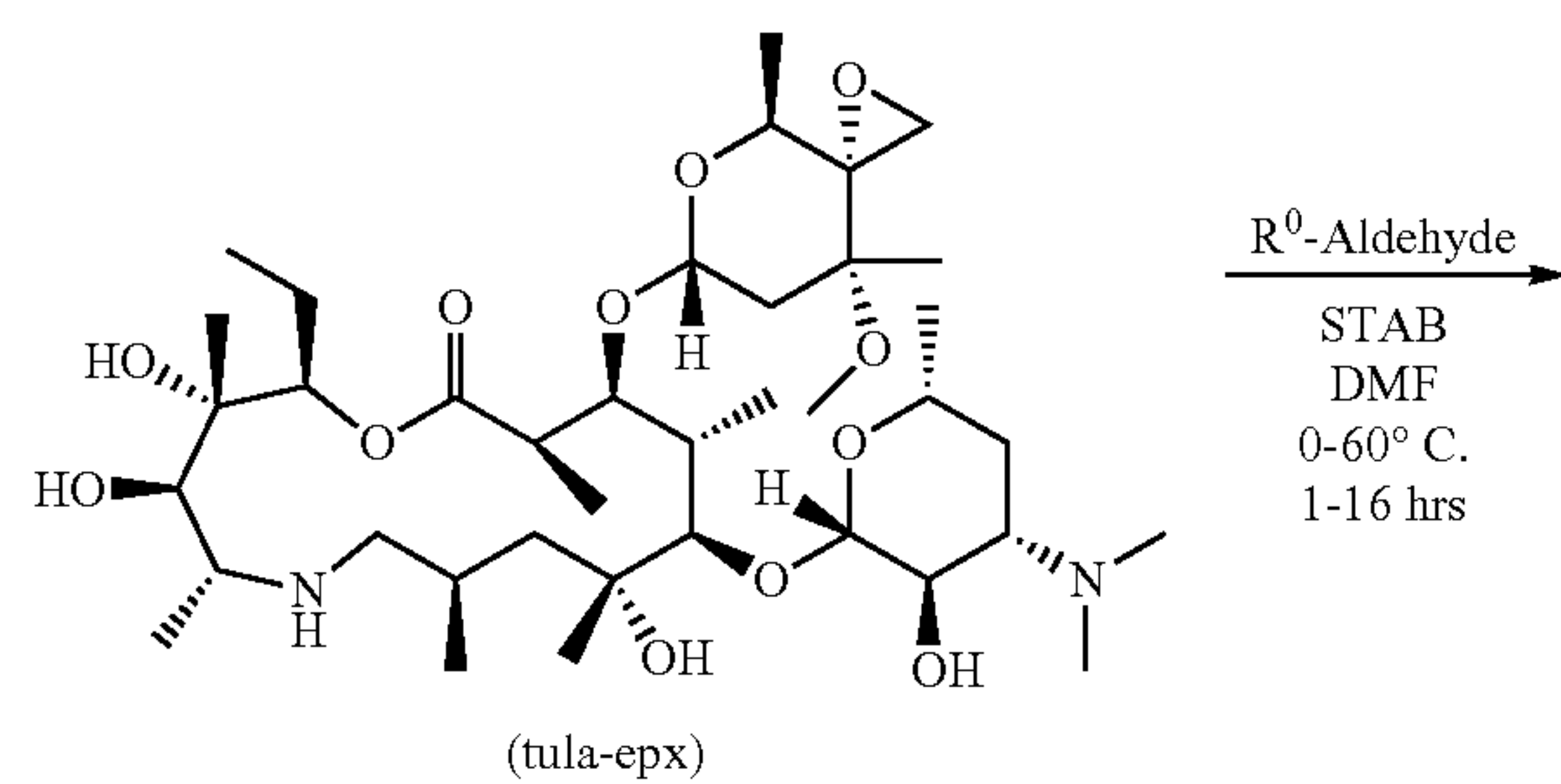
Scheme 5. Preparation of Alkylated Core Nitrogen Formula (1) Compounds by Reductive Amination
