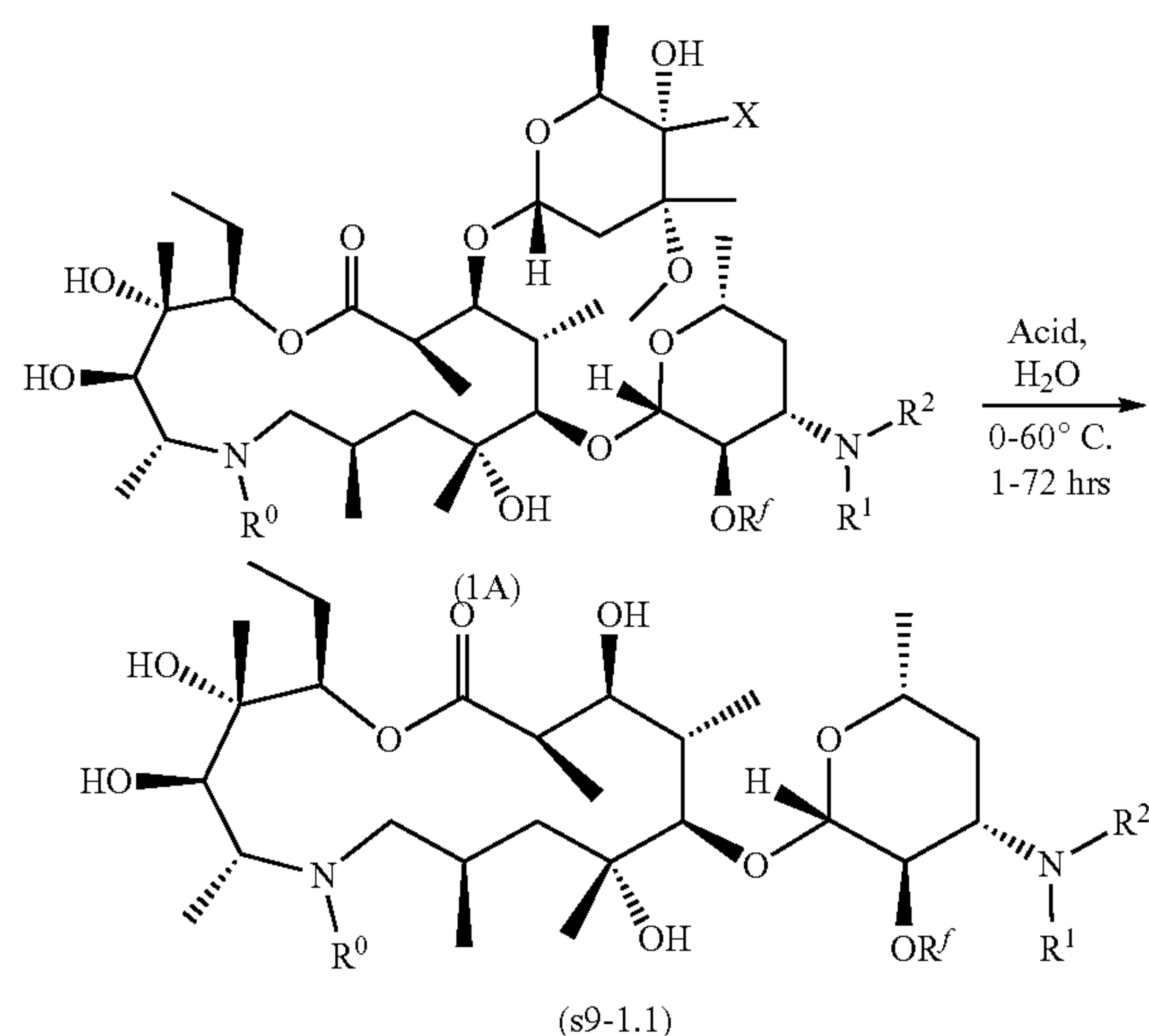
Scheme 9. Preparation of Formula (1.1) Des-cladinose Compounds
