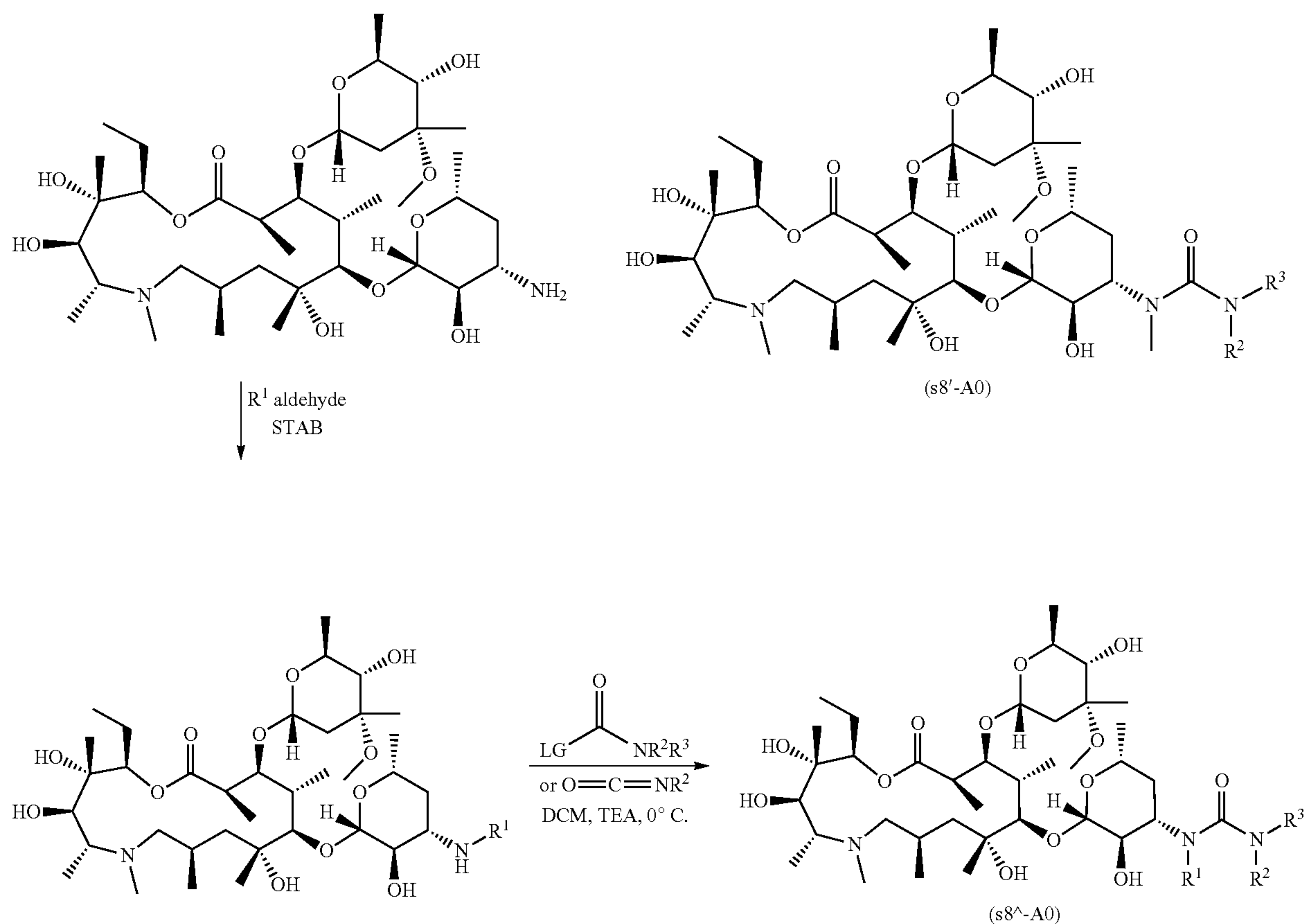
Scheme 9. Preparation of Formula (1.1) Des-cladinose Compounds
