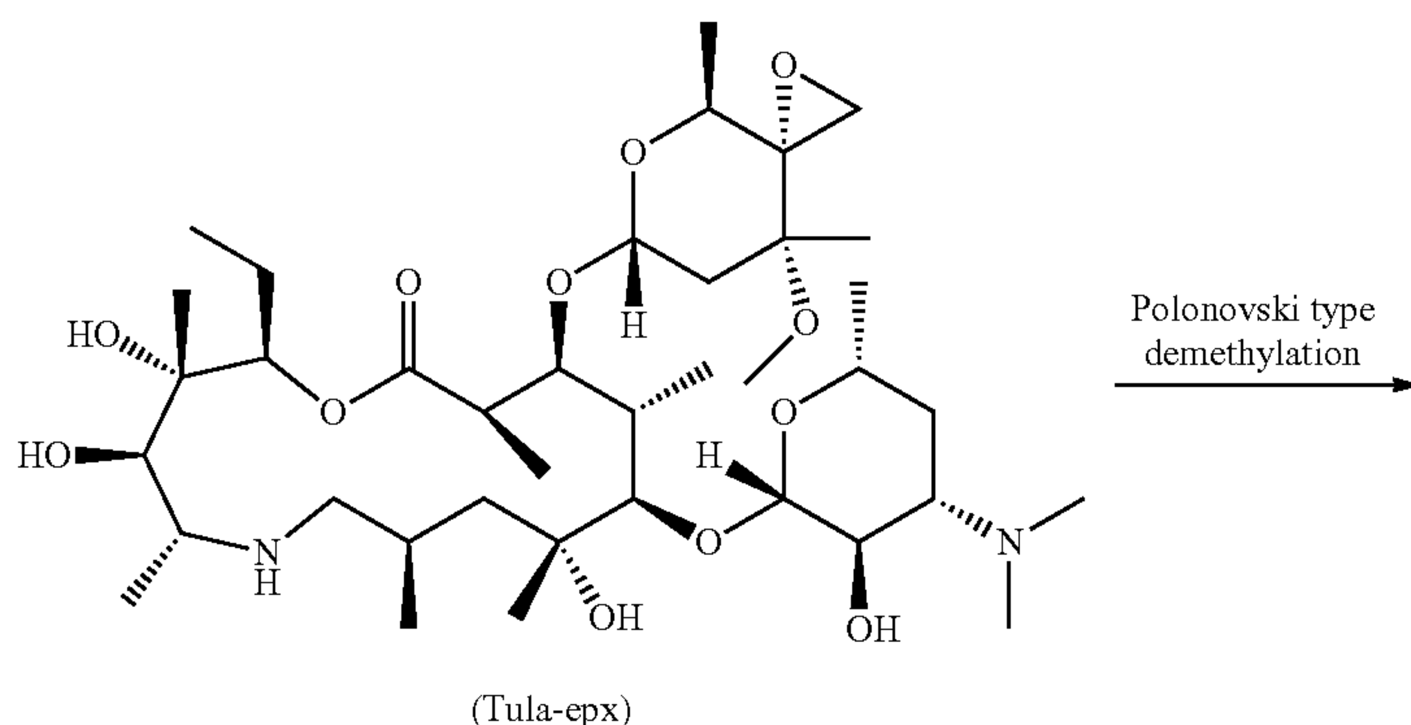
Scheme 1a. Preparation of Formula (1) Urea Compounds (1-A1) through (1-A6)
