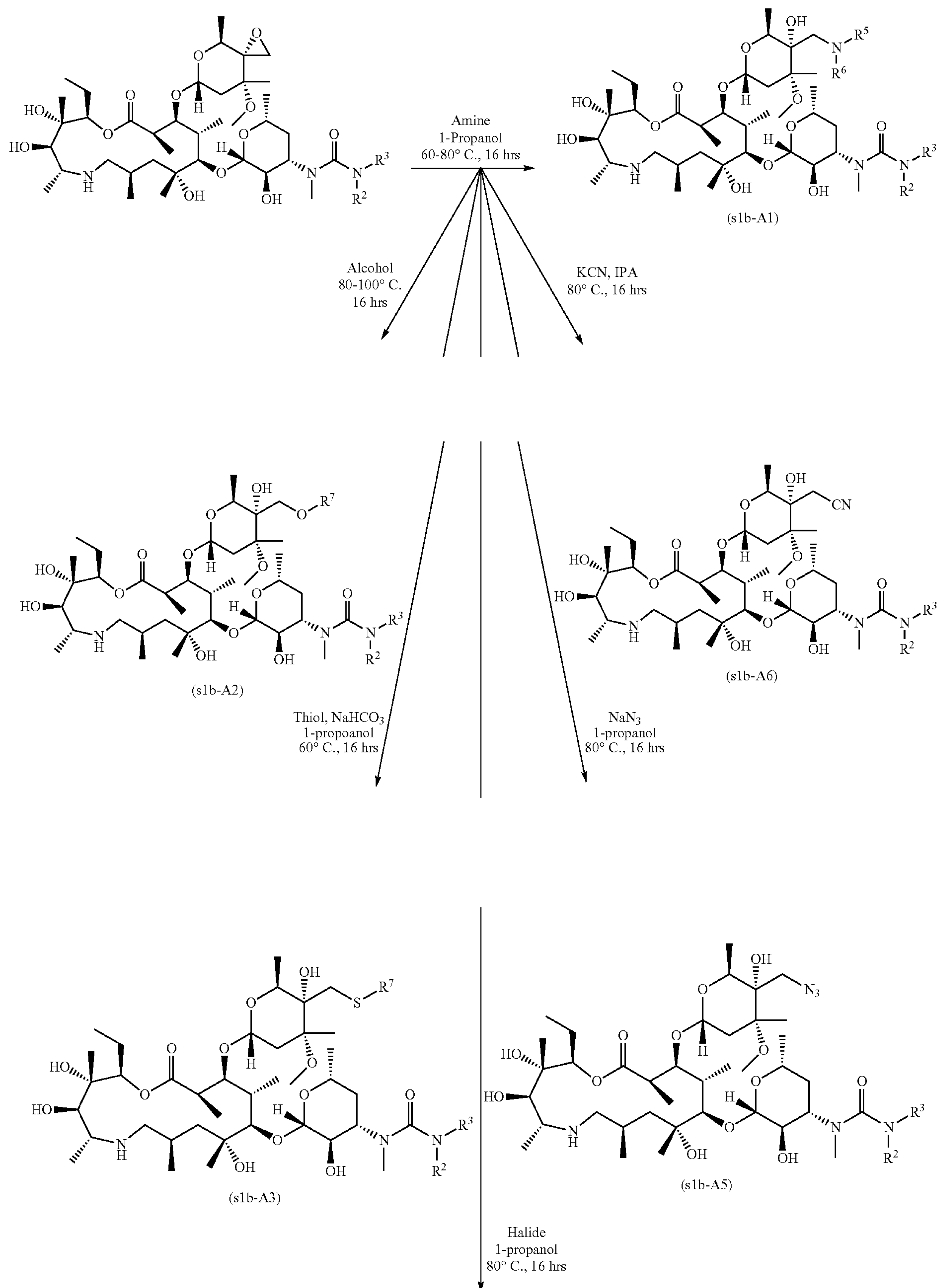
Scheme 1b: Details for Scheme 1a Step 3 (Nucleophilic Epoxide Opening)
