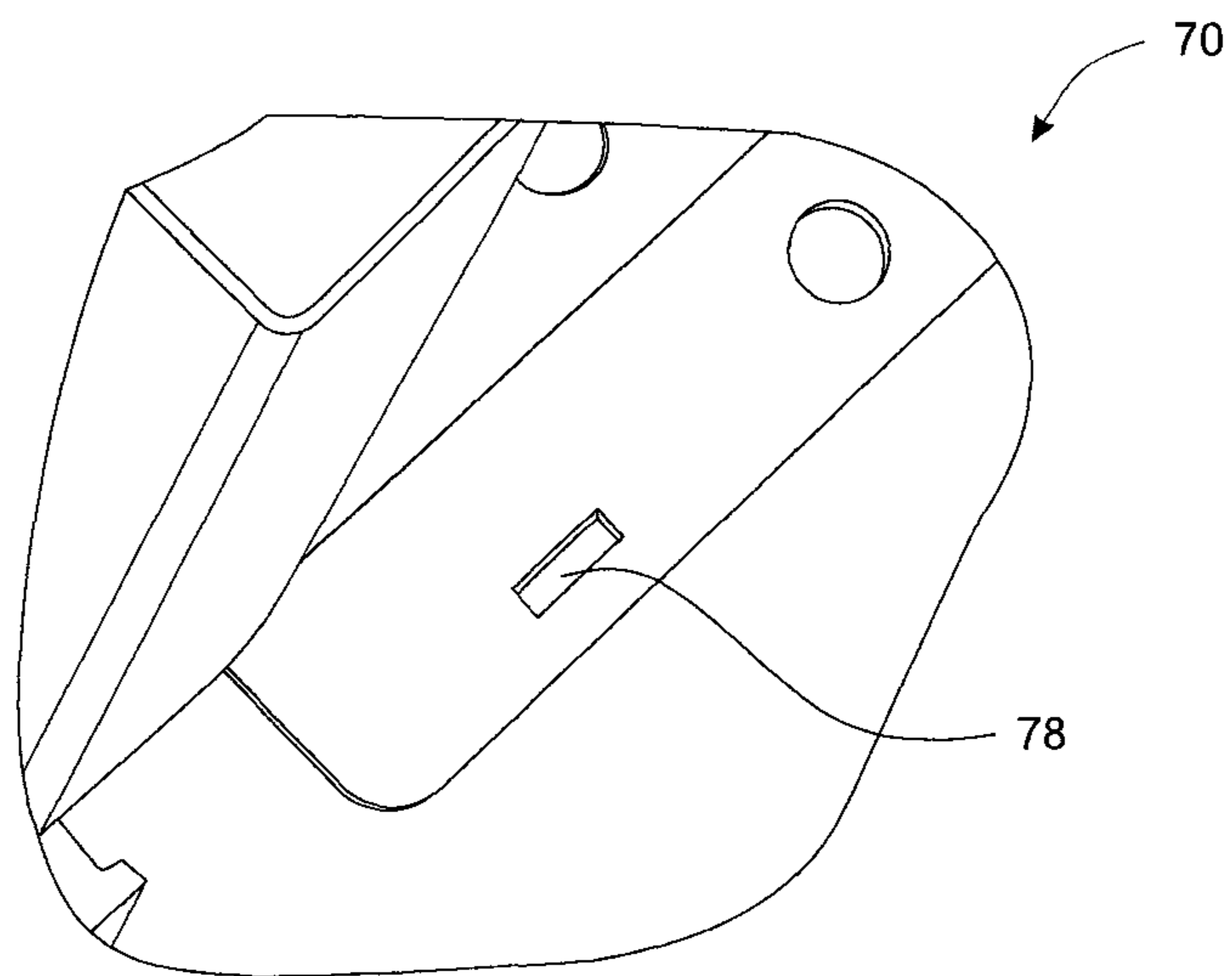
FIGURE 7
