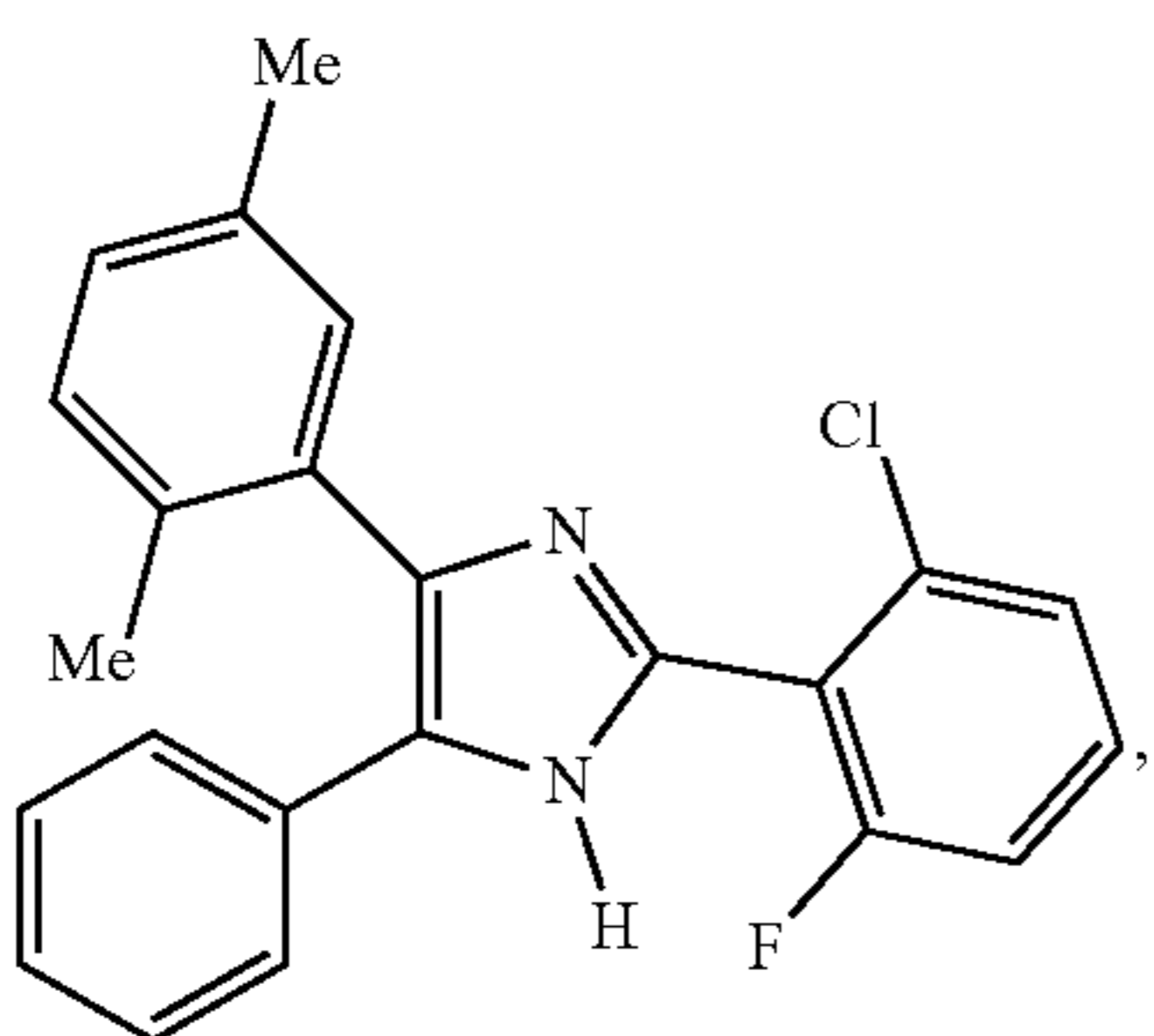
2-(2-chloro-6-fluorophenyl)-4-(2,5-dimethylphenyl)-5-phenyl-1H-imidazole
