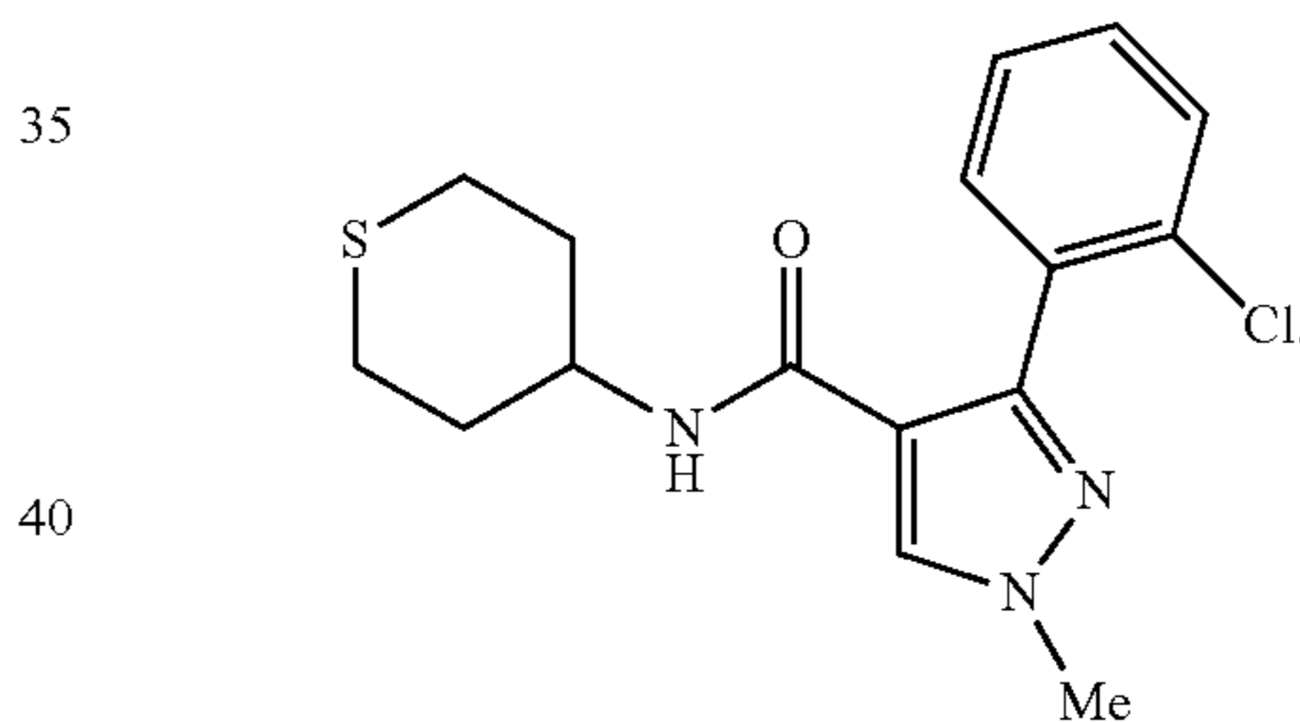
3-(2-chlorophenyl)-1-methyl-N-(tetrahydro-2H-thiopyran-4-yl)-1H-pyrazole-4-carboxamide
