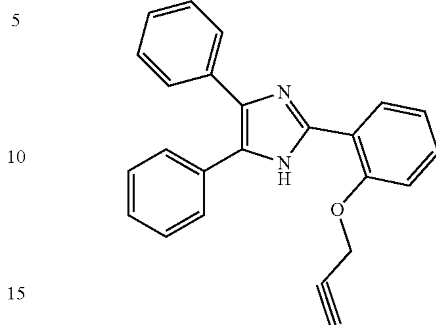
4,5-diphenyl-2-(2-(prop-2-yn-1-yloxy)phenyl)-1H-imidazole
