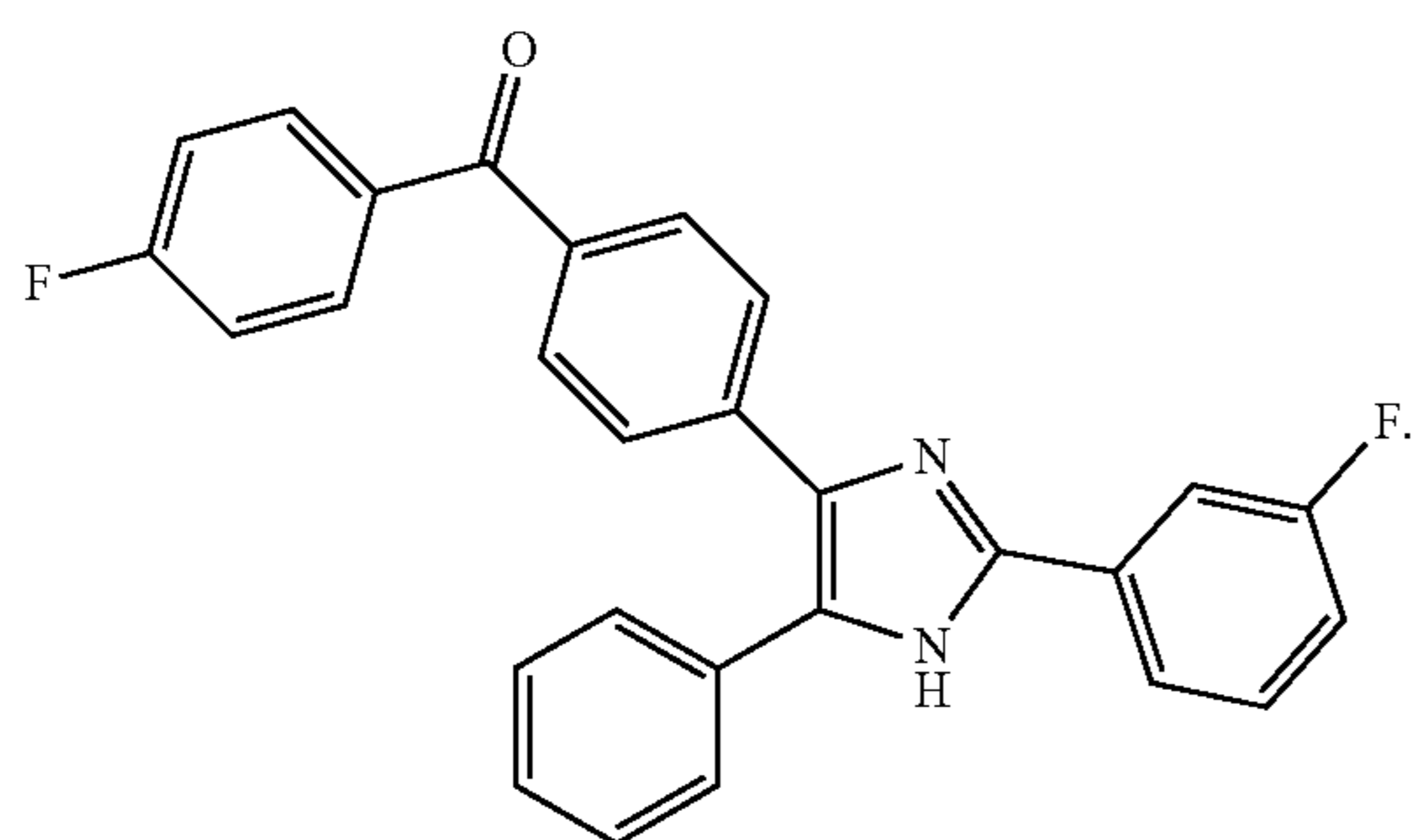
(4-fluorophenyl)(4-(2-(3-fluorophenyl)-5-phenyl-1H-imidazol-4-yl)phenyl)methanone
