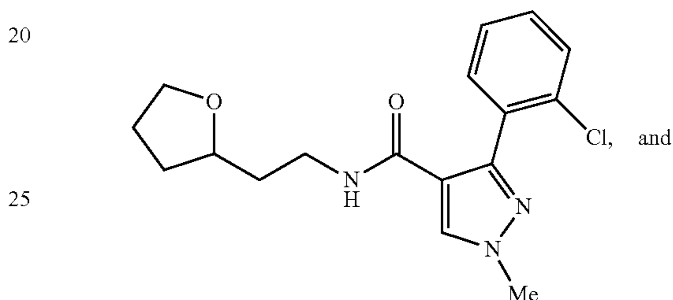
3-(2-chlorophenyl)-1-methyl-N-(2-(tetrahydrofuran-2-yl)ethyl)-1H-pyrazole-4-carboxamide
