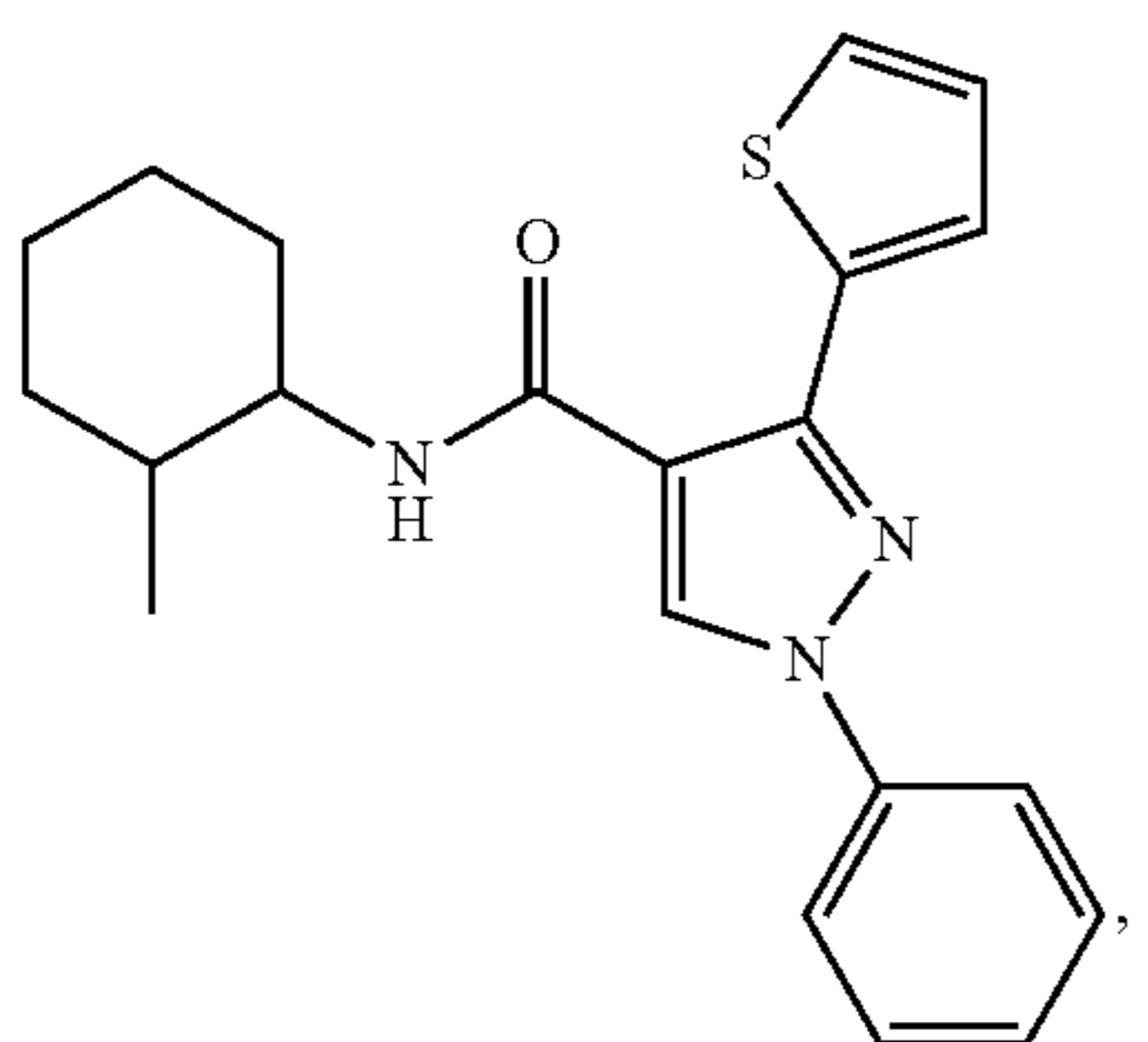
N-(2-methylcyclohexyl)-1-phenyl-3-(thiophen-2-yl)-1H-pyrazole-4-carboxamide
