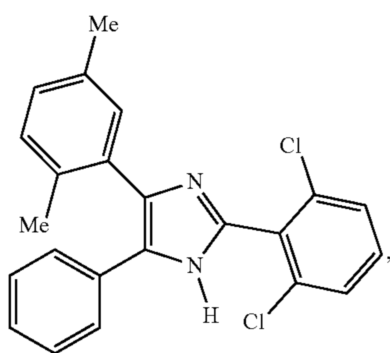
2-(2,6-dichlorophenyl)-4-(2,5-dimethylphenyl)-5-phenyl-1H-imidazole
