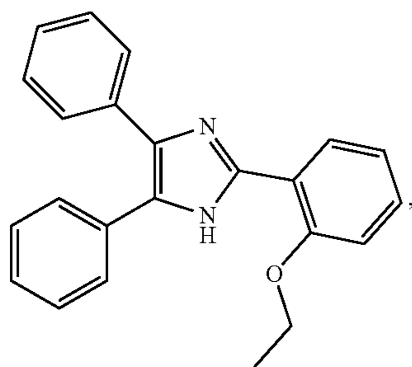
2-(2-ethoxyphenyl)-4,5-diphenyl-1H-imidazole
