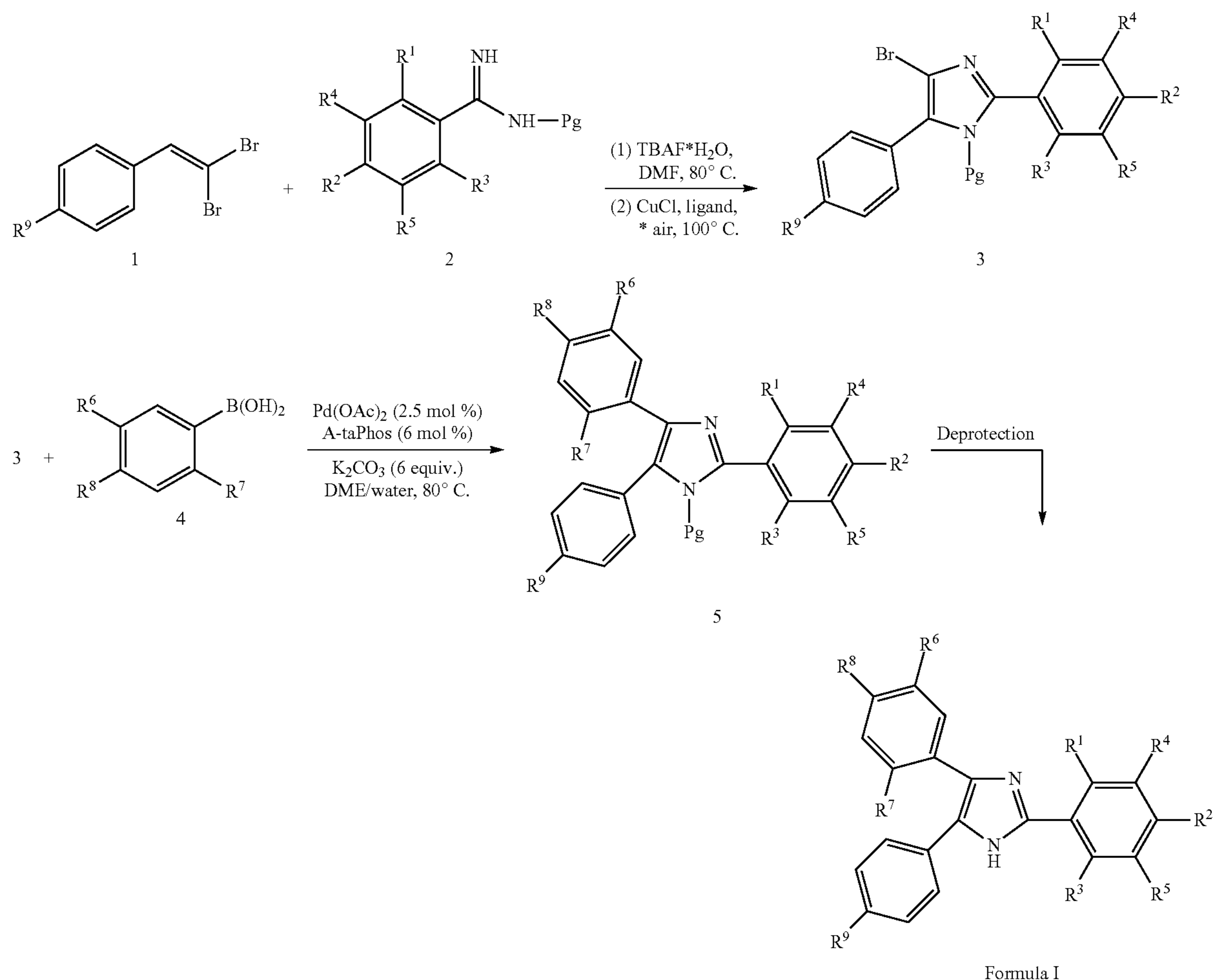
Scheme 1: Synthetic scheme for the preparation of compounds of Formula I
