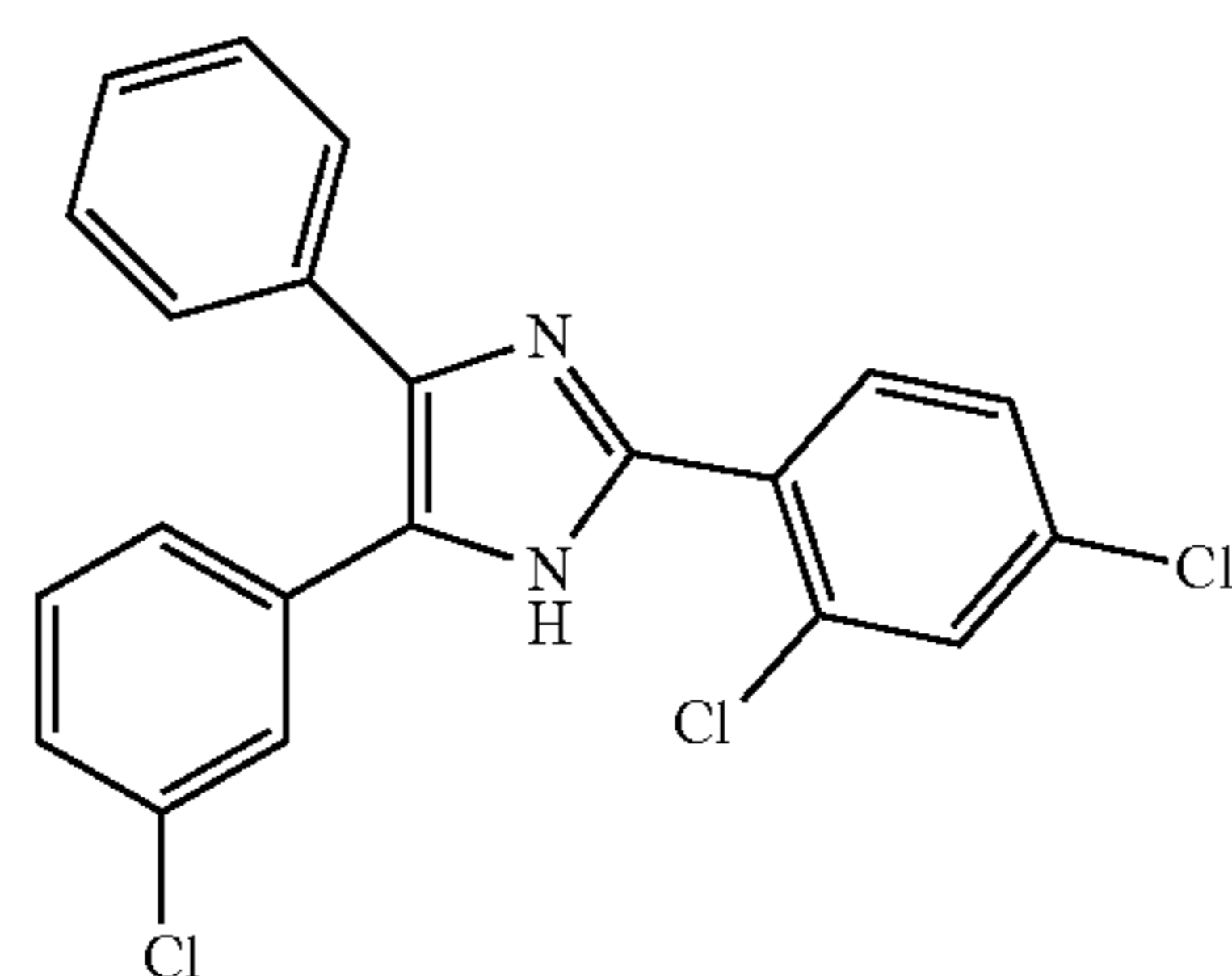
5-(3-chlorophenyl)-2-(2,4-dichlorophenyl)-4-phenyl-1H-imidazole
