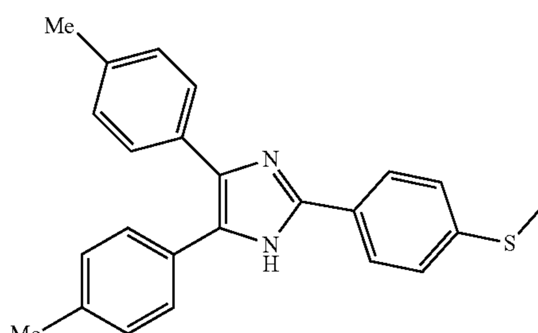
2-(4-(methylthio)phenyl)-4,5-di-p-tolyl-1H-imidazole
