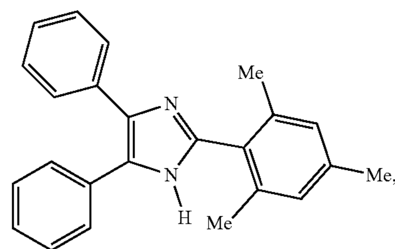
2-mesityl-4,5-diphenyl-1H-imidazole
