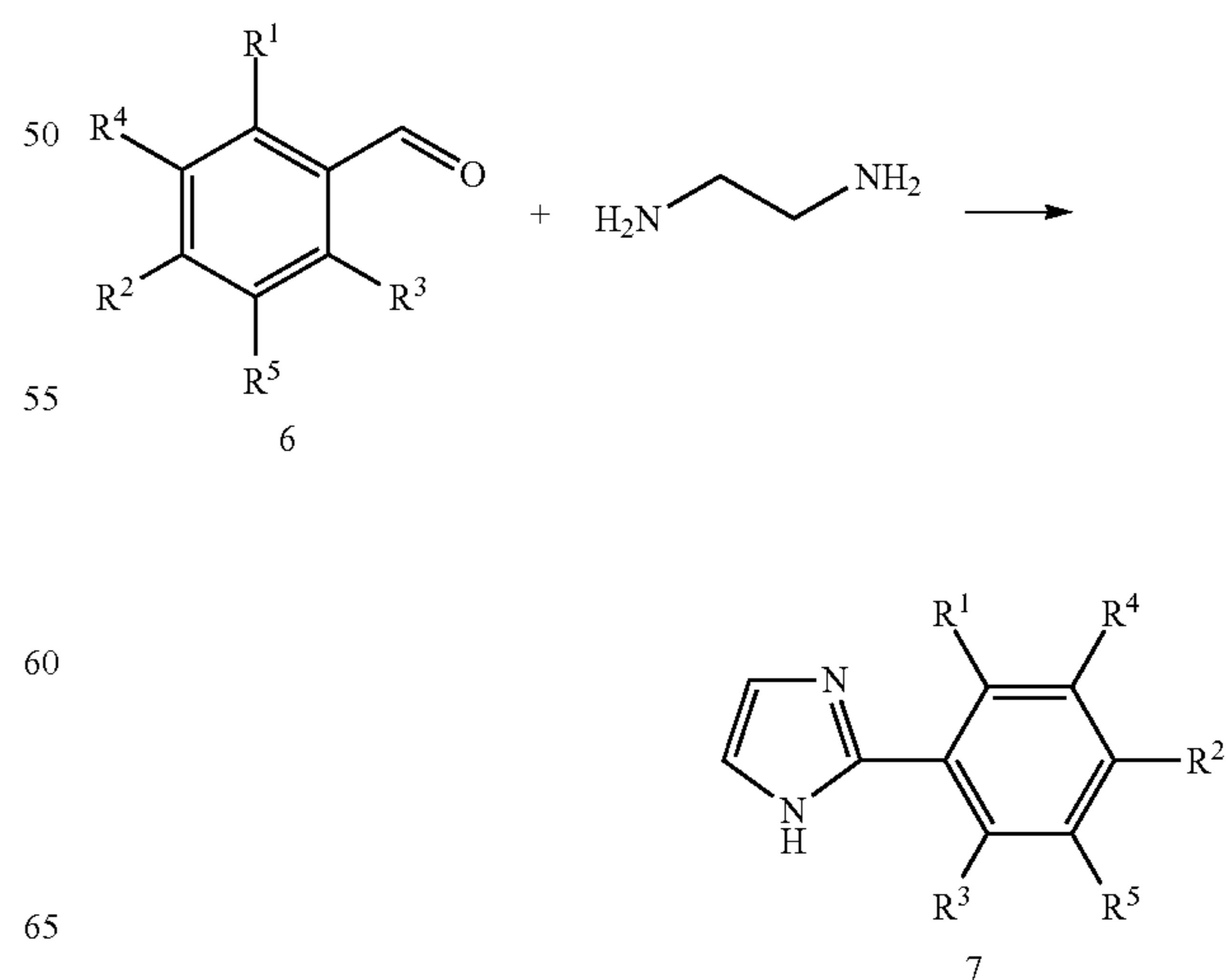
Scheme 2: Synthetic Scheme for the preparation of compounds of Formula I
