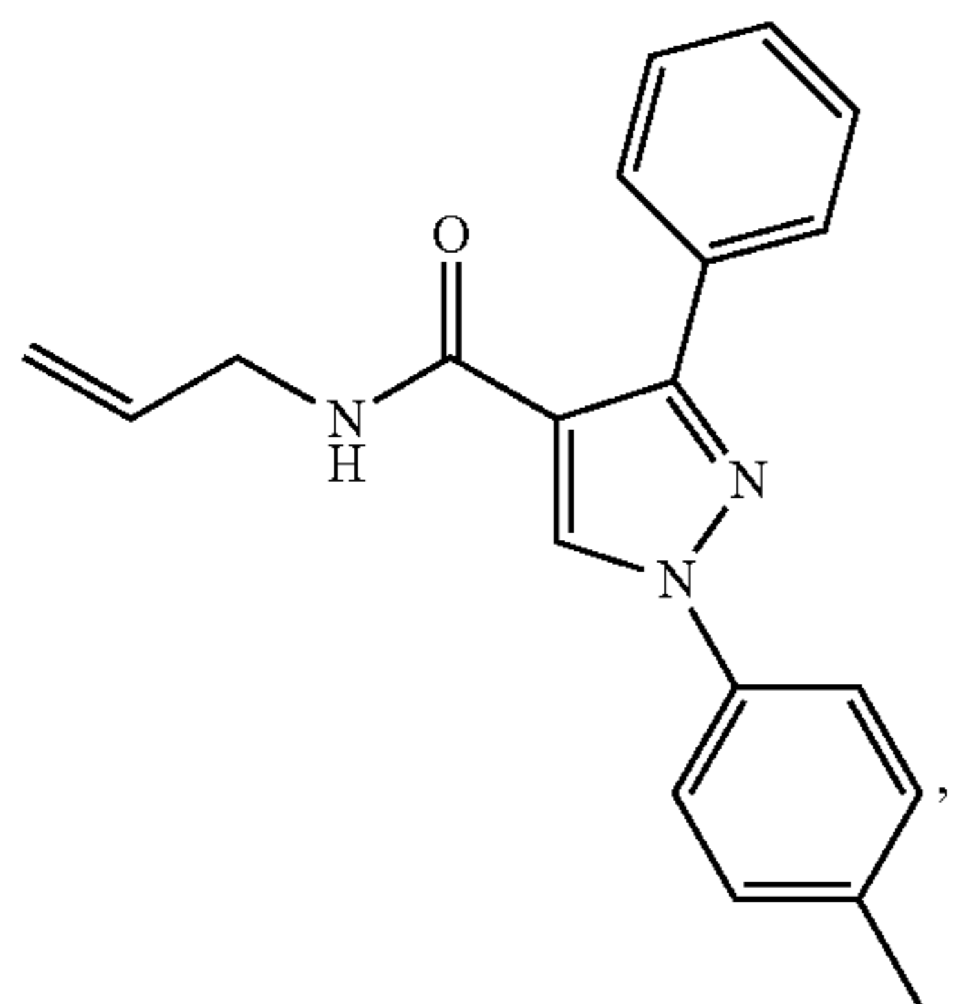
N-allyl-3-phenyl-1-(p-tolyl)-1H-pyrazole-4-carboxamide
