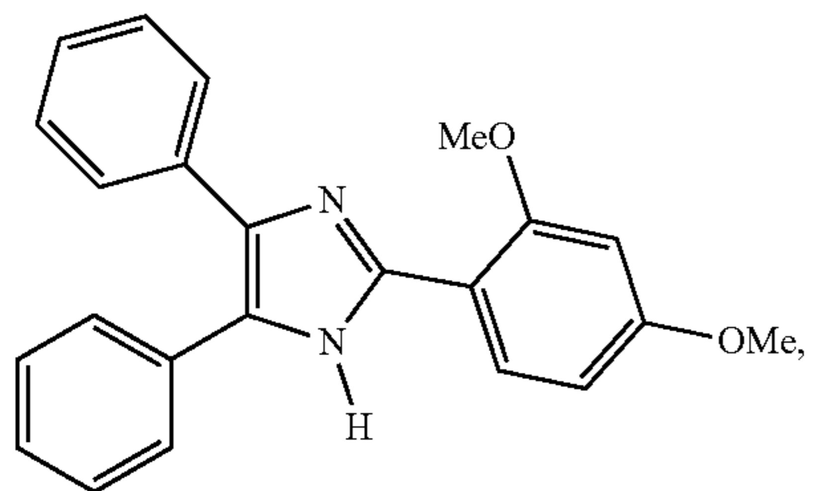
2-(2,4-dimethoxyphenyl)-4,5-diphenyl-1H-imidazole
