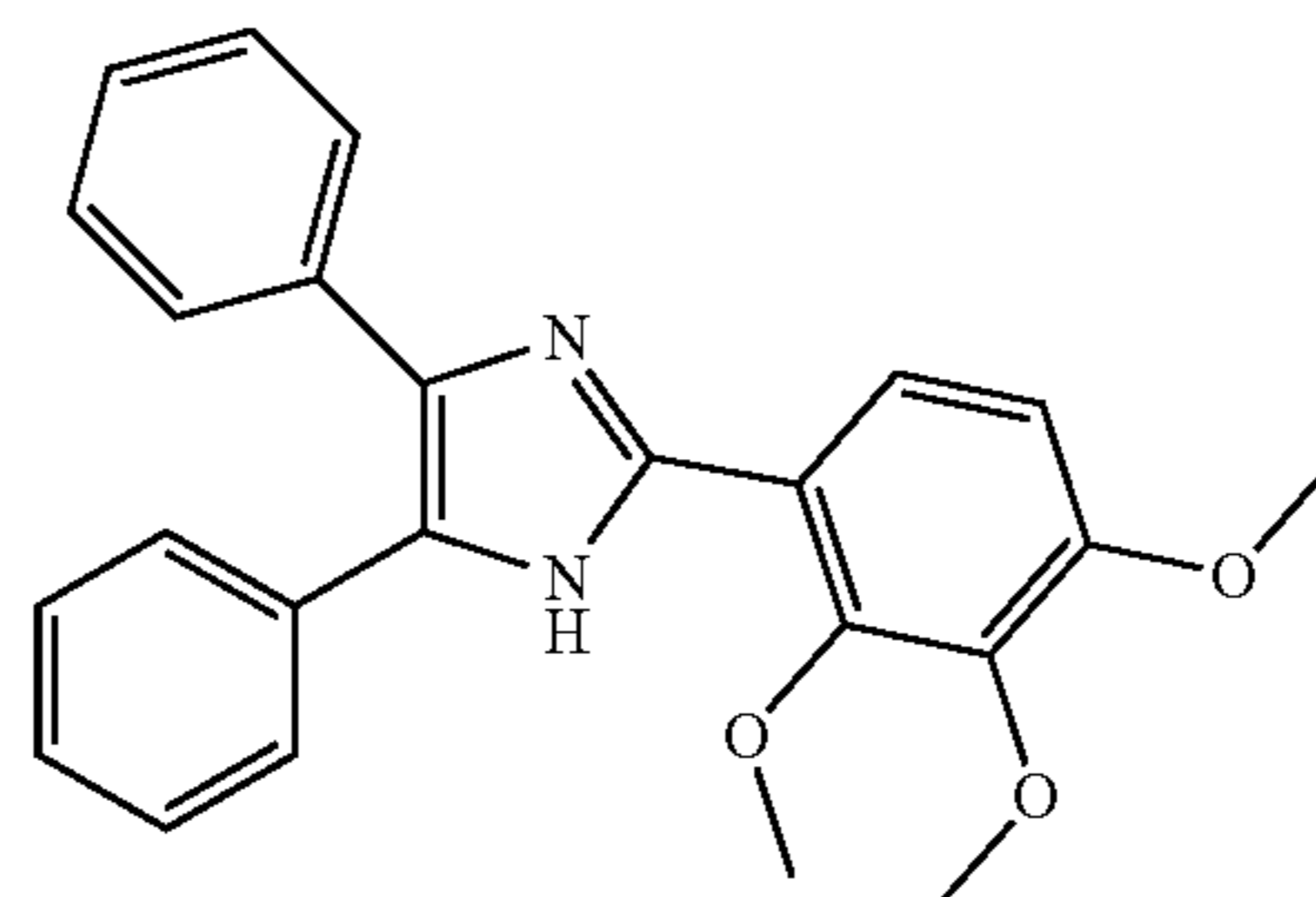
4,5-diphenyl-2-(2,3,4-trimethoxyphenyl)-1H-imidazole
