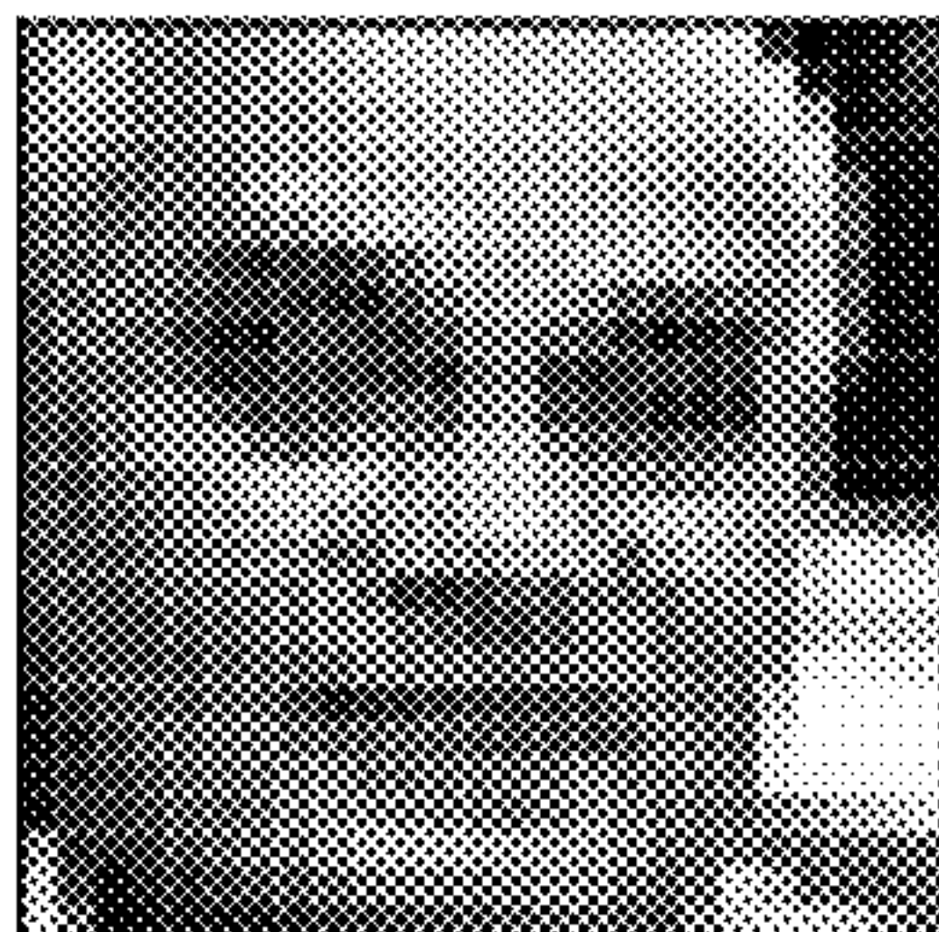
First-Images
