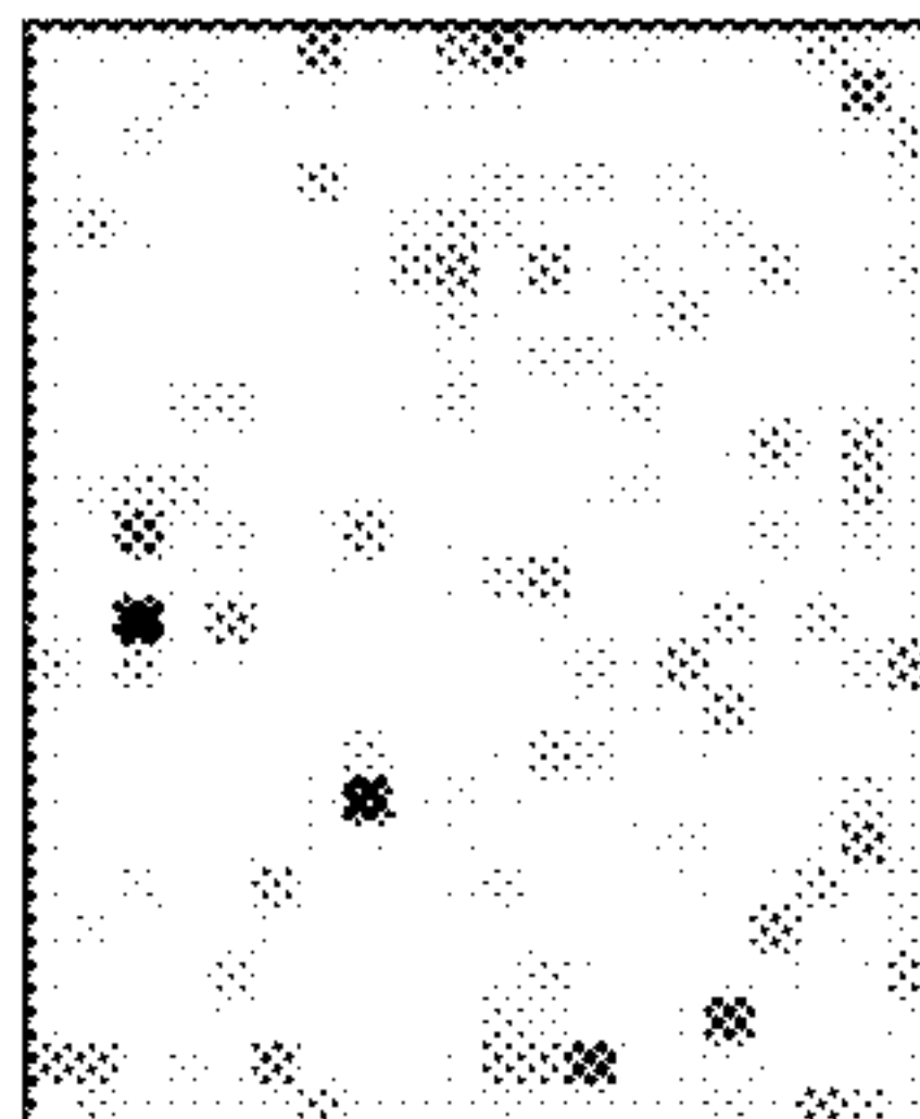
Pseudo-images
