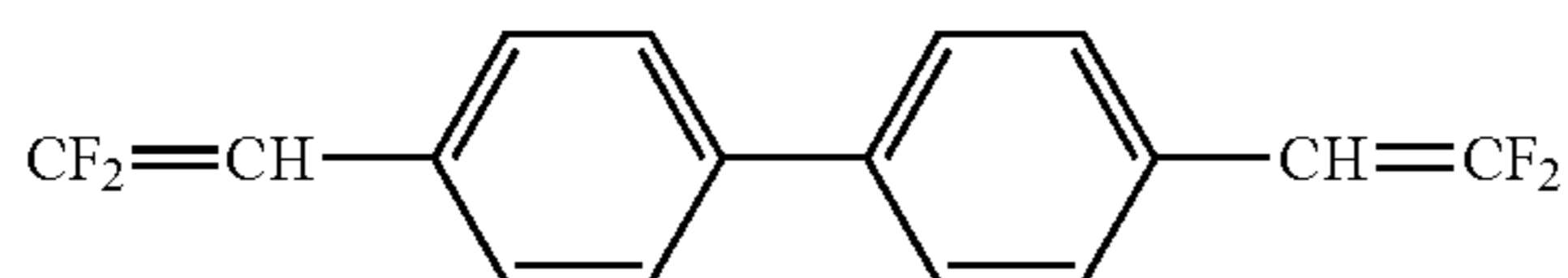
(Compound 2)
