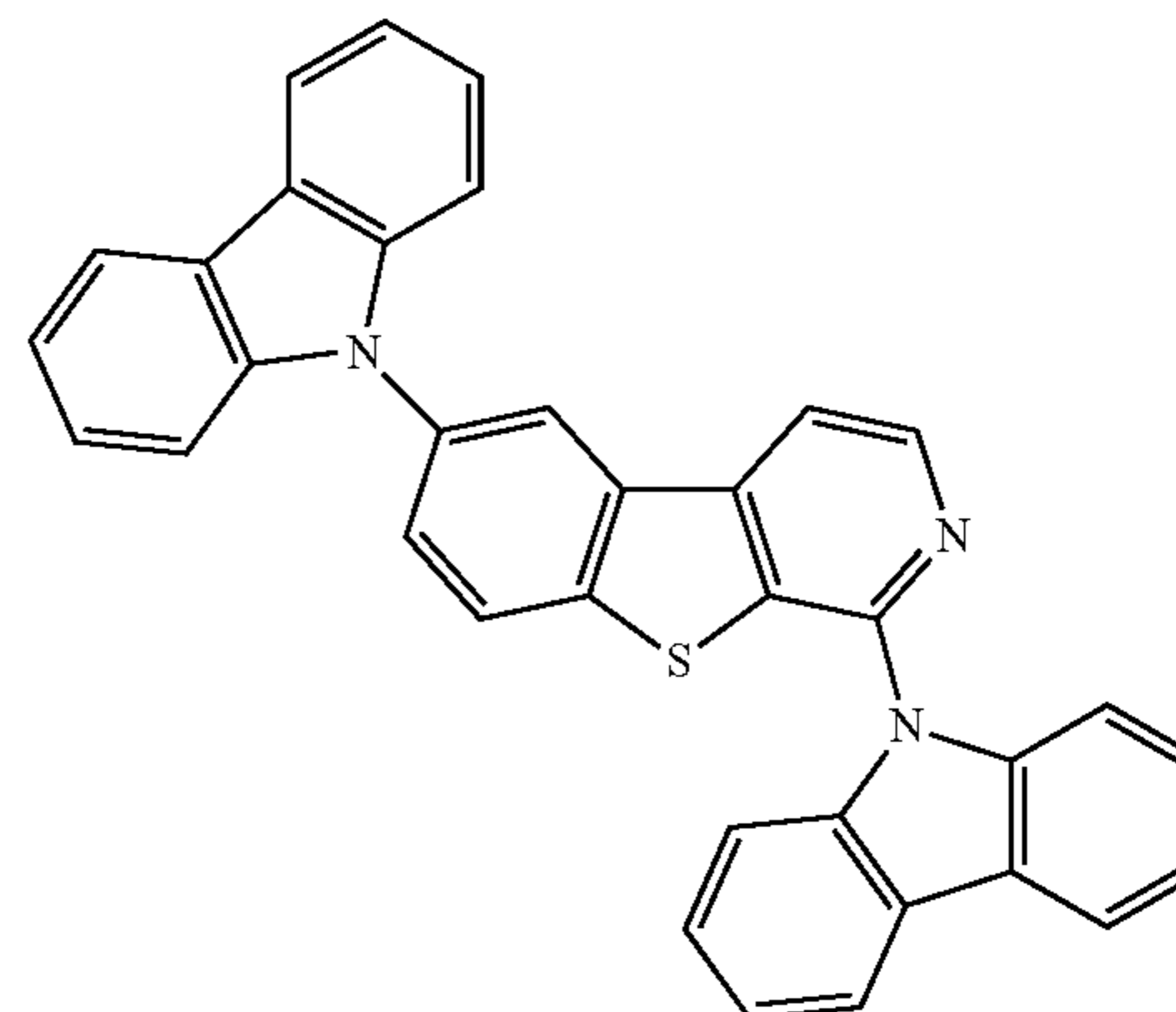
Compound 3
