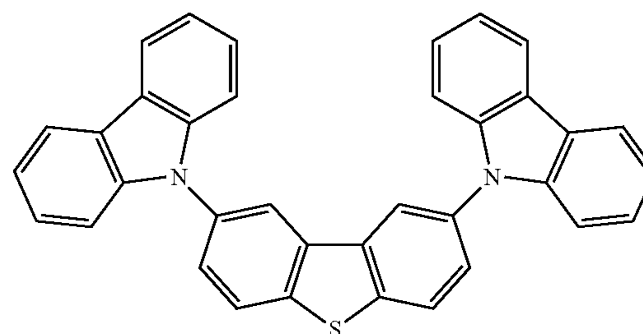
Compound 4
