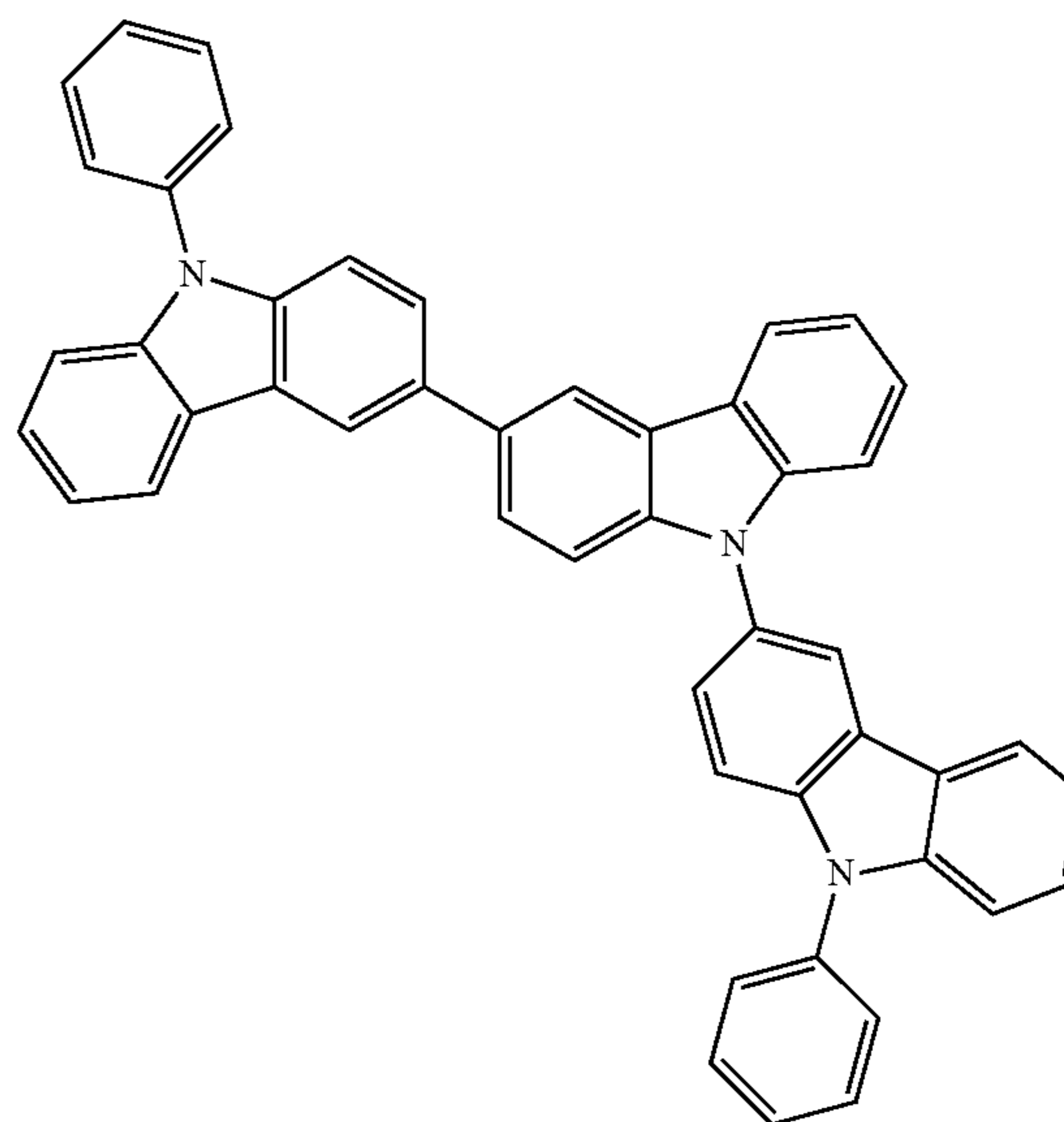
Compound 10
