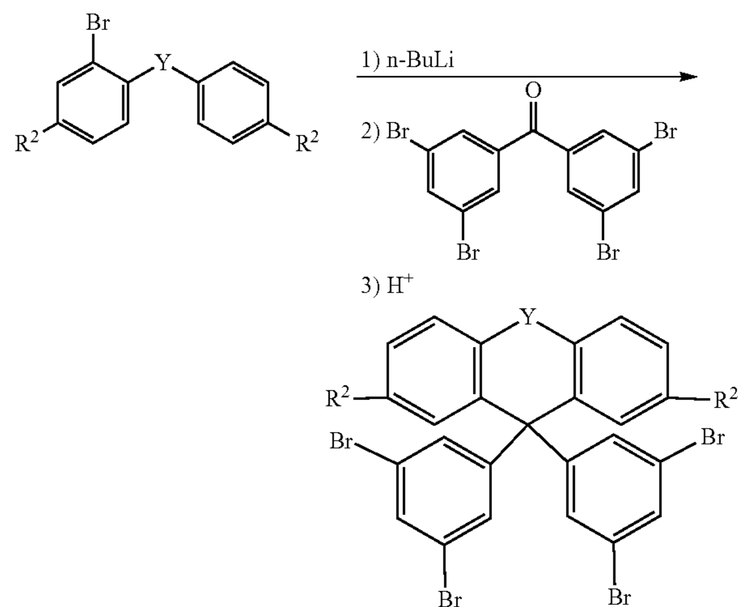
Scheme 1
