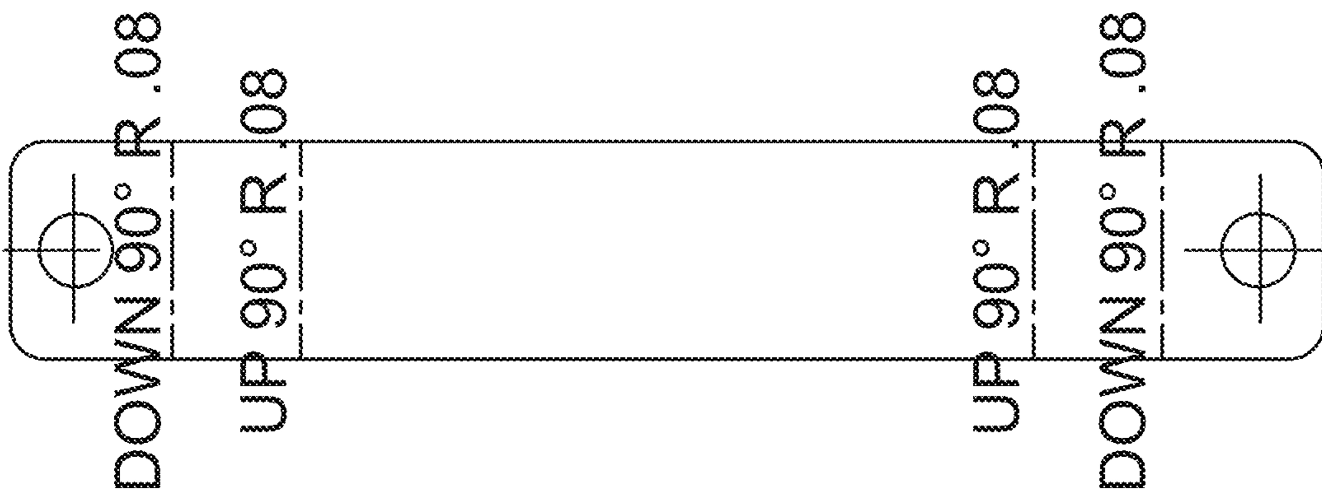
FLAT PATTERN
