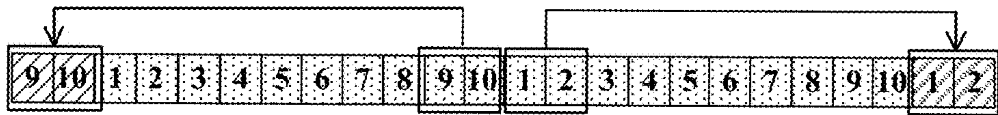
(c)OFDM baseband signal generation method-3 for Alt-3
