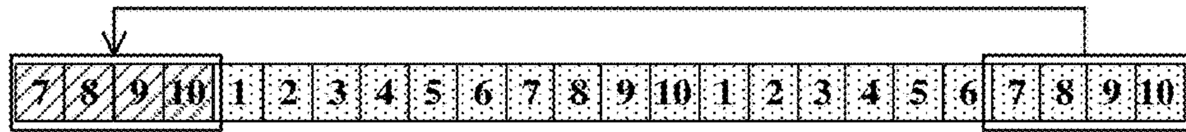
(a)OFDM baseband signal generation method-1 for two-symbol RS
