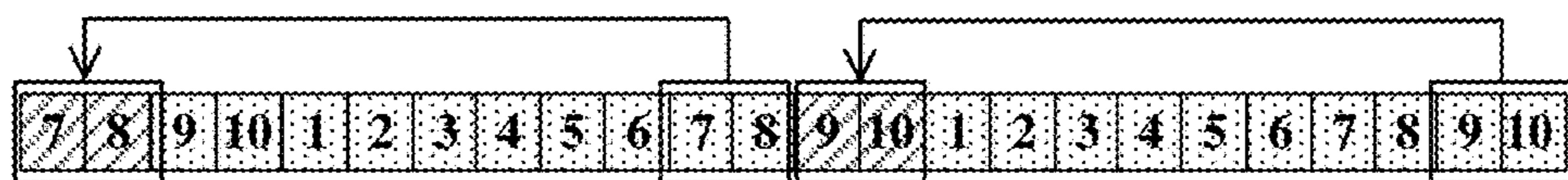
(b)OFDM baseband signal generation method-2 for two-symbol RS
