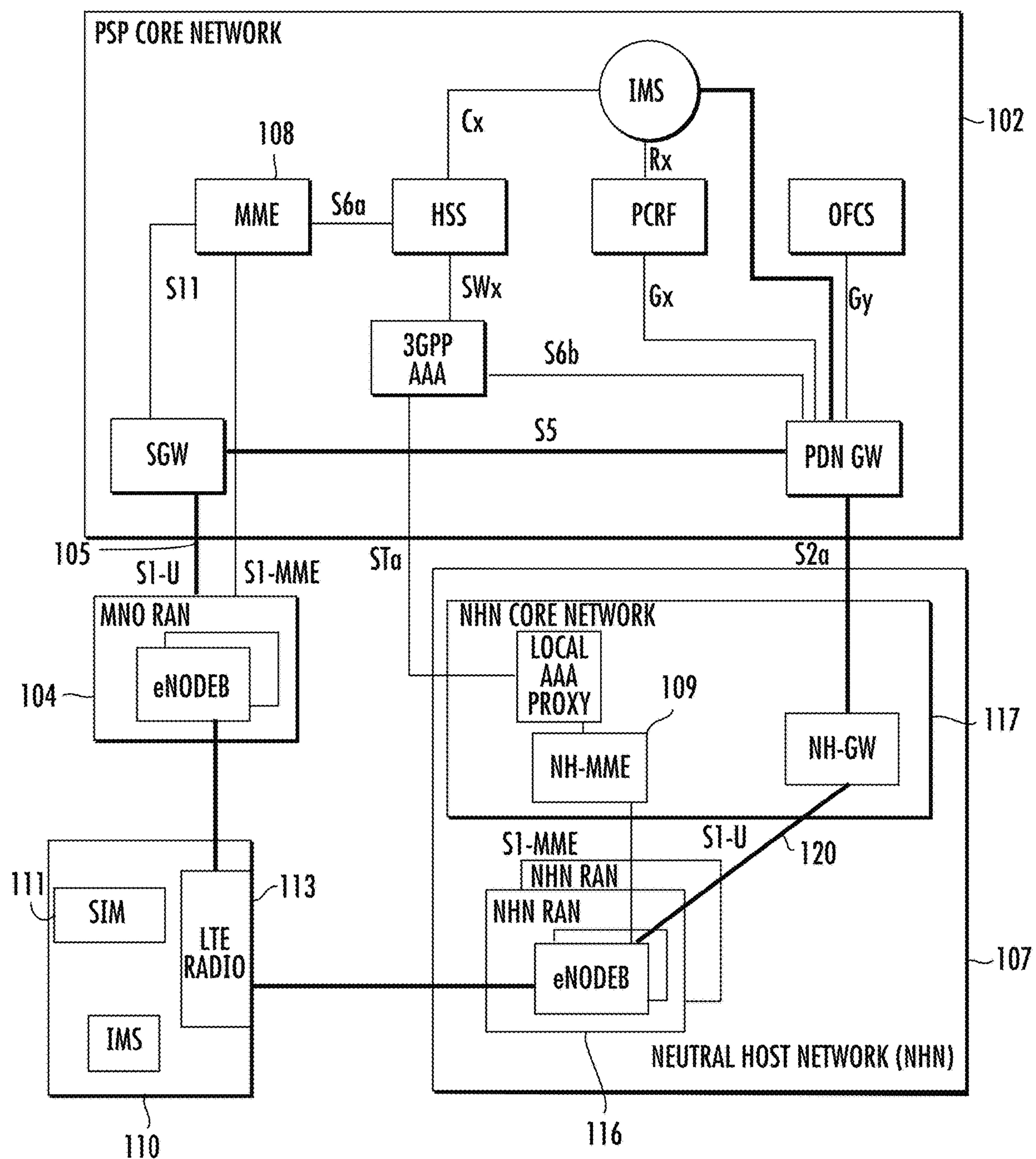
FIG. 1 PRIOR ART
