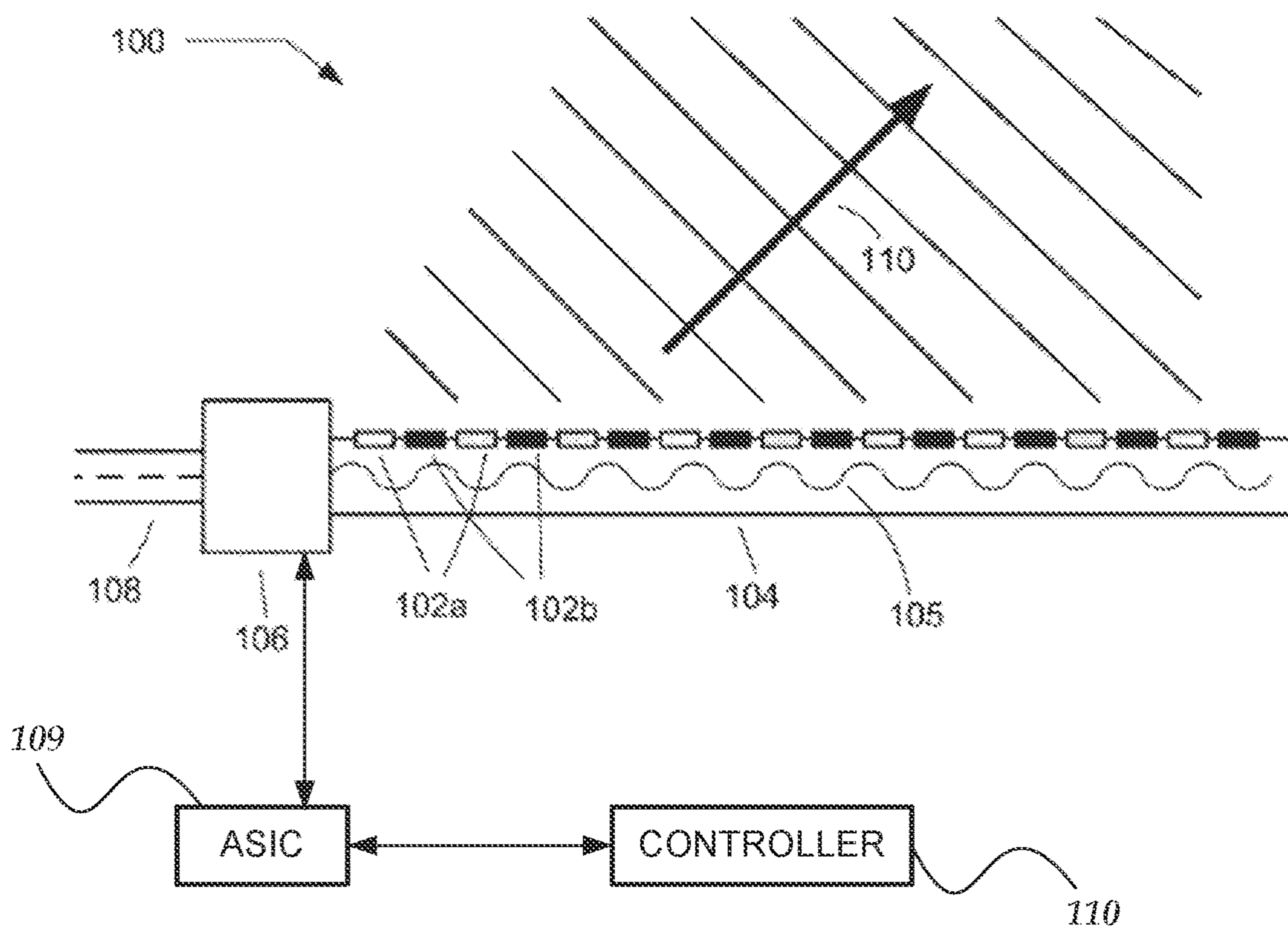
FIG. 1C – PRIOR ART
