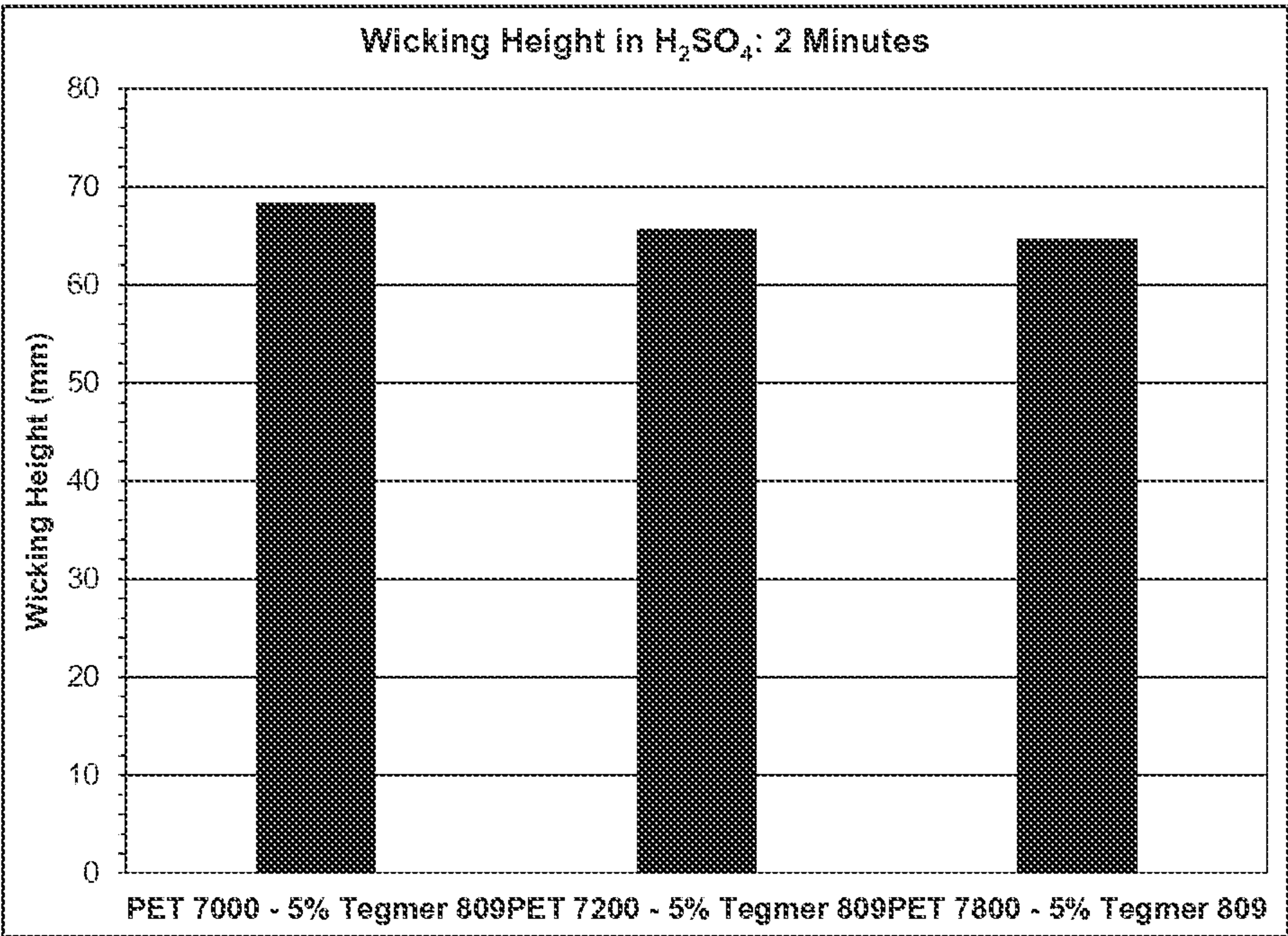
Fig. 9. Two-minute wicking performance of melt blown polymer fiber sheets prepared from different PET resins.
