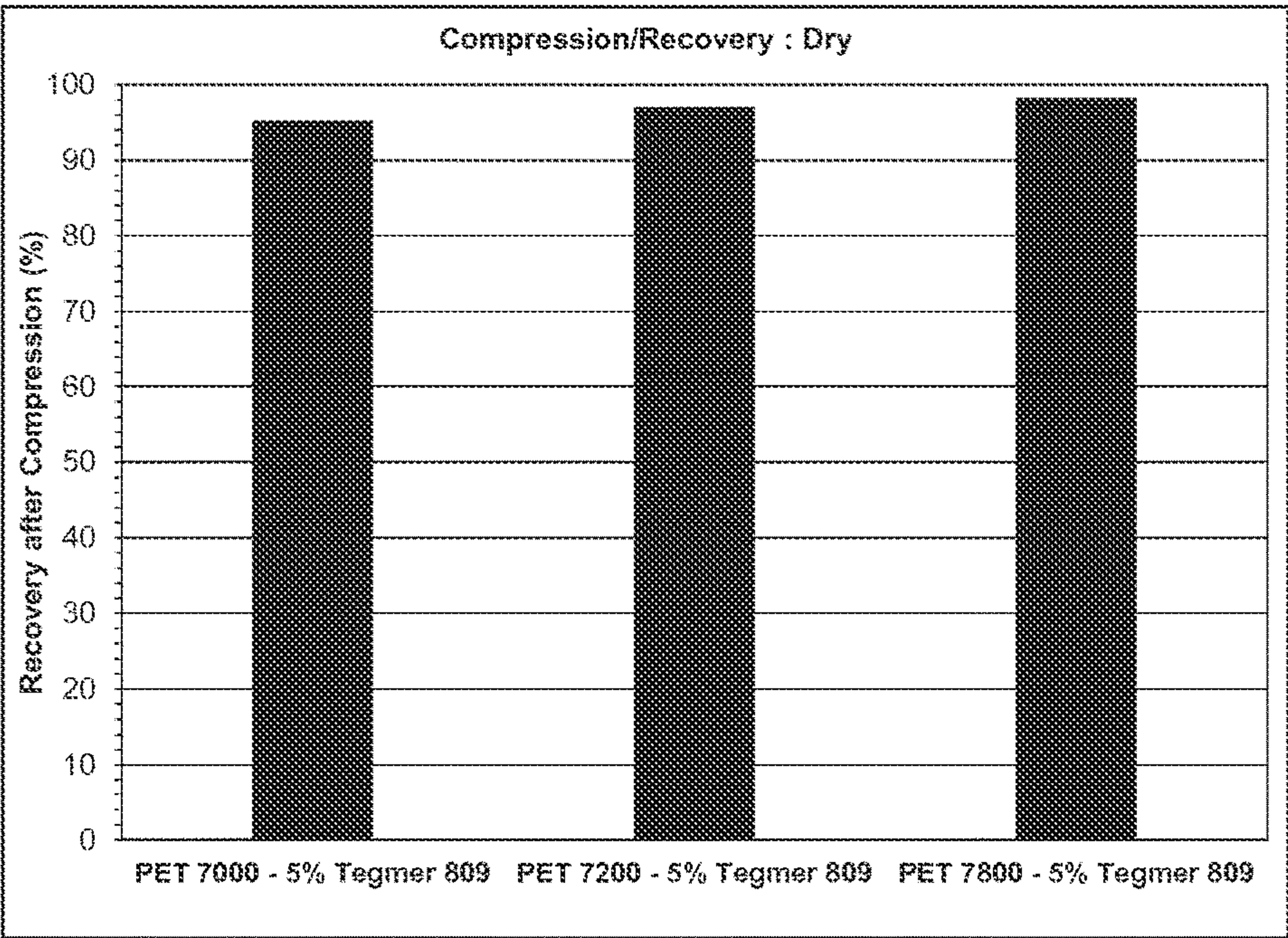
Fig. 11. Compression recovery results of melt blown polymer fiber sheets prepared from different PET resins.
