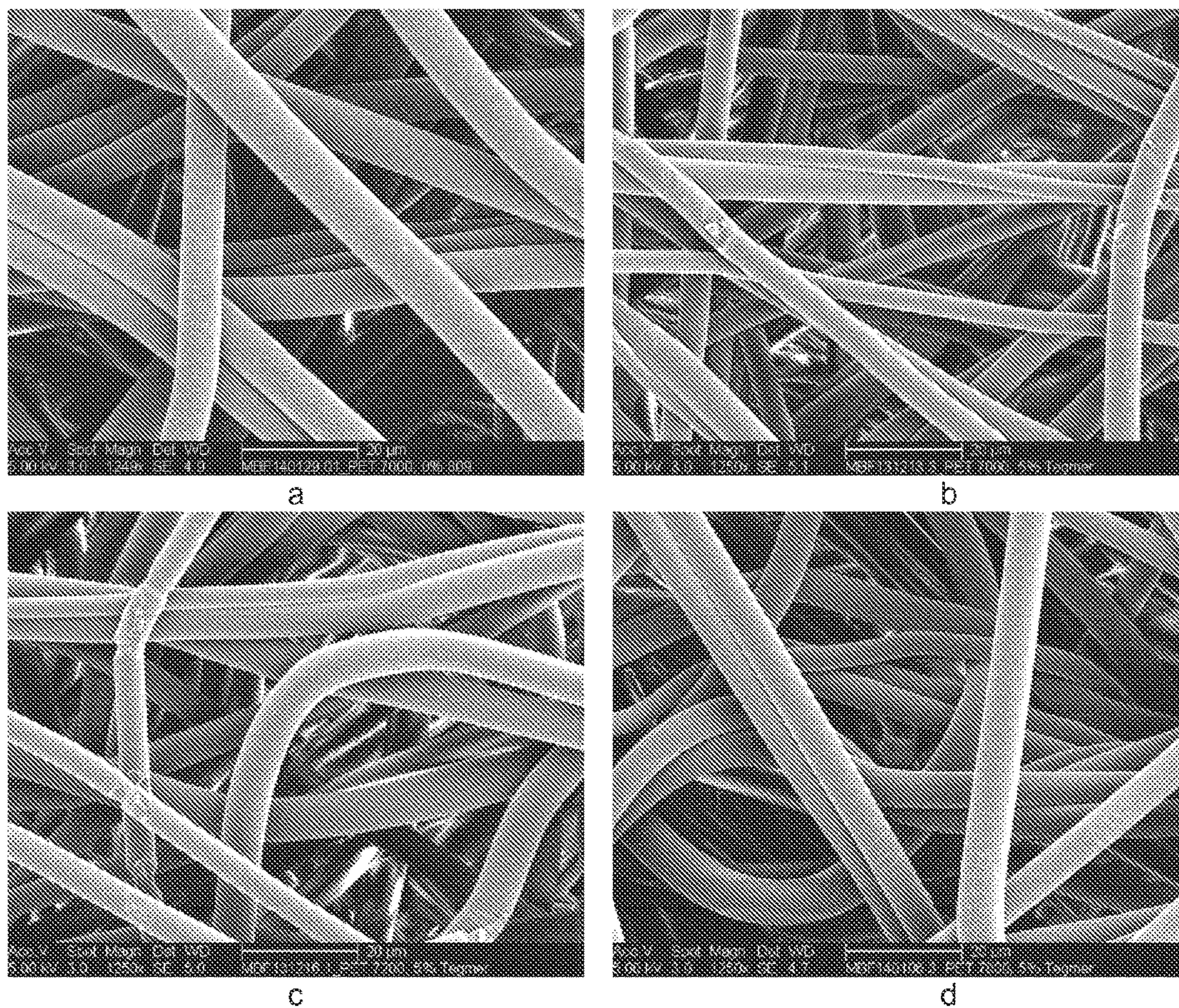
Fig. 7. Scanning electron micrographs of the melt blown polymer fiber sheets prepared from (a) neat PET 7000, (b) PET 7000 with 5 wt.% TegMeR® 809, (c) PET 7200 with 5 wt.% TegMeR® 809, and (d) PET 7800 with 5 wt.% TegMeR® 809.
