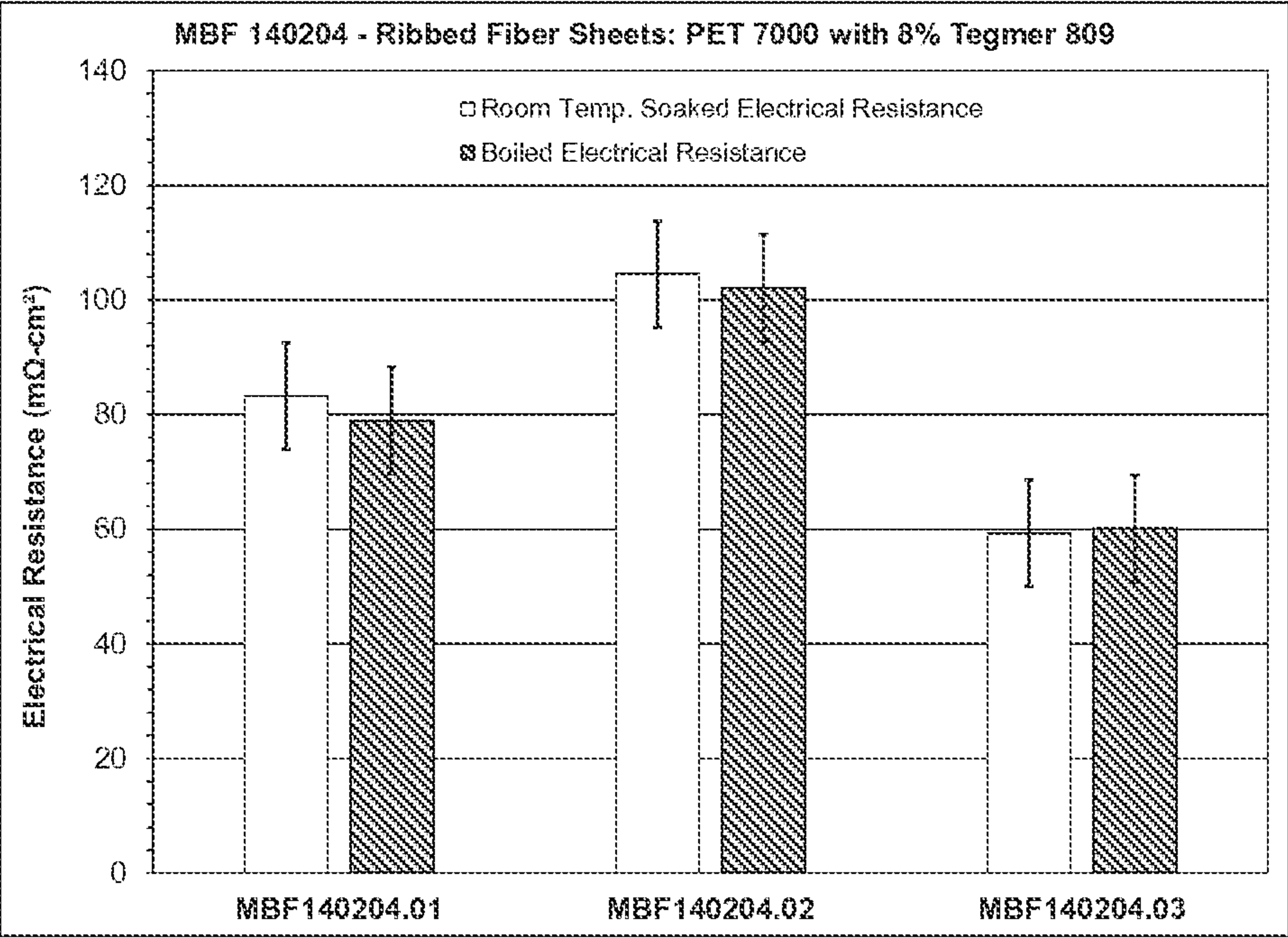
Fig. 19. Electrical resistance of ribbed PET fiber sheets.
