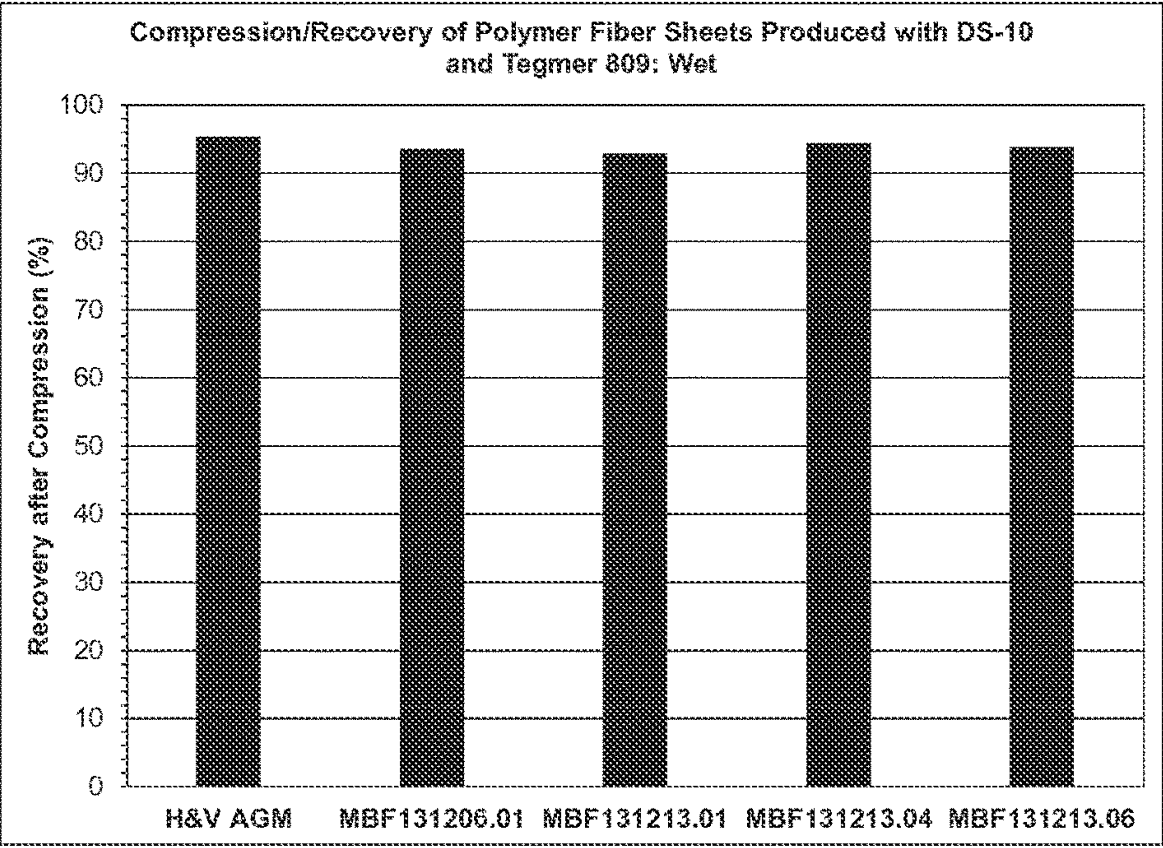
Fig. 18. Recovery after compression of PET fiber sheets with DS-10 and TegMeR® 809 – wet condition.
