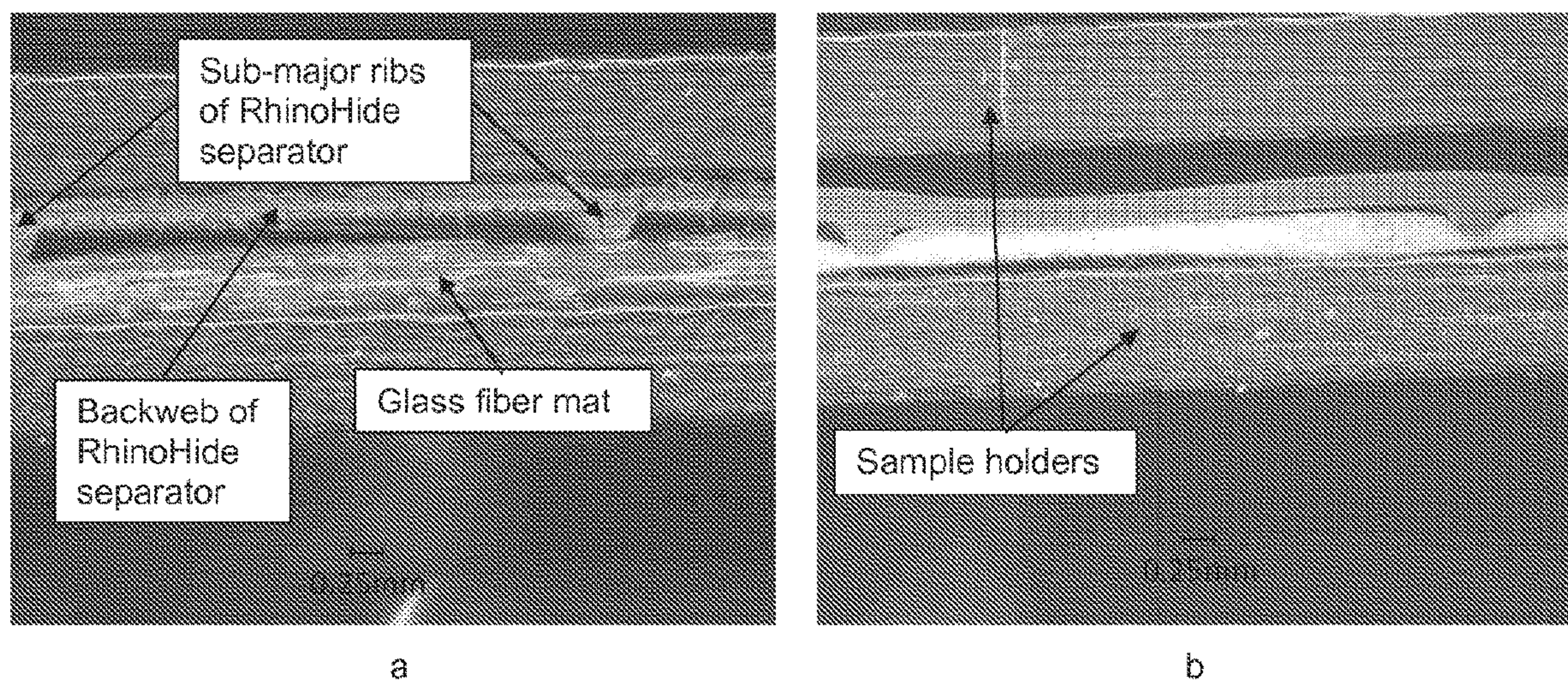
Fig. 23. Optical micrographs at the interfaces of (a) RhinoHide® separator-glass fiber mat and (b) RhinoHide® separator-PET fiber sheet.
