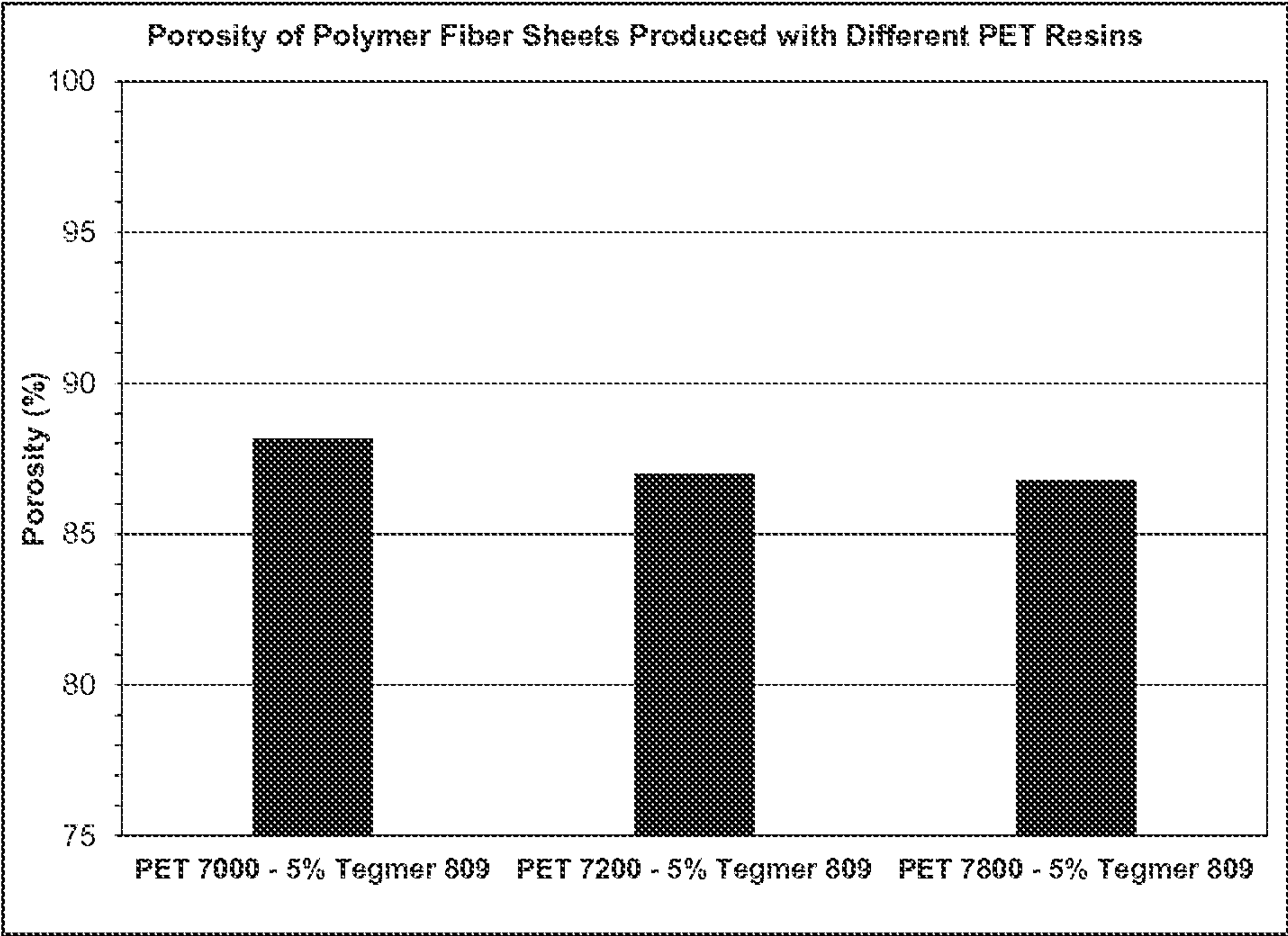
Fig. 8. Porosity of fiber sheets prepared from different PET resins.
