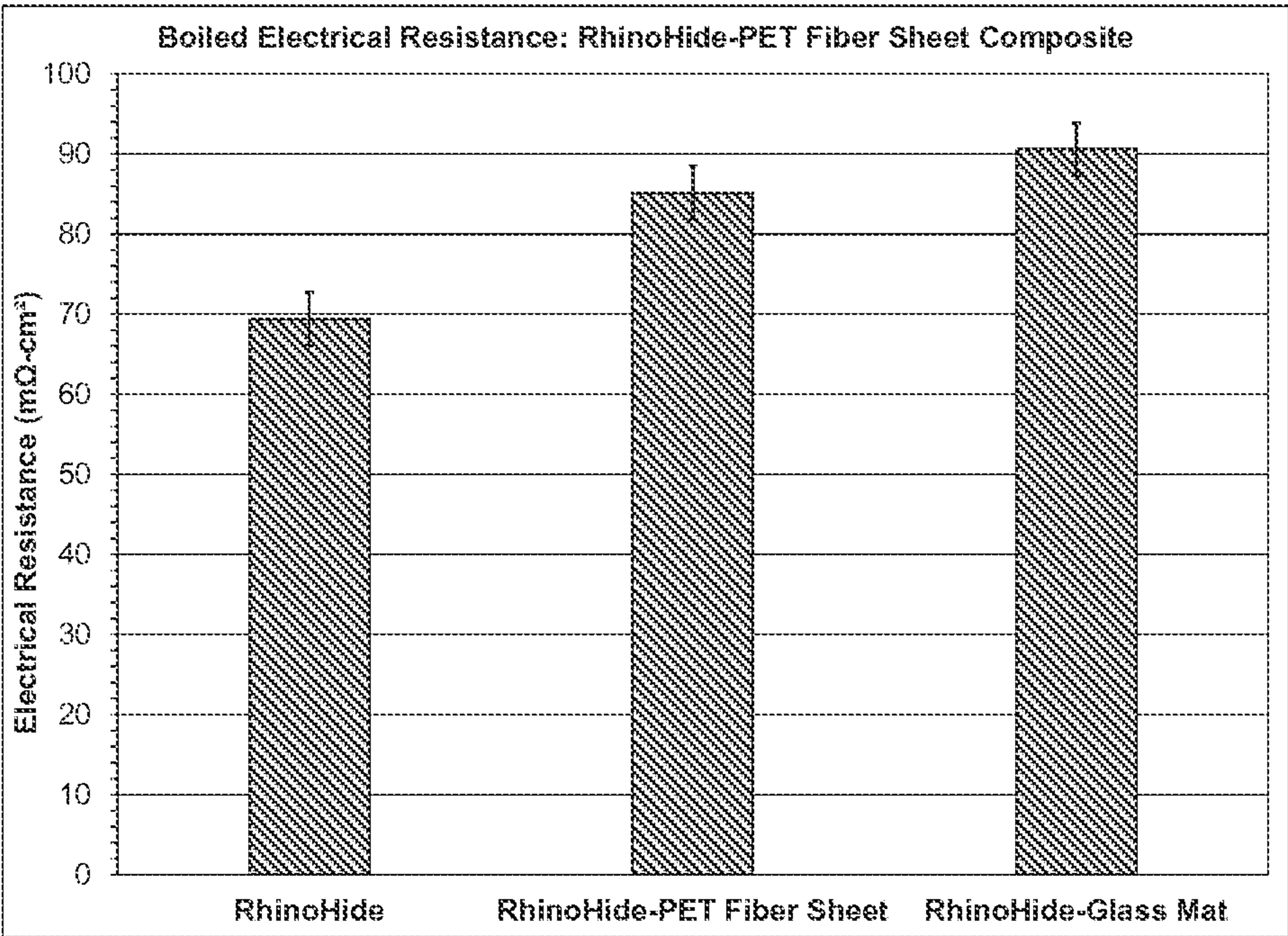
Fig. 26. Boiled electrical resistance of the traditional RhinoHide® separator-glass fiber mat laminate and the RhinoHide® separator-PET fiber sheet composite.
