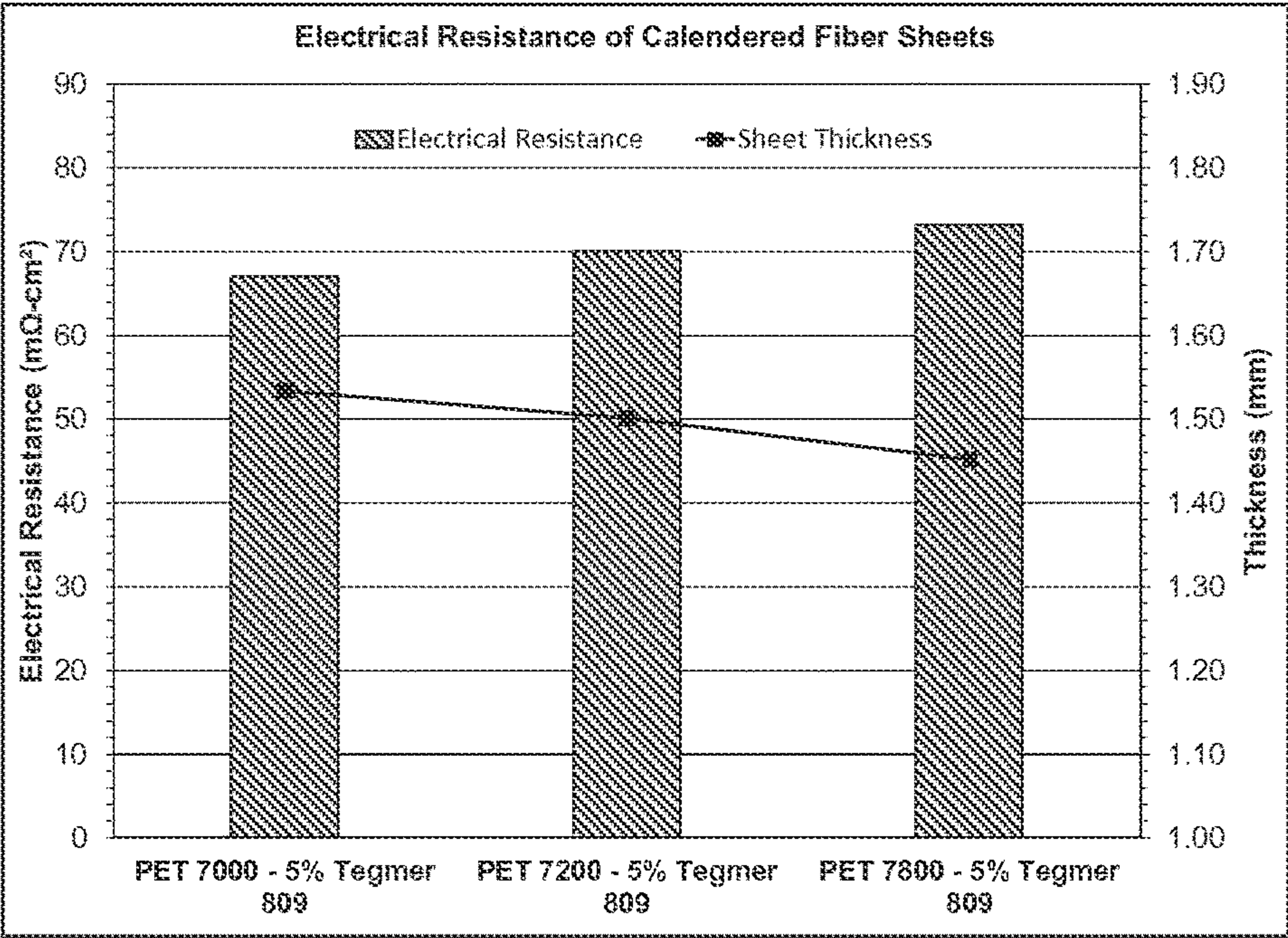
Fig. 10. Electrical resistance of melt blown polymer fiber sheets prepared from different PET resins.
