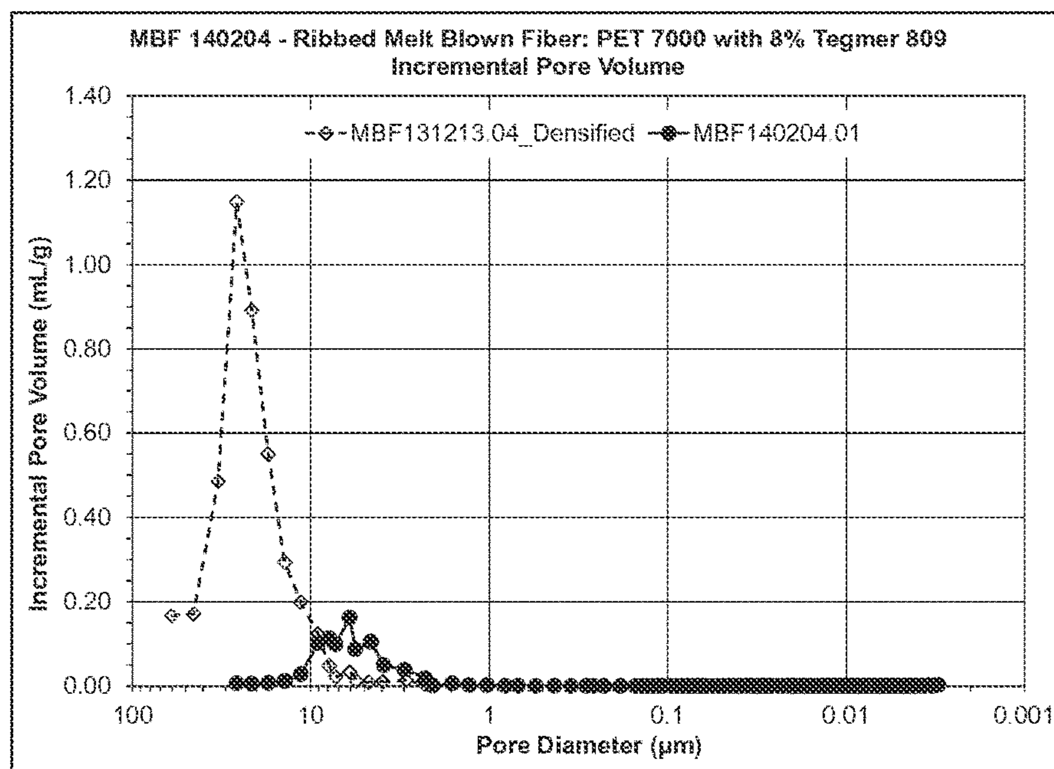
Fig. 21. Pore size distributions by mercury intrusion porosimetry of a densified PET fiber sheet and a ribbed PET fiber sheet.
