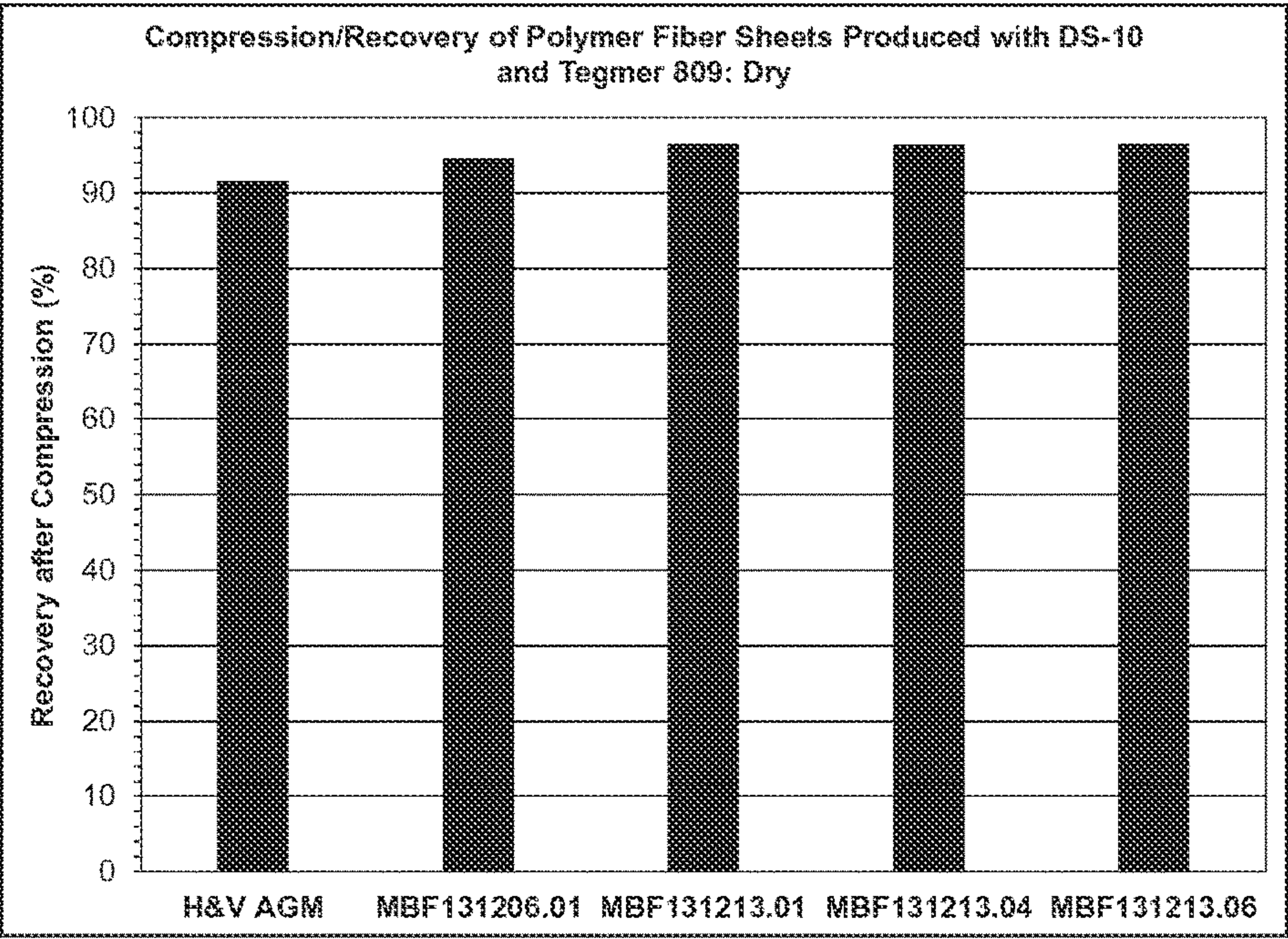
Fig. 17. Recovery after compression of PET fiber sheets with DS-10 and TegMeR® 809 – dry condition.
