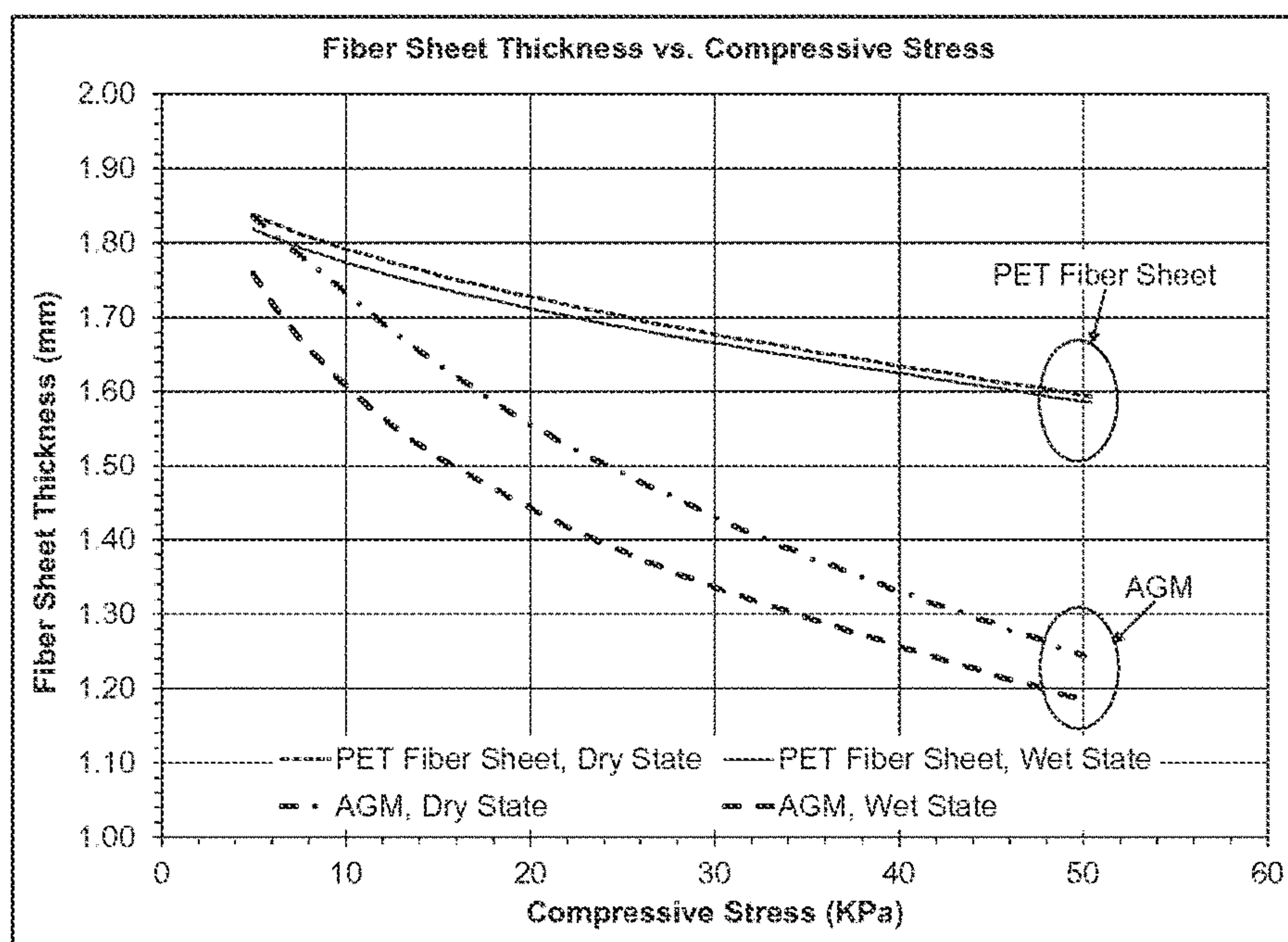
Fig. 16. Change in thickness vs. applied compressive stress for AGM and PET fiber sheets. The tests were performed in both dry and wet states for each AGM and PET fiber sheet.
