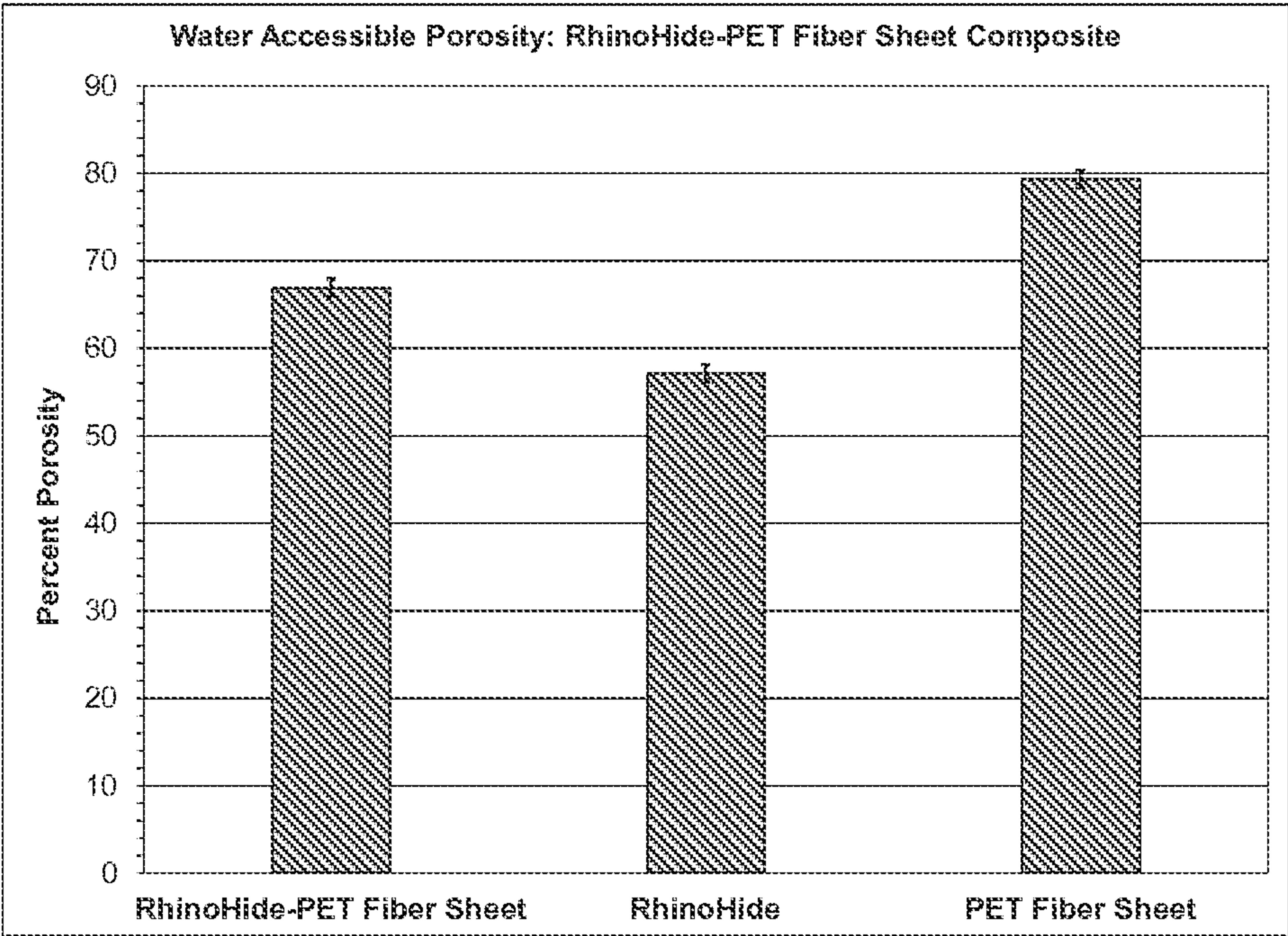
Fig. 25. Water accessible porosity of the RhinoHide® separator-PET fiber sheet composite and its components.
