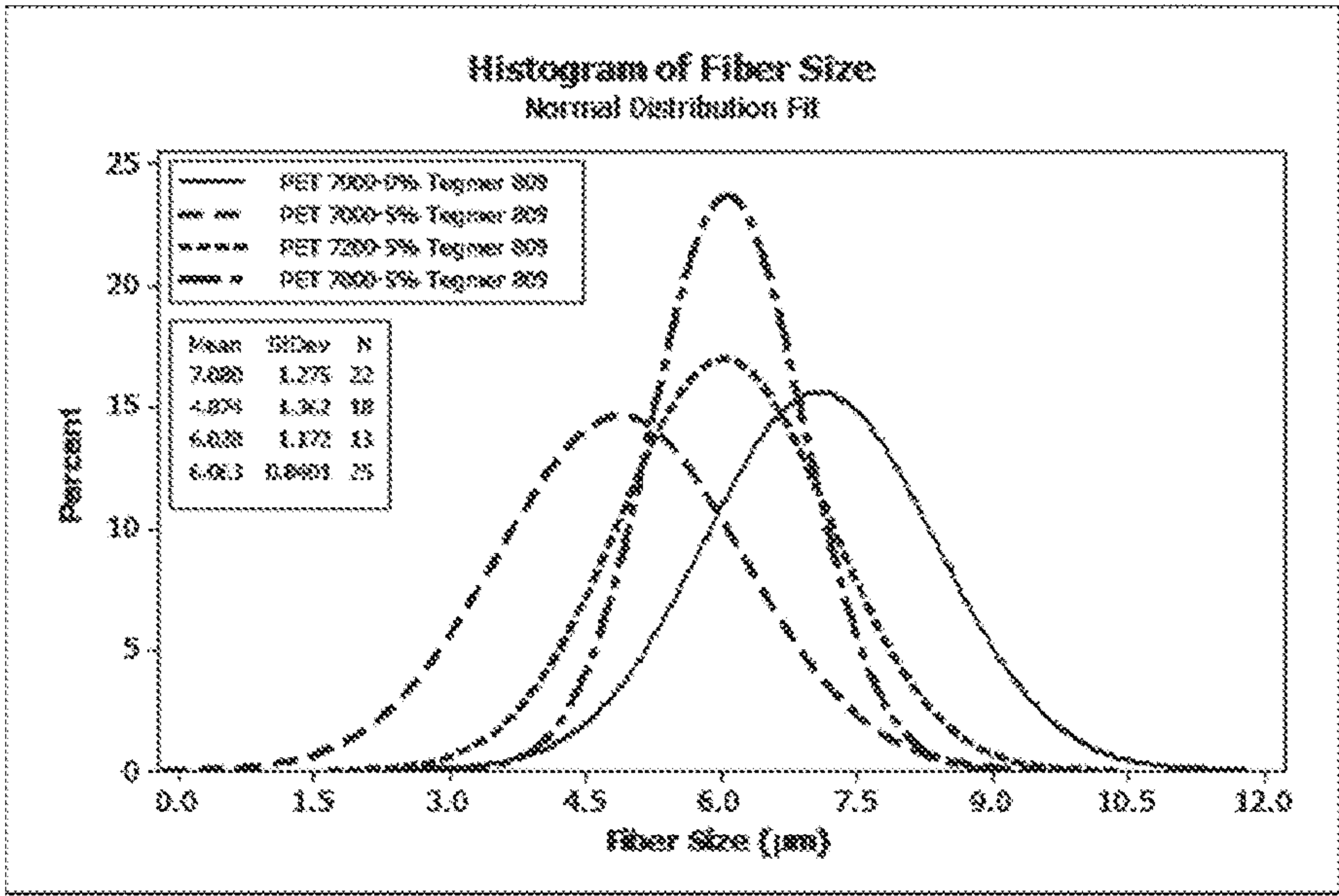
Fig. 6. Fittings (based on normal distribution) of the fiber size distributions of polymer fiber sheets prepared with PET resins having different intrinsic viscosity values, utilizing a TegMeR® 809 fiber modifying agent.
