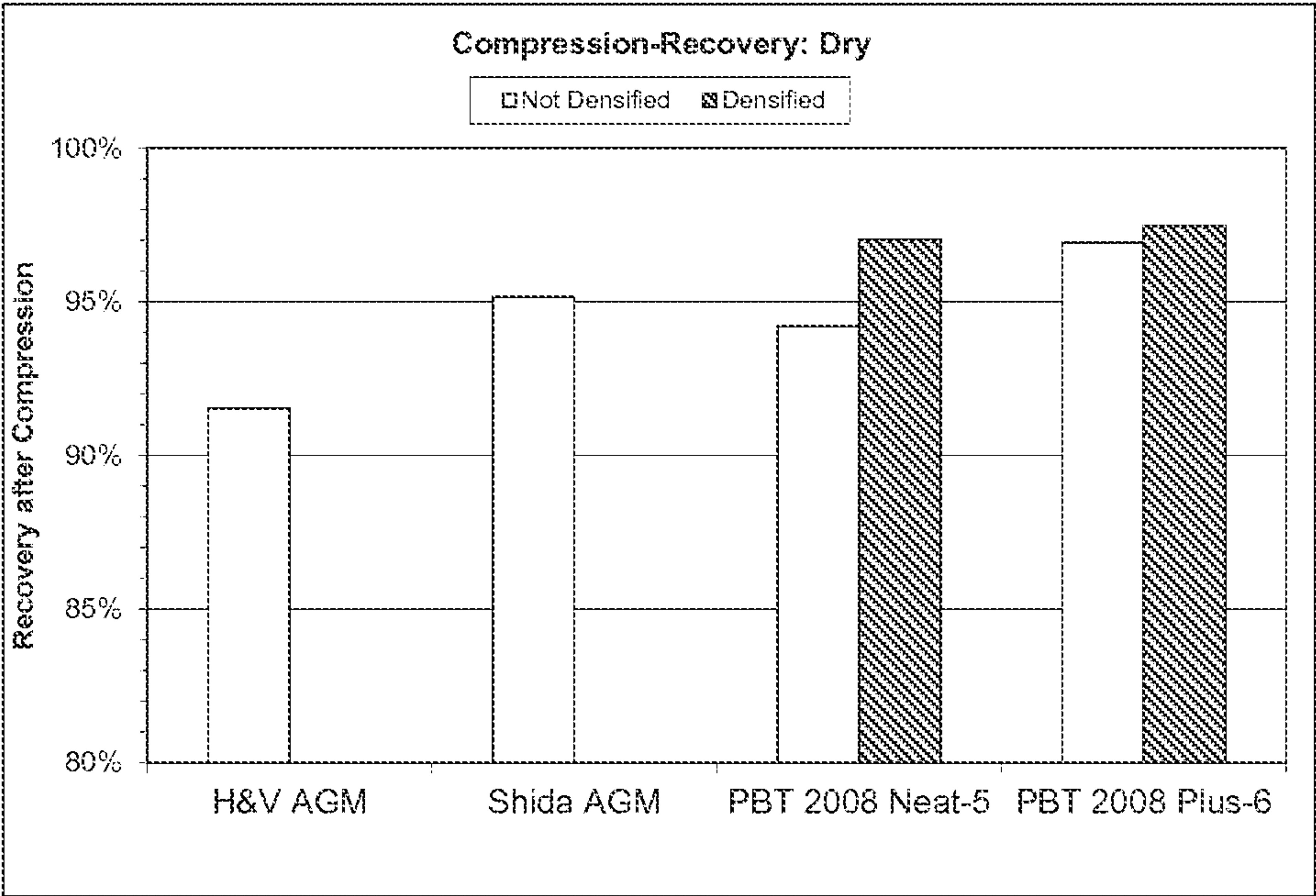
Fig. 3. Recovery after compression results for PBT fiber sheets as compared to those of AGM. The sample designated with “Plus” contains a surface modifying agent.
