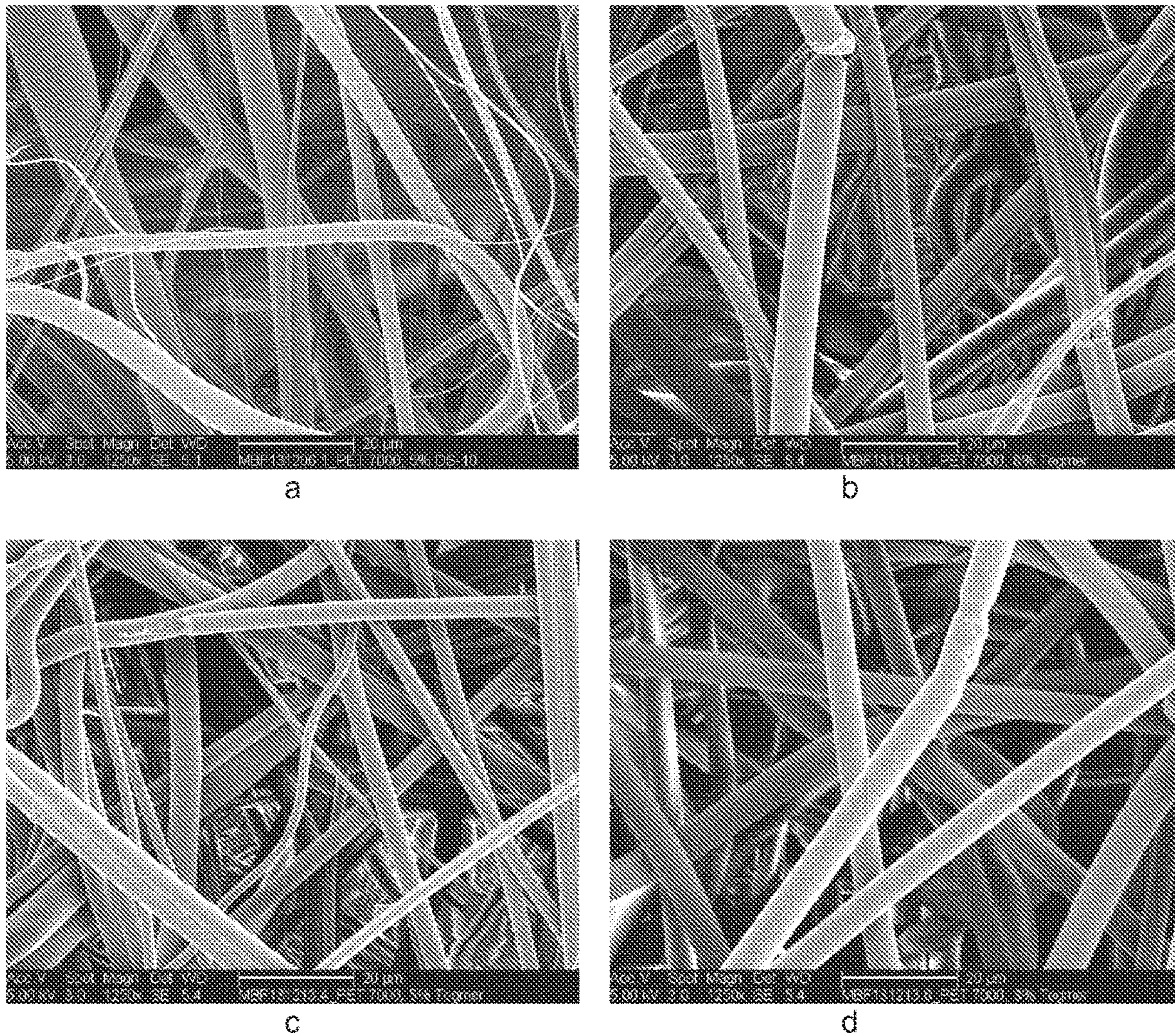
Fig. 12. SEM images of PET fiber sheets made with (a) 5 wt.% DS-10, (b) 8 wt.% TegMeR® 809, (c) 5 wt.% TegMeR® 809, and (d) 3 wt.% TegMeR® 809.
