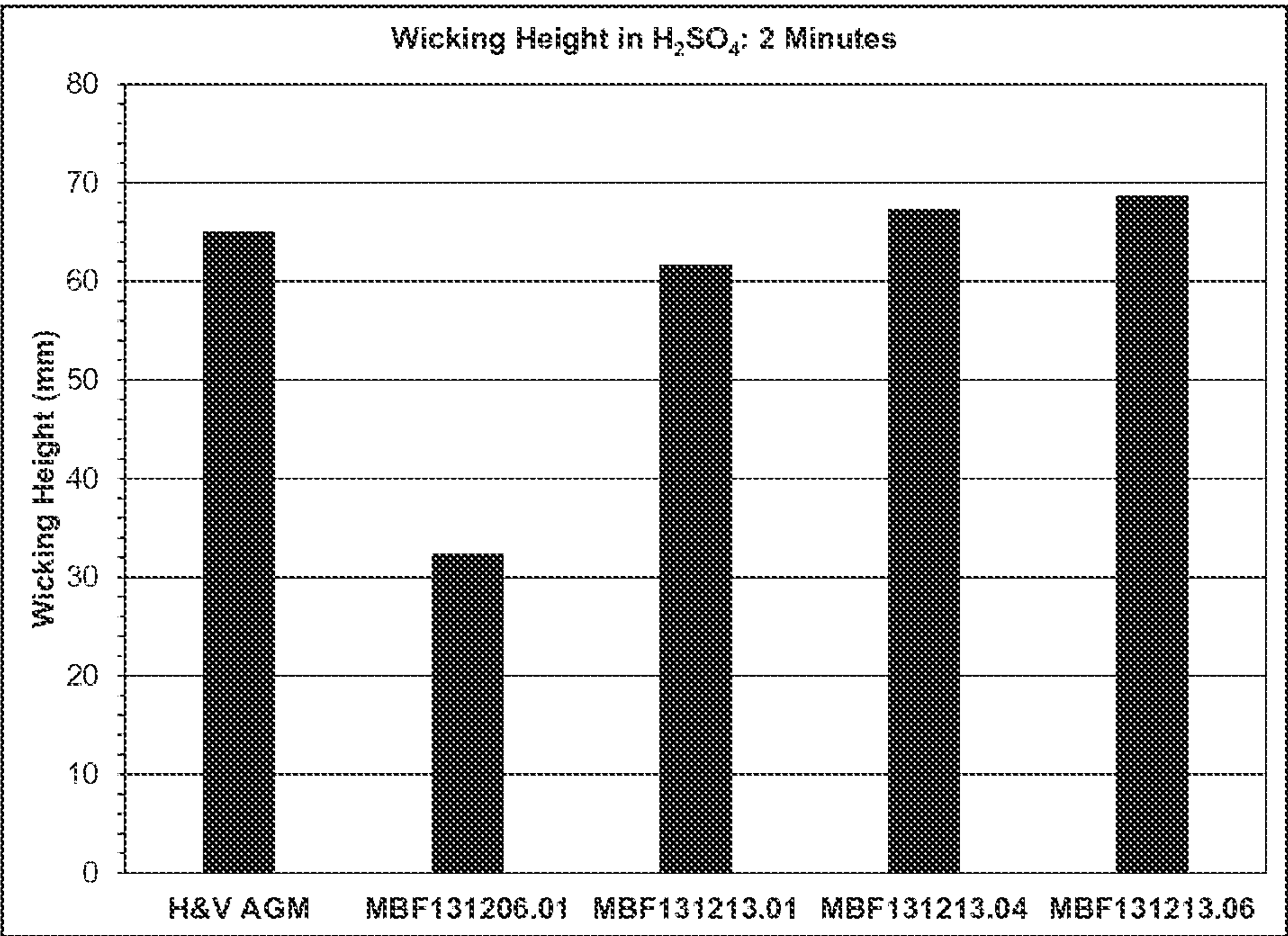
Fig. 14. Two-minute wicking height of PET fiber sheets in sulfuric acid.
