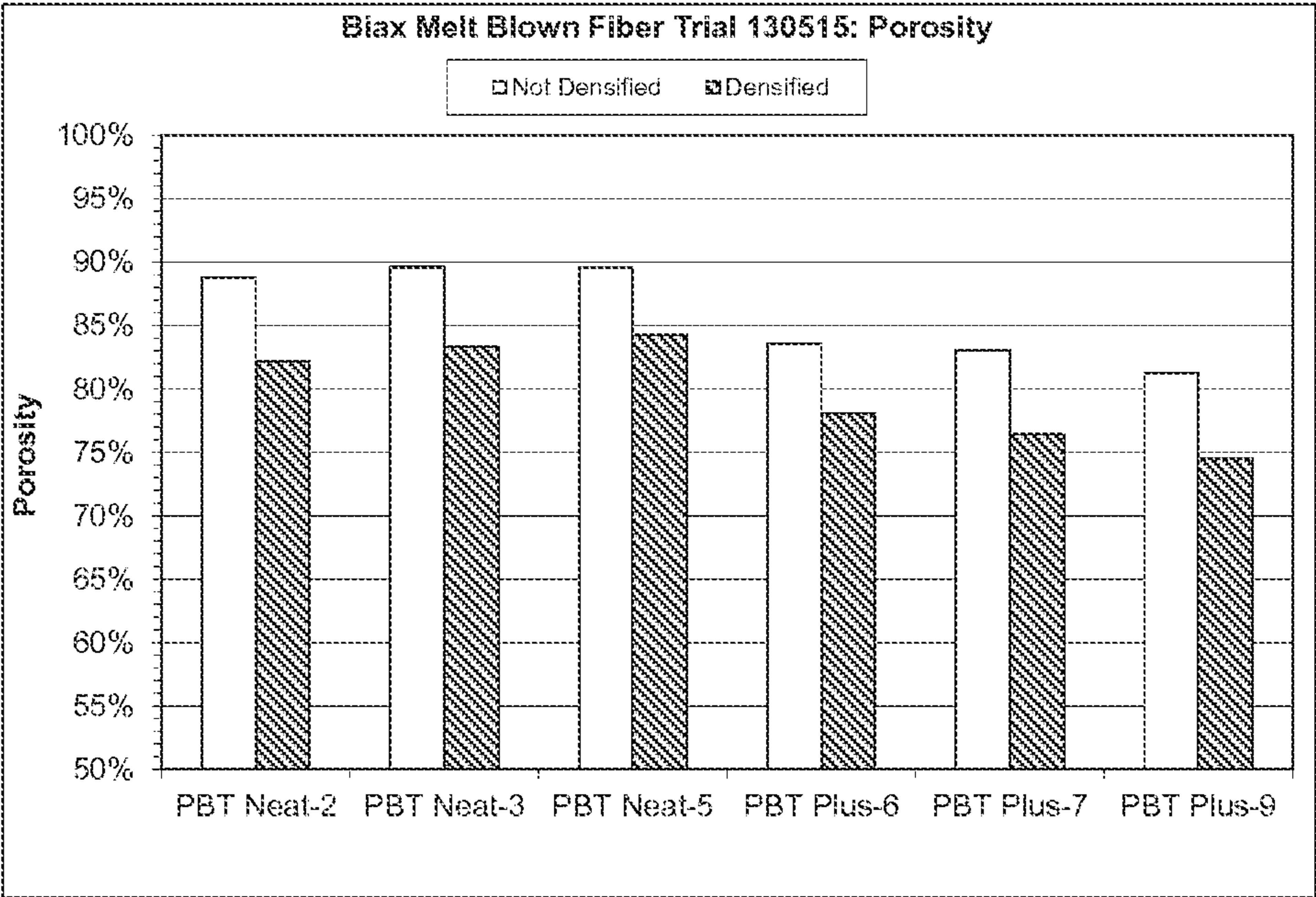
Fig. 2. Porosity of PBT fiber sheets before and after densification. The samples designated with “Plus” contain a surface modifying agent.
