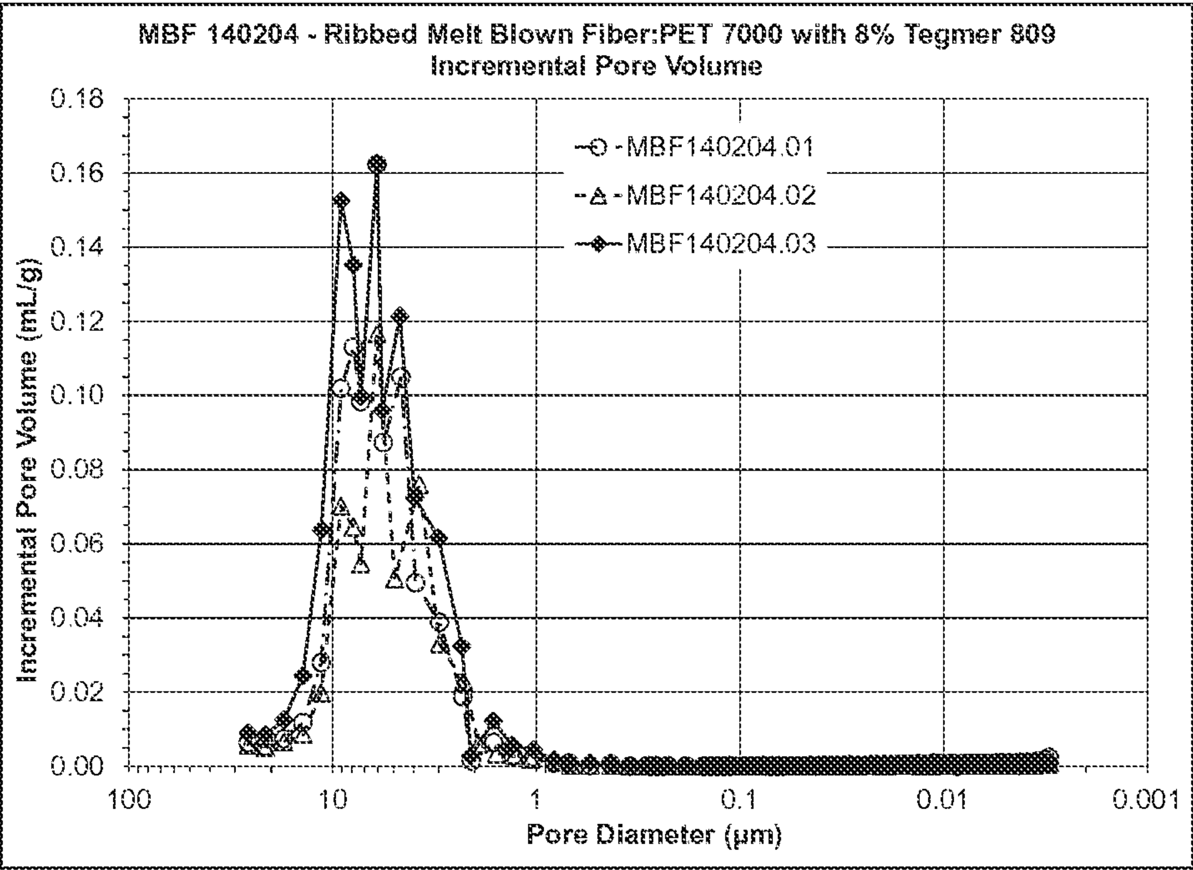
Fig. 20. Pore size distributions by mercury intrusion porosimetry of the ribbed PET fiber sheets.
