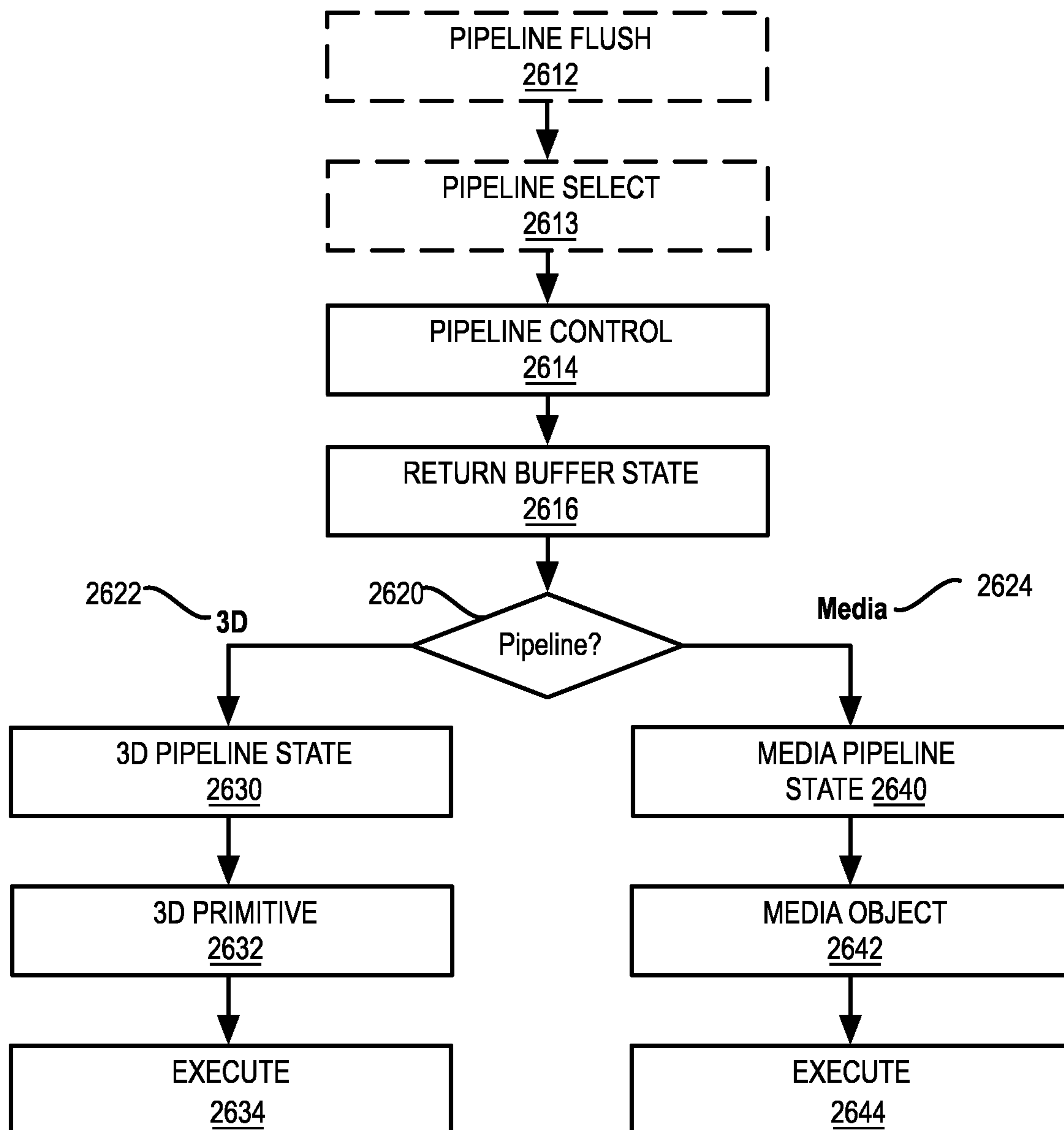
GRAPHICS PROCESSOR COMMAND SEQUENCE 2610
