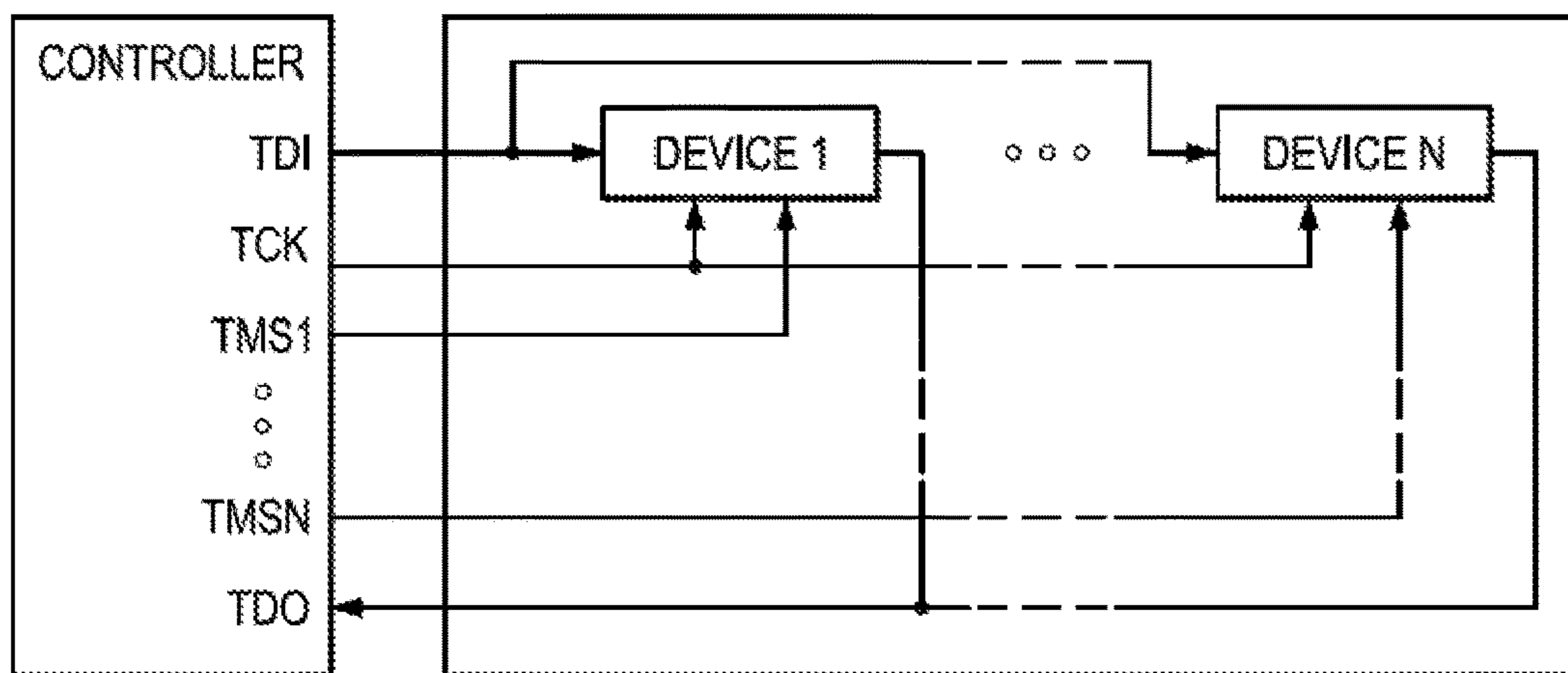
FIG. 5 (PRIOR ART)
