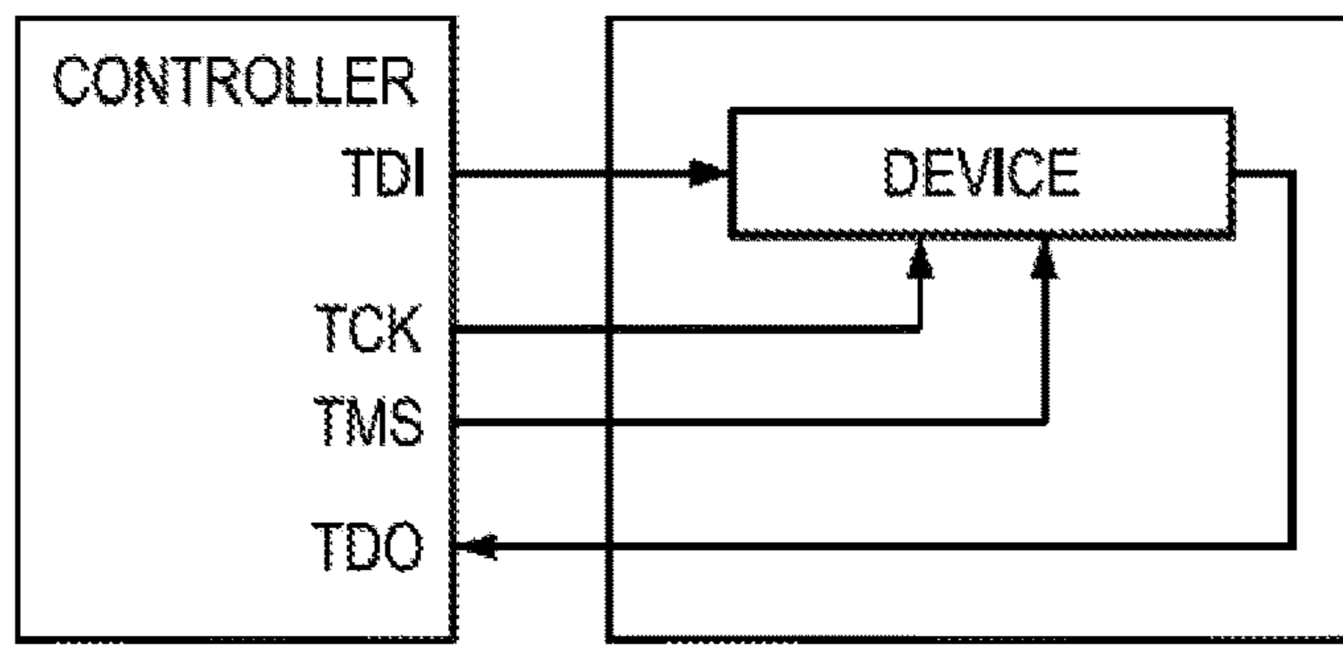
FIG. 4 (PRIOR ART)
