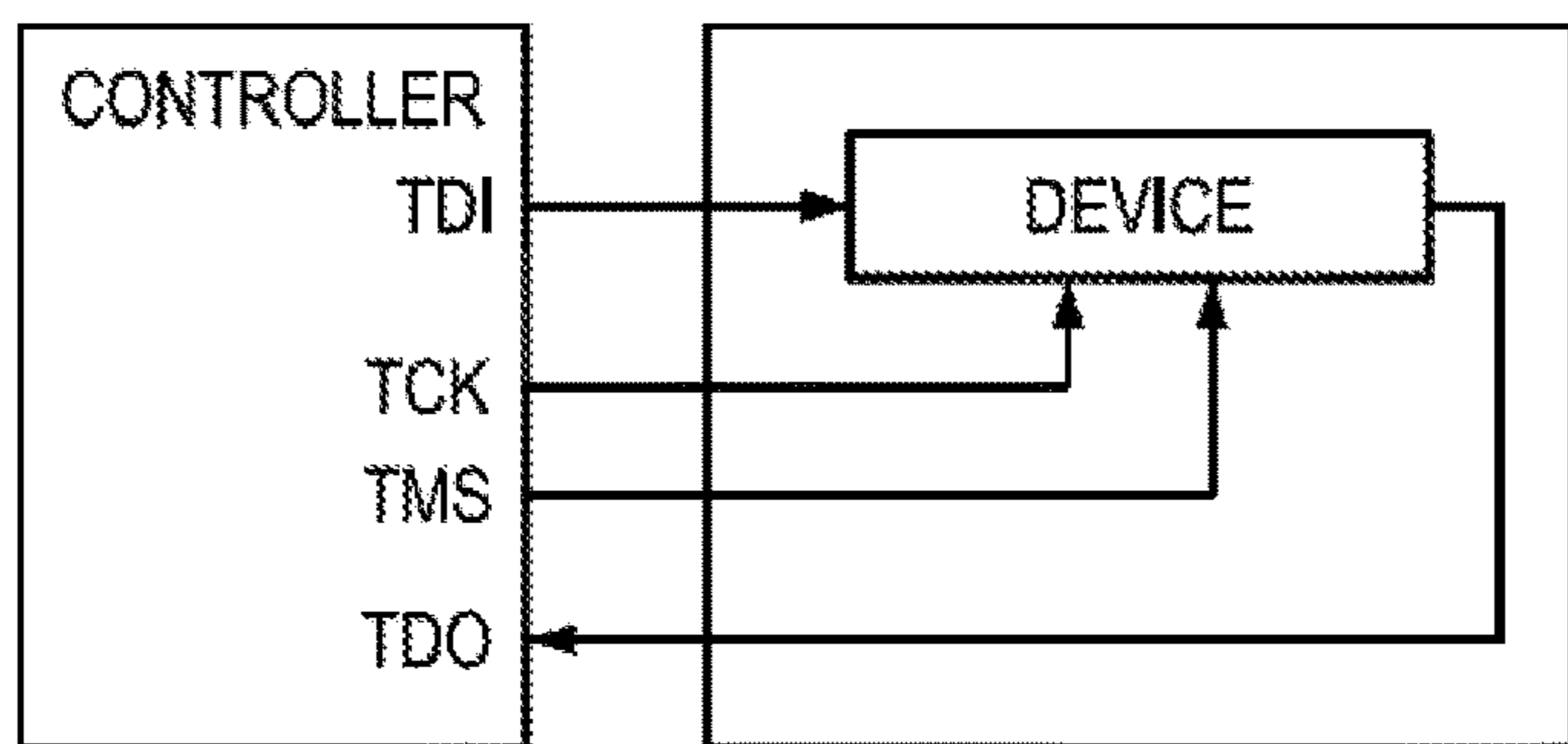
FIG. 4 (PRIOR ART)
