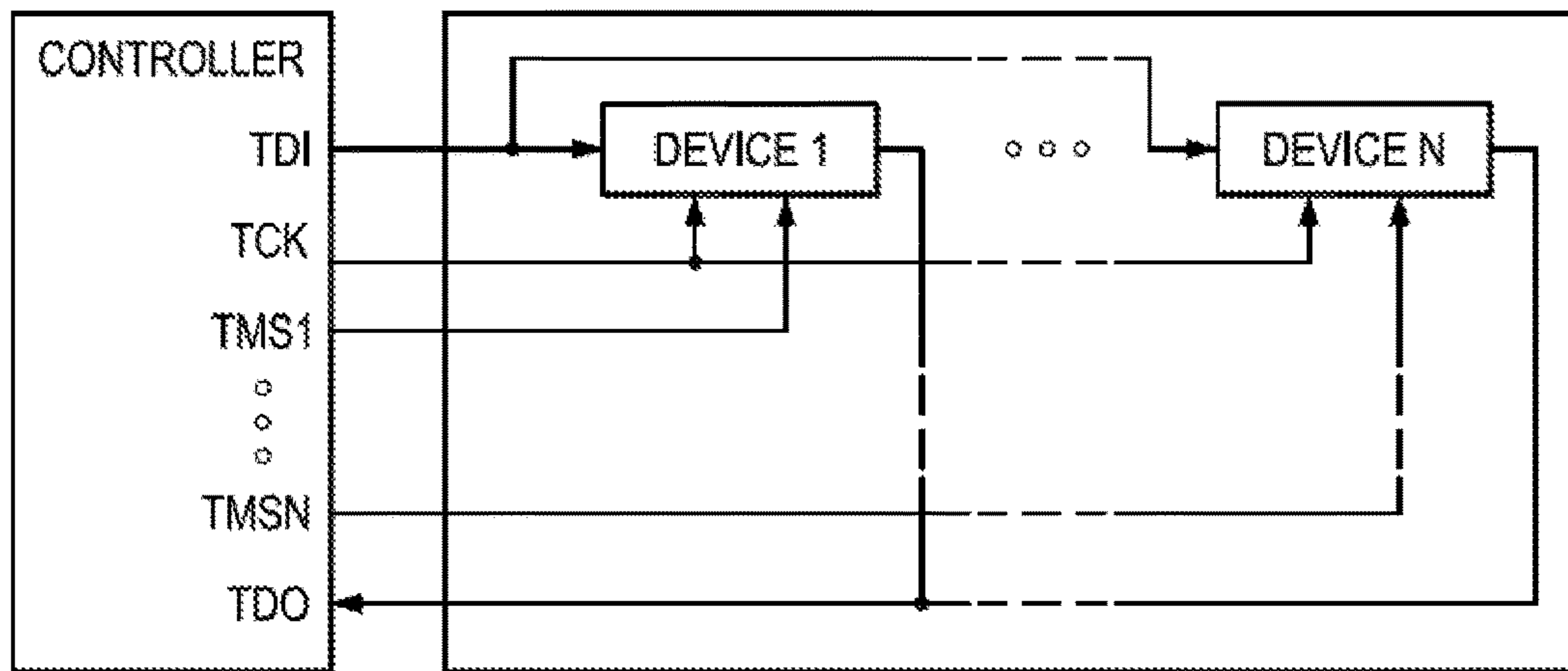
FIG. 5 (PRIOR ART)
