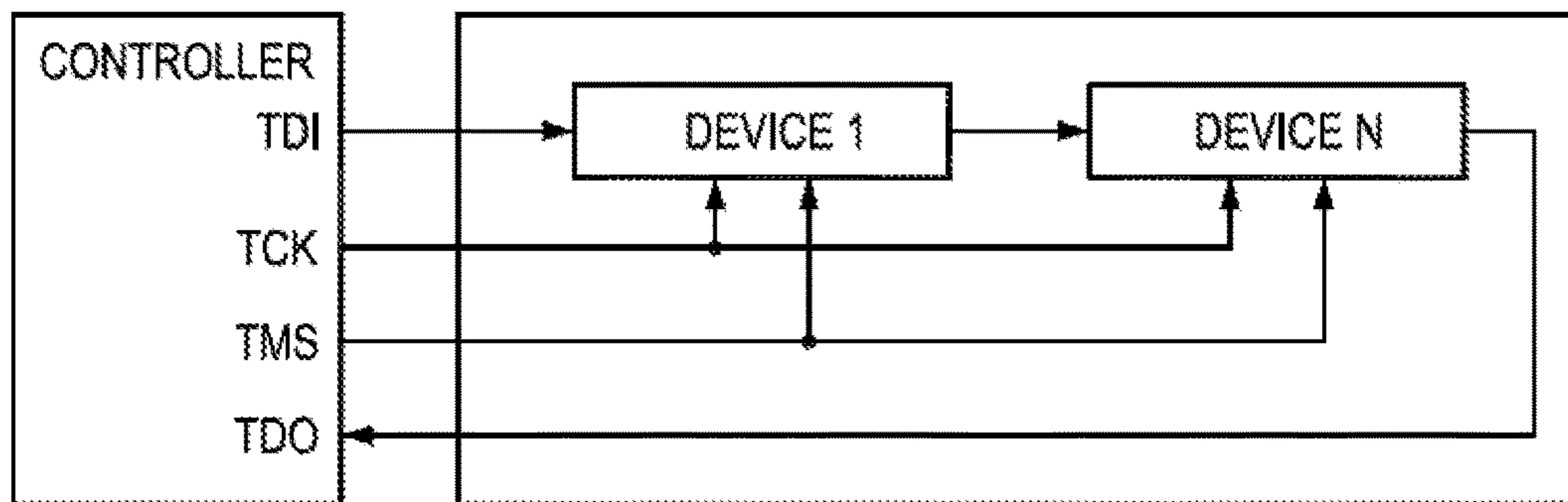
FIG. 6 (PRIOR ART)
