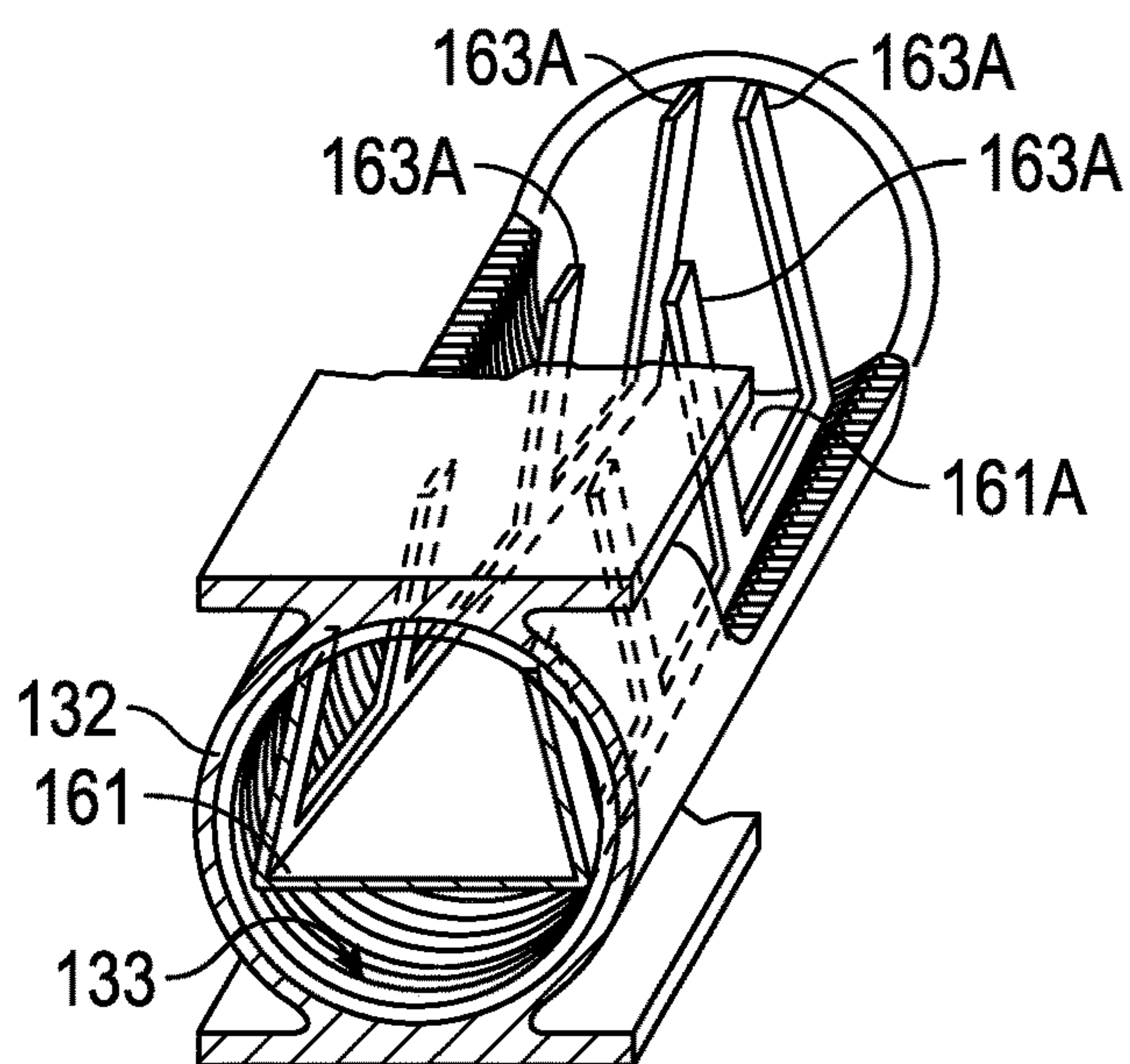
FIG. 6D (Section D-D)
