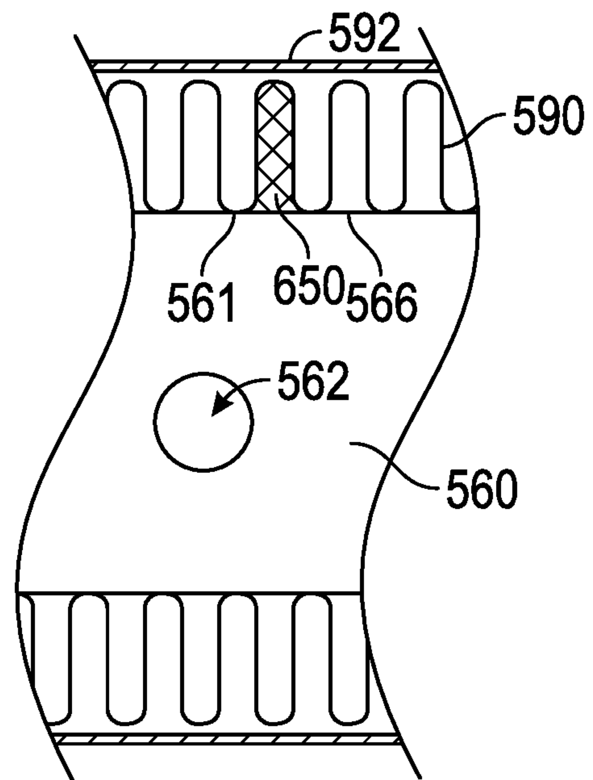
FIG. 12C (Section H-H)
