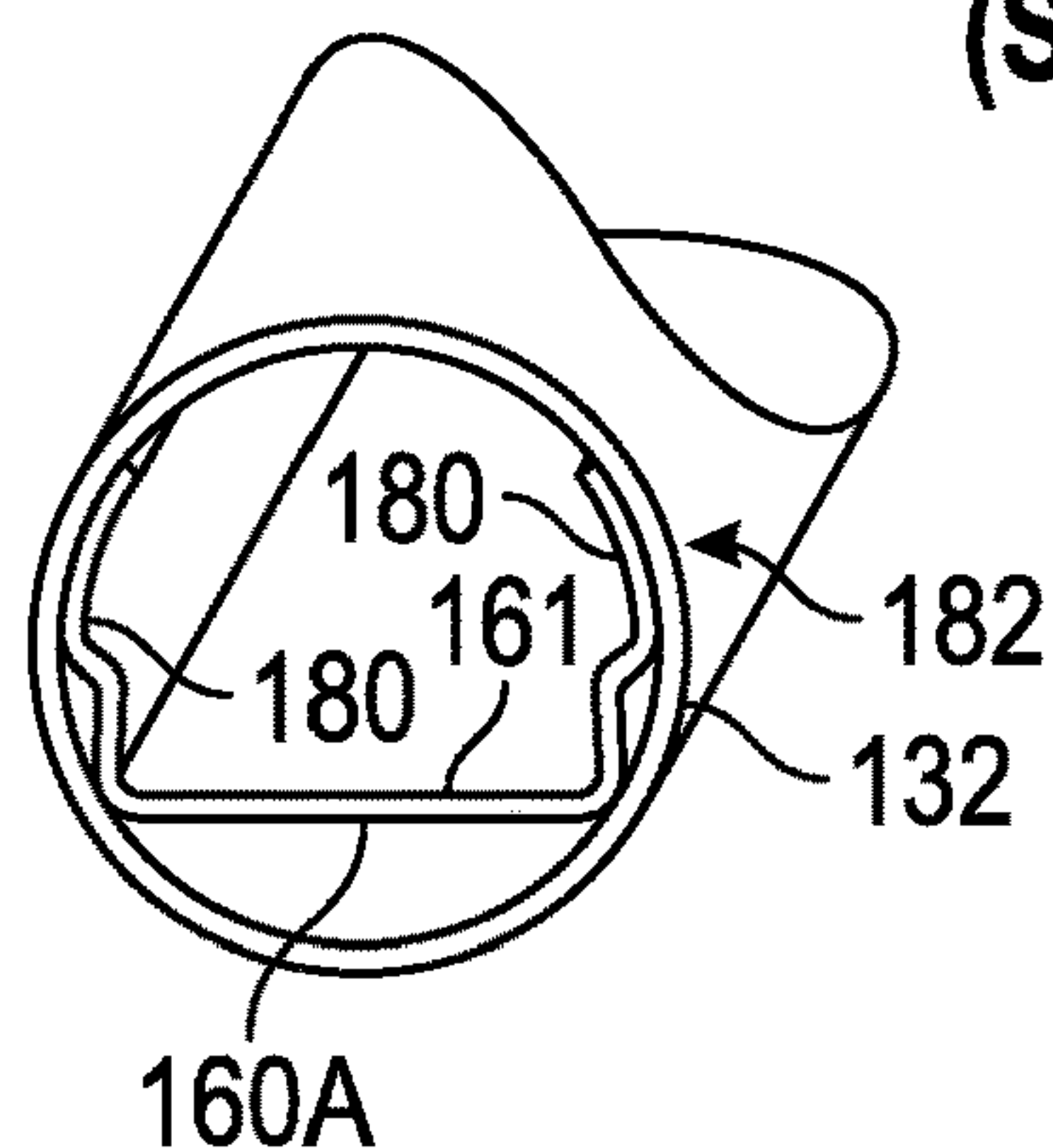
FIG. 6C (Section C-C)
