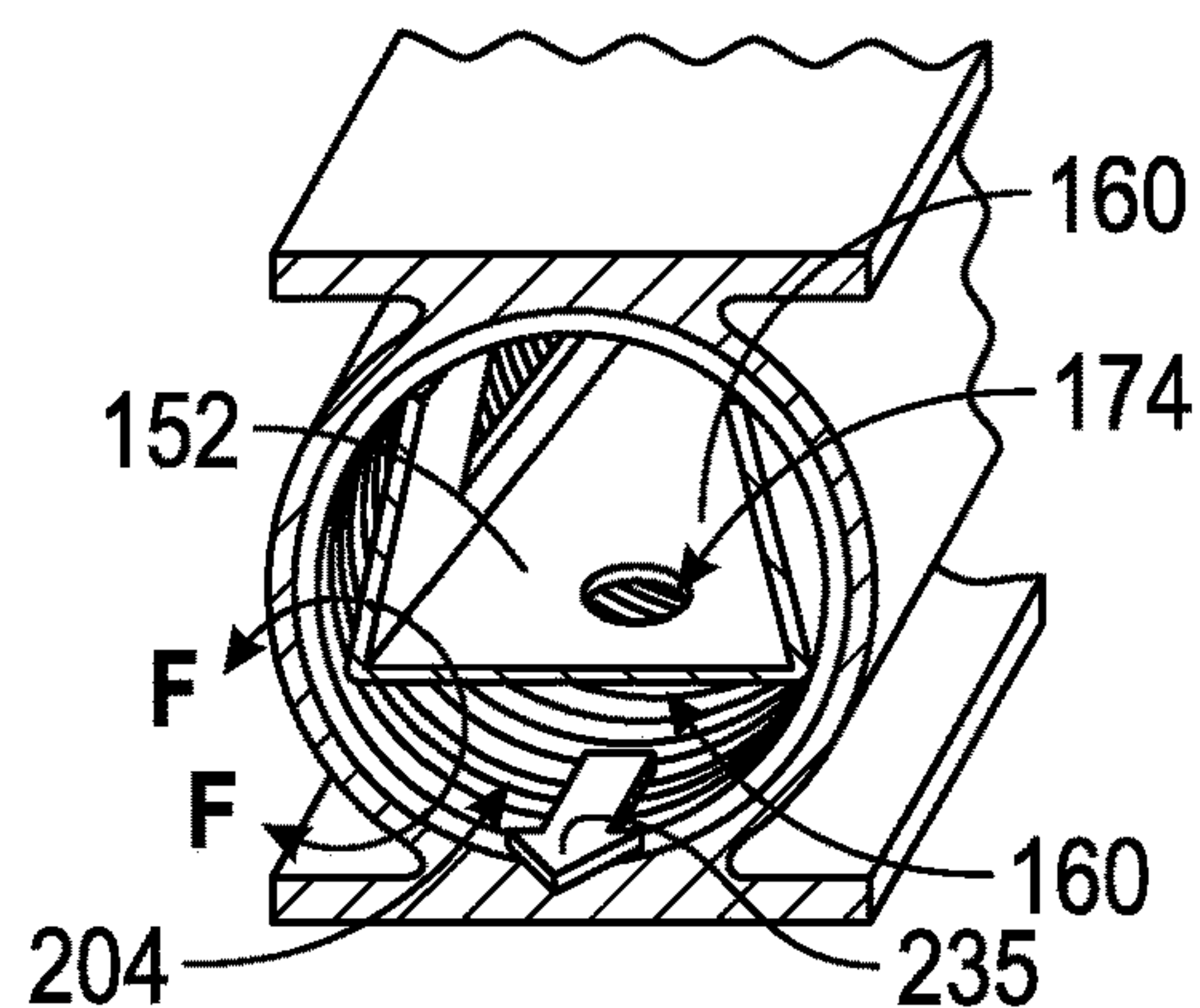
FIG. 6B (Section B-B)
