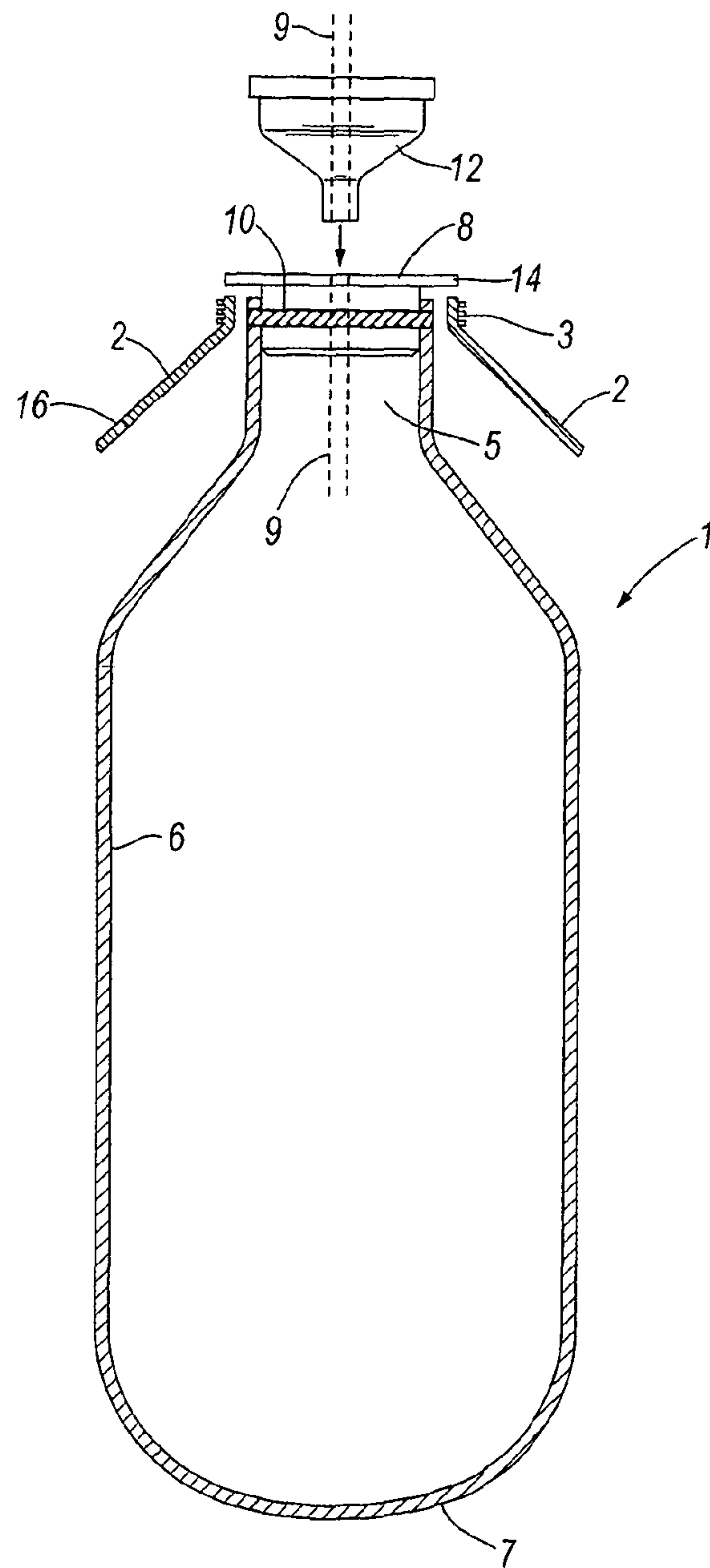
Fig. 1 PRIOR ART
