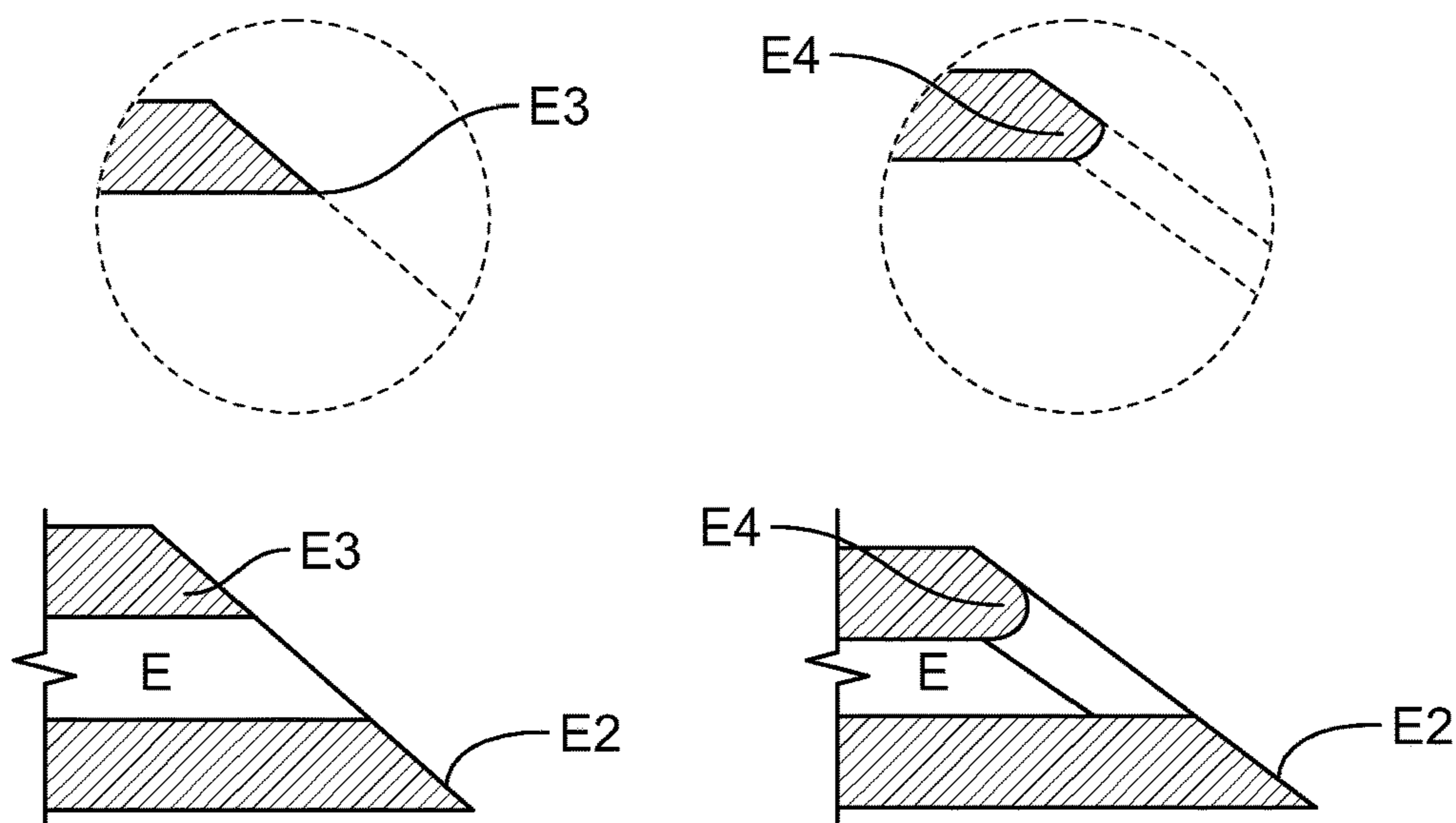
FIGURE 19 (Prior Art)
