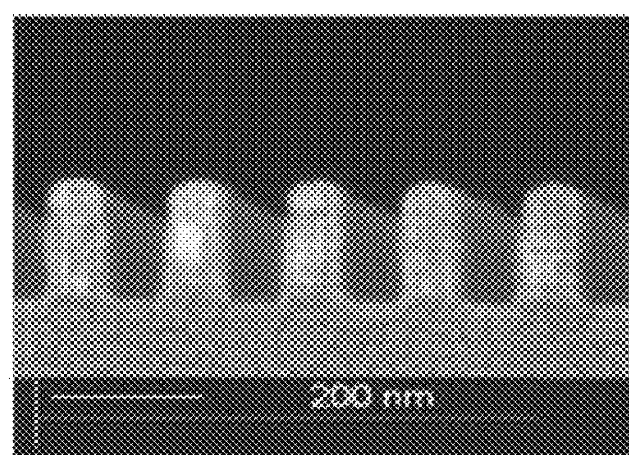
SEM Image of a side view of aluminum nanowire
