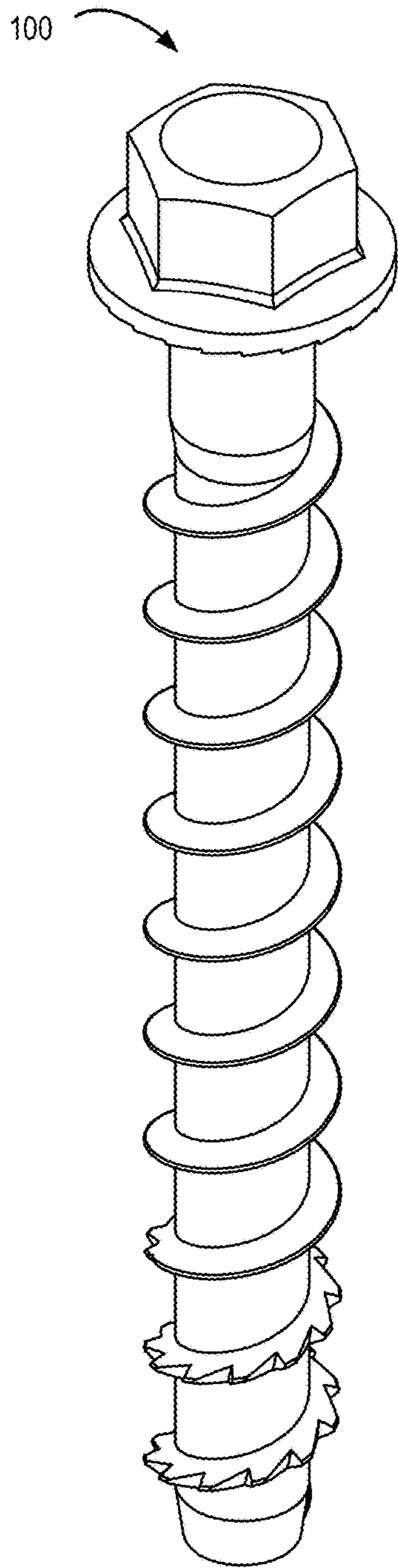
FIG. 1 (Prior Art)
