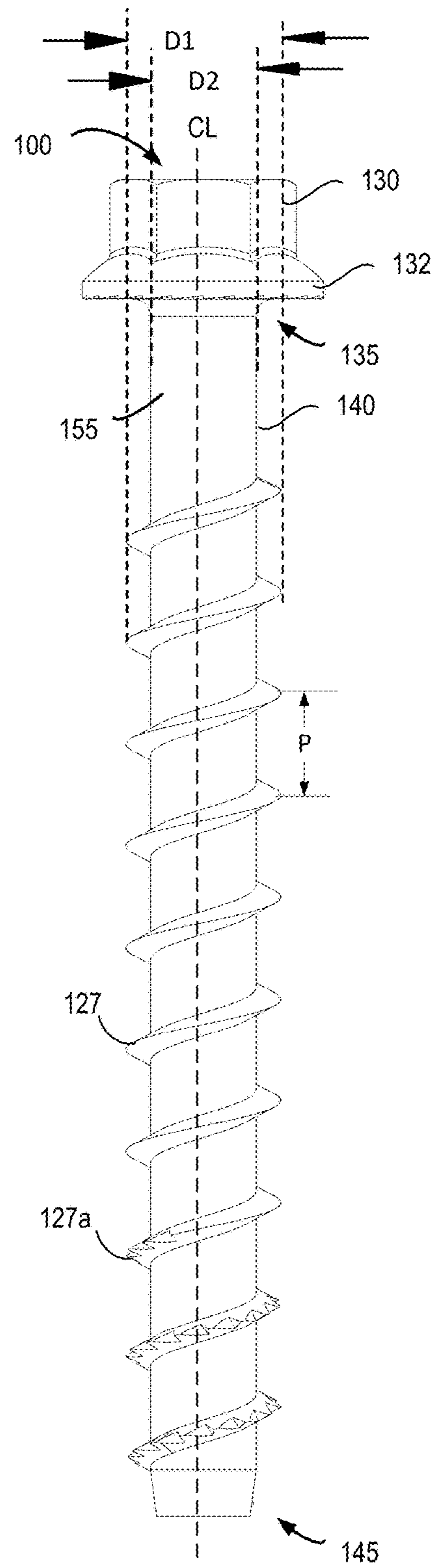
FIG. 2 (Prior Art)
