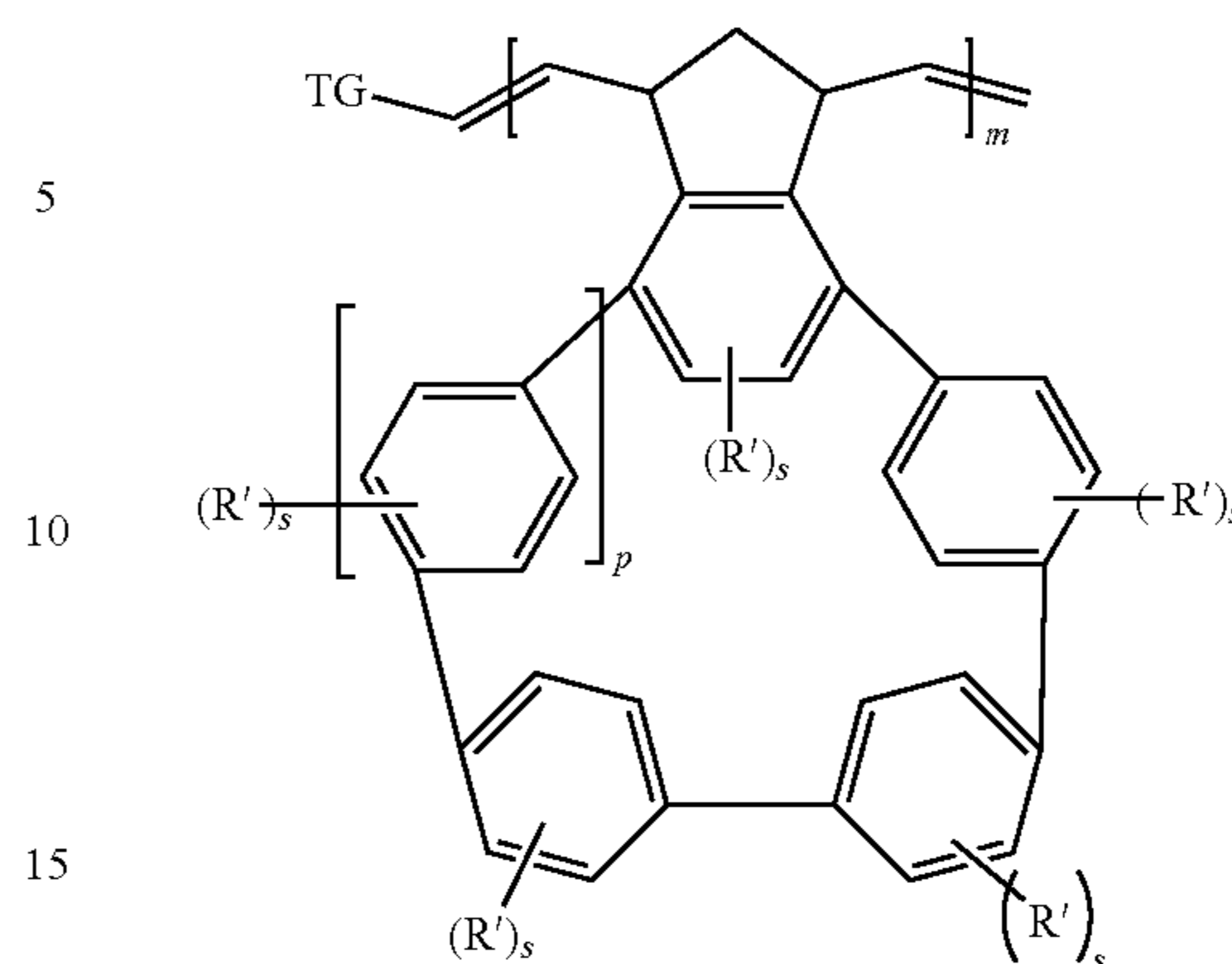
Formula II
