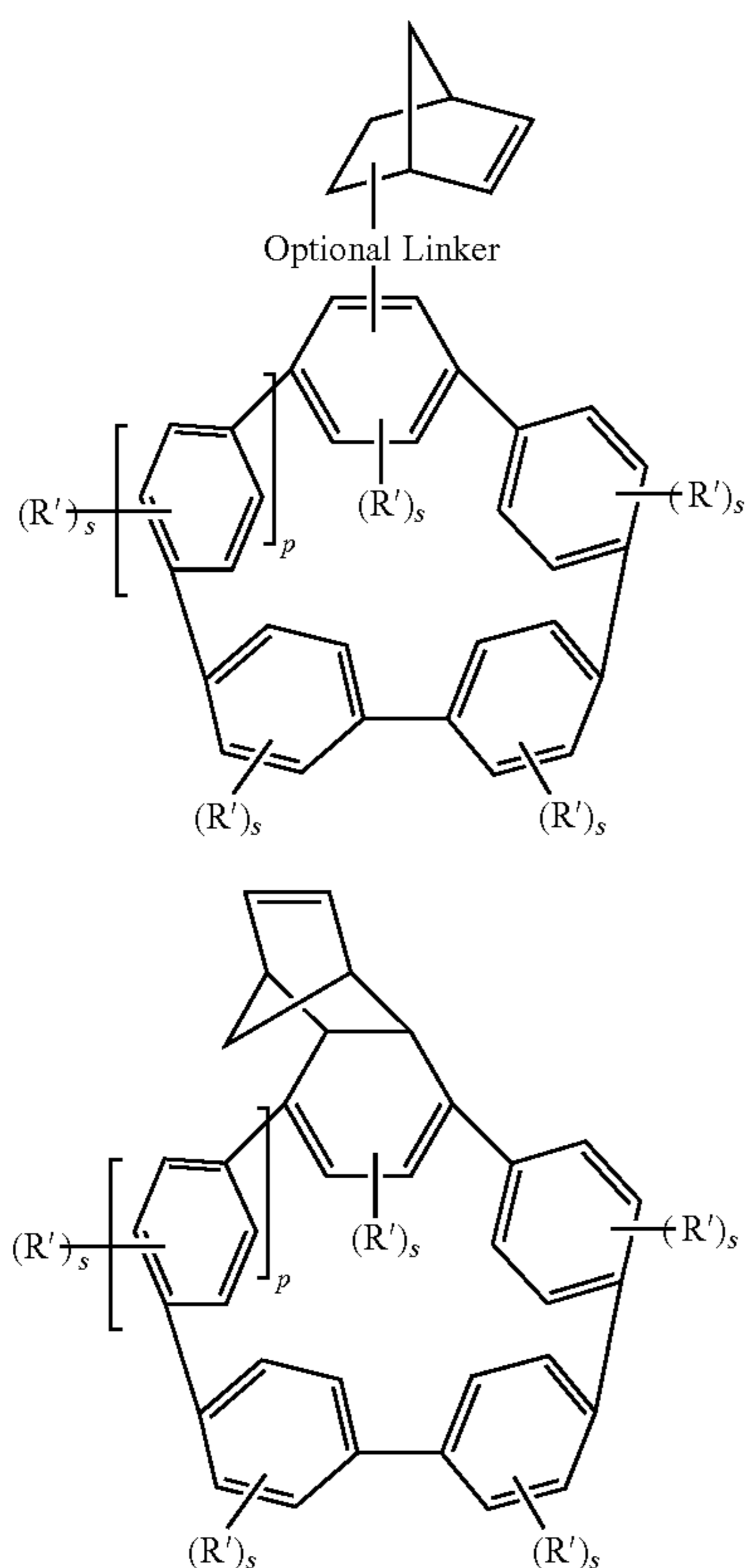
Formula VIII
