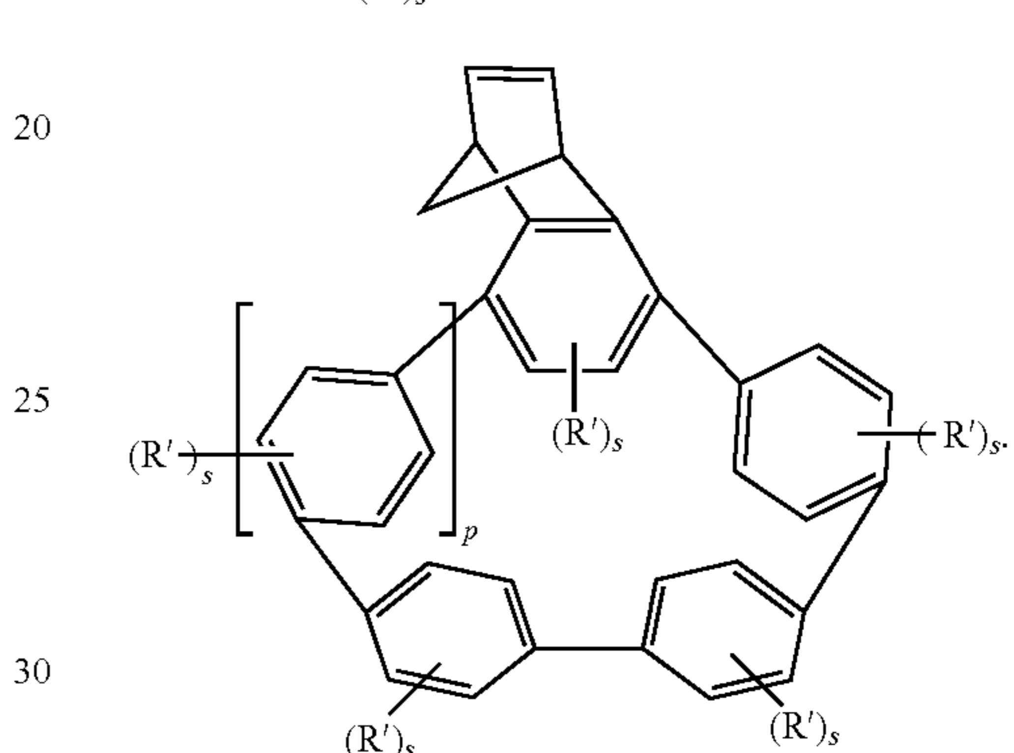
Formula VIII
