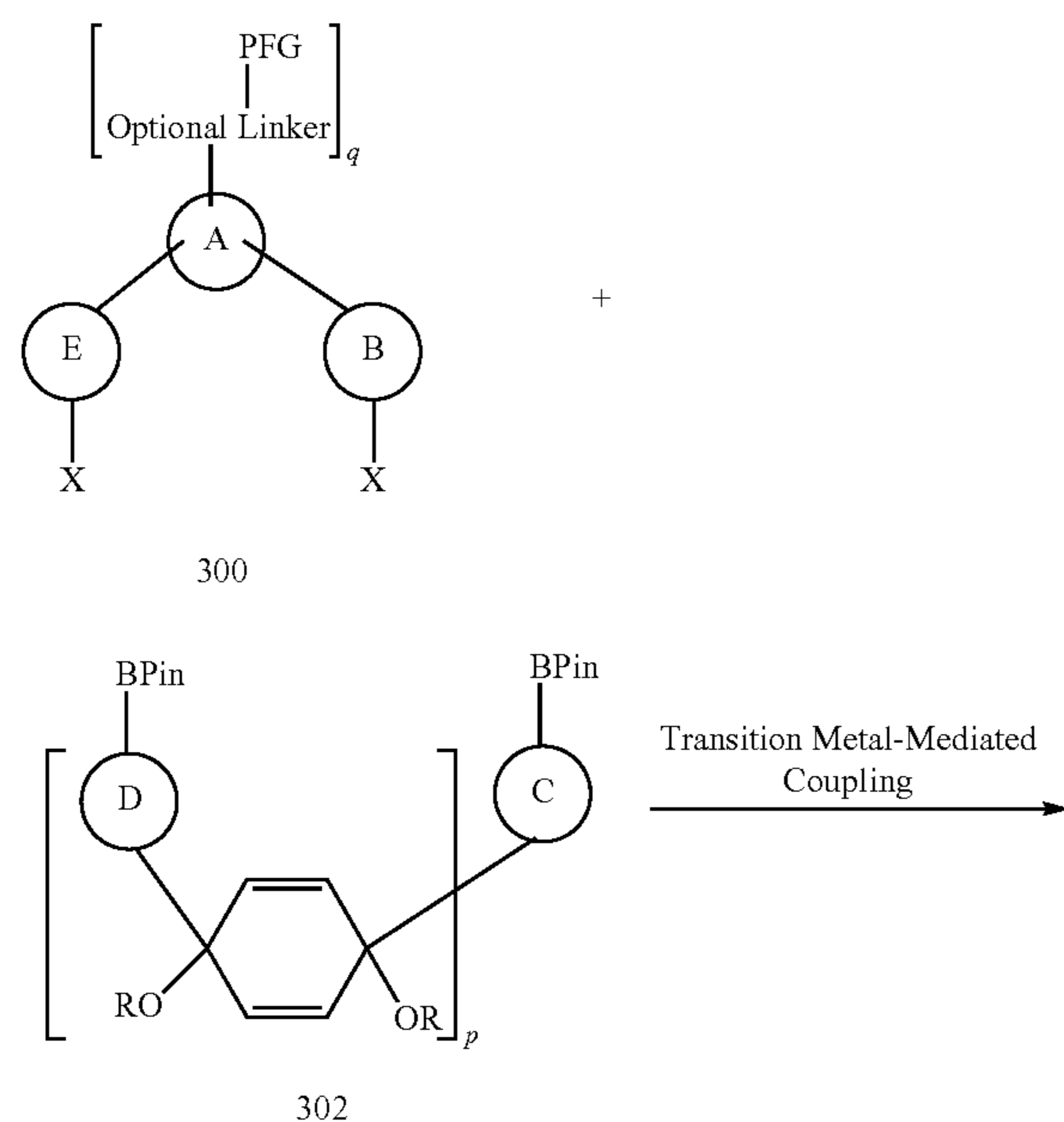
Scheme 3
