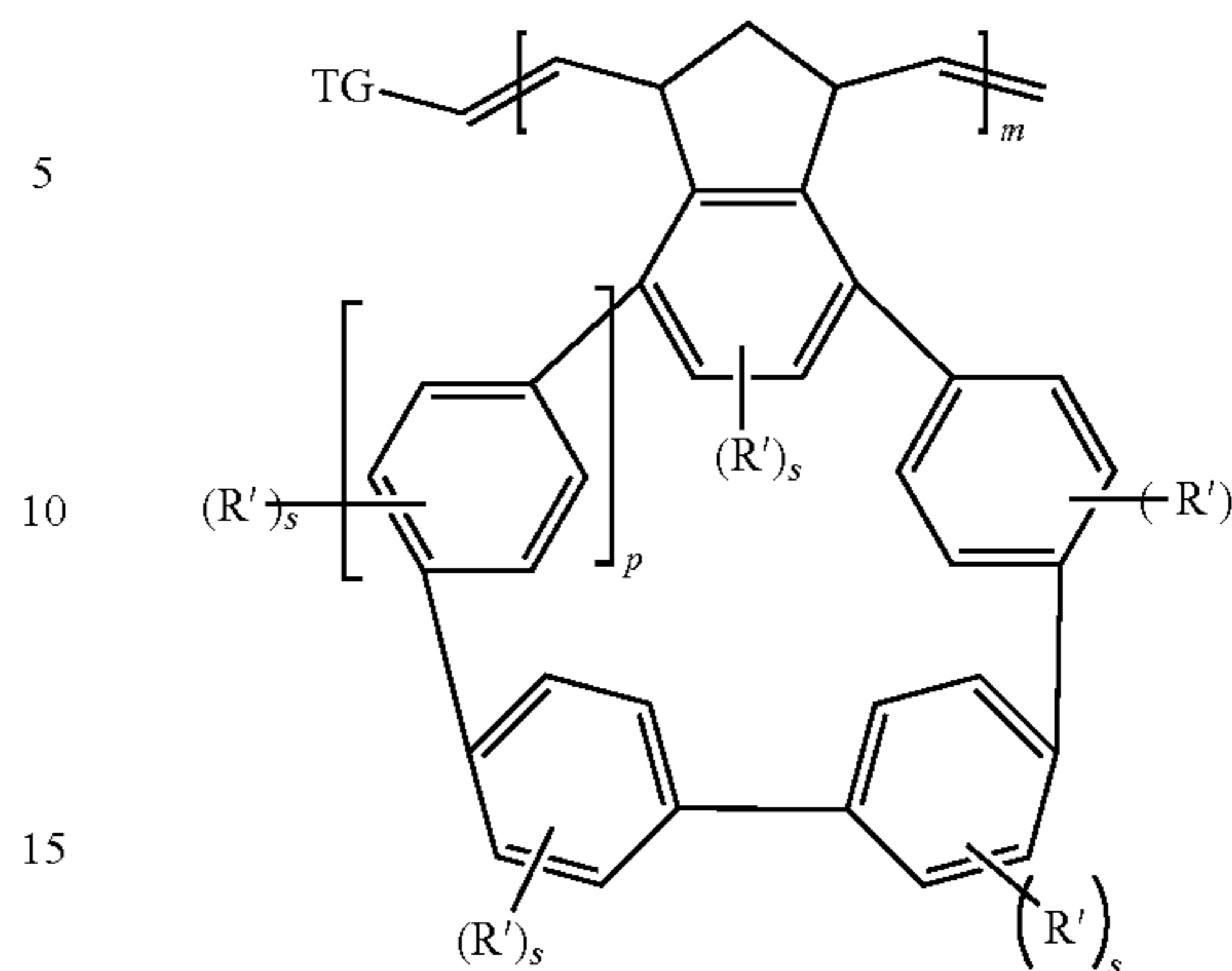
Formula II
