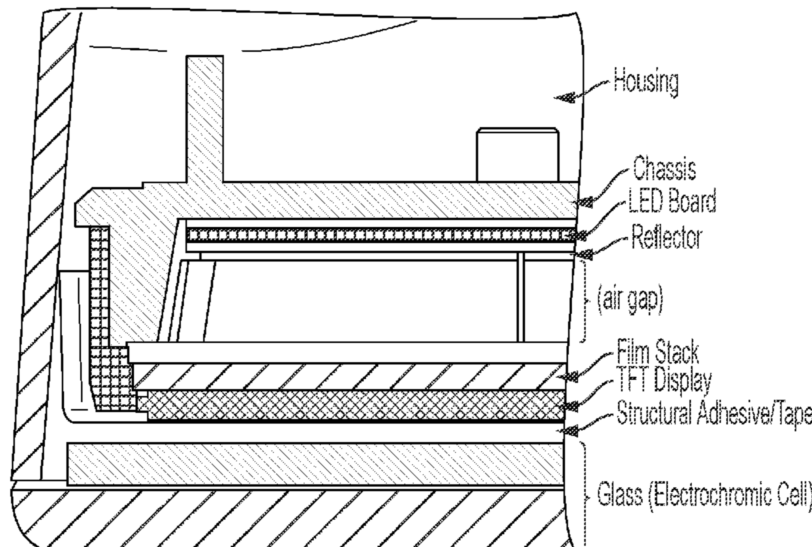
Backlight Stack Cross Section - Current
