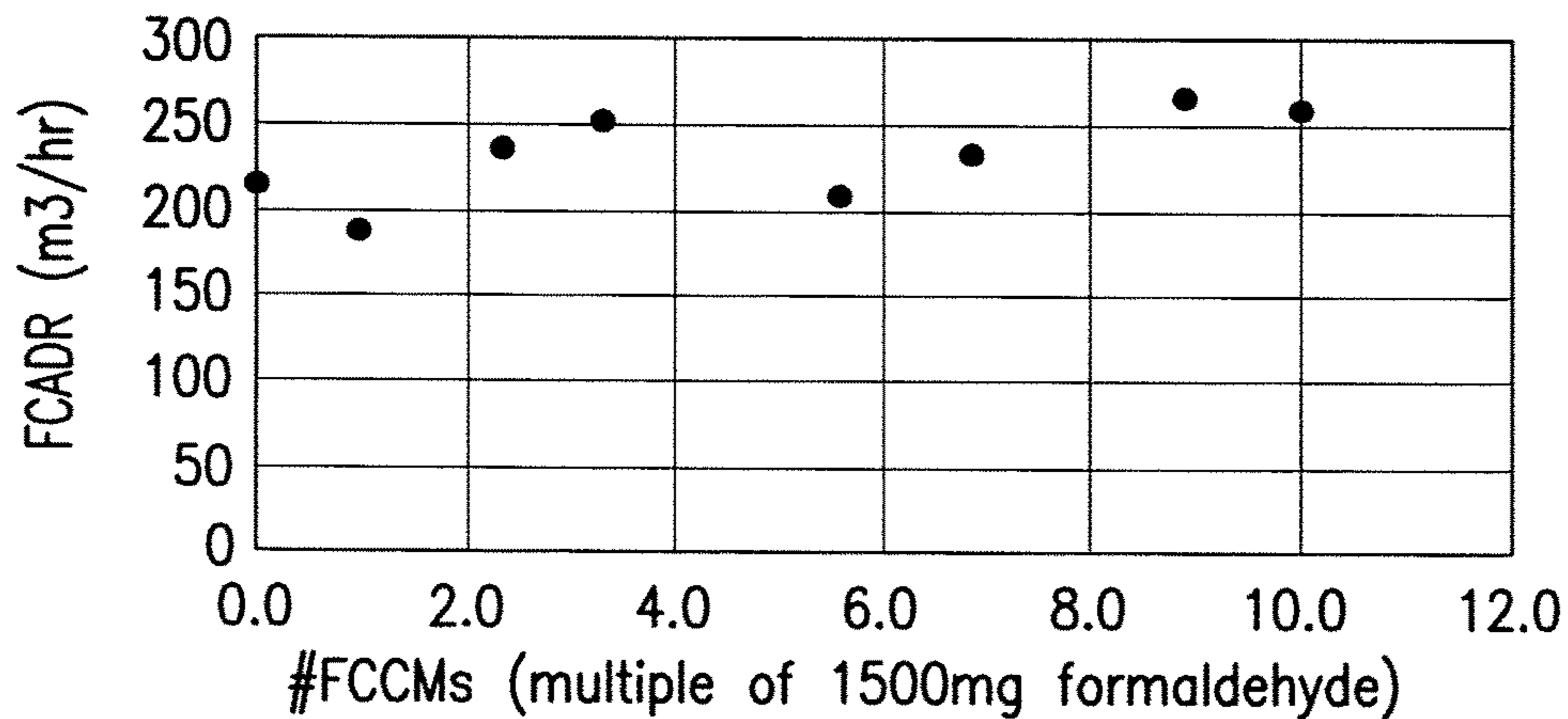
Formaldehyde CADR during FCCM test with Formaldehyde Catalyst (No Ozone During Testing)
