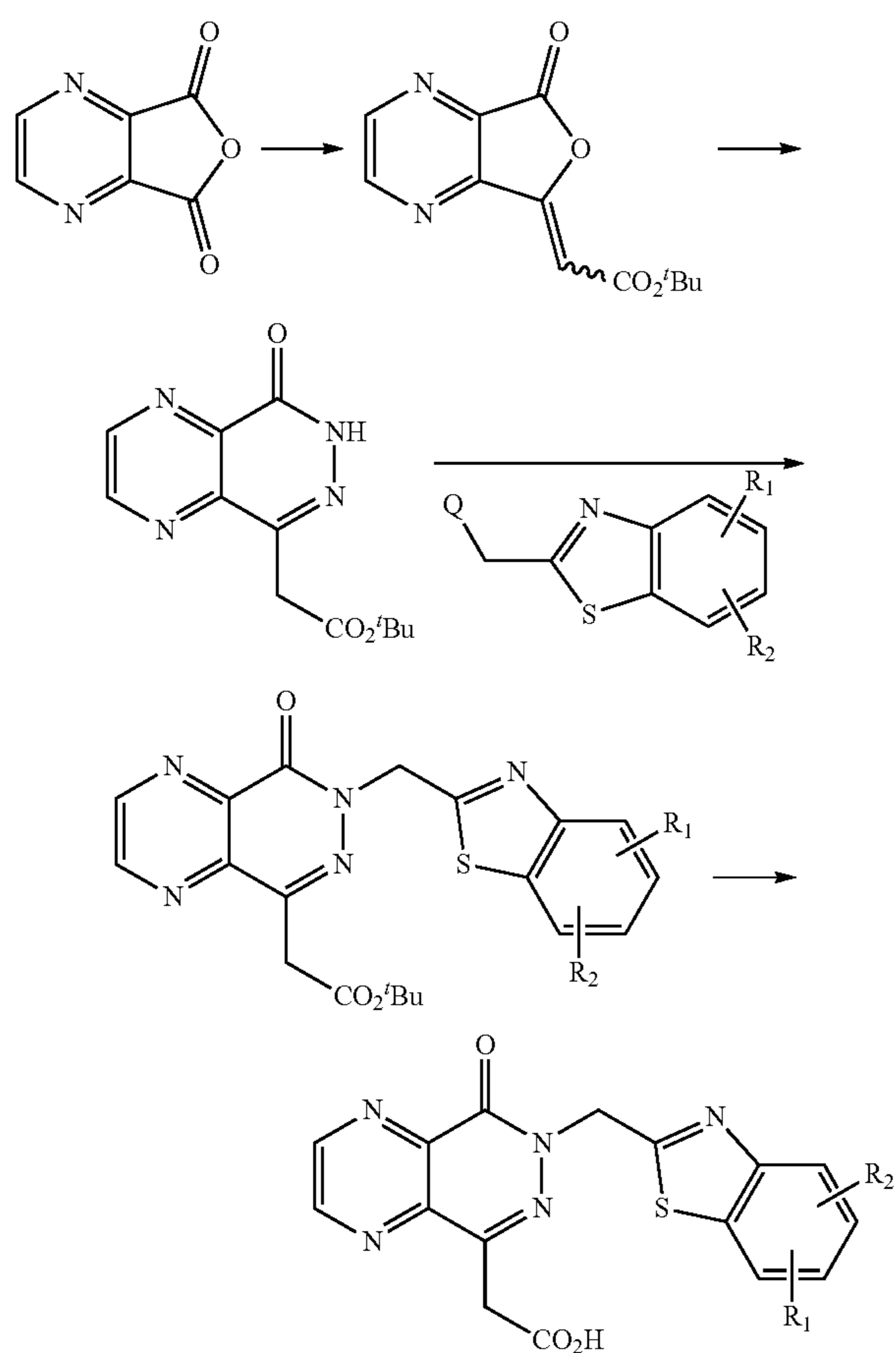
Scheme 17
