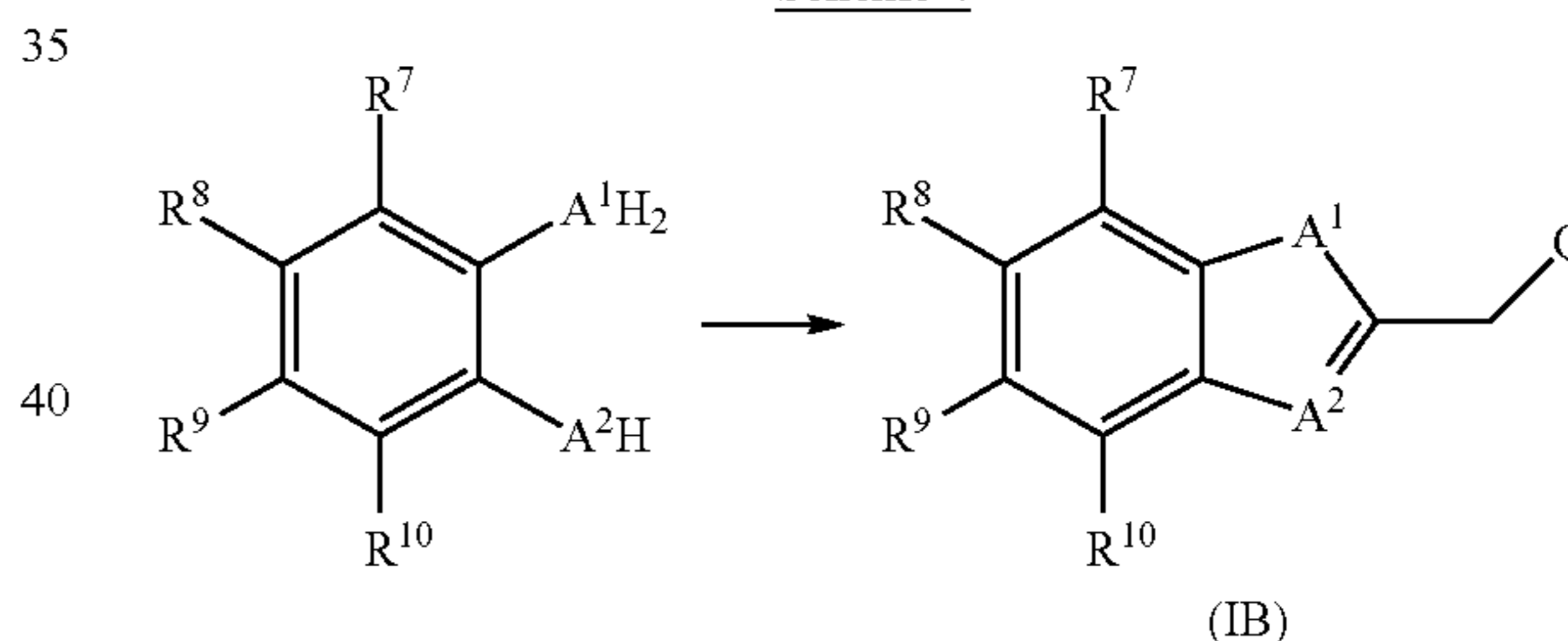
Scheme 4
