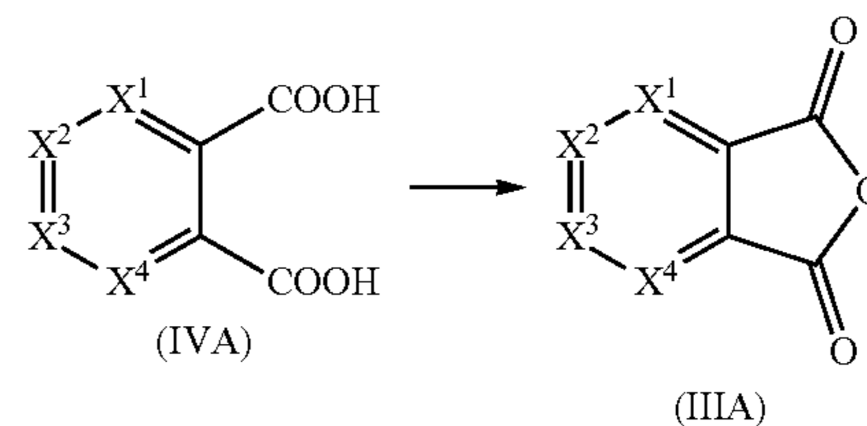
Scheme 8
