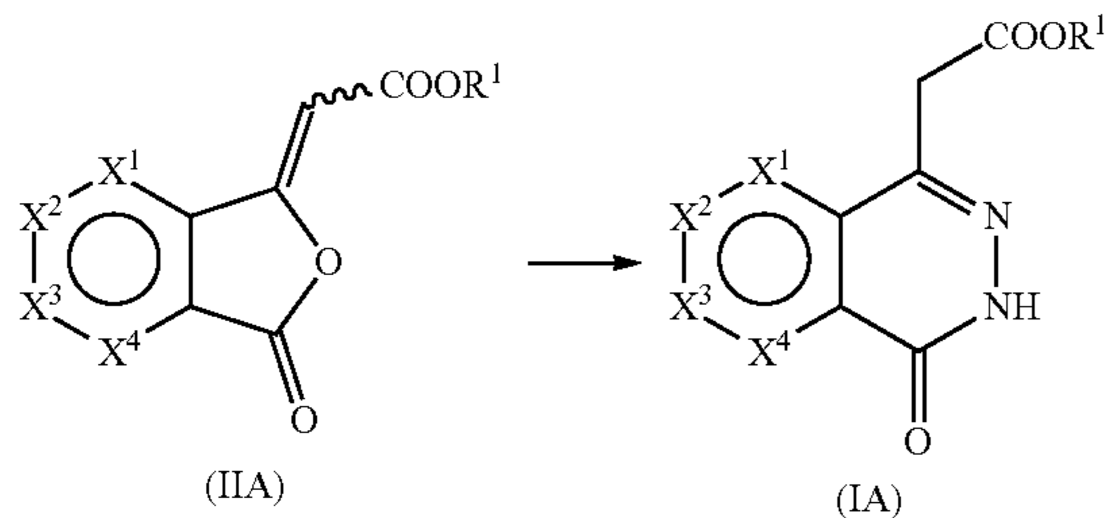
Scheme 5
