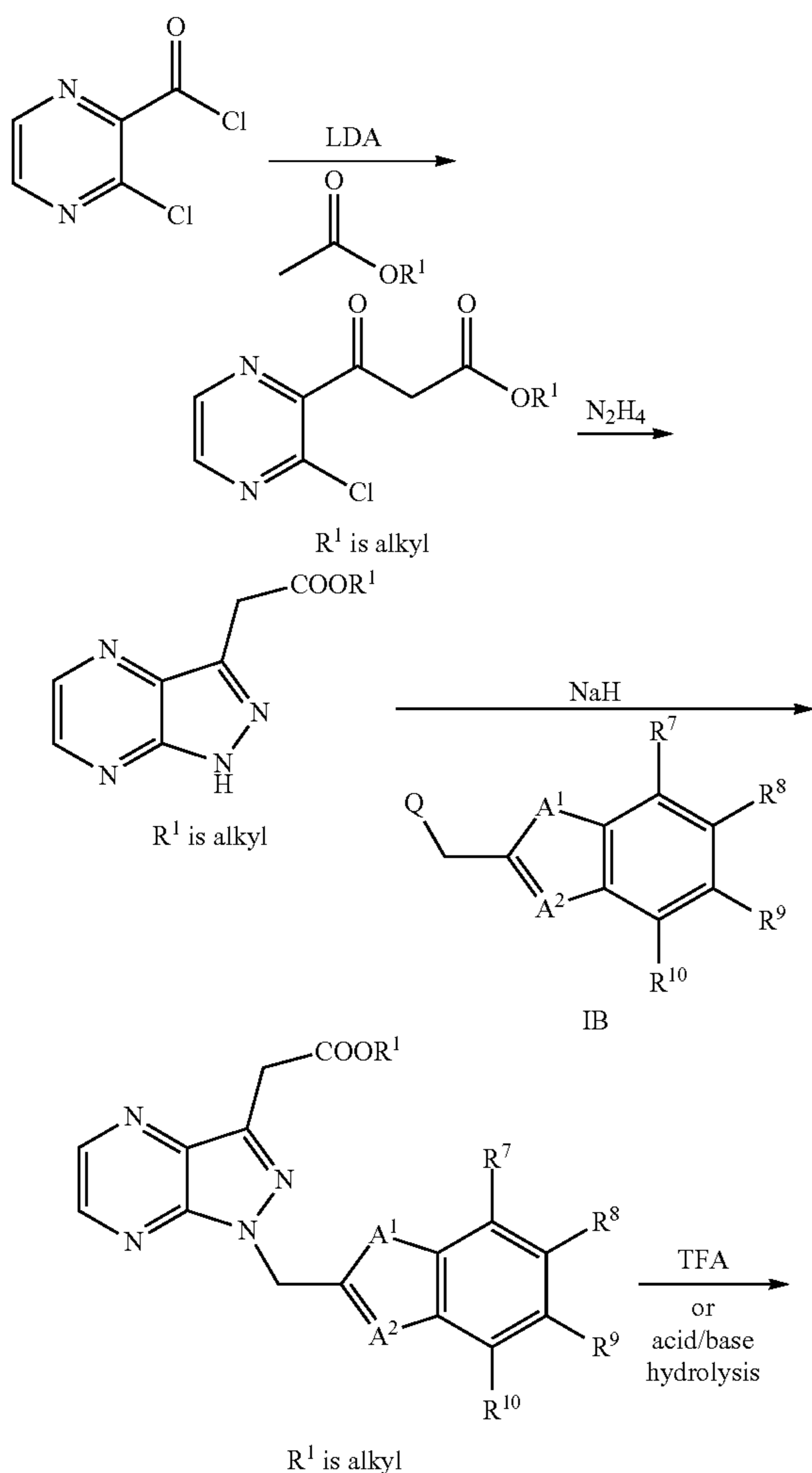
Scheme 21
