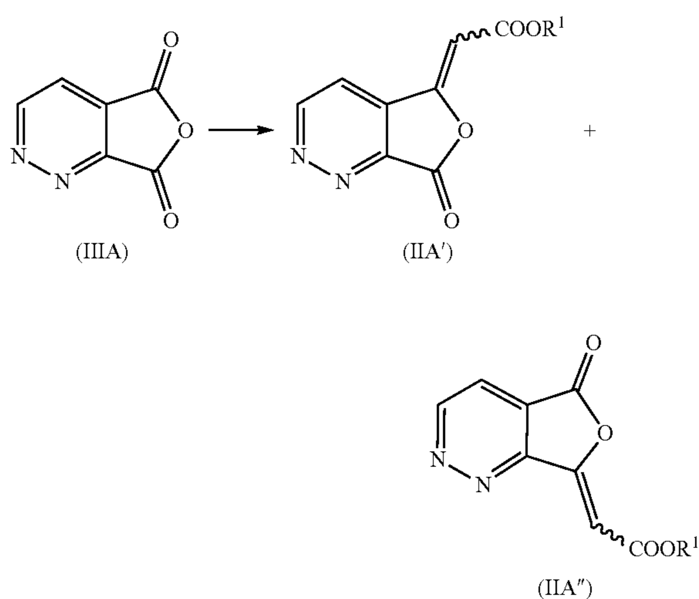
Scheme 7
