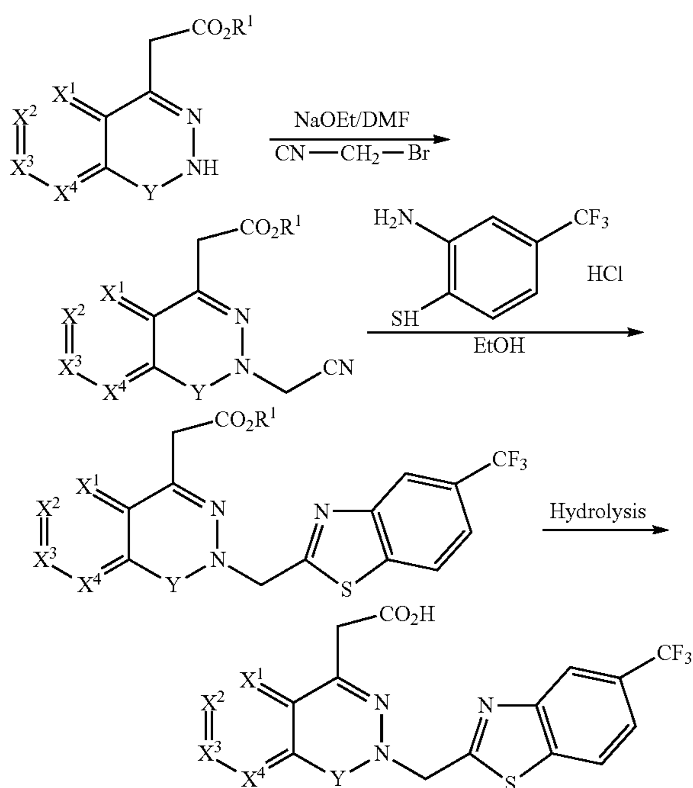
Scheme 15
