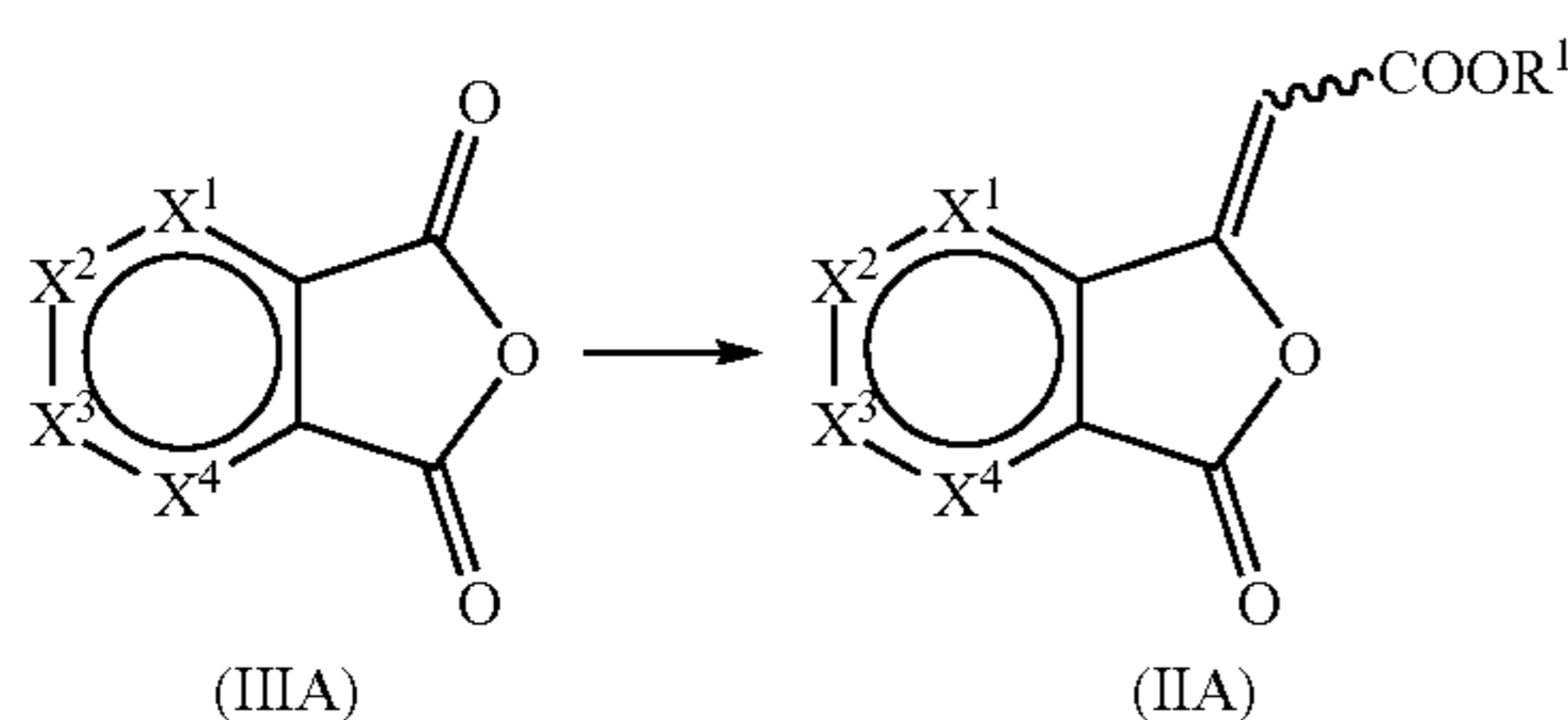
Scheme 6
