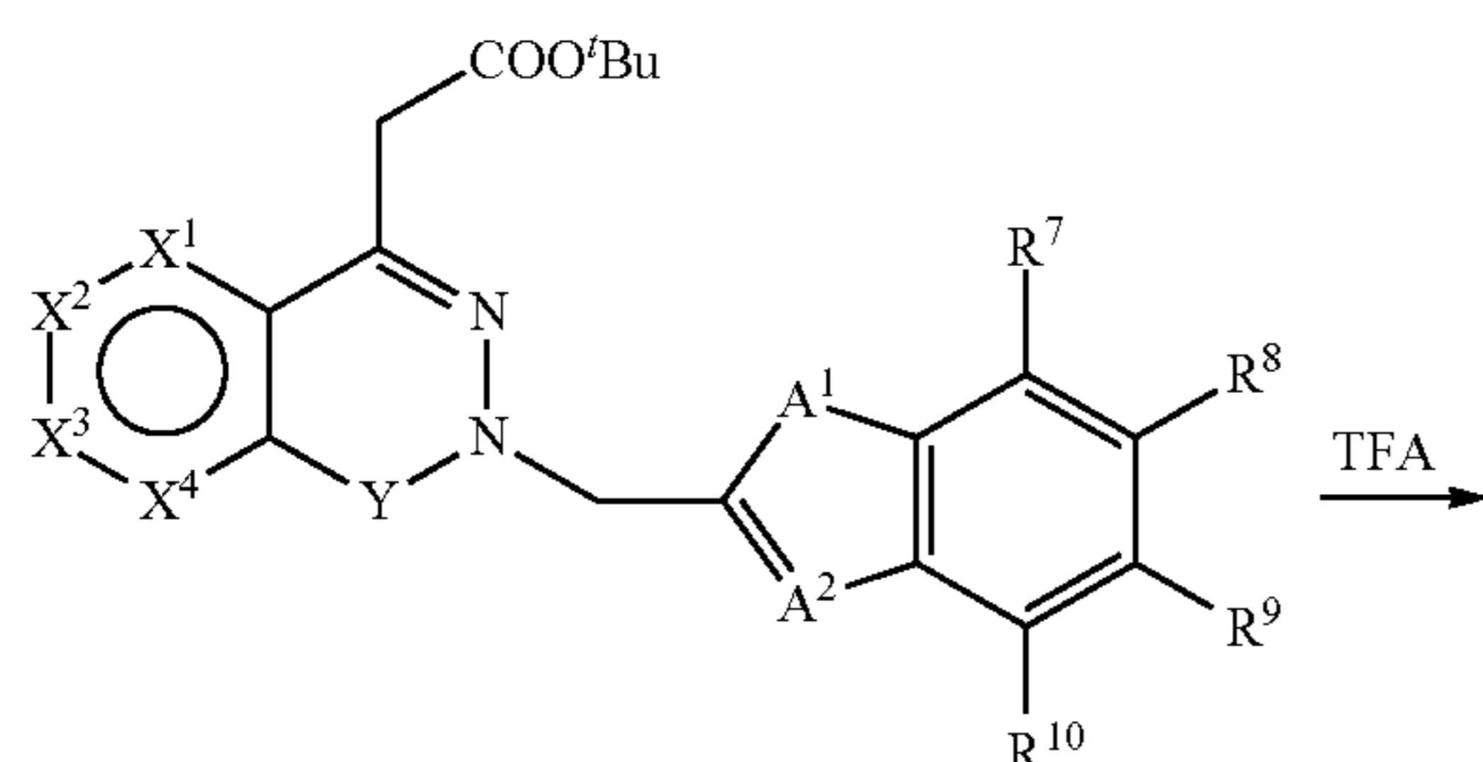
Scheme 3
