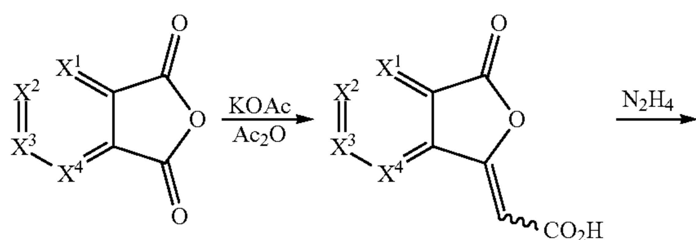
Scheme 13
