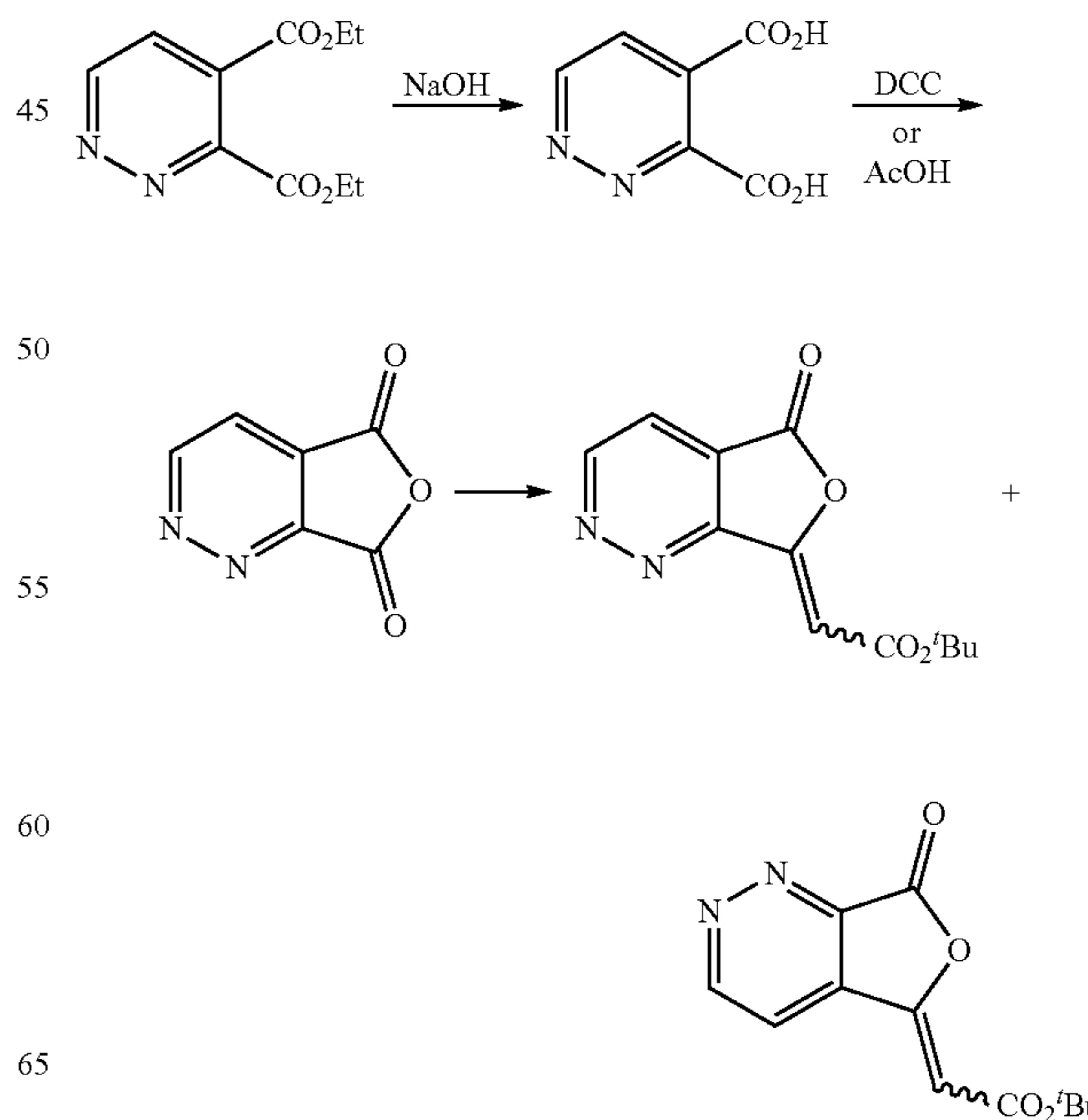
Scheme 19
