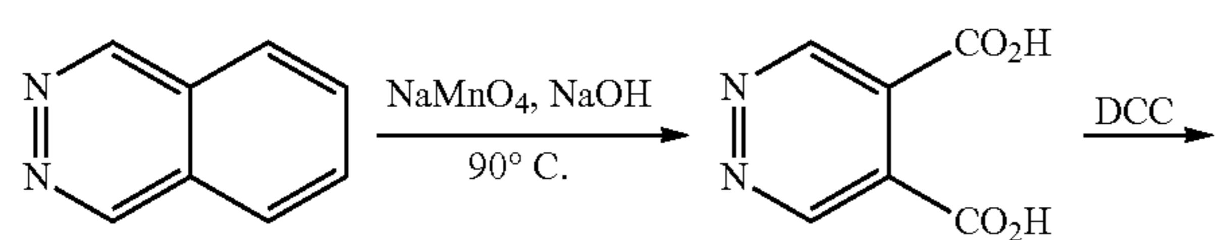
Scheme 18
