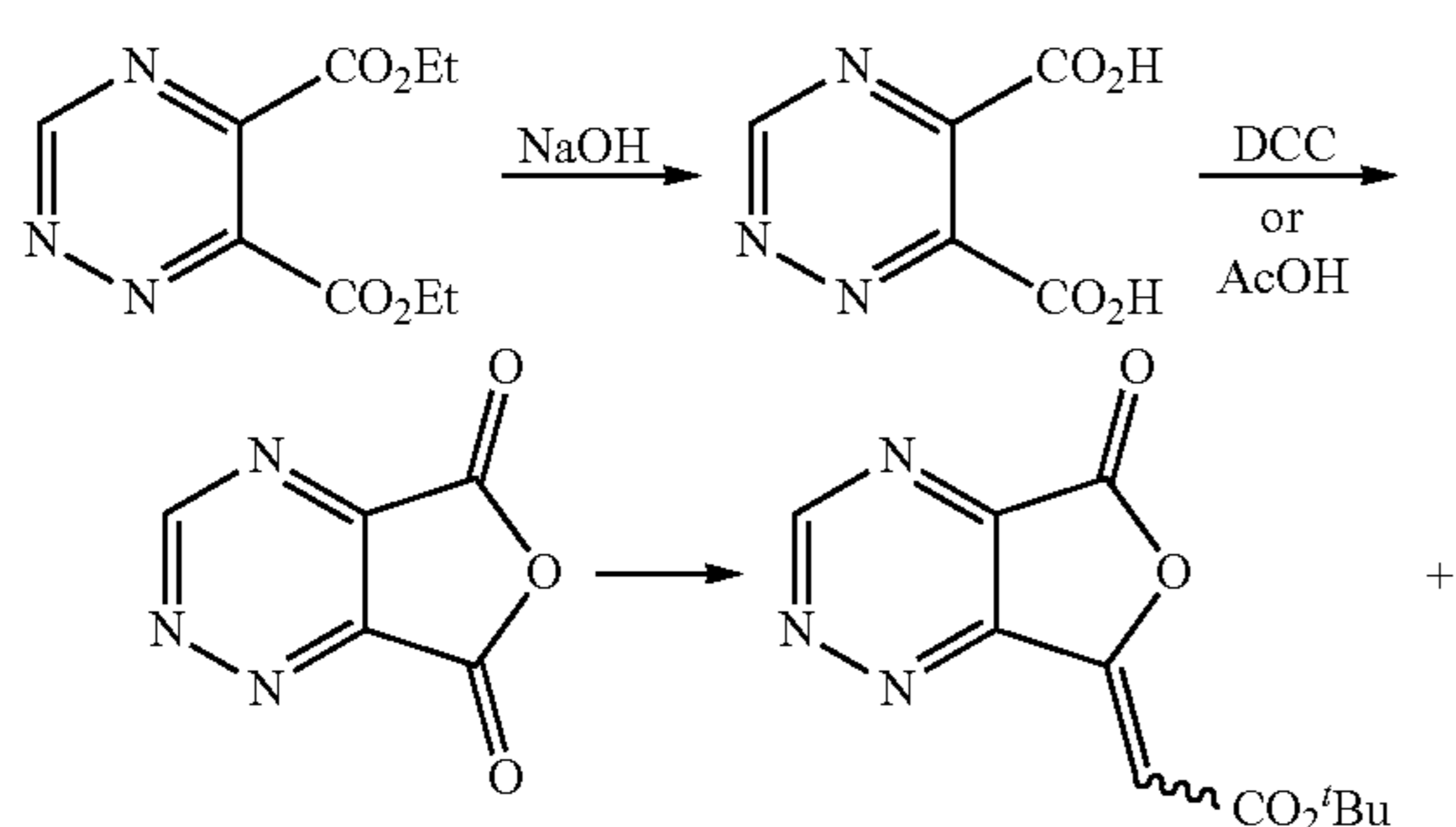
Scheme 16
