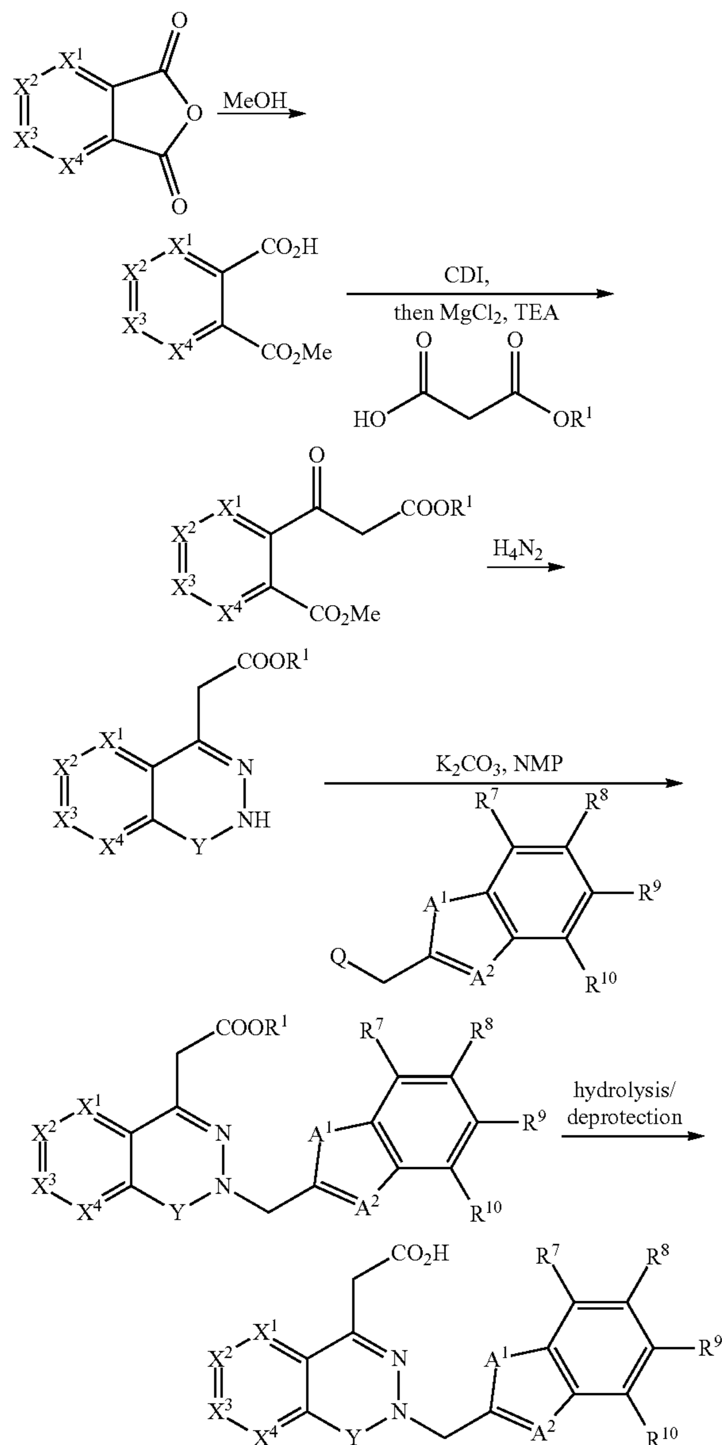
Scheme 2
