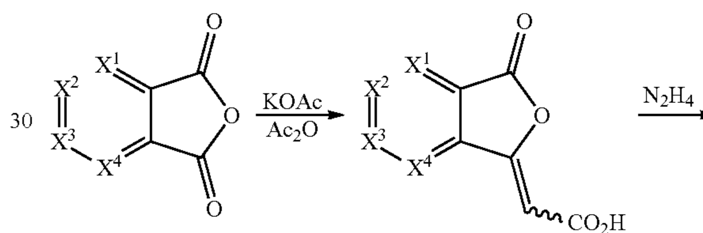
Scheme 14
