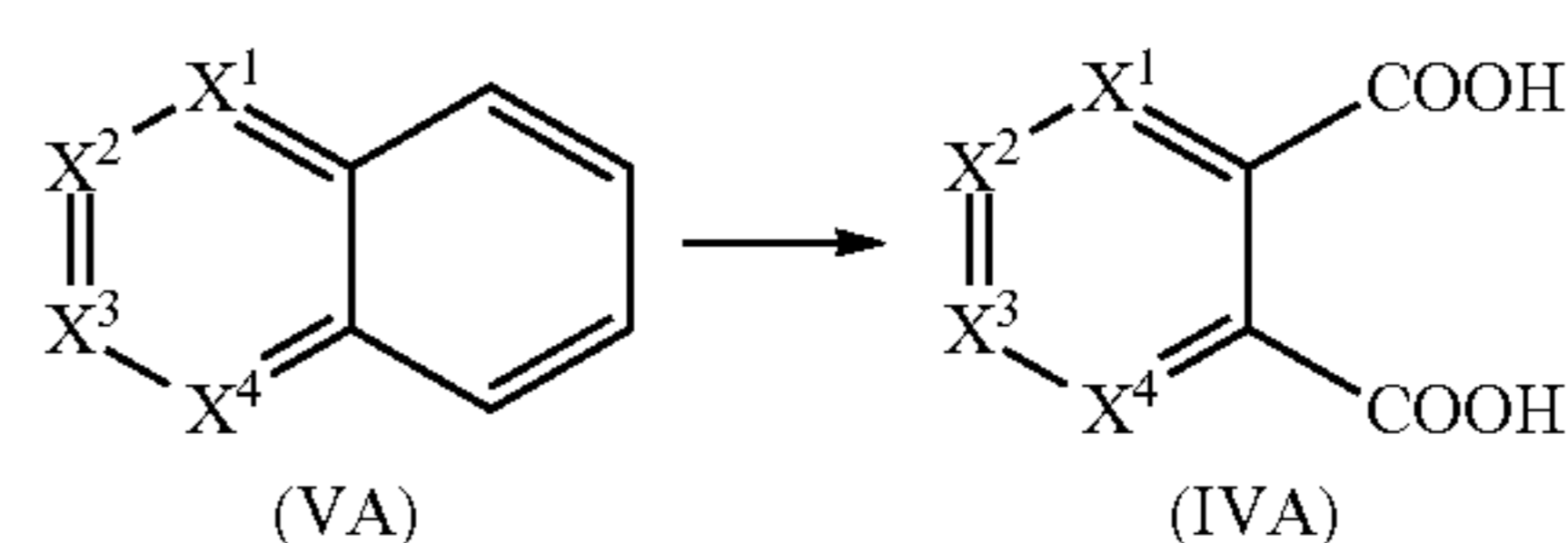
Scheme 9
