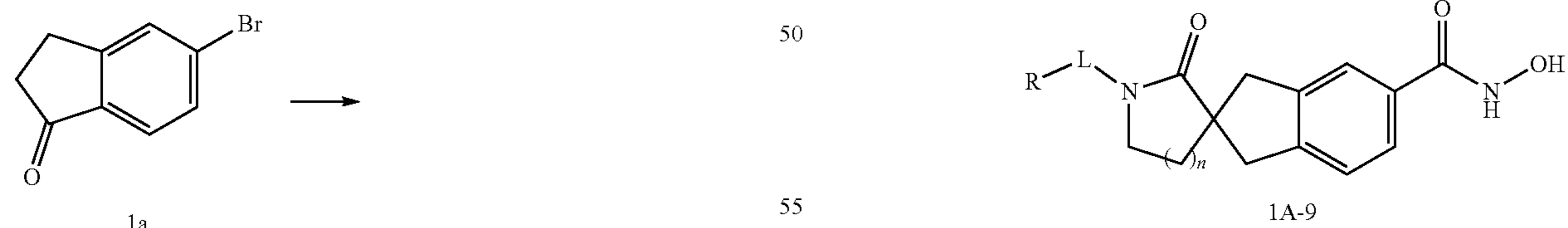
Scheme 1. General Synthesis of compounds of Formula IA-9
