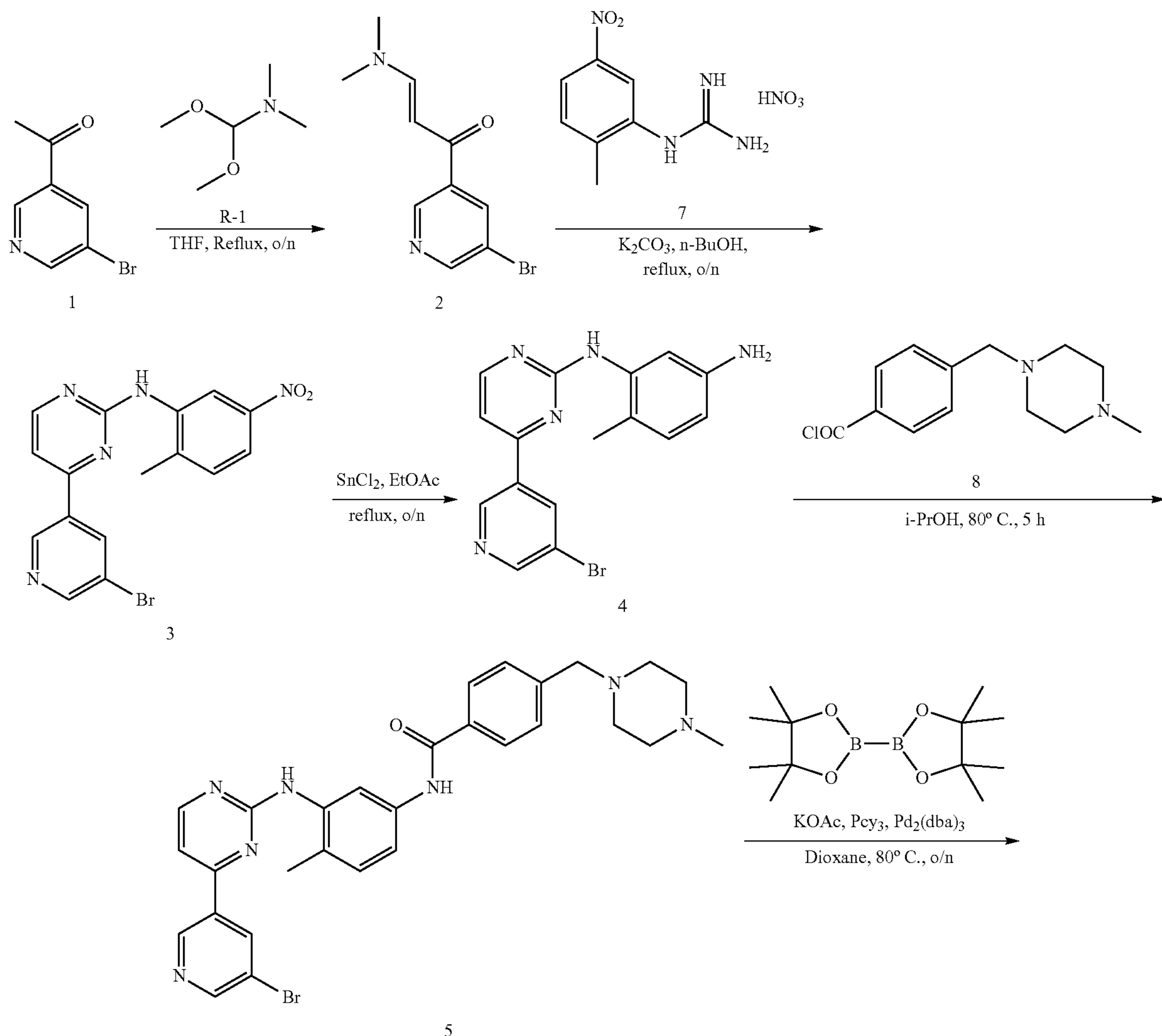
Scheme 1: Synthesis of Intermediates 5 and 6
