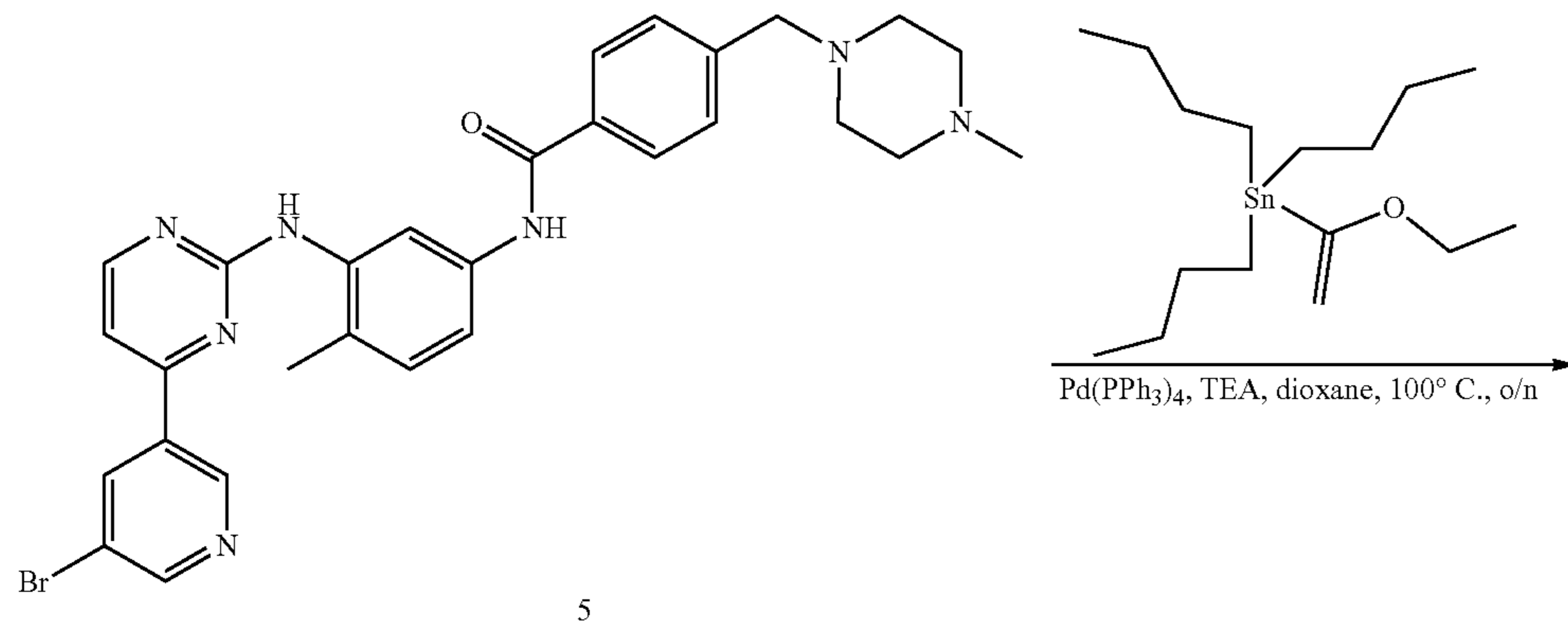
Scheme 2: Synthesis of Intermediates 7, 8 and 9
