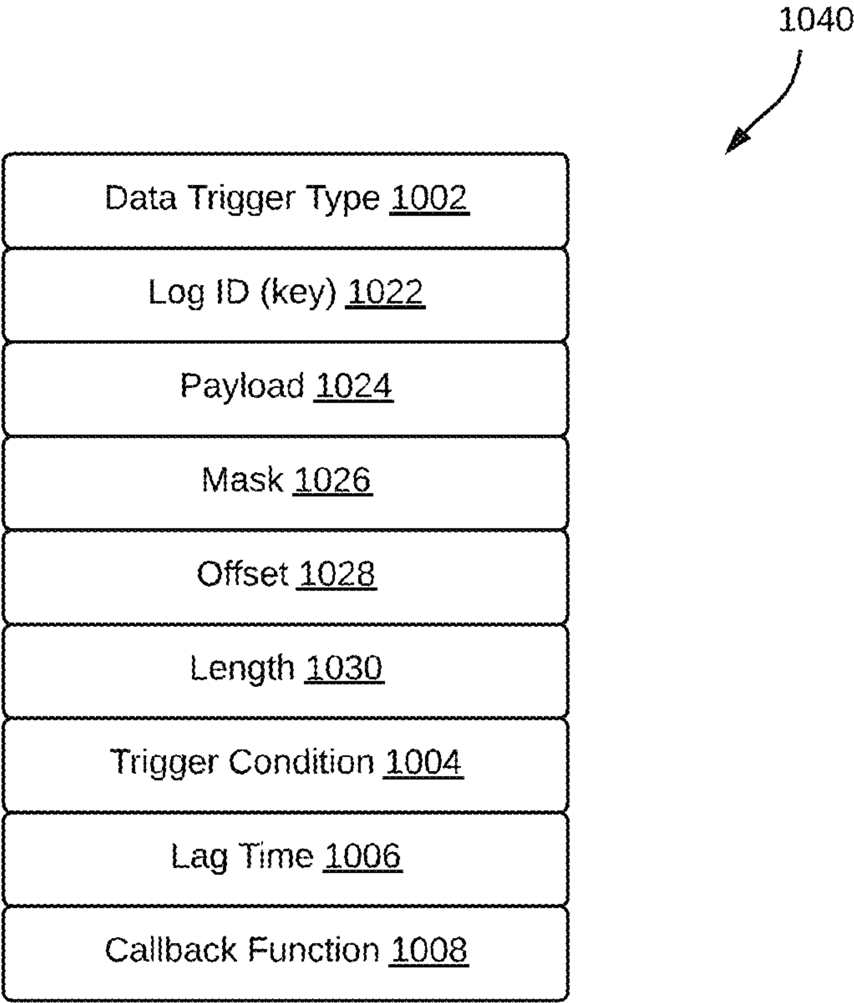
Log and Trigger Configuration Structure
