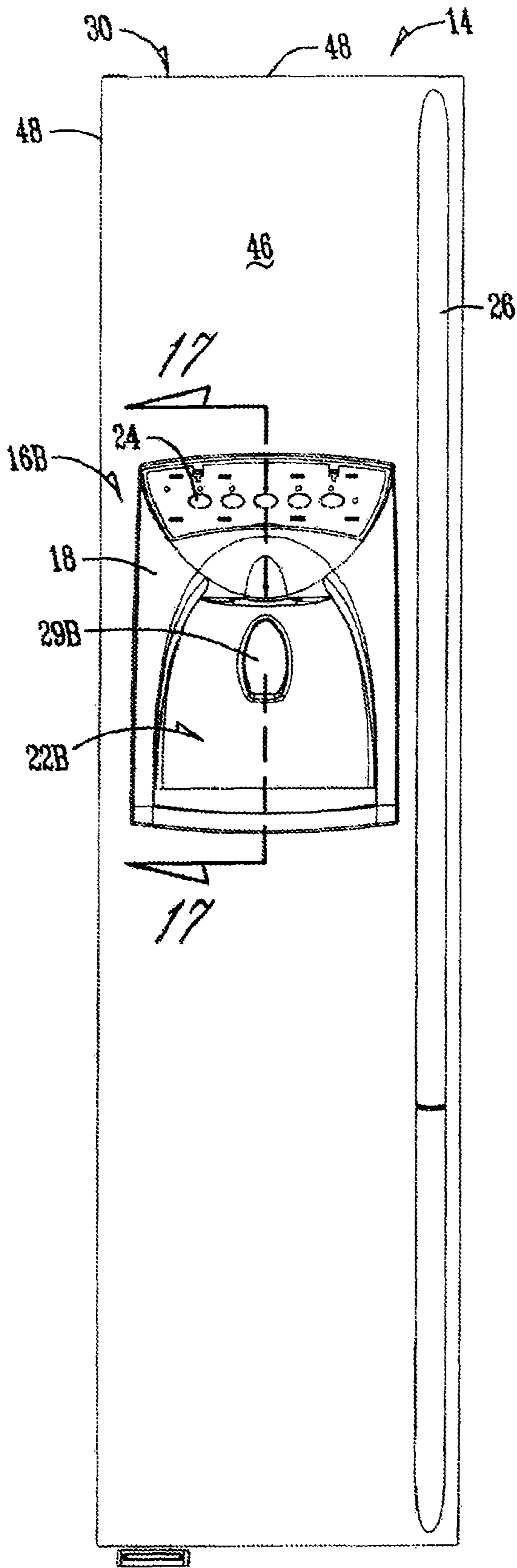
Fig. 15 (Prior Art)
