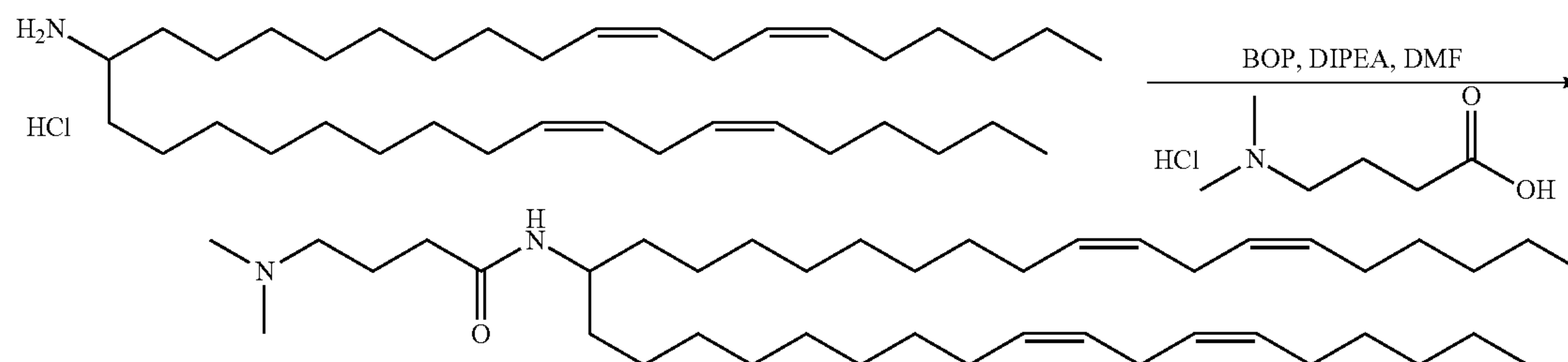
Scheme 11
