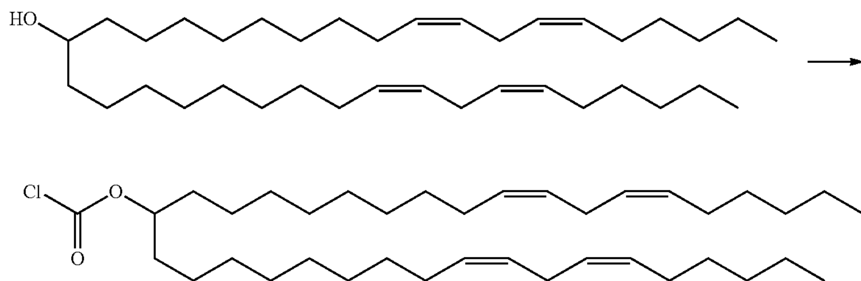
Scheme 4
