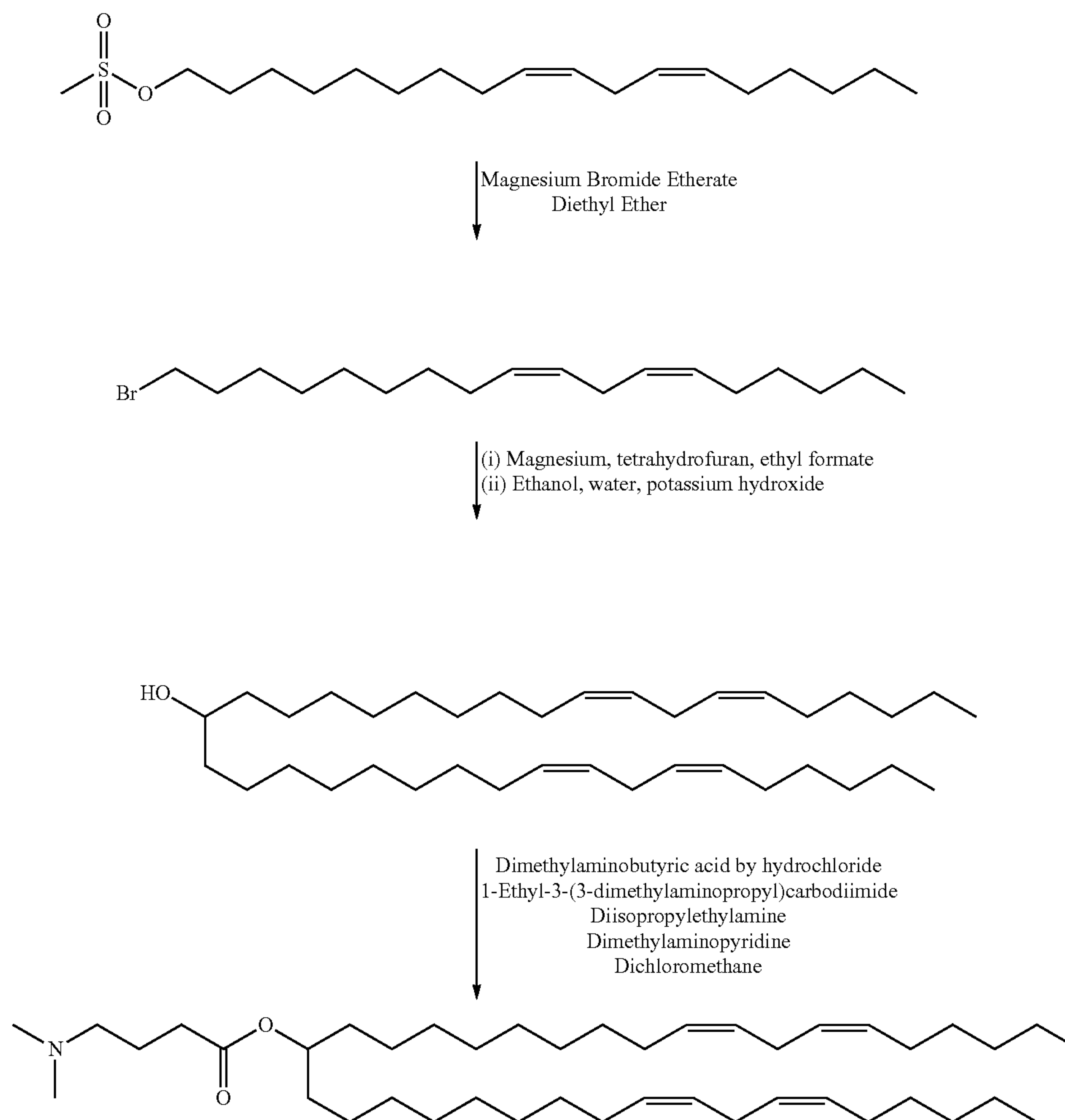
Scheme 1
