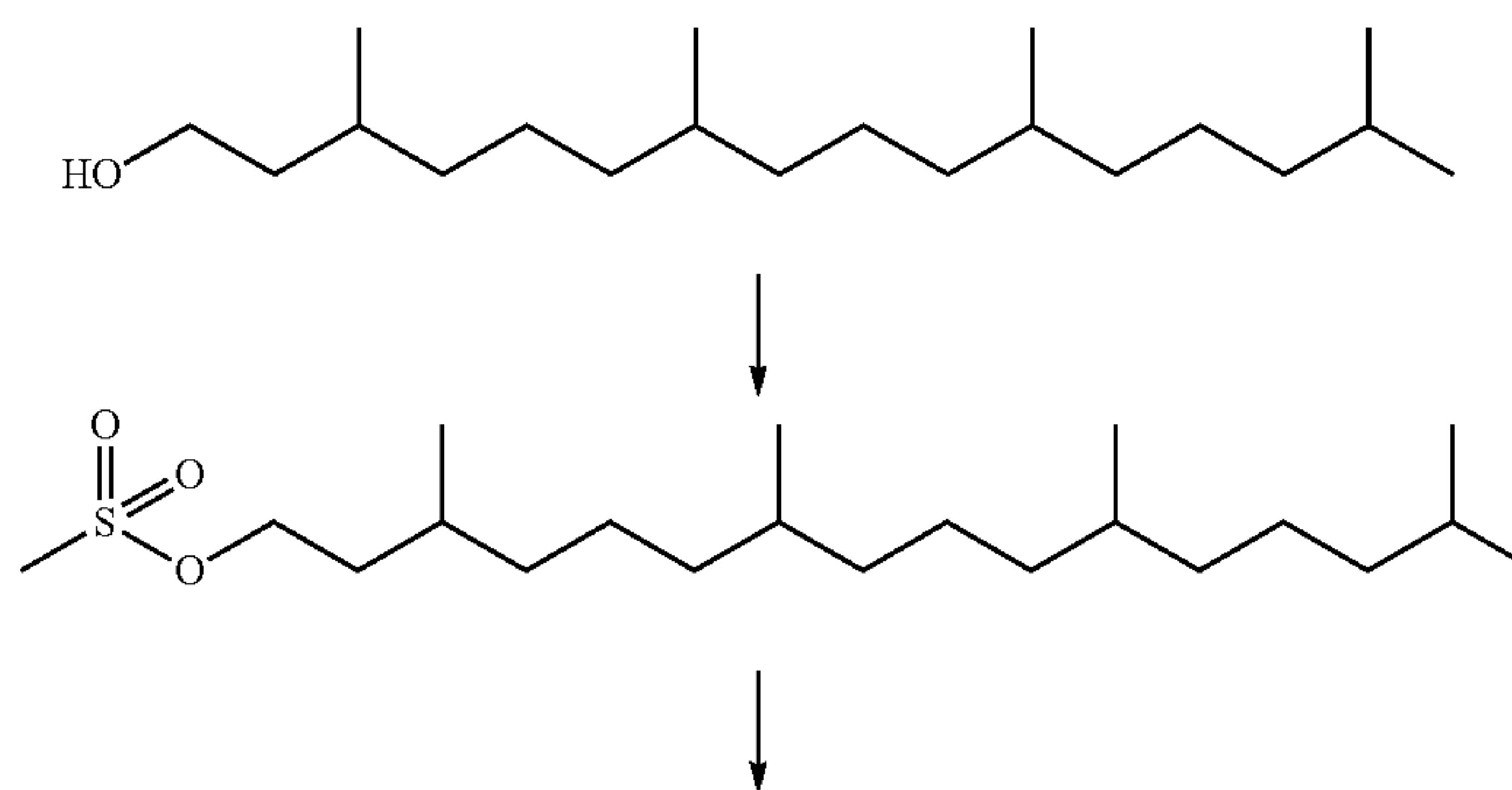
Scheme 12
