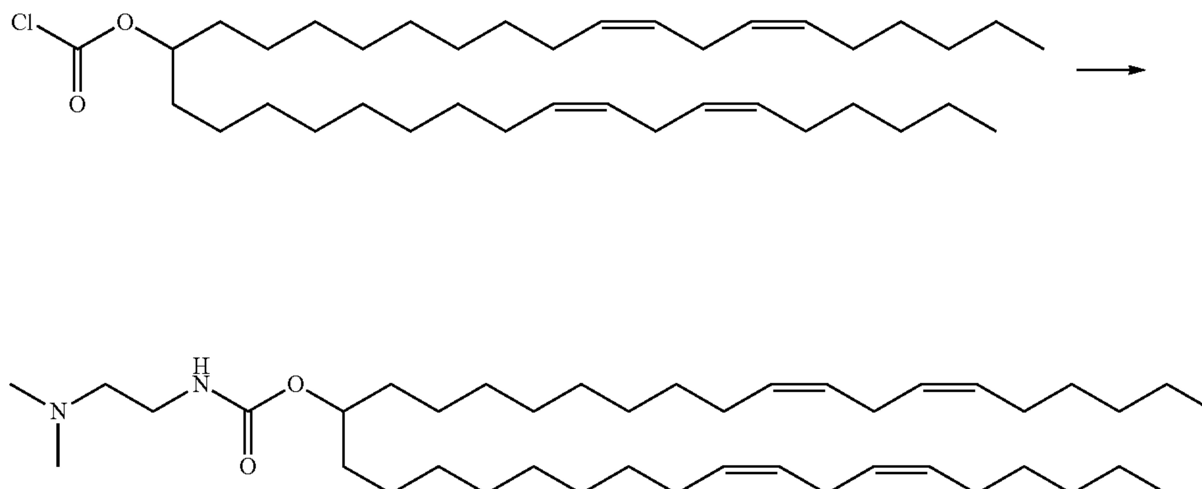
Scheme 7
