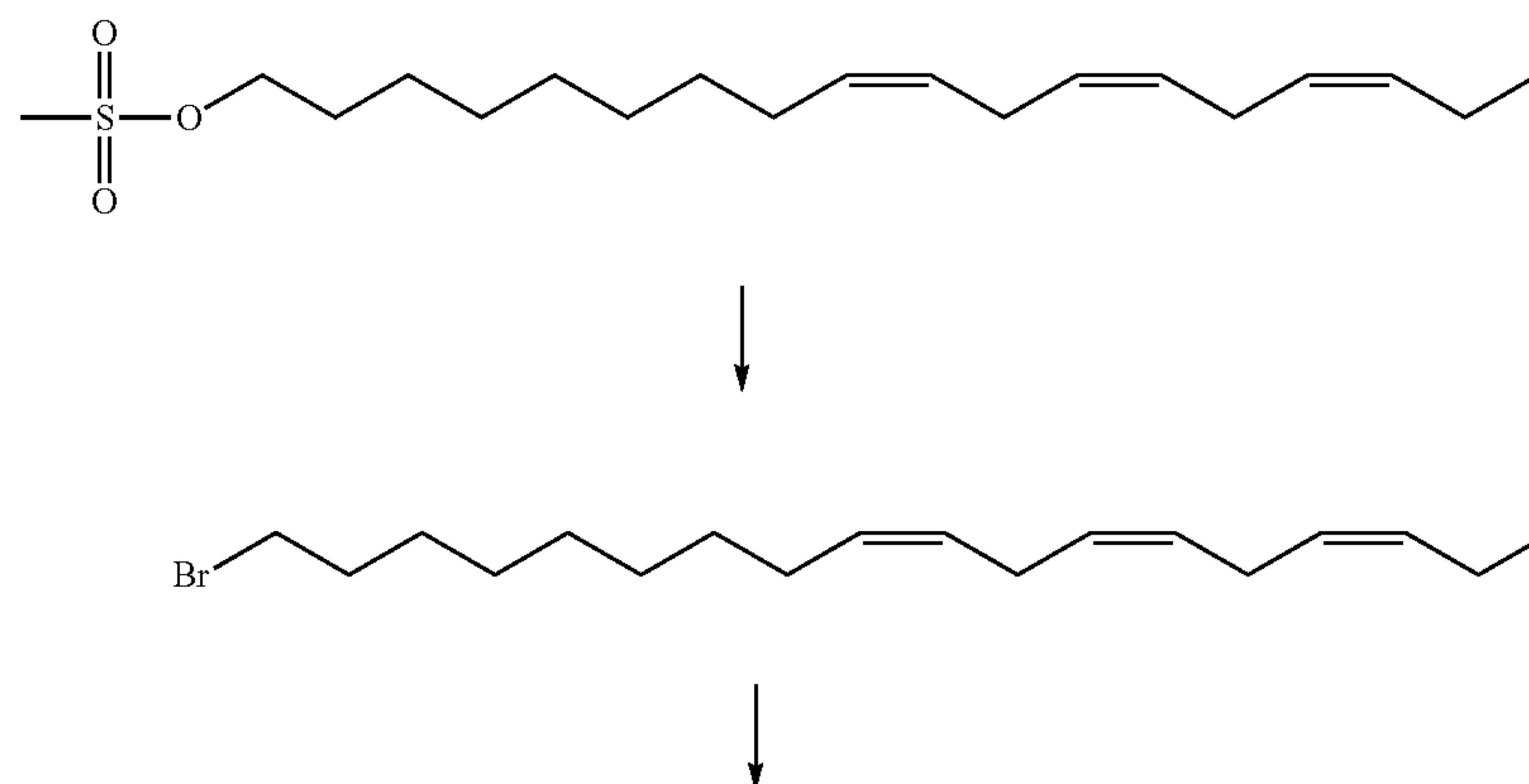
Scheme 2
