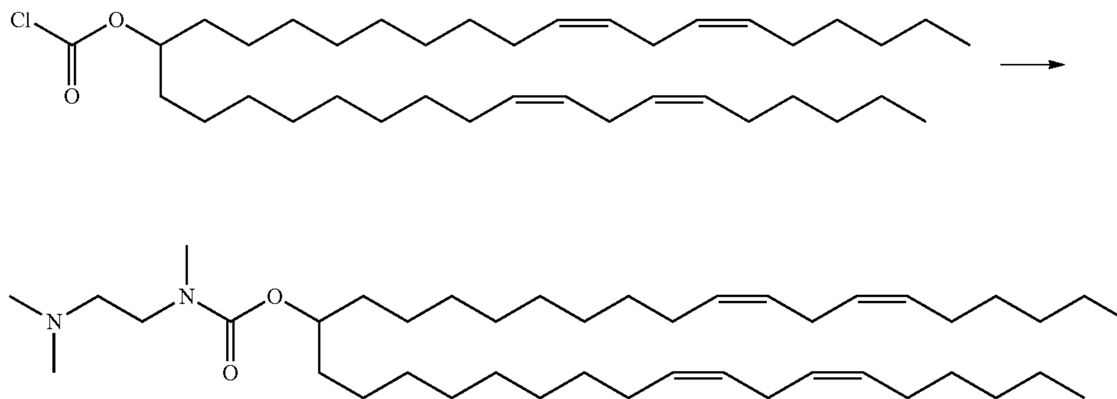
Scheme 6
