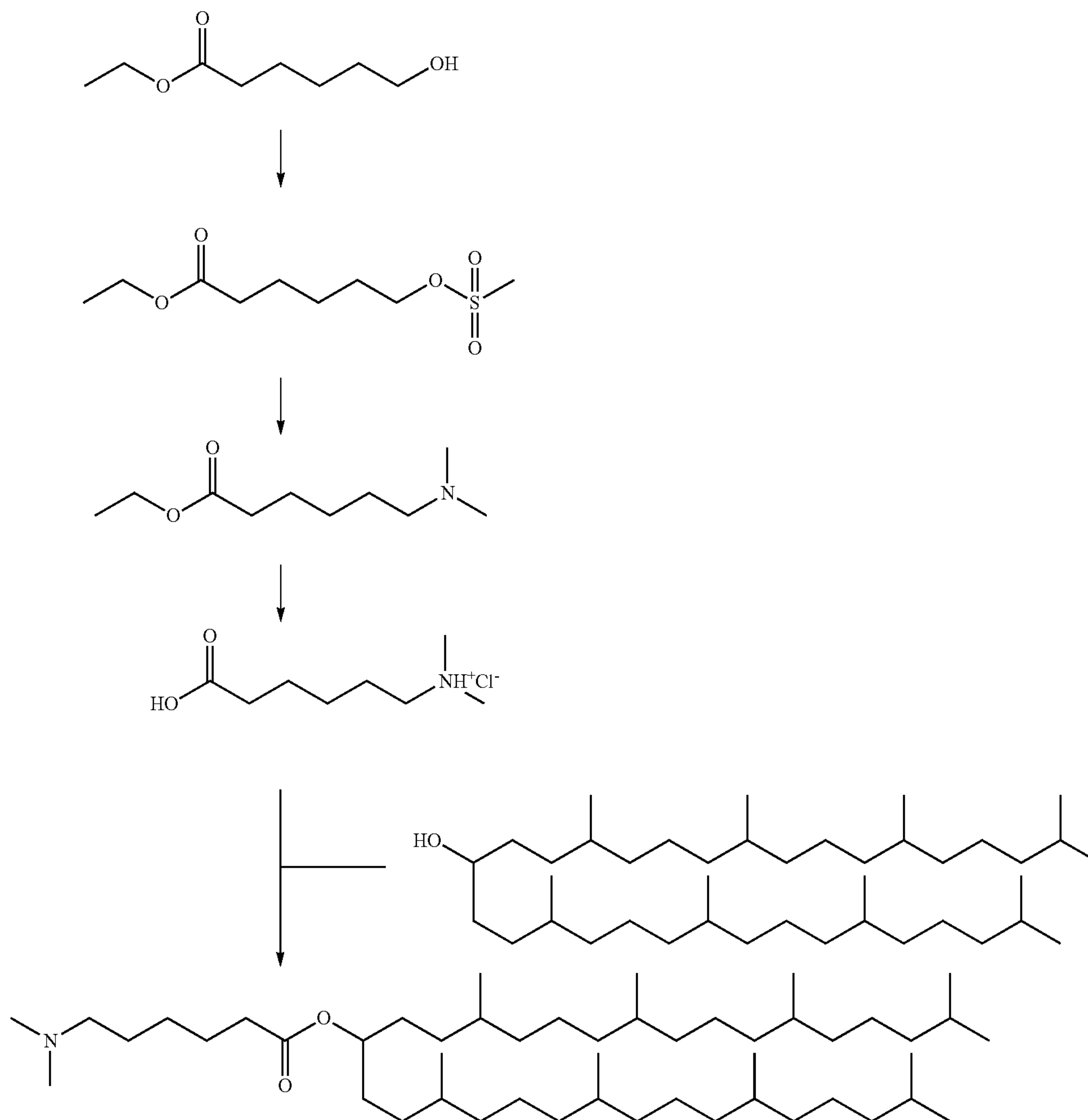
Scheme 14
