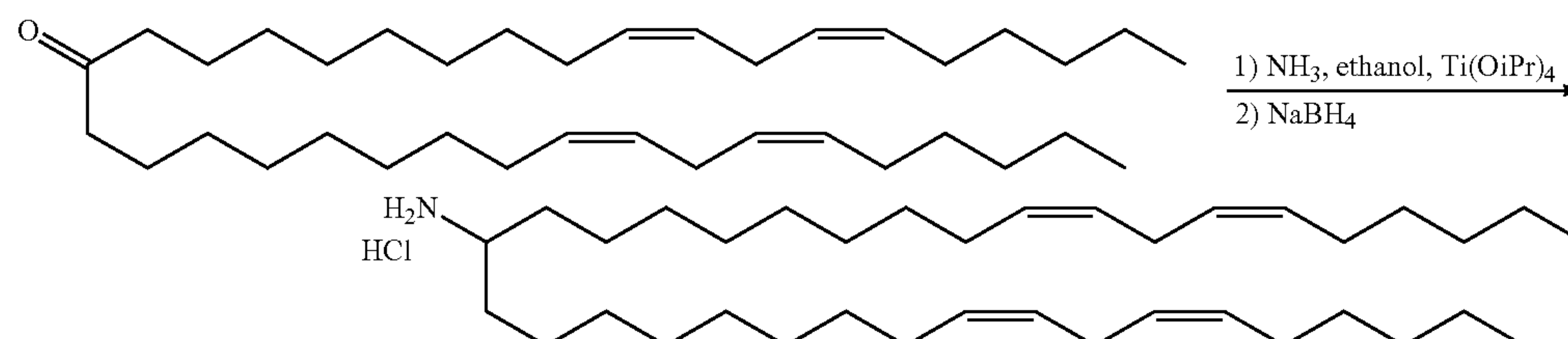
Scheme 10
