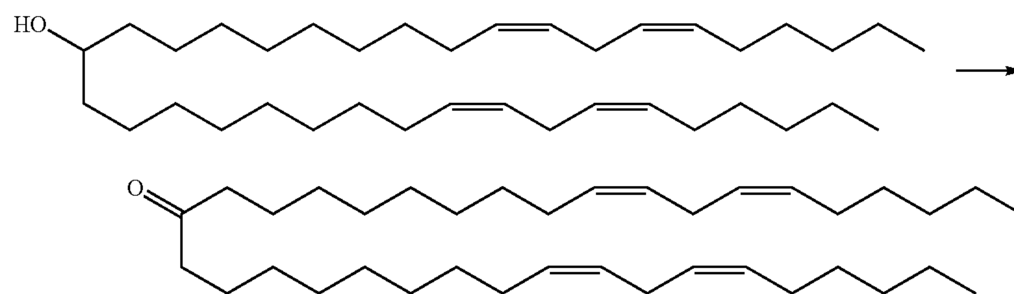
Scheme 9
