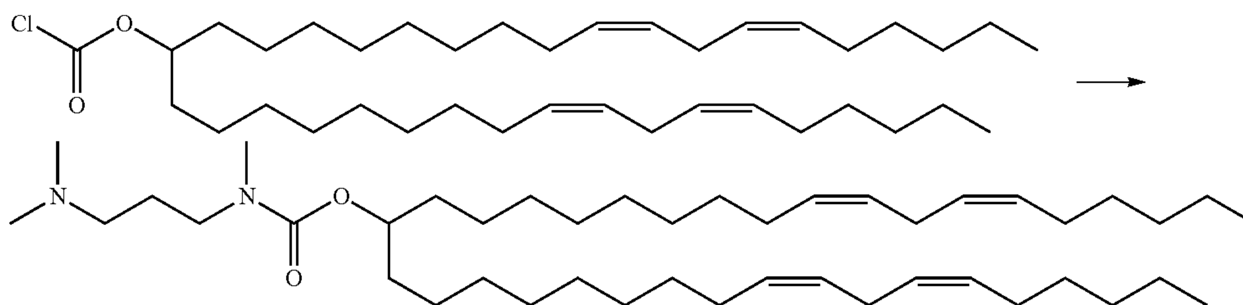
Scheme 5
