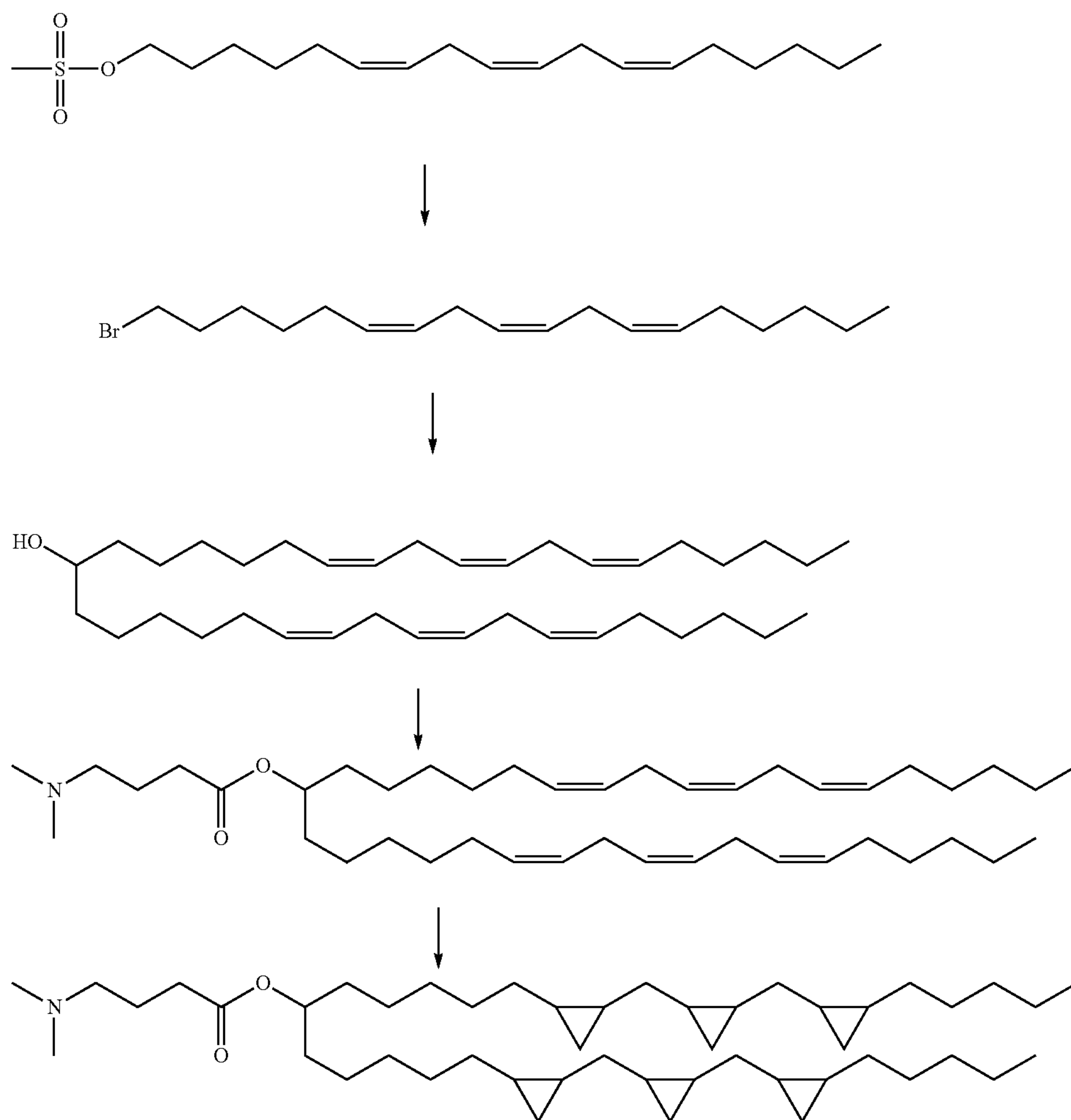
Scheme 3
