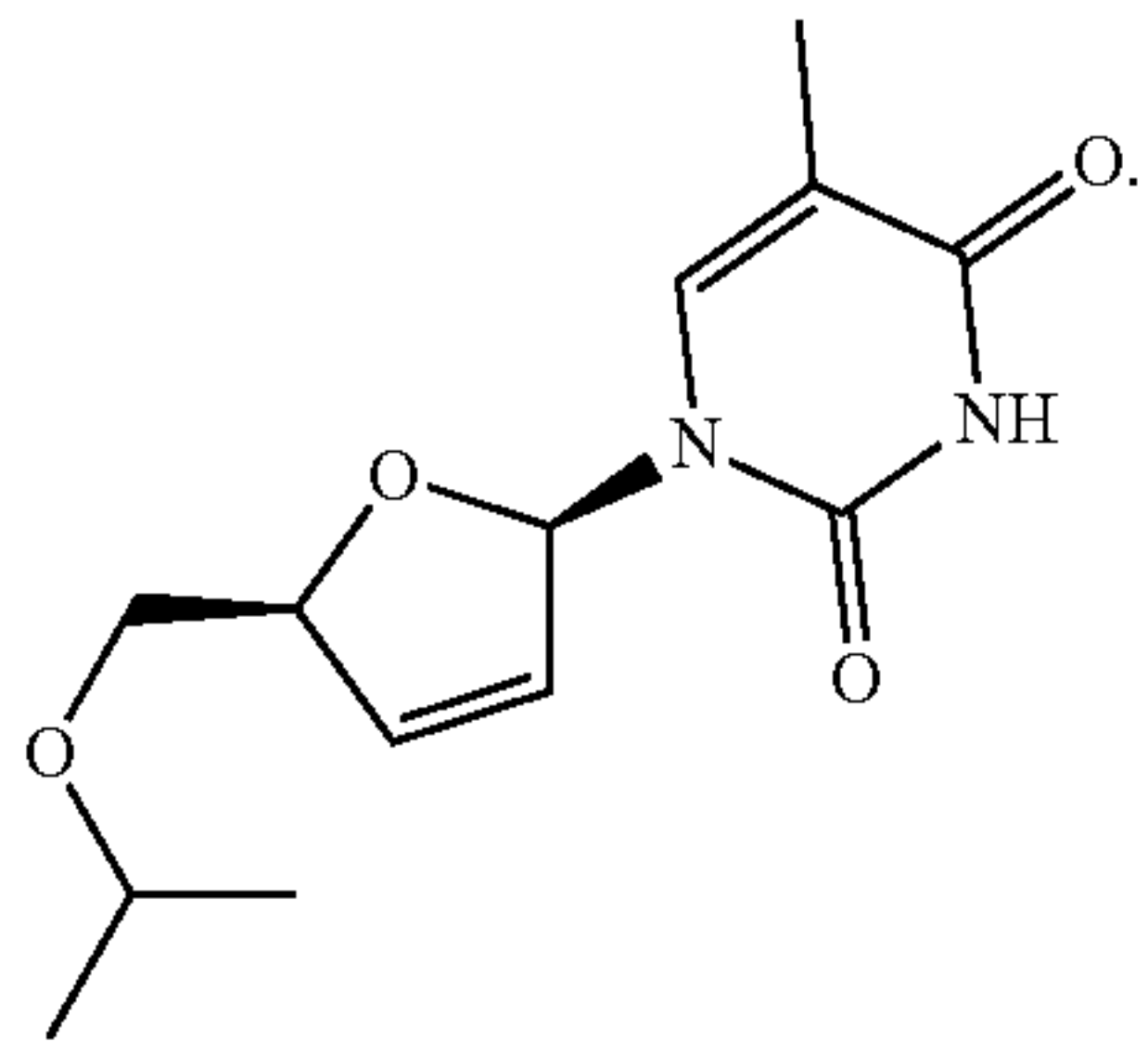
O-isopropyl-d4T
