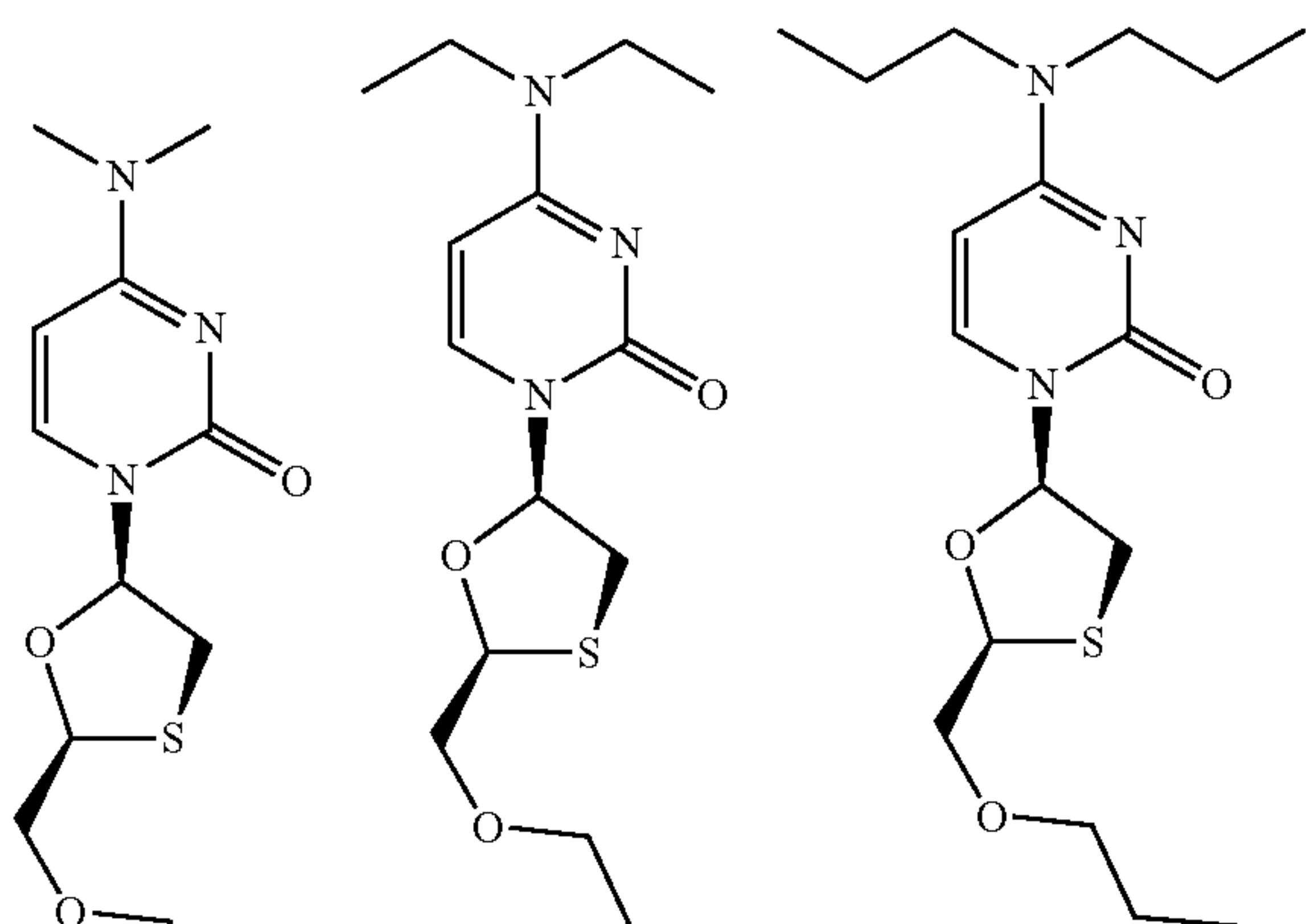
3-Me-3TC
