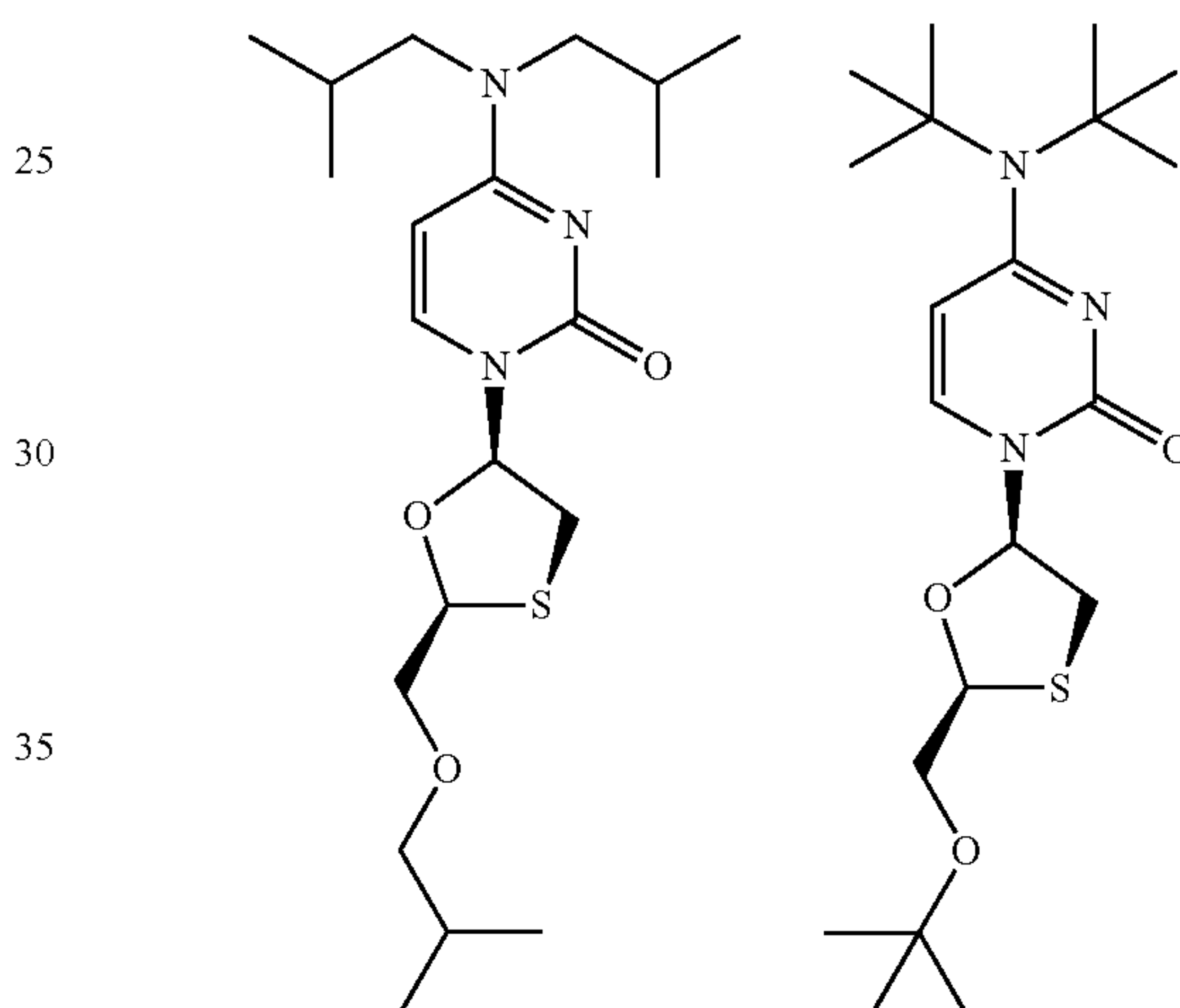
3-Isobutyl-3TC
