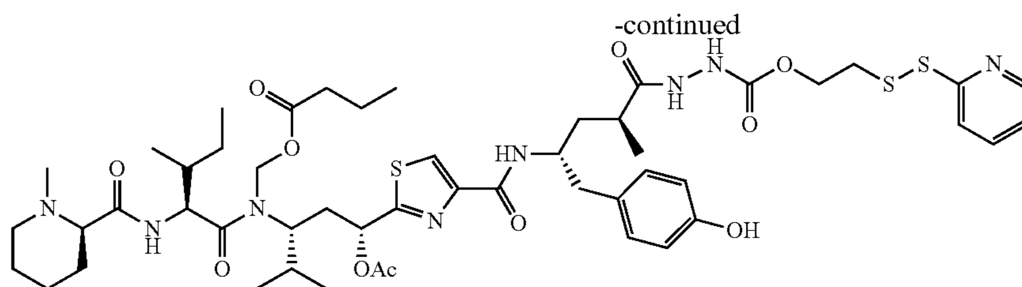
EC0312 C_{50}H_{72}N_8O_{11}S_3 Mol. Wt.: 1057.35
