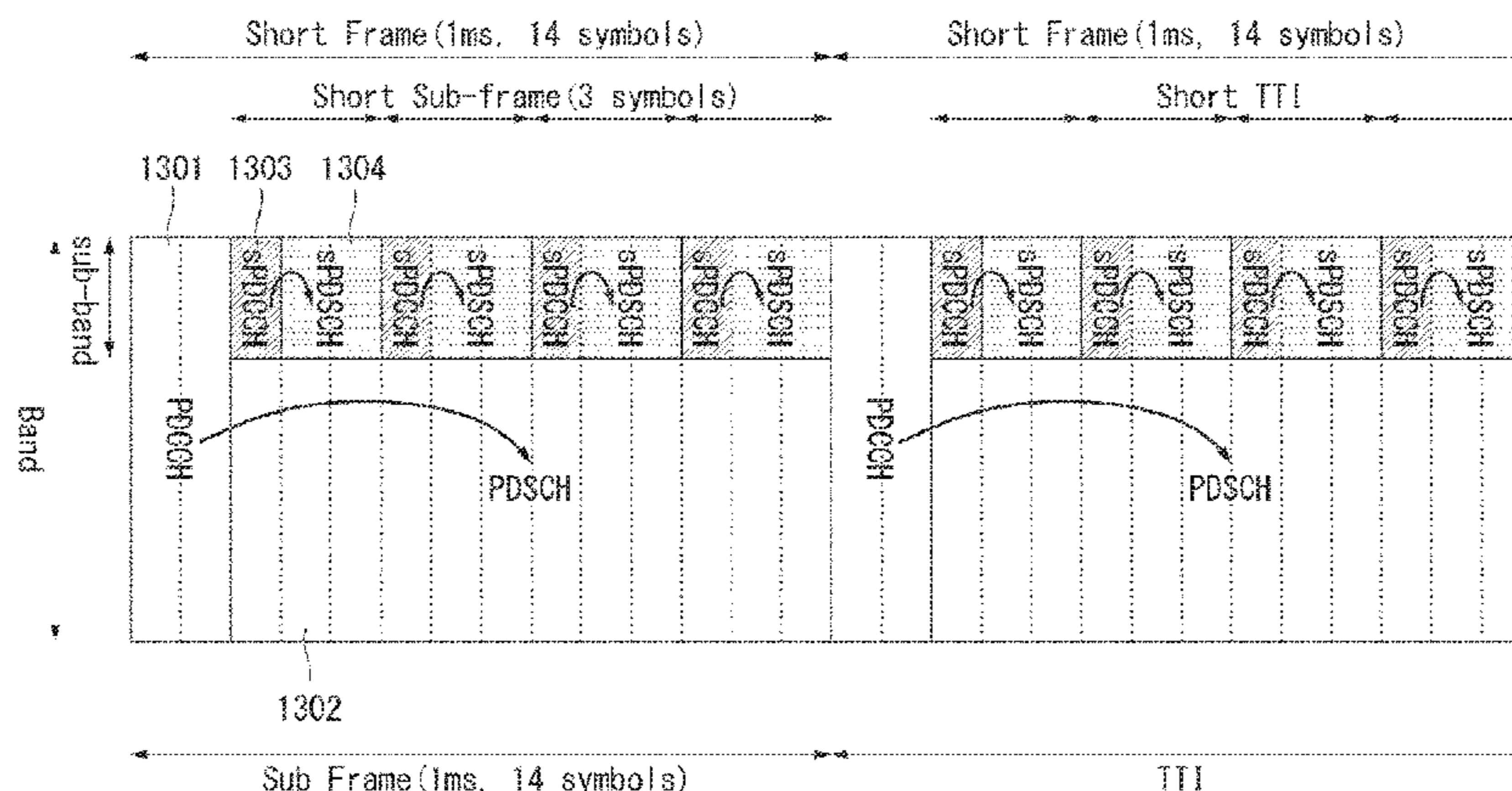
Short Frame structure for low latency
