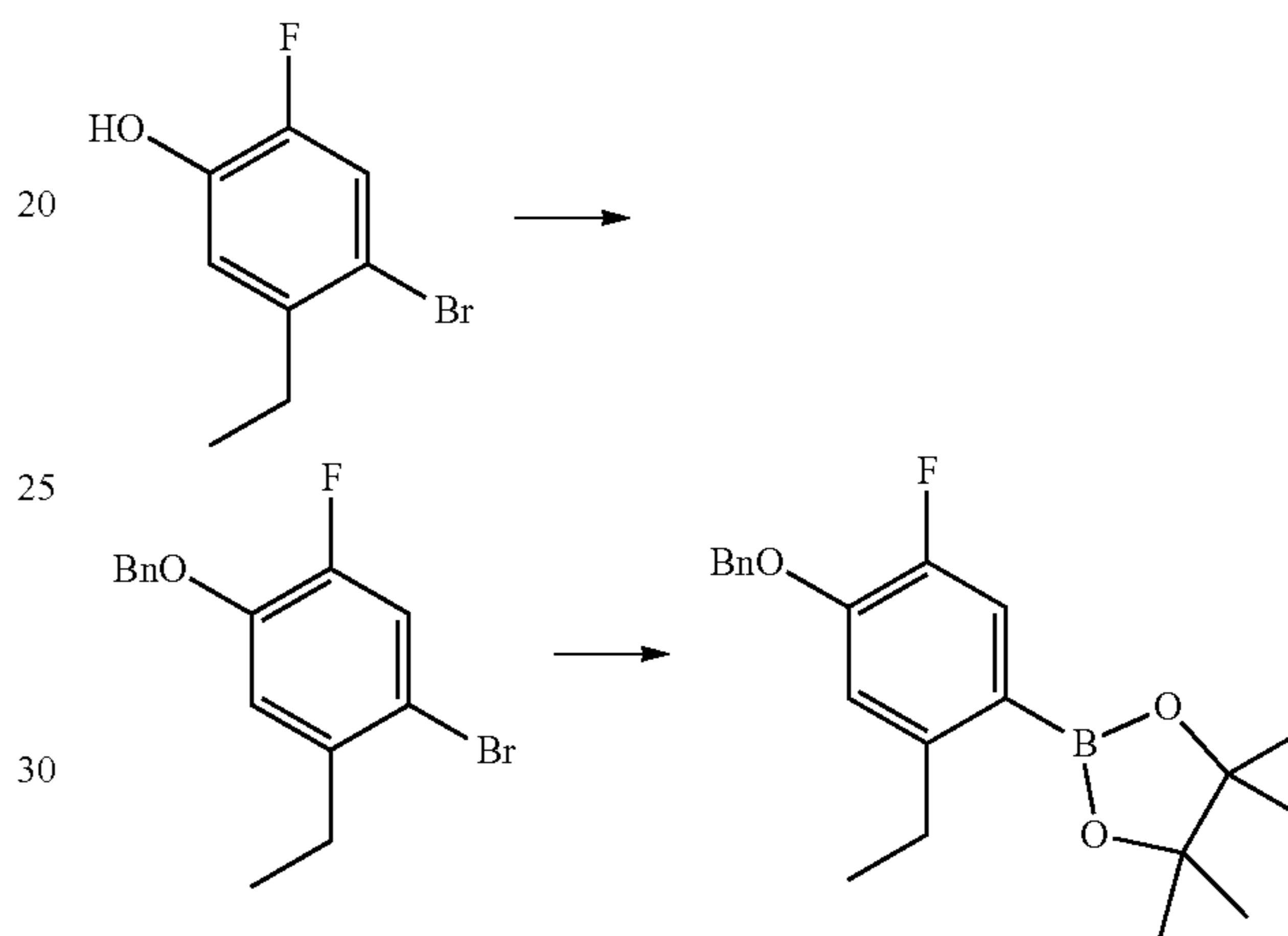
(a) 1-(Benzyloxy)-4-bromo-5-ethyl-2-fluorobenzene
